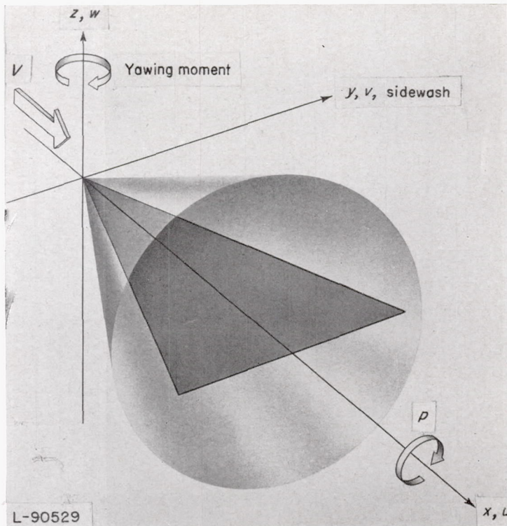
FIGURE 1.—Triangular wing oriented with respect to body system of axes used in analysis and associated symbol data.
