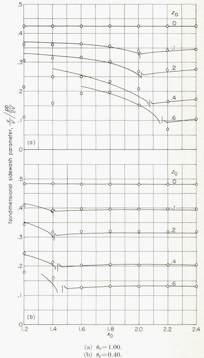
FIGURE 7.—Comparison of lifting-line and lifting-surface sidewash for \theta_0 = 1.00 and 0.40 . Circles represent points calculated by lifting-line method.
