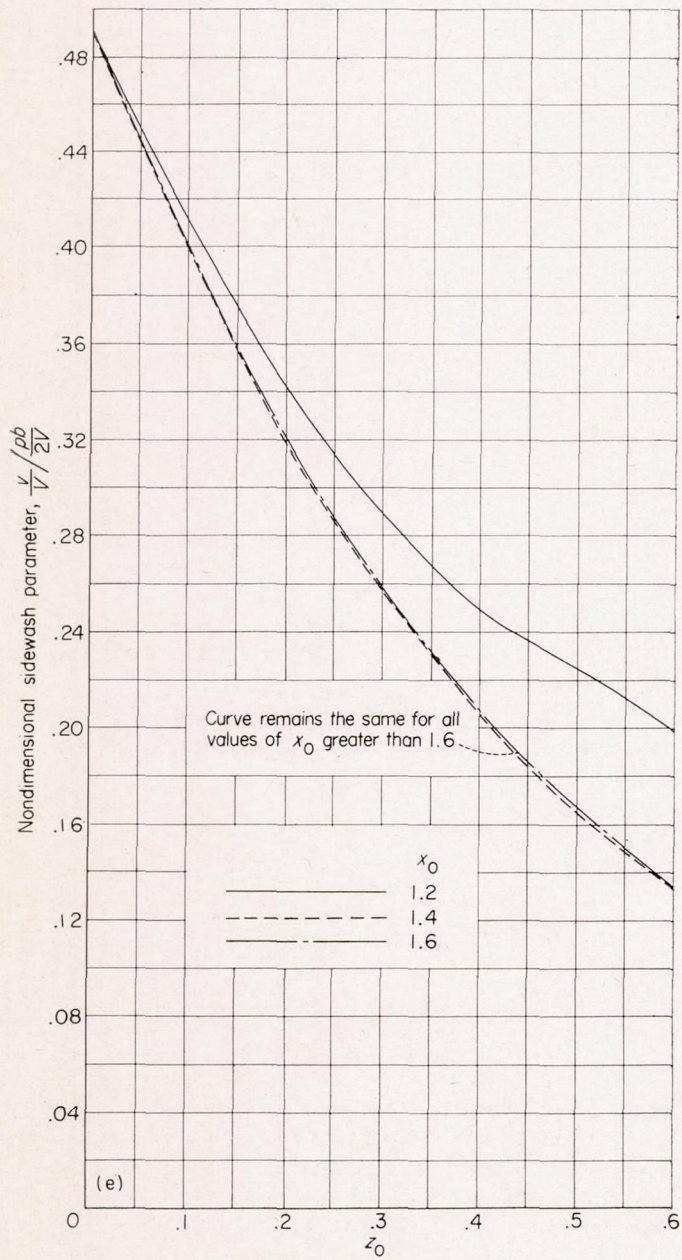
(e) \theta_0 = 0.30 . FIGURE 5.—Concluded.
