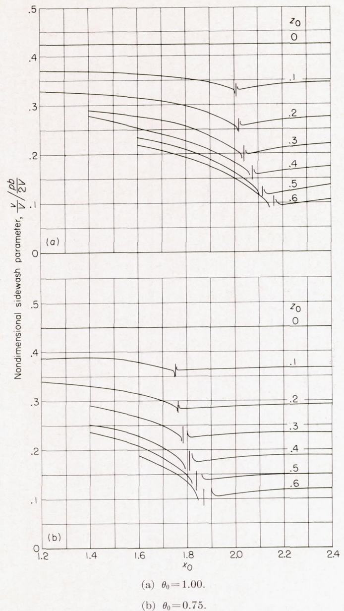
FIGURE 4.—Longitudinal variation of nondimensional sidewash parameter \frac{v/V}{pb/2V} in x_0z_0 -plane behind triangular wing for a number of values of z_0 and \theta_0 .
