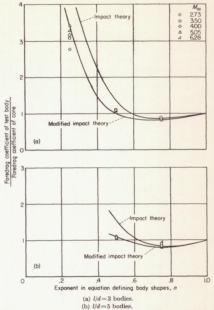
FIGURE 7.—The ratios of foredrag coefficients of test bodies to foredrag coefficients of cones as functions of the exponent, n , in the equation defining body shapes.
