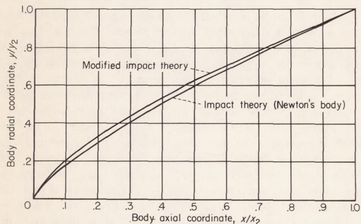
FIGURE 8.—The effect of centrifugal forces on the shape of the minimum drag body of given length and base diameter ( l/d=6.18 ).
