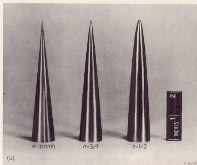
(b) Fineness ratio 5 bodies.
