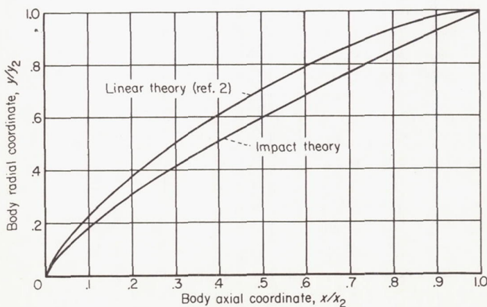
FIGURE 3.—Comparison of minimum drag bodies of given length and base diameter determined by linear theory and by impact theory.
