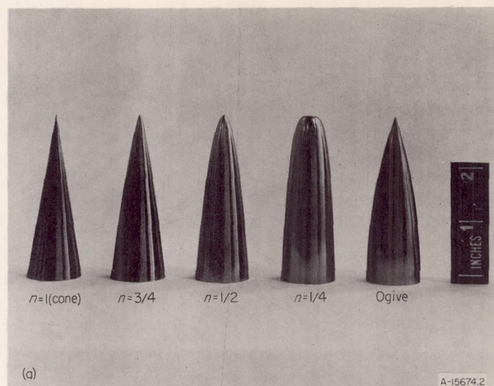
(a) Fineness ratio 3 bodies.
