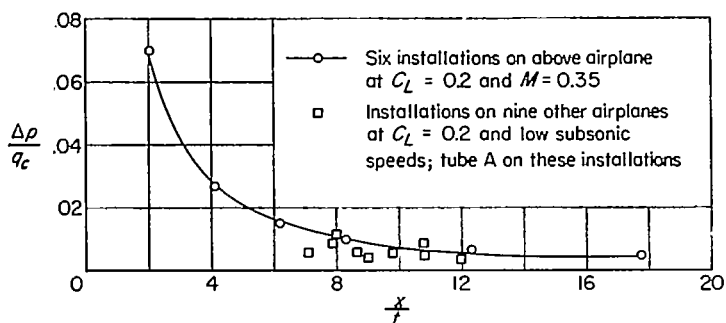
FIGURE 28.—Static-pressure errors at various distances ahead of the wing tips of unswept-wing airplanes (ref. 22).
