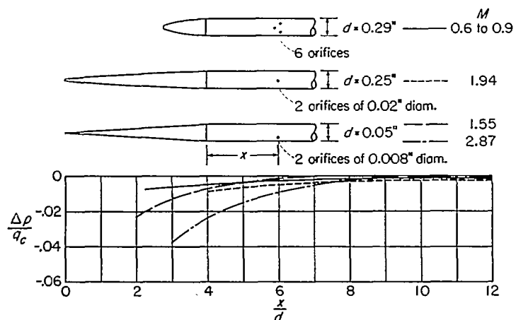
FIGURE 2.—Experimental pressure distribution along static-pressure tubes (refs. 6, 7, and 8).
