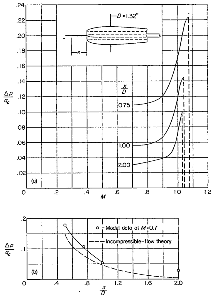
(a) Variation of static-pressure error with Mach number (inlet-velocity ratio 0.68 at M=0.7 ; 0.57 at M=1.0 ).
