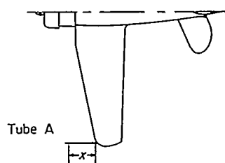
FIGURE 30.—Diagram showing position of shock waves with respect to a wing-tip installation on an unswept-wing airplane.
