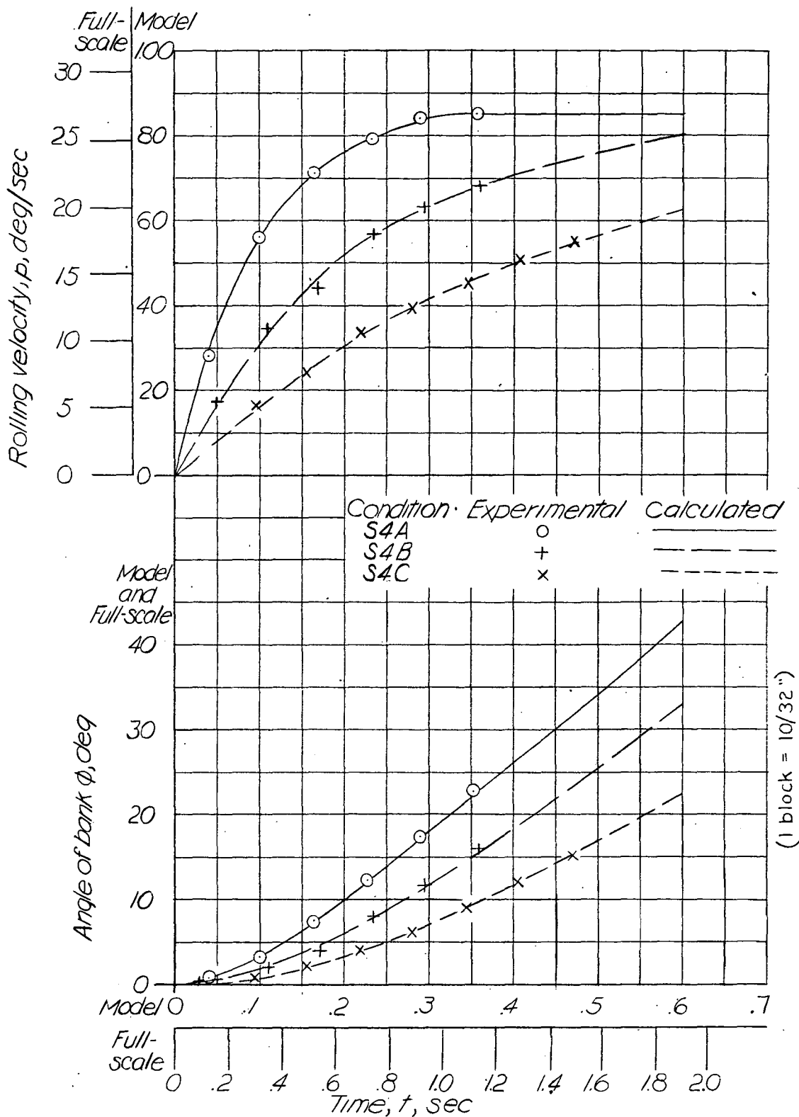
FIGURE 11.- Time histories of abrupt aileron maneuvers with different moment-of-inertia conditions. Small positive dihedral. Vertical tail 4. C_L=1.0 .
