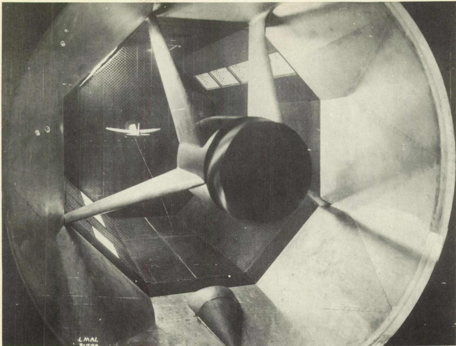
Figure 1.- Test section of NACA free-flight tunnel showing powered model in flight.
