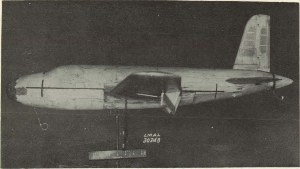
Figure 3.- Side view of model used in mass-distribution investigation in the NACA free-flight tunnel.
