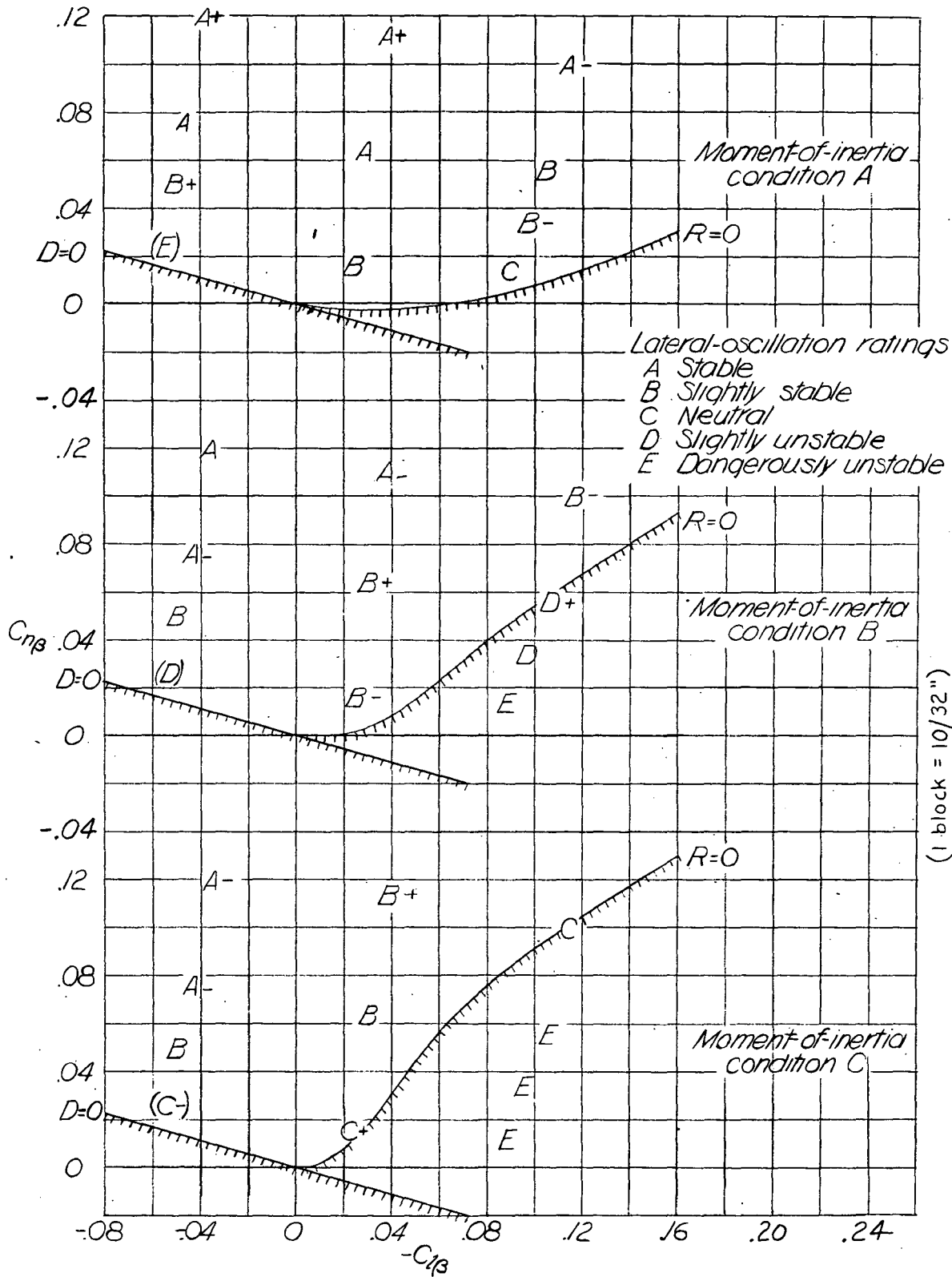
FIGURE 8.- Ratings for damping of lateral oscillation for different test conditions. C_L=1.0 . (Ratings possibly influenced by directional stability enclosed in parentheses)
