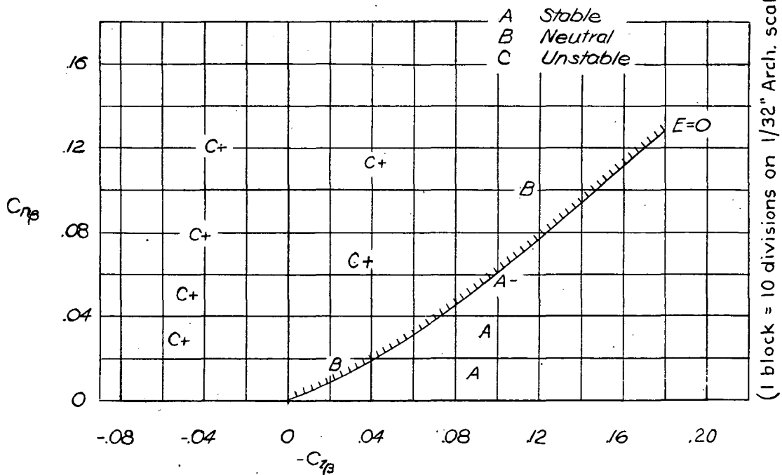
FIGURE 5.- Stability chart showing stability boundaries and model configurations. C_L=1.0 for all boundaries and configurations.
