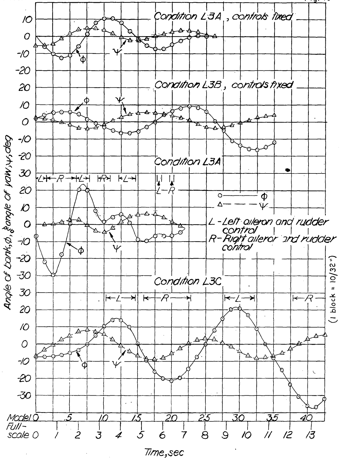
FIGURE 10.- Time histories of banking and yawing motions of model showing effect of increased moments of inertia on damping of lateral oscillation. Large positive dihedral. Vertical tail 3. C_L=1.0 .
