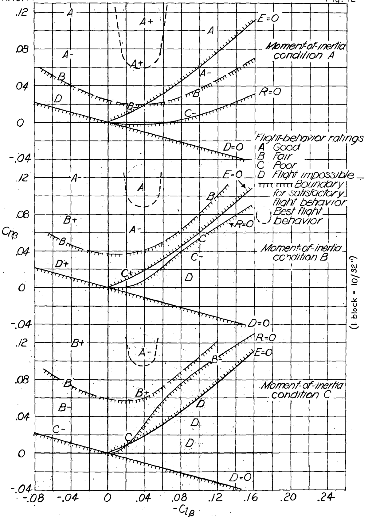
FIGURE 12.- Flight-behavior ratings for different test conditions. C_L=1.0 .
