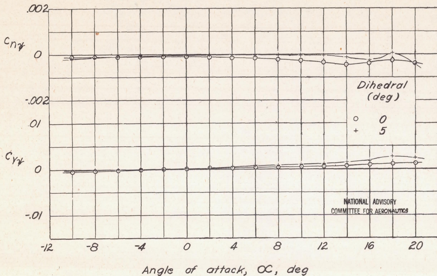
Figure 4.—Variation of lateral-stability slopes C_{ny} and C_{yx} with angle of attack for NACA 23012 rectangular wing. q , 65 lb/sq ft. ( C_{ny} measured about center of gravity.)
