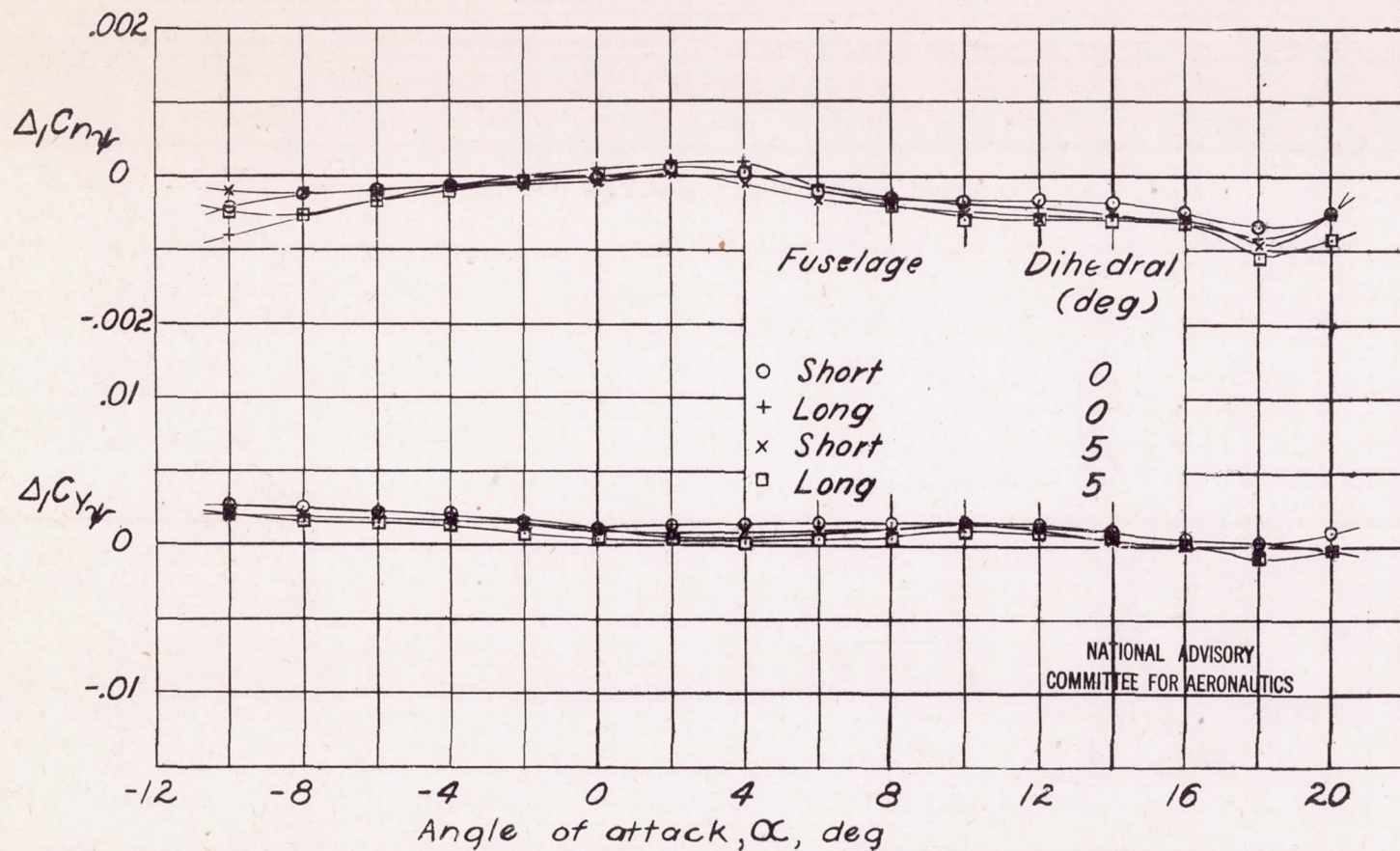
Figure 5.- Increments of C_{ny} and C_{yv} due to wing-fuselage interference. Horizontal and vertical tails off; q , 65 lb/sq ft.
