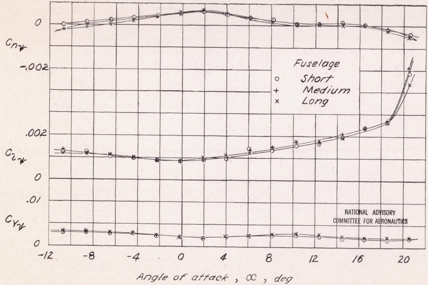
Figure 11.- Concluded. (b) Γ, 5°.
