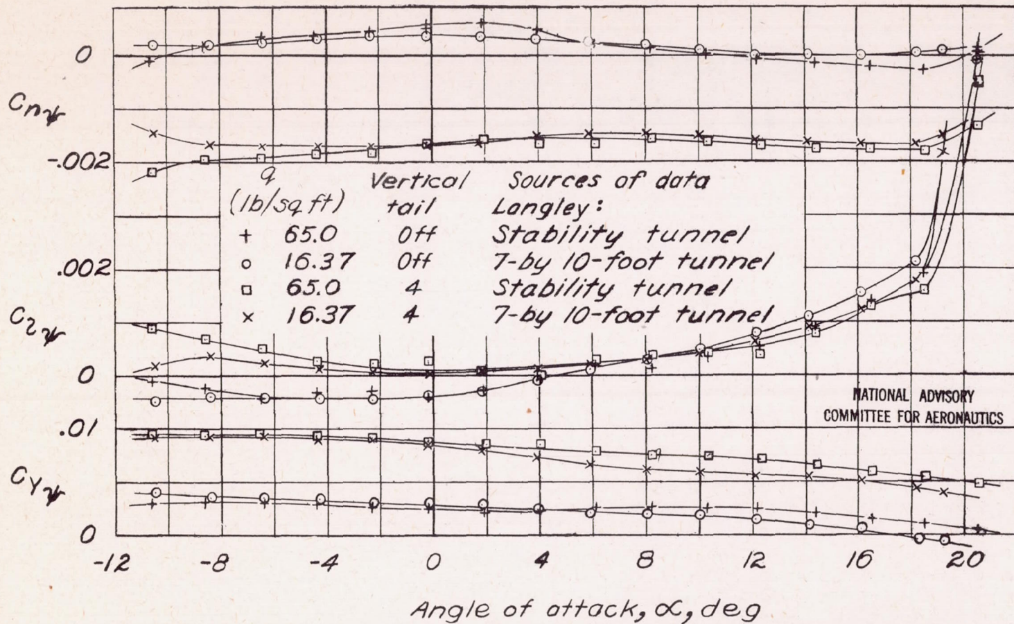
Figure 20.- Comparison of data from Langley stability and Langley 7-by 10-foot tunnels for variation of lateral-stability slopes C_{ny} , C_{\zeta\eta} , and C_{y\zeta} with angle of attack. Short fuselage in combination with rectangular wing; horizontal tail off; \Gamma , 0^\circ .
