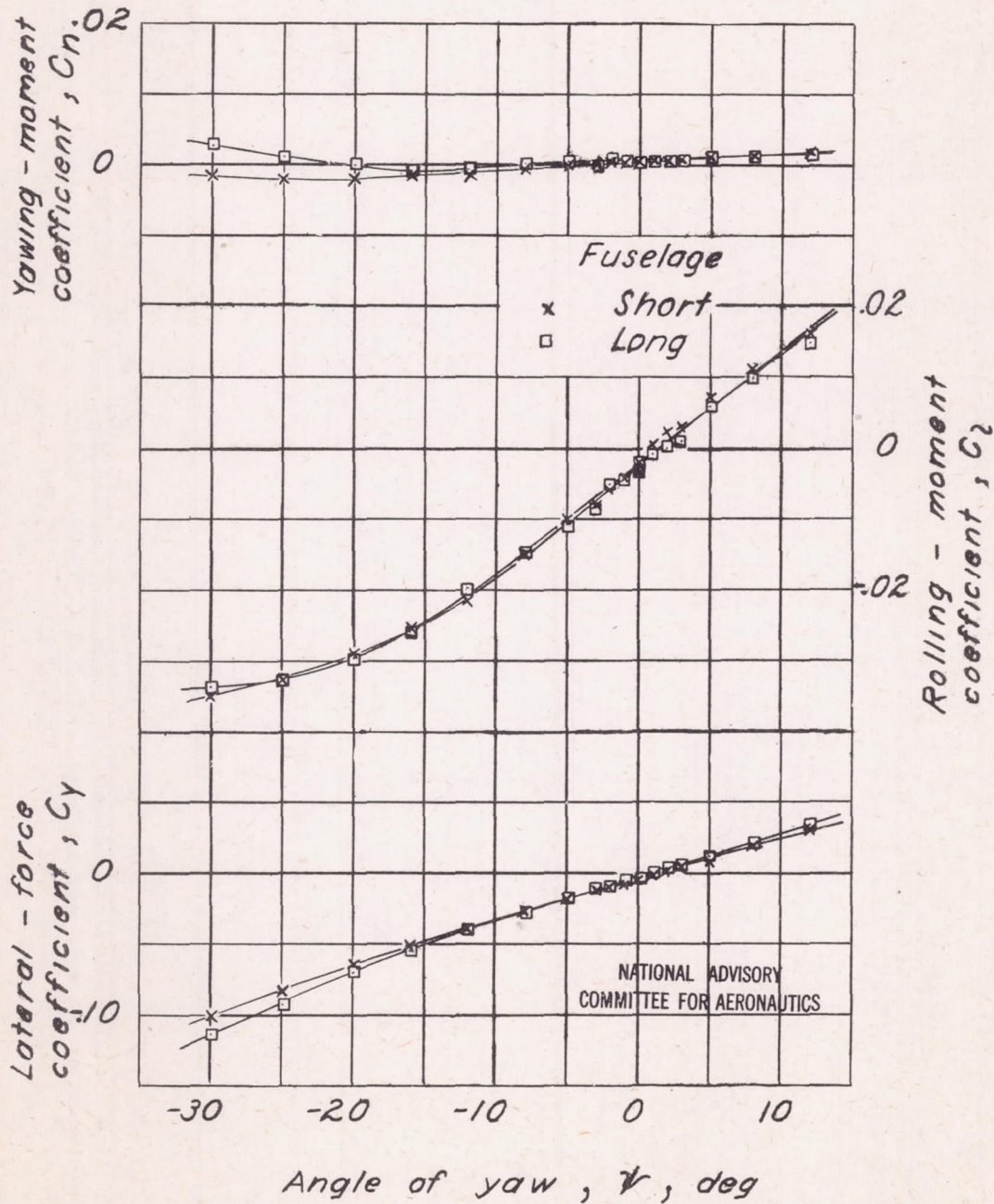
Figure 10. - Effect of changing fuselage length on variation of yawing - moment, rolling - moment, and lateral - force coefficients with angle of yaw. Horizontal and vertical tails off; \alpha , 10.2^\circ ; \Gamma , 5^\circ ; q , 65 lb/sq ft.
