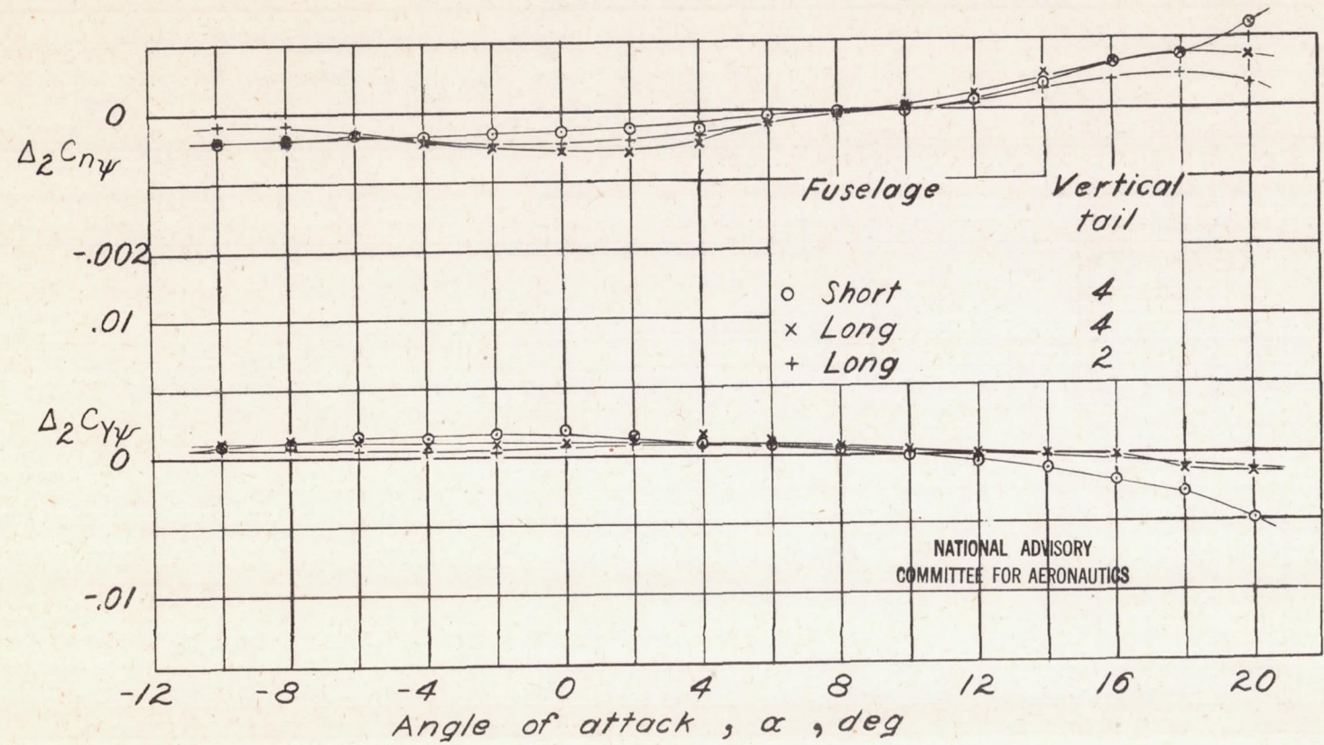
(a) \Gamma, 0^\circ . Figure 6.- Increments of C_{ny} and C_{yv} due to wing-fuselage interference on vertical tail. Horizontal tail on; q, 65 \text{ lb/sq ft} .
