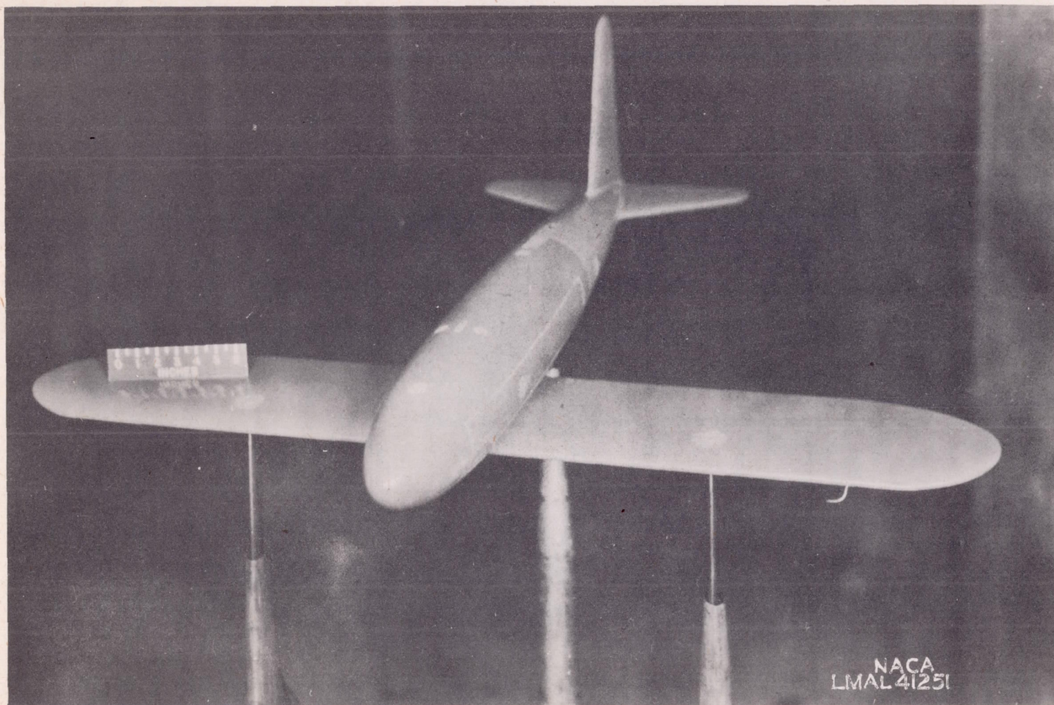
Figure 2.- Rectangular-low-wing model equipped with short fuselage and vertical tail 5 mounted for tests in Langley stability tunnel.
