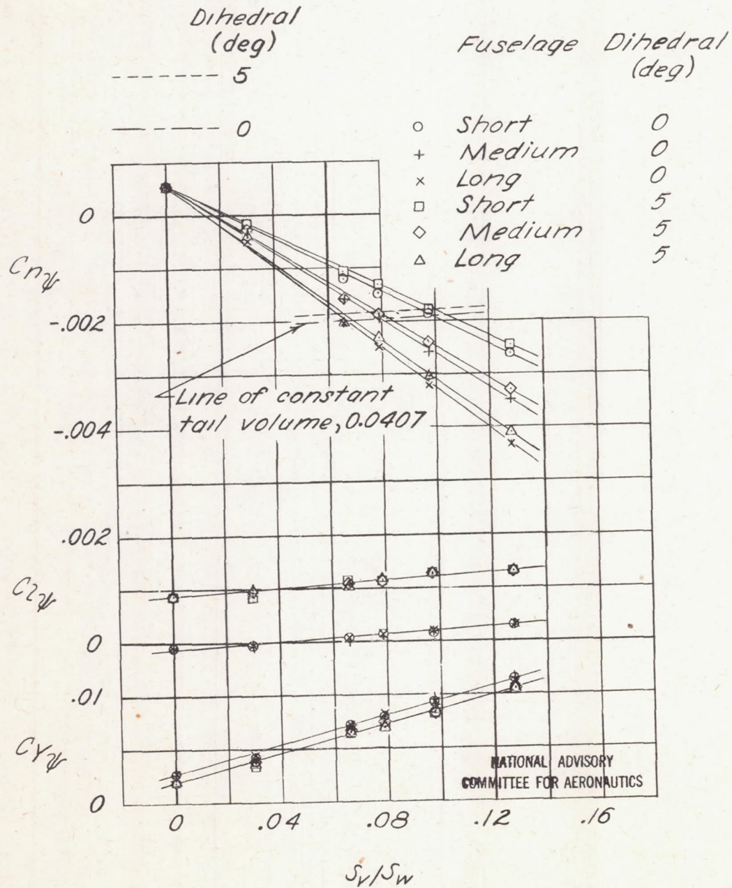
Figure 14.-Effect of changing fuselage length on variation of lateral-stability slopes C_{n\dot{y}} , C_{\dot{z}y} , and C_{y\dot{y}} with vertical-tail area. Horizontal tail on ; q, 65 \text{ lb/sq ft} .
