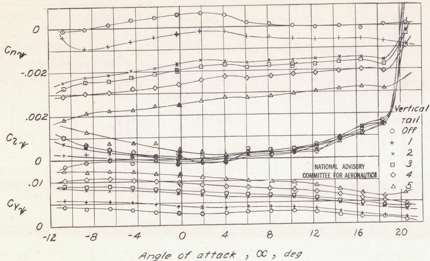
Figure 15.—Effect of changing vertical-tail area on variation of lateral-stability slopes C_{n\dot{w}} , C_{z\dot{w}} , and C_{y\dot{w}} with angle of attack. Medium-length fuselage with horizontal tail; q, 65 \text{ lb/sq ft} .
