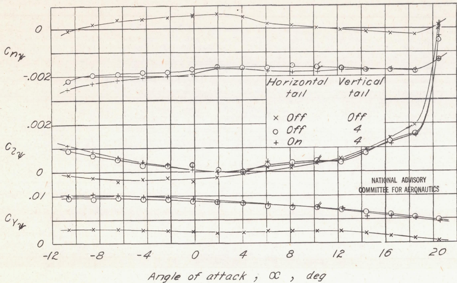
(a) \Gamma, 0^\circ . Figure 7.- Effect of horizontal tail surface on variation of lateral-stability slopes C_{ny} , C_{zeta} , and C_{ye} with angle of attack. Short fuselage; q, 65 \text{ lb/sq ft} .
