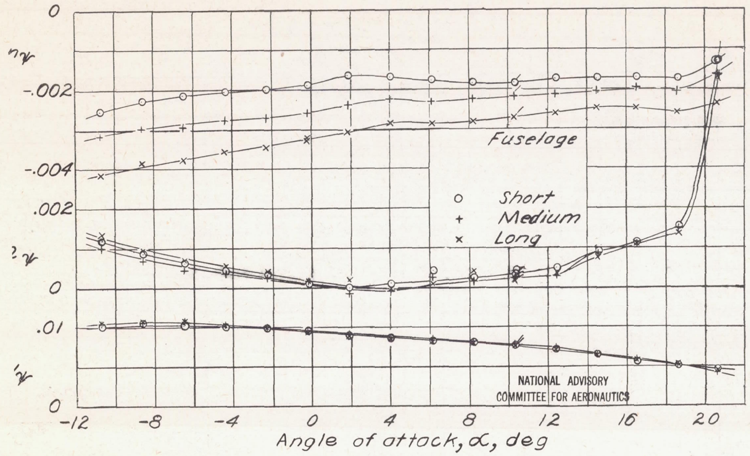
Figure 12.- Effect of changing fuselage length on variation of lateral-stability slopes C_{n\dot{\psi}} , C_{l\dot{\psi}} , and C_{y\dot{\psi}} with angle of attack. Horizontal tail and vertical tail 4 on ; q, 65 \text{ lb/sq ft} .
