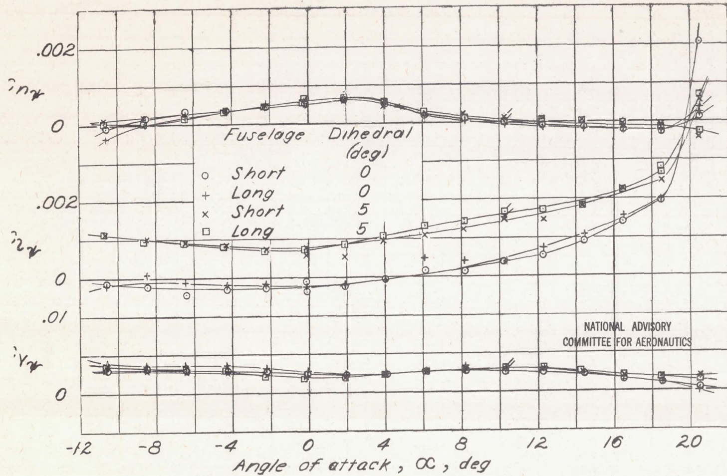
Figure 9.- Effect of changing fuselage length on variation of lateral-stability slopes C_{ny} , C_{zw} , and C_{yw} with angle of attack. Horizontal and vertical tails off; q , 65 lb/sq ft.
