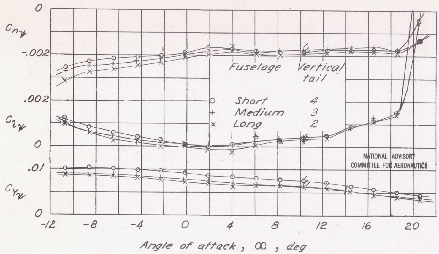
Figure 18.- Effect of several combinations having constant tail volume on variation of lateral-stability slopes C_{ny} , C_{zw} , and C_{yw} with angle of attack. Tail volume, 0.0407; horizontal tail on; q , 65 lb/sq ft.
