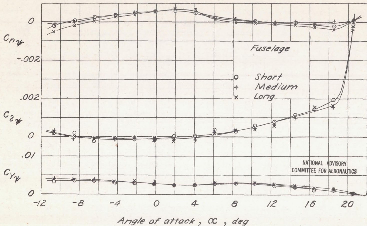
Figure 11.—Effect of changing fuselage length on variation of lateral-stability slopes C_{n\beta} , C_{2\beta} , and C_{Y\beta} with angle of attack. Horizontal tail on; vertical tail off; q, 65 \text{ lb/sq ft} .
