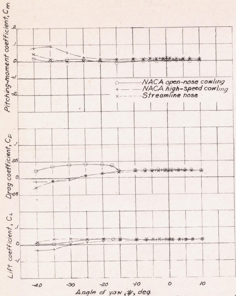
Figure 9.- Variation of lift, drag, and pitching-moment coefficients with angle of yaw. Fuselage alone; K , maximum; \alpha , 0.
