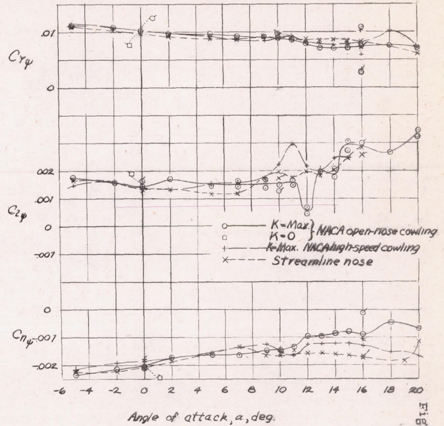
Figure 14.- Variation of C_{x\psi} , C_{z\psi} , and C_{n\psi} with angle of attack. Complete model.
