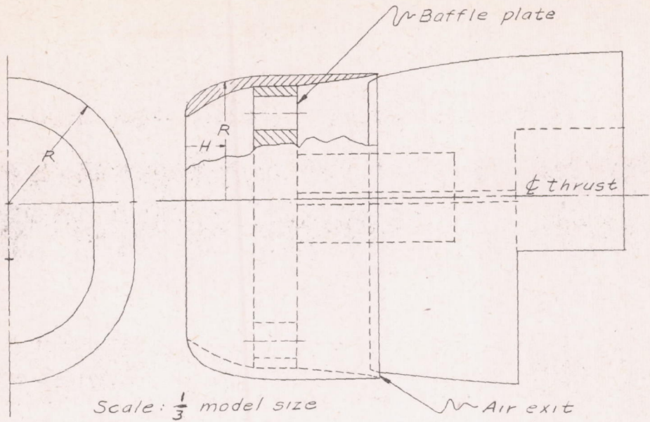
Figure 3.- Test arrangement for NACA open-nose cowling.
