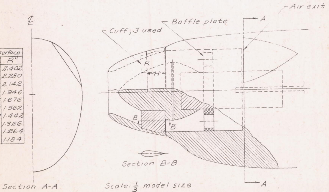
Figure 4.- Test arrangement of NACA high-speed cowling.
