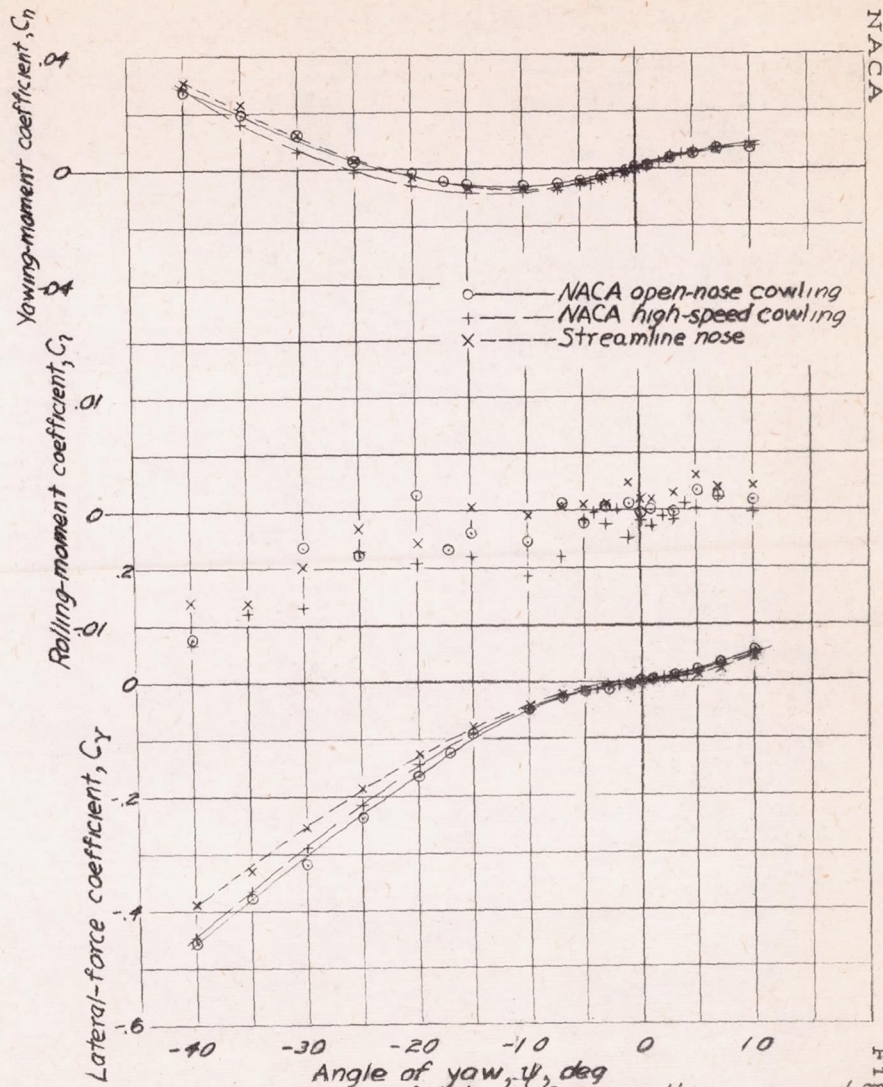
Figure 10.- Variation of lateral-force, rolling-moment, and yawing-moment coefficients with angle of yaw. Fuselage alone; K , maximum; \alpha , 0.
