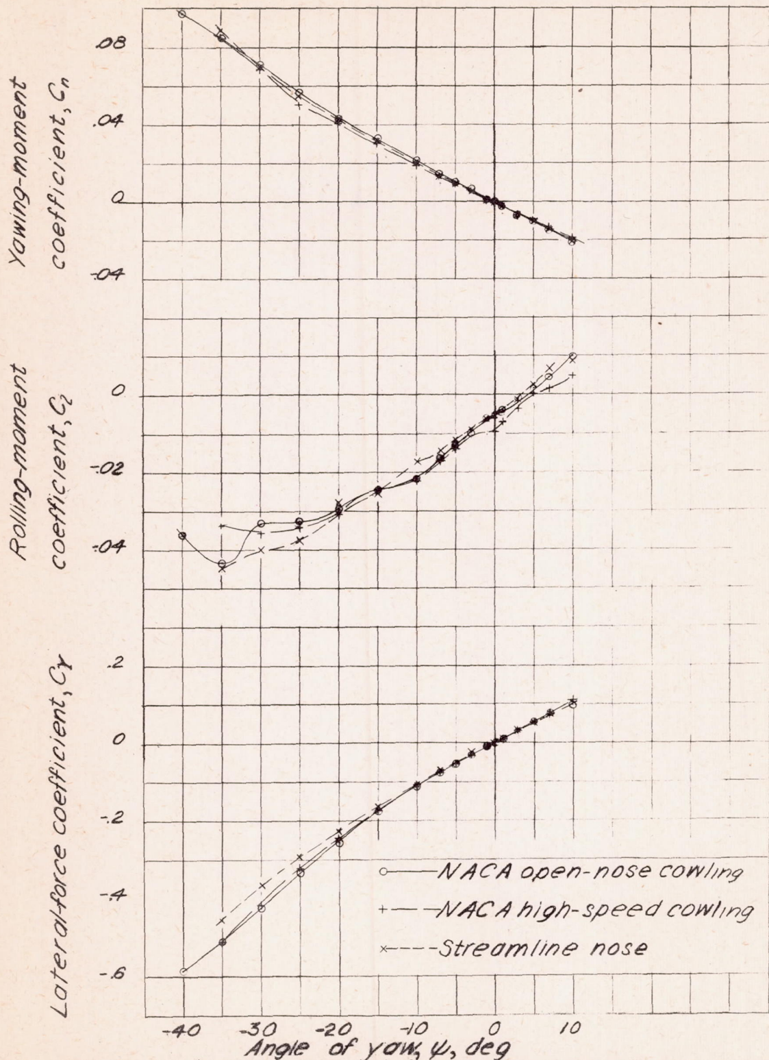
Figure 11.- Variation of lateral-force, rolling-moment, and yawing-moment coefficients with angle of yaw. Complete model; K , maximum; \alpha , 0.
