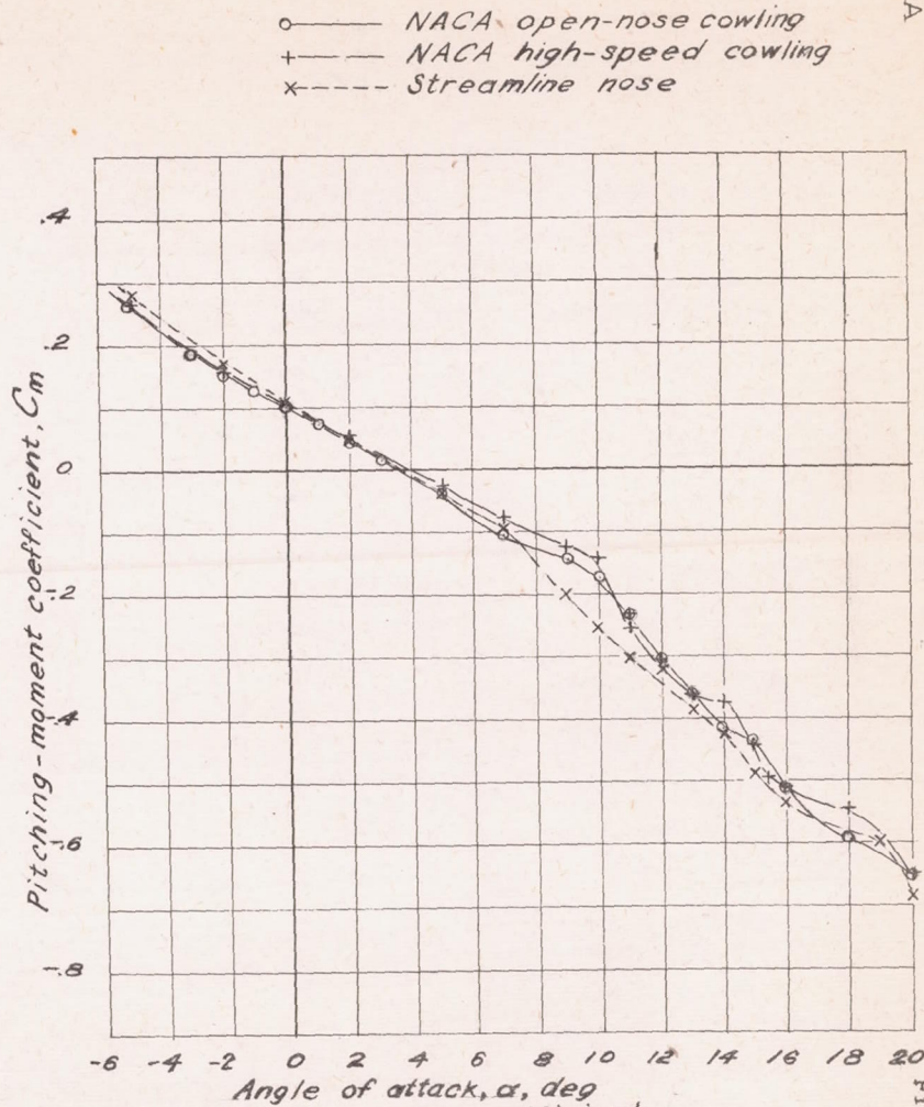
(b) Pitching-moment coefficient Figure 7.-Concluded.
