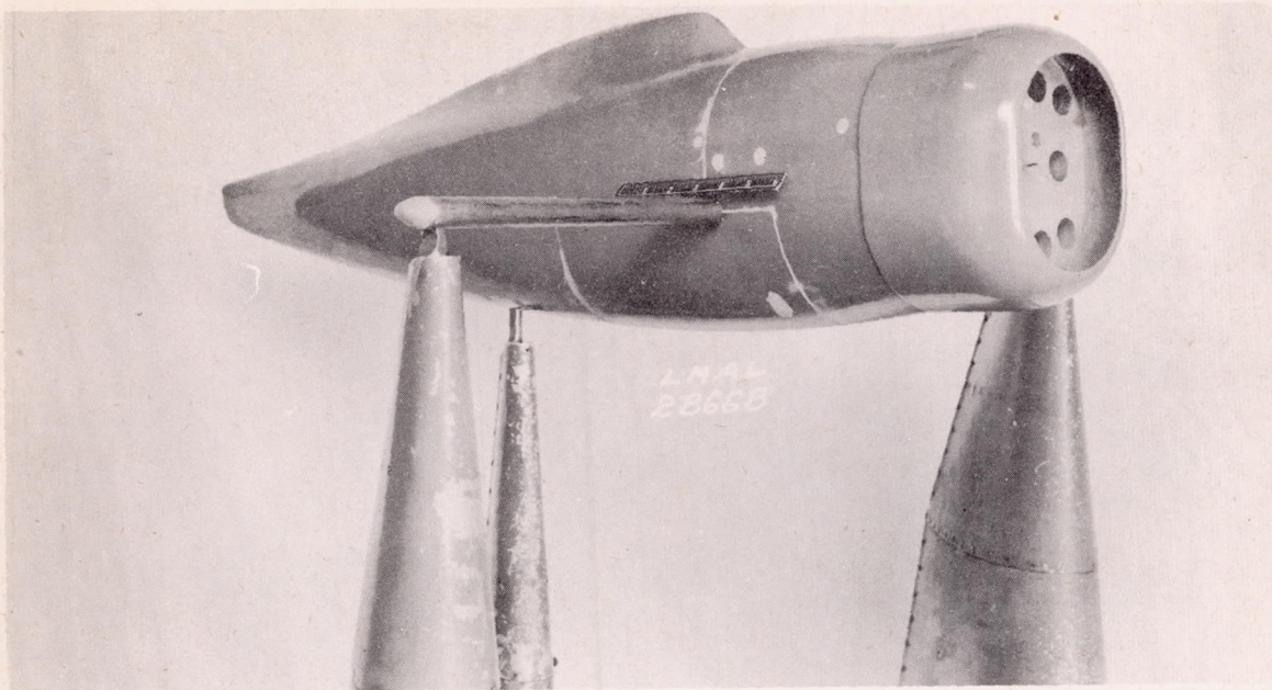
(B) FUSELAGE WITH NACA OPEN-NOSE COWLING.
