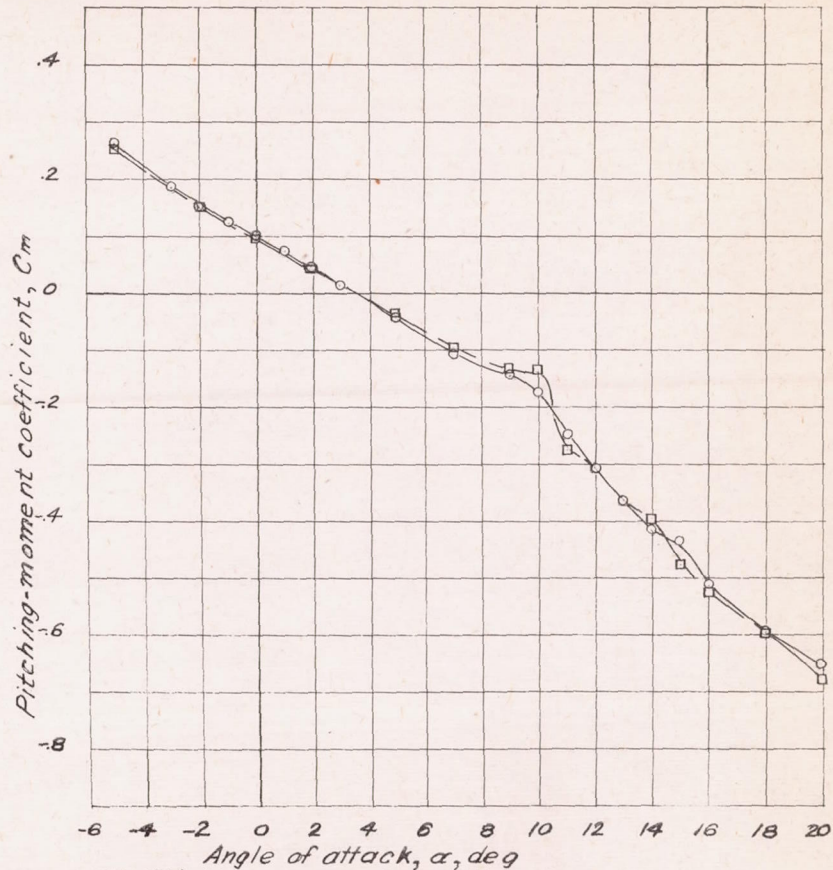
(b) Pitching-moment coefficient. Figure 8.- Concluded.
