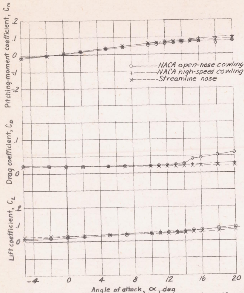
Figure 6.-Variation of lift, drag, and pitching-moment coefficients with angle of attack. Fuselage alone; k , maximum; \gamma , 0.
