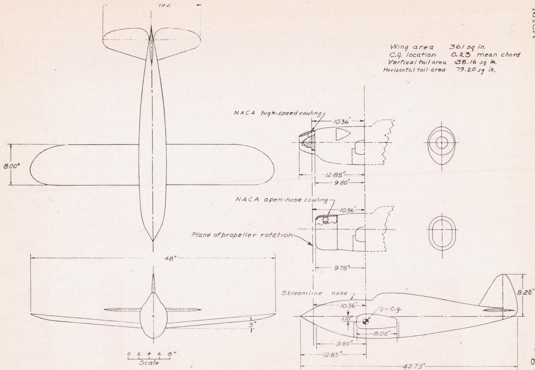
Figure 2.- Three-view drawing of the 0.1-scale pursuit airplane model with three nose sections.
