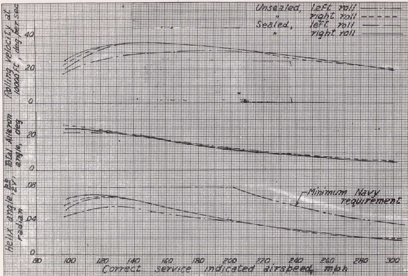
Figure 43.- Variation of helix angle, \frac{pb}{2V} , total aileron angle, and rolling velocity at 10,000 feet altitude obtainable with 30 pounds stick force as a function of speed. Flaps up, landing gear up, power for level flight, Curtiss SB2C-1 airplane.
