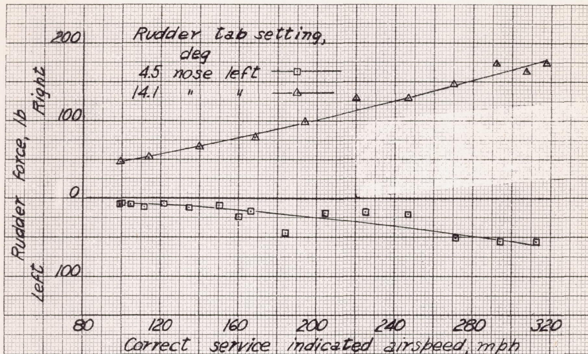
Figure 54.- Variation of rudder force with speed with two rudder trim tab settings; flaps up, landing gear up, front hood closed, rear hood open, power off. Curtiss SB2C-1 airplane.
