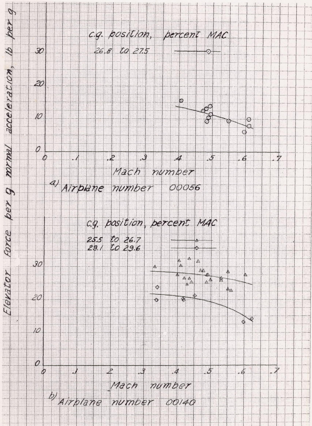
Figure 27.- Variation of elevator force per g normal acceleration with Mach number in pull-outs from dives. Curtiss SB2C-1 airplanes number 00056 and 00140, flaps up, landing gear up, front hood open, rear hood closed, power off.
