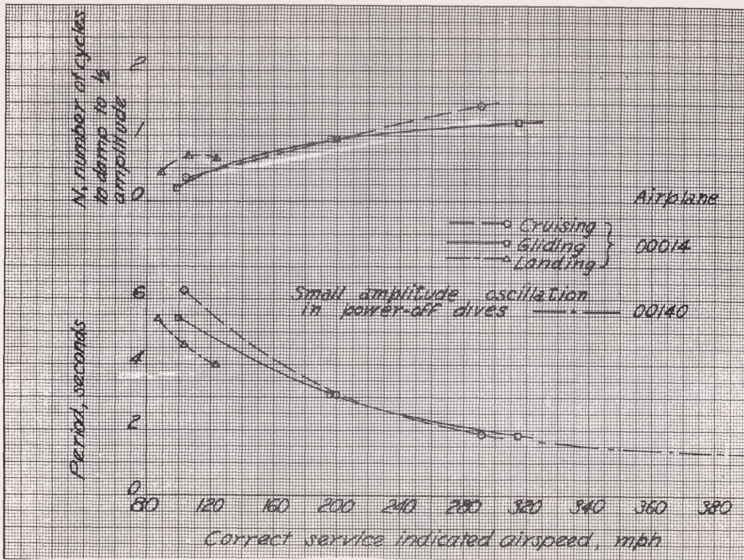
Figure 36.- Period and damping of lateral oscillations. Curtiss SB2C-1 airplane.
