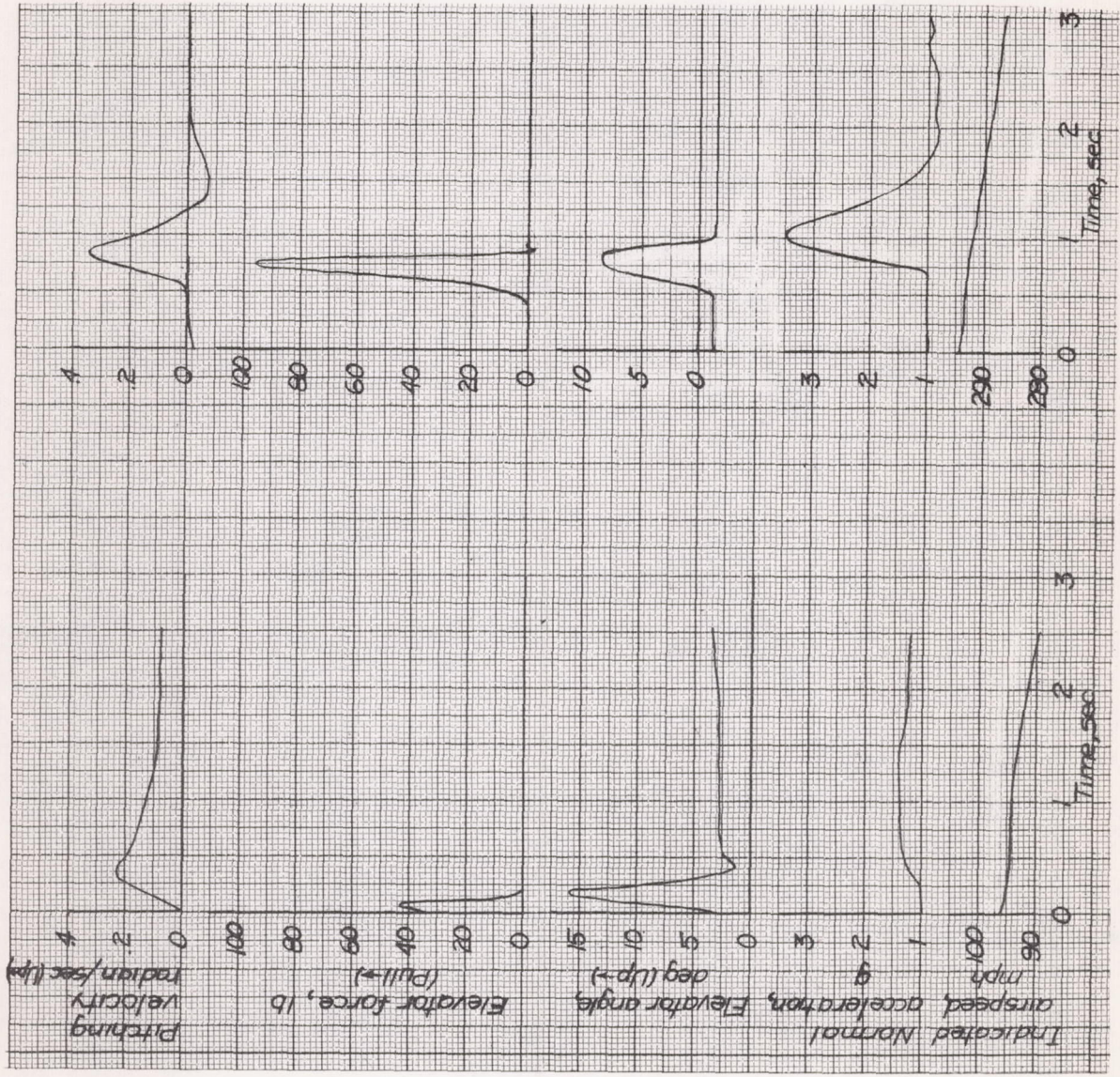
Figure 11.- Time histories of typical attempted longitudinal oscillations. SE2C-1 airplane (flaps up, landing gear up, rated power).
