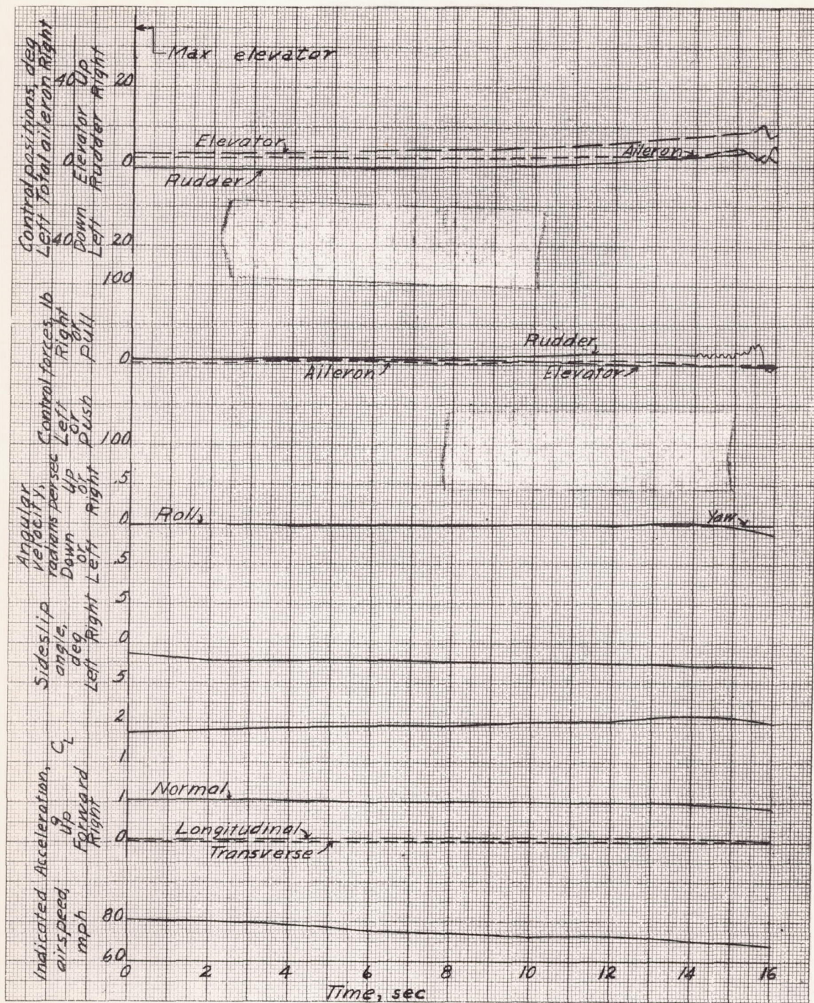
Figure 61.- Time history of a stall in the landing condition (flaps down, landing gear down, hoods closed, cowl flaps closed, power off) center of gravity at 26.8 percent of the mean aerodynamic chord. Curtiss SB2C-1 airplane.
