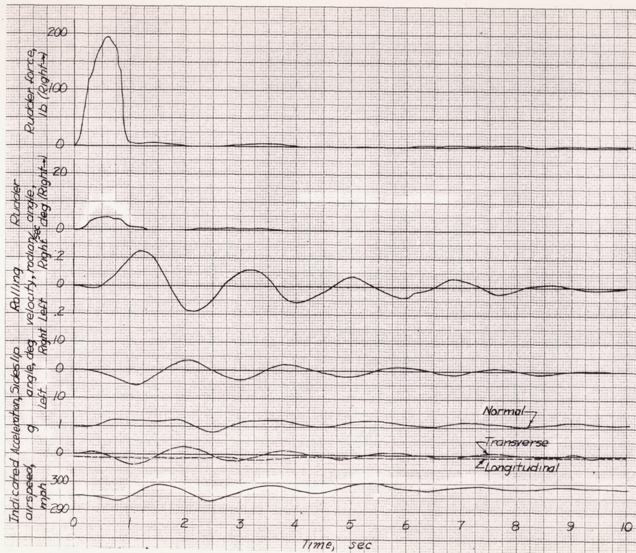
Figure 35.- Time history of a typical lateral oscillation at approximately 295 mph. Curtiss SB2C-1 airplane, flaps up, landing gear up, rated power.
