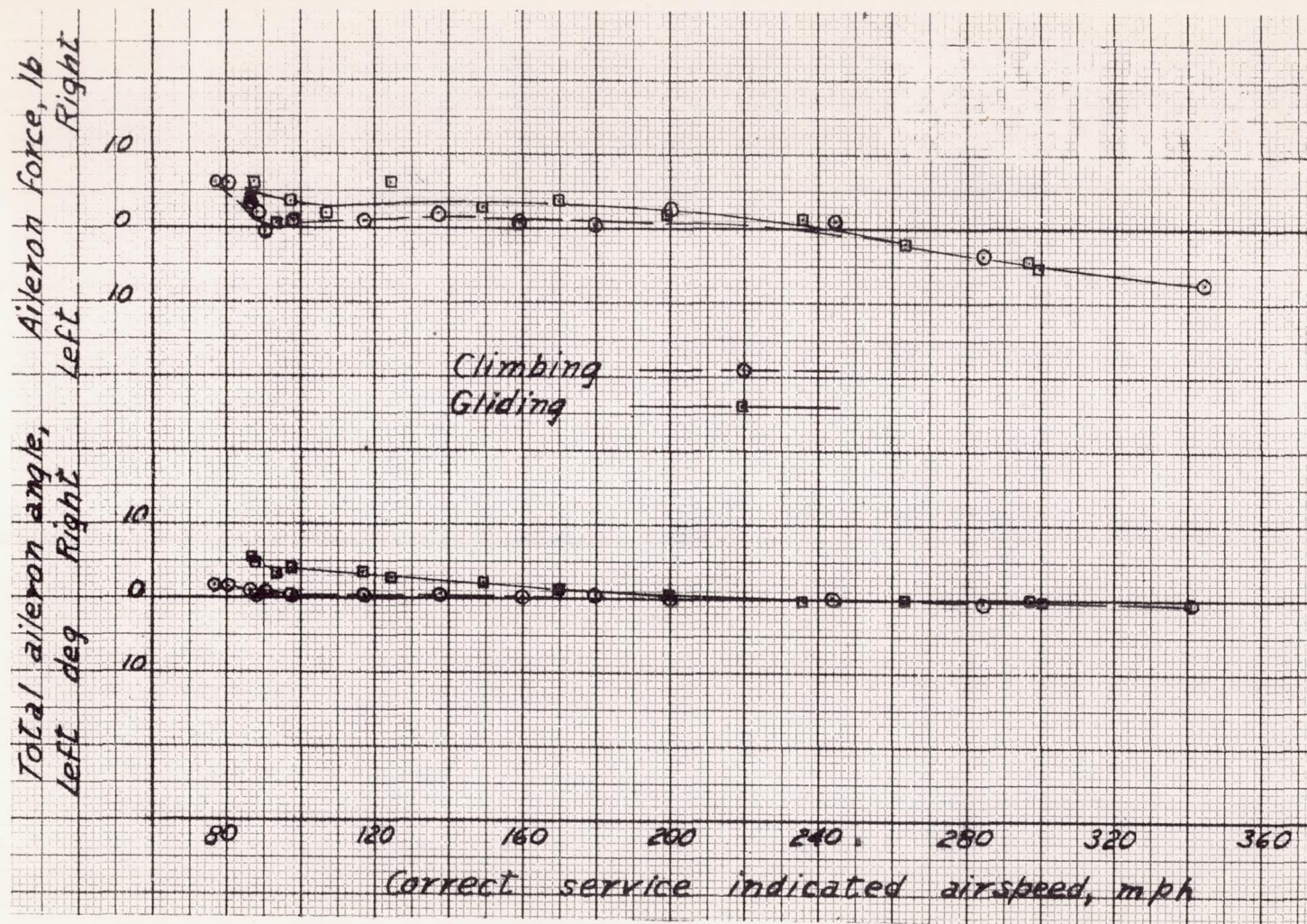
Figure 57.- Variation with speed of aileron angle and aileron force required for trim; aileron gap unsealed, Curtiss SB2C-1 airplane.
