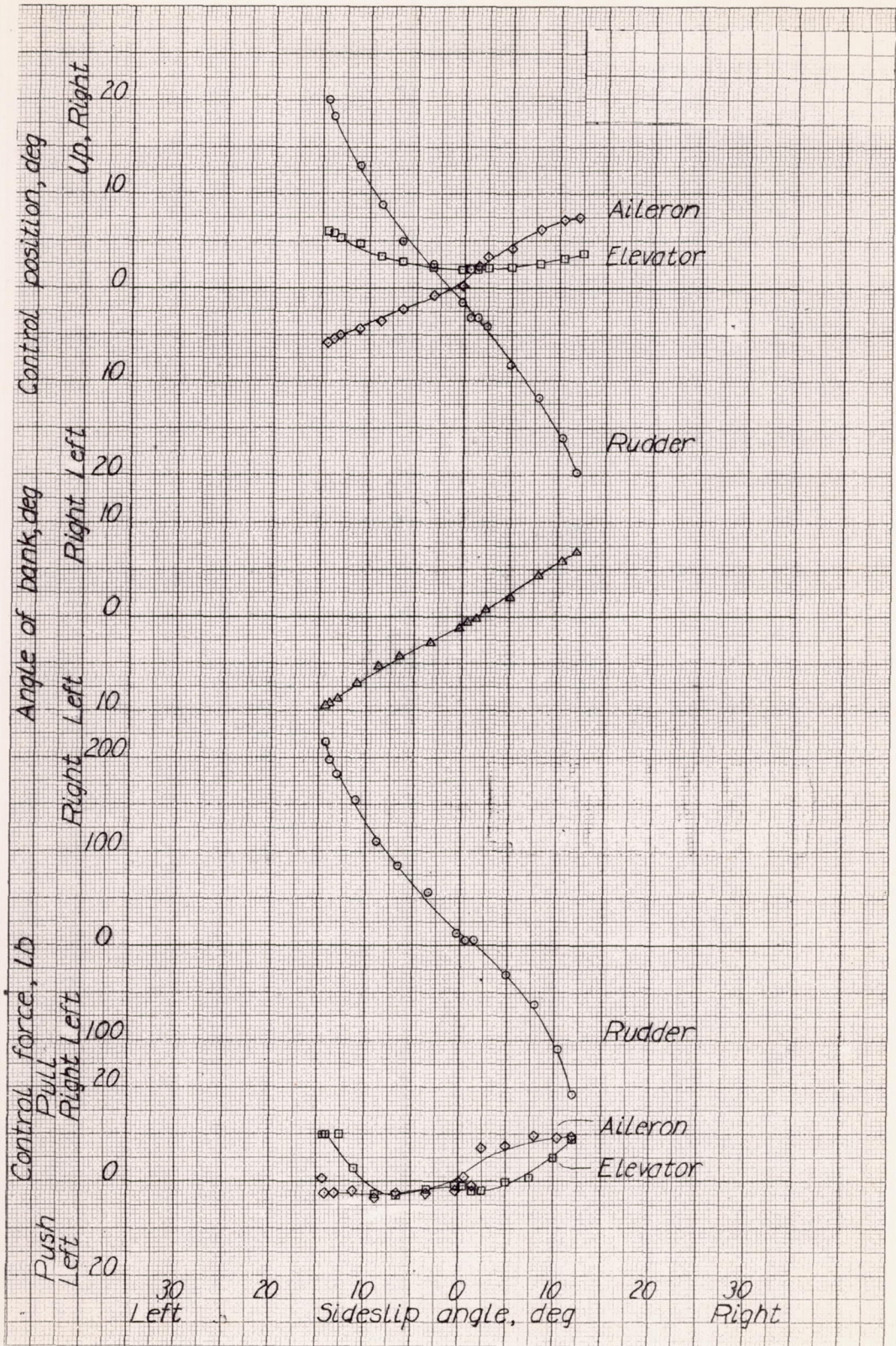
Figure 47.- Steady sideslip characteristics in the landing condition (flaps down, landing gear down, power off) at 120 miles per hour. Curtiss SB2C-1 airplane.
