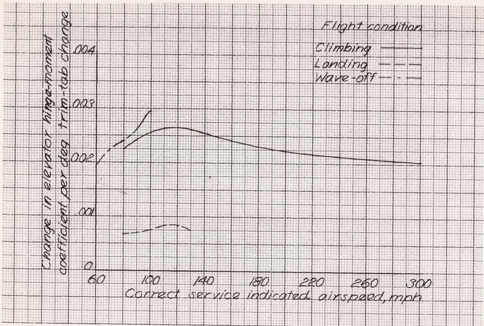
Figure 33.- Variation of change in elevator hinge moment coefficient per degree trim-tab deflection with indicated airspeed. Curtiss SB2C-1 airplane.
