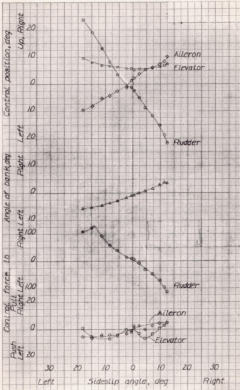
Figure 46.- Steady sideslip characteristics in the landing condition (flaps down, landing gear down, power off) at 95 miles per hour. Curtiss SB2C-1 airplane.
