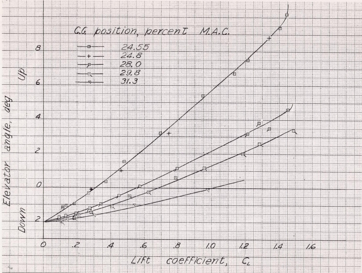
Figure 16.- Variation of elevator angle measured from thrust axis with lift coefficient in the gliding condition (flaps up, landing gear up, power off) Curtiss SB2C-1 airplane
