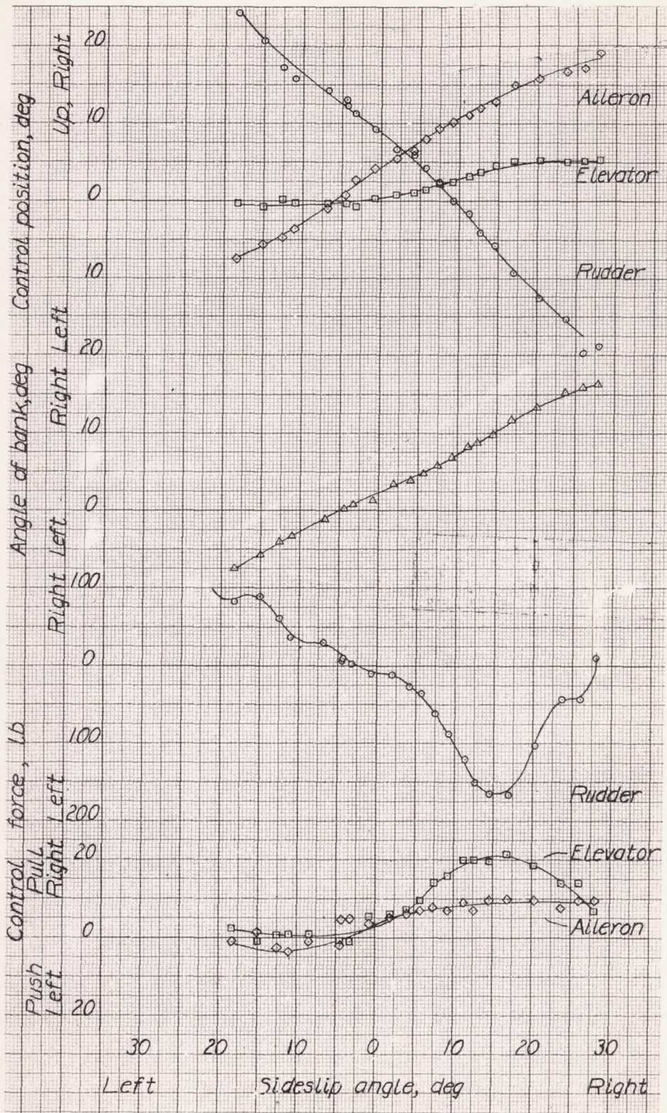
Figure 48.- Steady sideslip characteristics in the climbing condition (flaps up, landing gear up, 38 inches of Hg at 2400 rpm) at 95 miles per hour. Curtiss SB2C-1 airplane.
