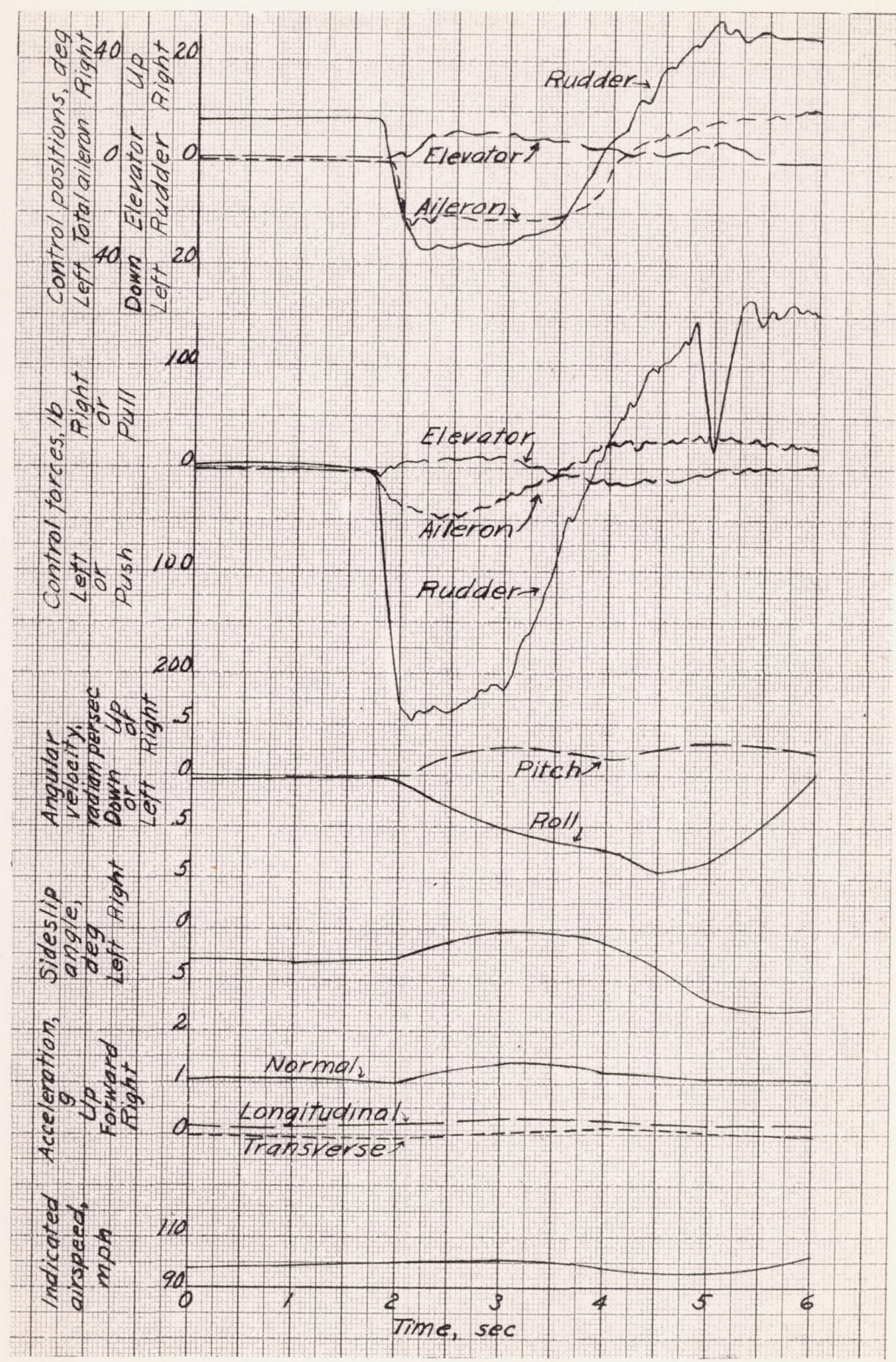
Figure 51.- Time history of a roll into a turn in which the rudder was used in an attempt to maintain zero sideslip. Curtiss SB2C-1 airplane, flaps up, landing gear up, power for level flight.
