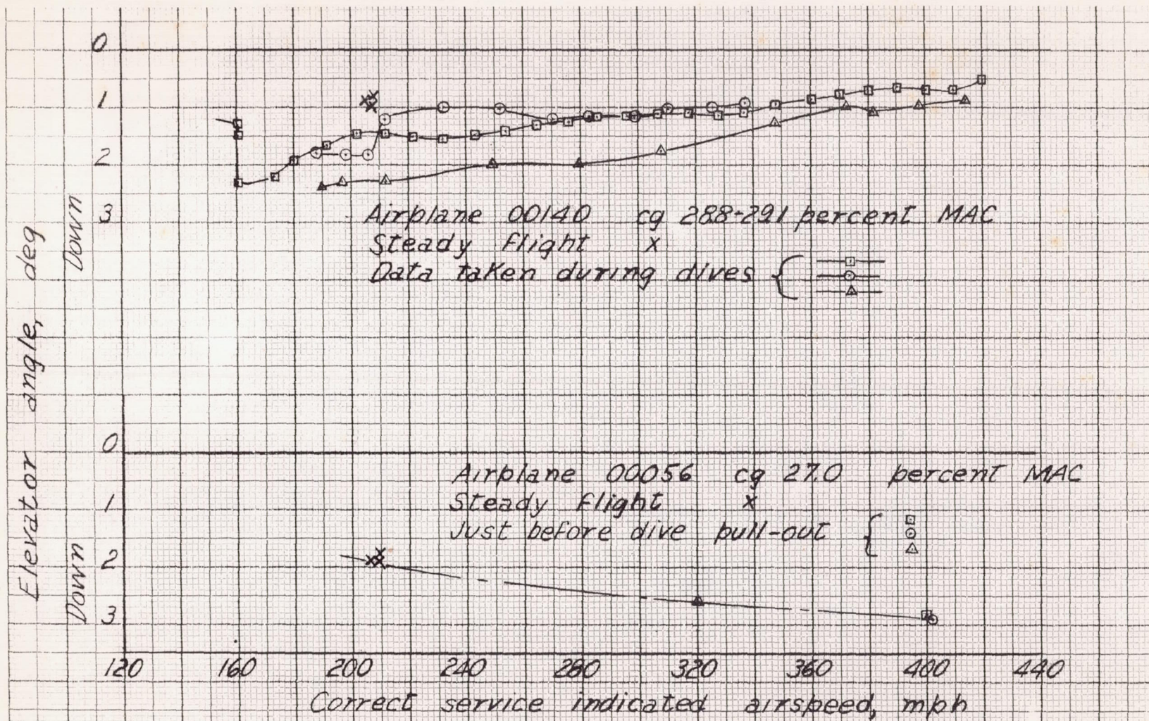
Figure 20.- Variation of elevator angle with speed in dives. Curtiss SB2C-1 airplane, flaps up, landing gear up, front hood open, rear hood closed, power off.
