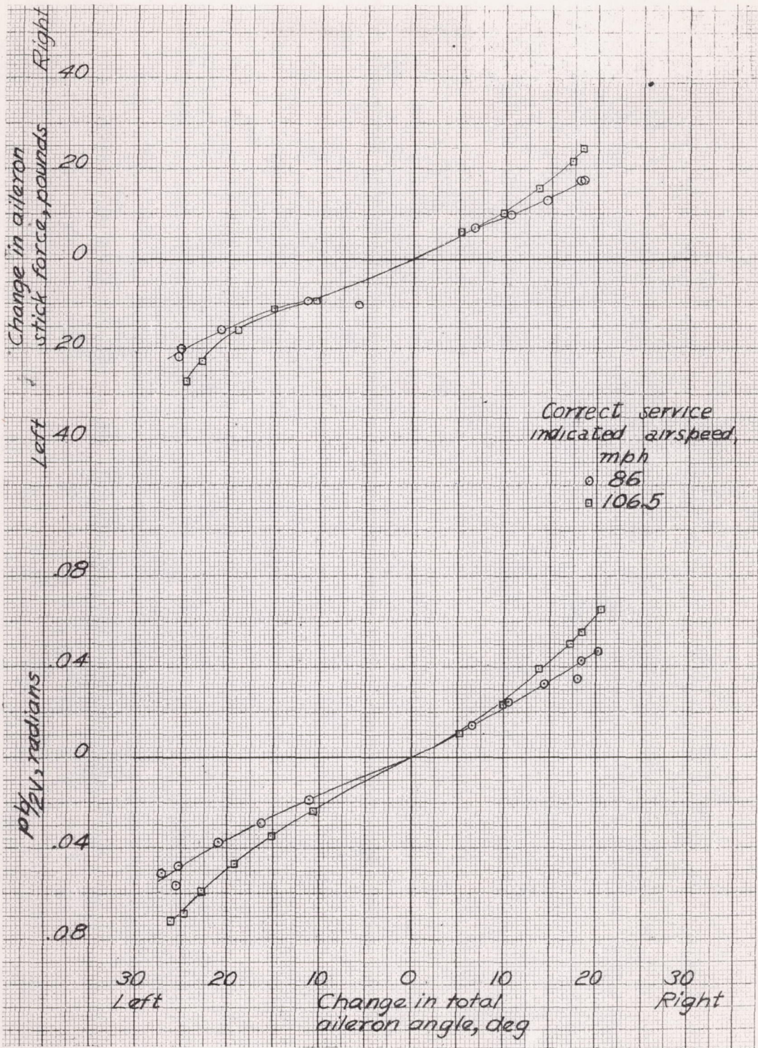
Figure 41.- Variation of aileron stick force and helix angle, pb/2V , with change in total aileron angle in rolls made at two speeds; flaps down, landing gear down, leading-edge slots open, power off, aileron gap unsealed, Curtiss SB2C-1 airplane.
