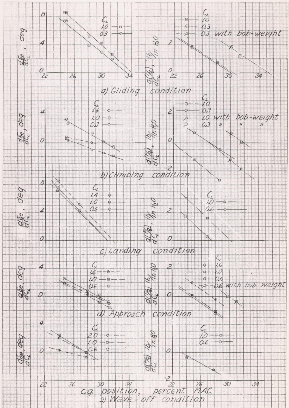
Figure 18.- Plots showing stick-fixed and stick-free neutral points for the various airplane conditions tested. Curtiss SB2C-1 airplane.
