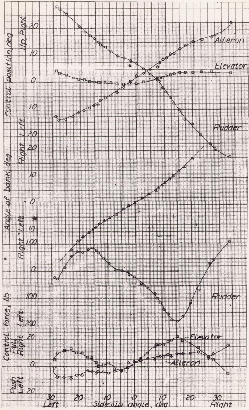
Figure 49.- Steady sideslip characteristics in the climbing condition (flaps up, landing gear up, 38 inches of Hg at 2400 rpm) at 120 miles per hour. Curtiss SB2C-1 airplane.
