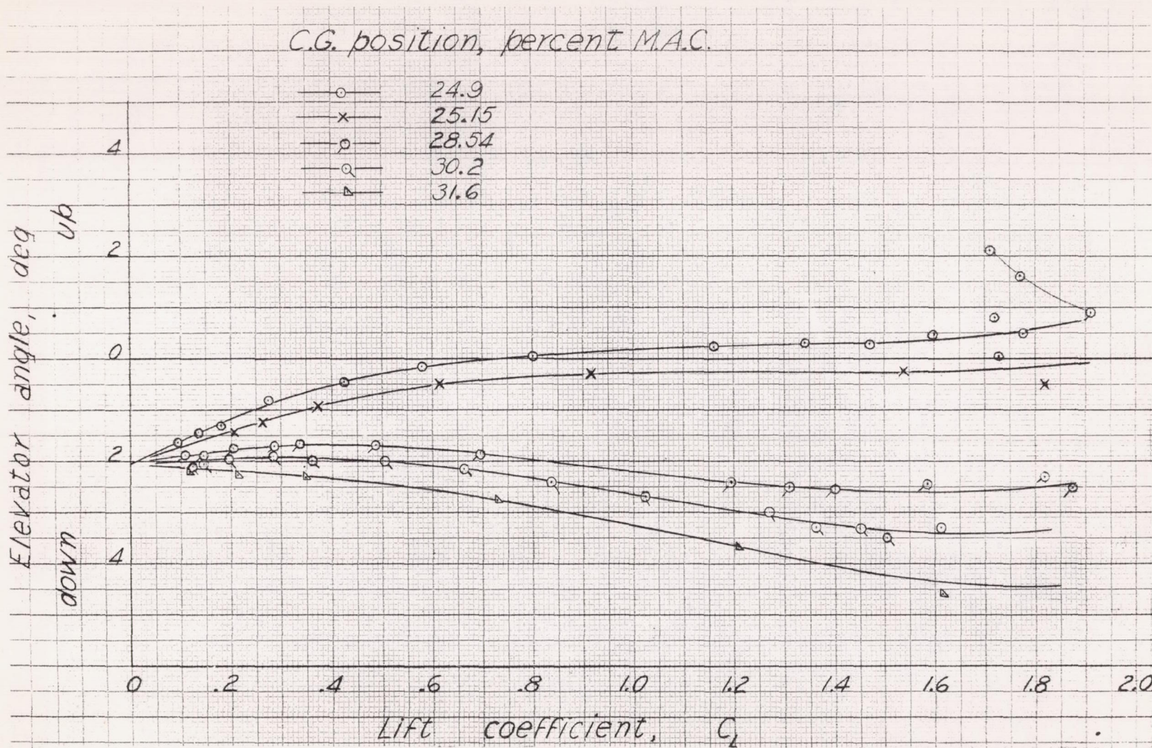
Figure 17.- Variation of elevator angle measured from thrust axis with lift coefficient in the climbing condition (flaps up, landing gear up, rated power) Curtiss SB2C-1 airplane.
