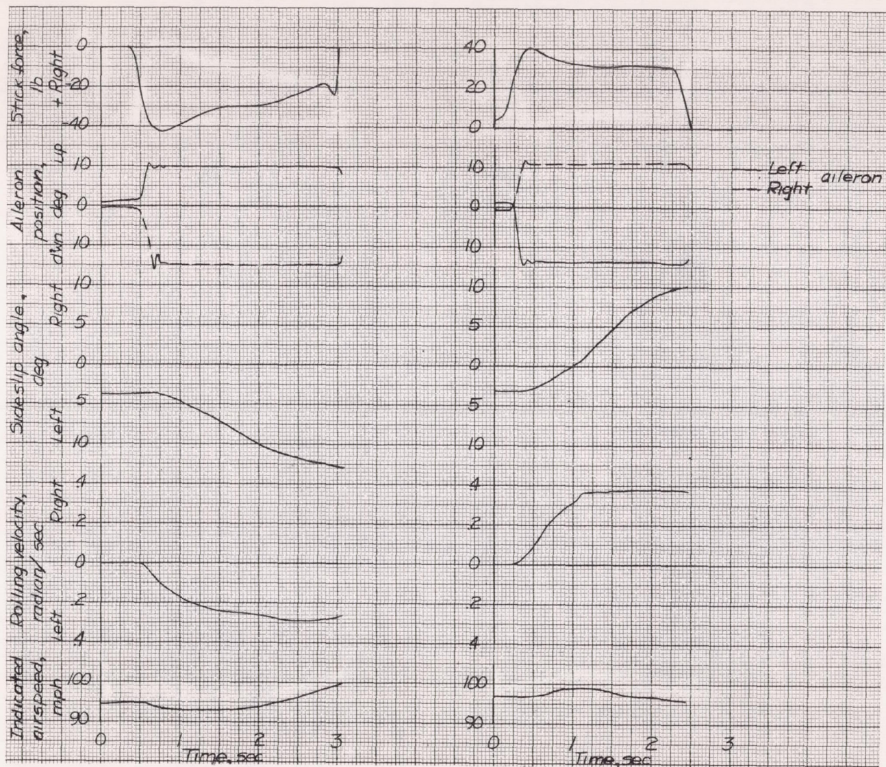
Figure 38.- Time histories of typical abrupt aileron rolls (rudder fixed) Curtiss SB2C-1 airplane, flaps up, landing gear up, power for level flight.
