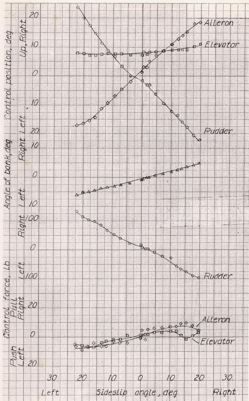
Figure 44.- Steady sideslip characteristics in the gliding condition (flaps up, landing gear up, power off) at 95 miles per hour. Curtiss SB2C-1 airplane.
