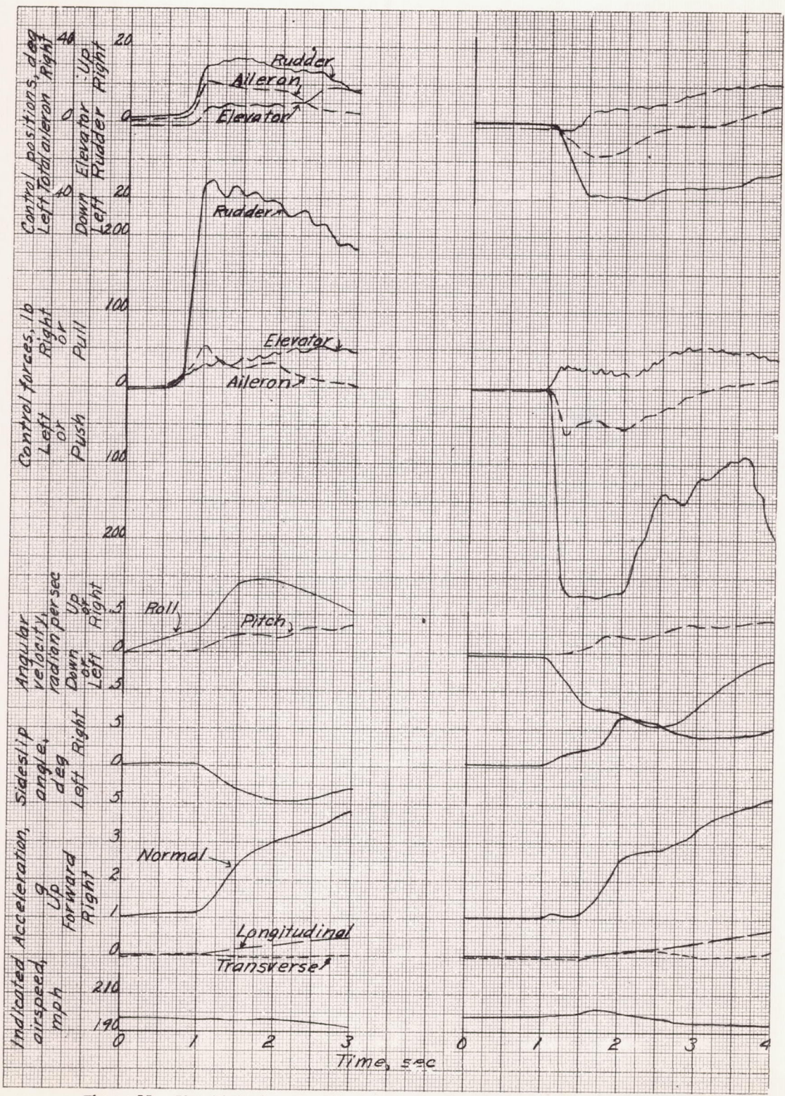
Figure 53.- Time histories of rolls into left and right turns in which the rudder was used in an attempt to maintain zero sideslip. Note that too much rudder deflection was used. Curtiss SB2C-1 airplane, flaps up, landing gear up, power for level flight.
