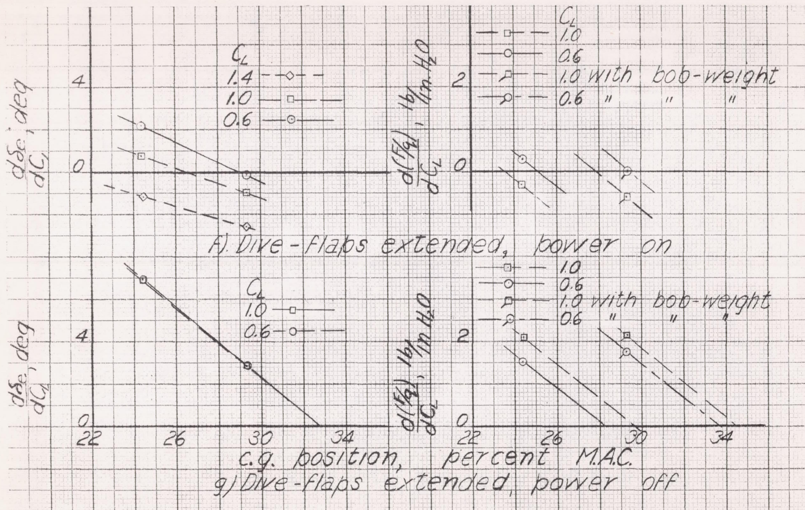
Figure 18.- (concluded) Plots showing stick-fixed and stick-free neutral points for the various airplane conditions tested. Curtiss SB2C-1 airplane.
