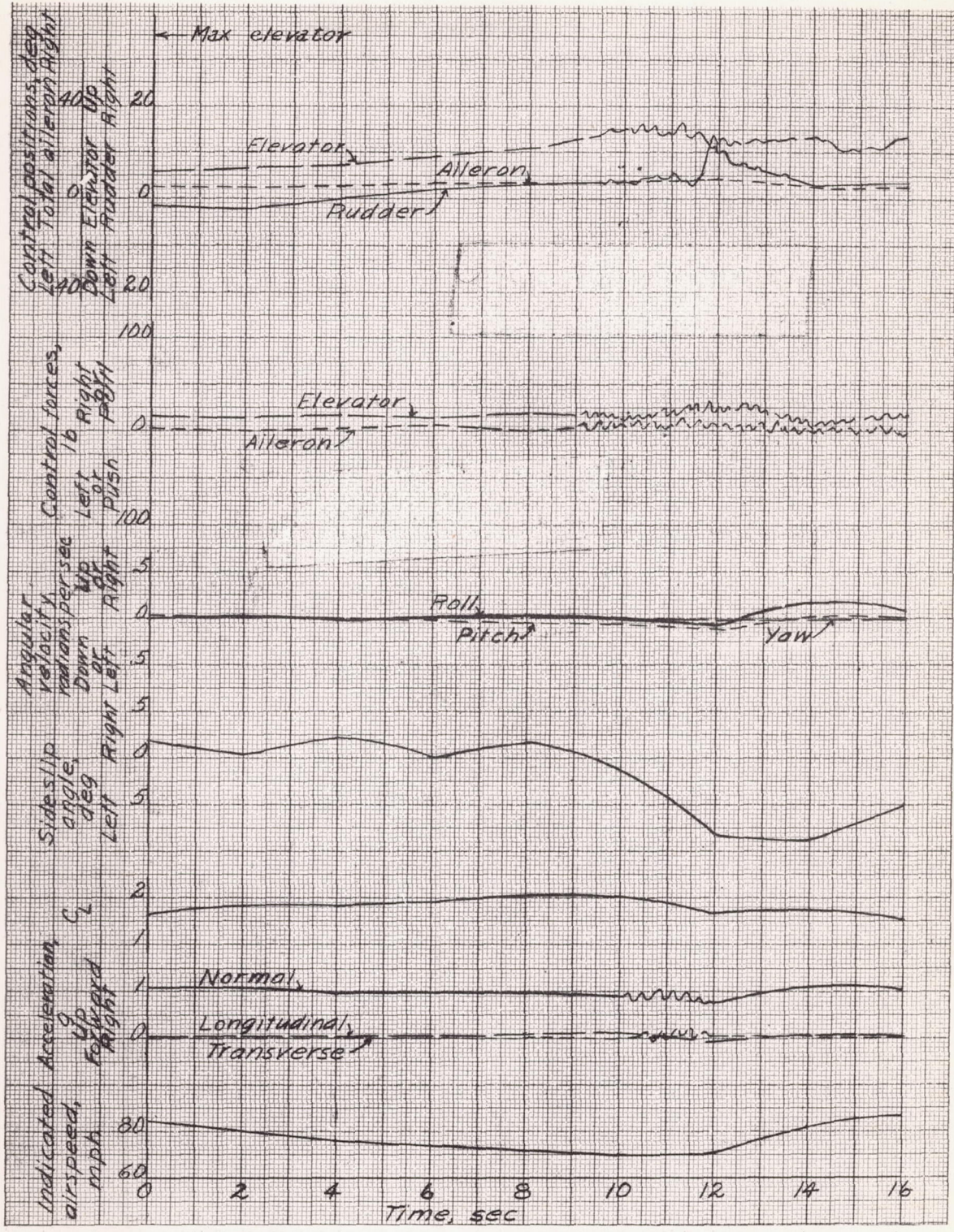
Figure 62.- Time history of a stall in the landing condition (flaps down, landing gear down, front hood closed (?), rear hood closed, cowl flaps open, power off) center of gravity at 24.8 percent of the mean aerodynamic chord. Curtiss SB2C-1 airplane.
