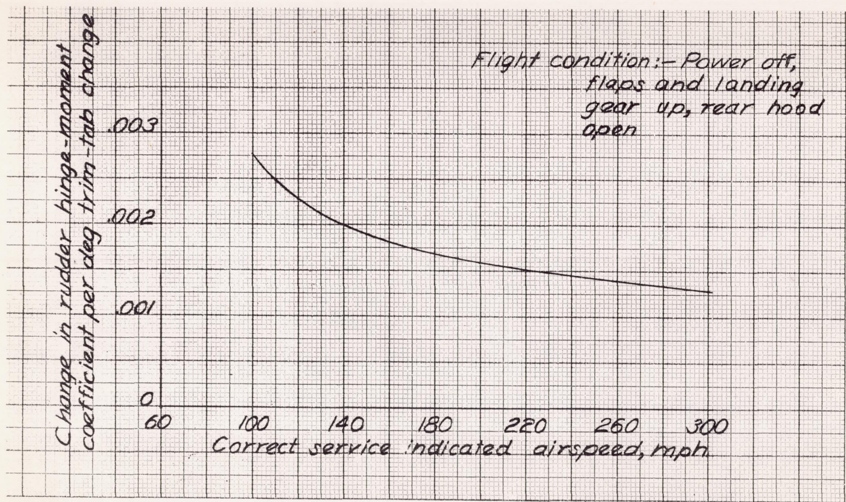
Figure 56.- Variation of changes in rudder hinge-moment coefficient per degree trim-tab deflection with indicated airspeed. Curtiss SB2C-1 airplane.
