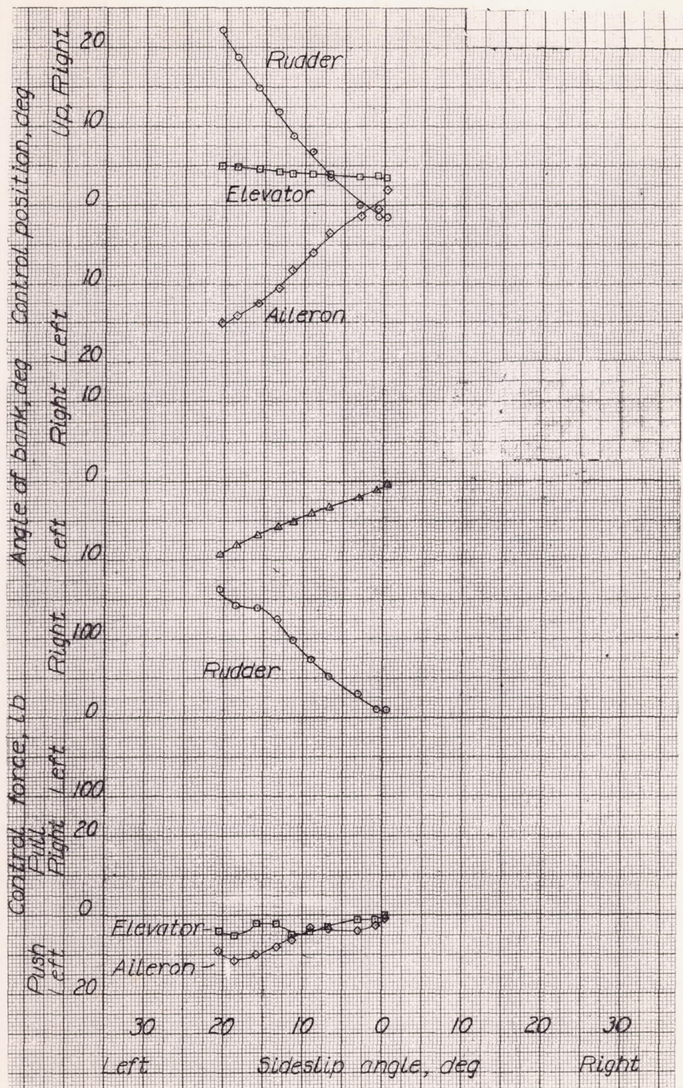
Figure 45.- Steady sideslip characteristics in the gliding condition (flaps up, landing gear up, power off) at 120 miles per hour. Curtiss SB2C-1 airplane.
