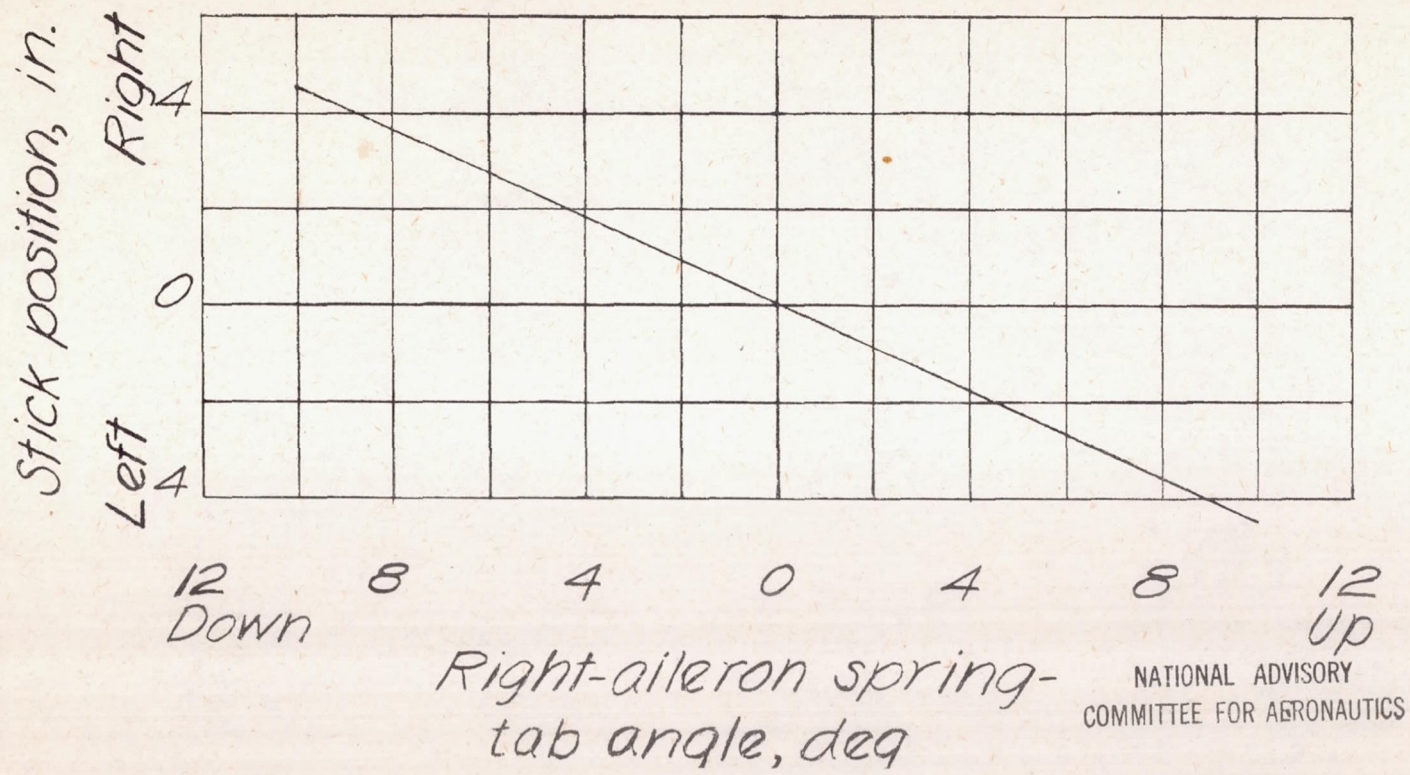
Figure 4.- Variation of stick position with right-aileron spring-tab angle. F6F-3 airplane; ailerons held neutral.
