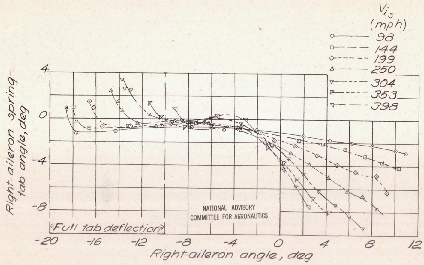
Figure 9.- Variation of right-aileron spring-tab angle with right-aileron angle in abrupt aileron rolls. F6F-3 airplane.
