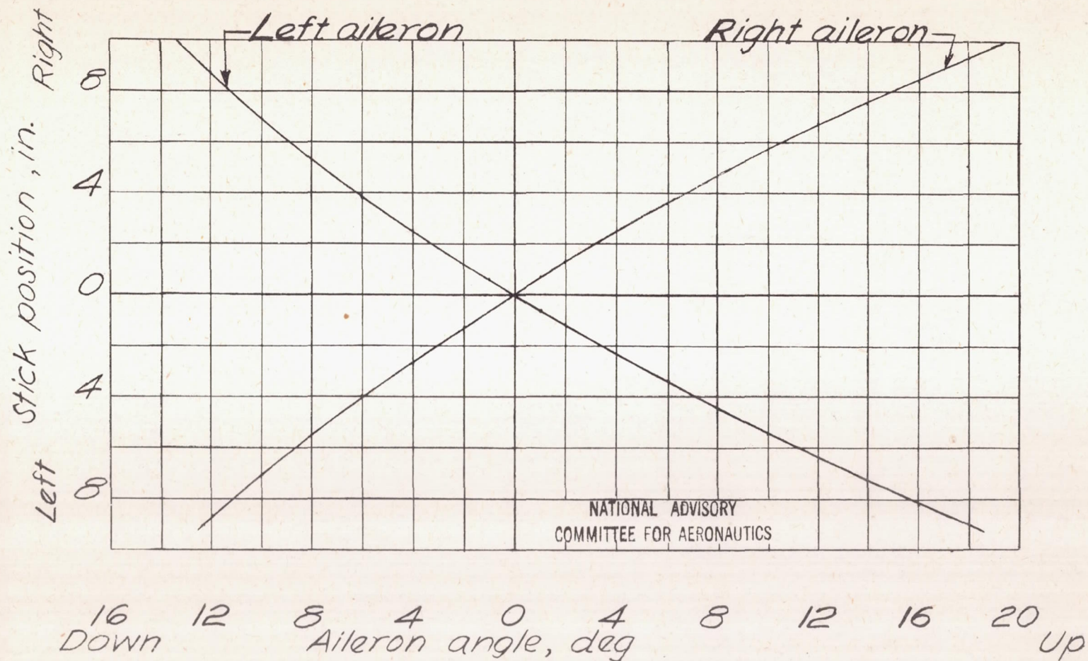
Figure 5.- Variation of stick position with left- and right-aileron angles. F6F-3 airplane with spring-tab ailerons; no load on control system.
