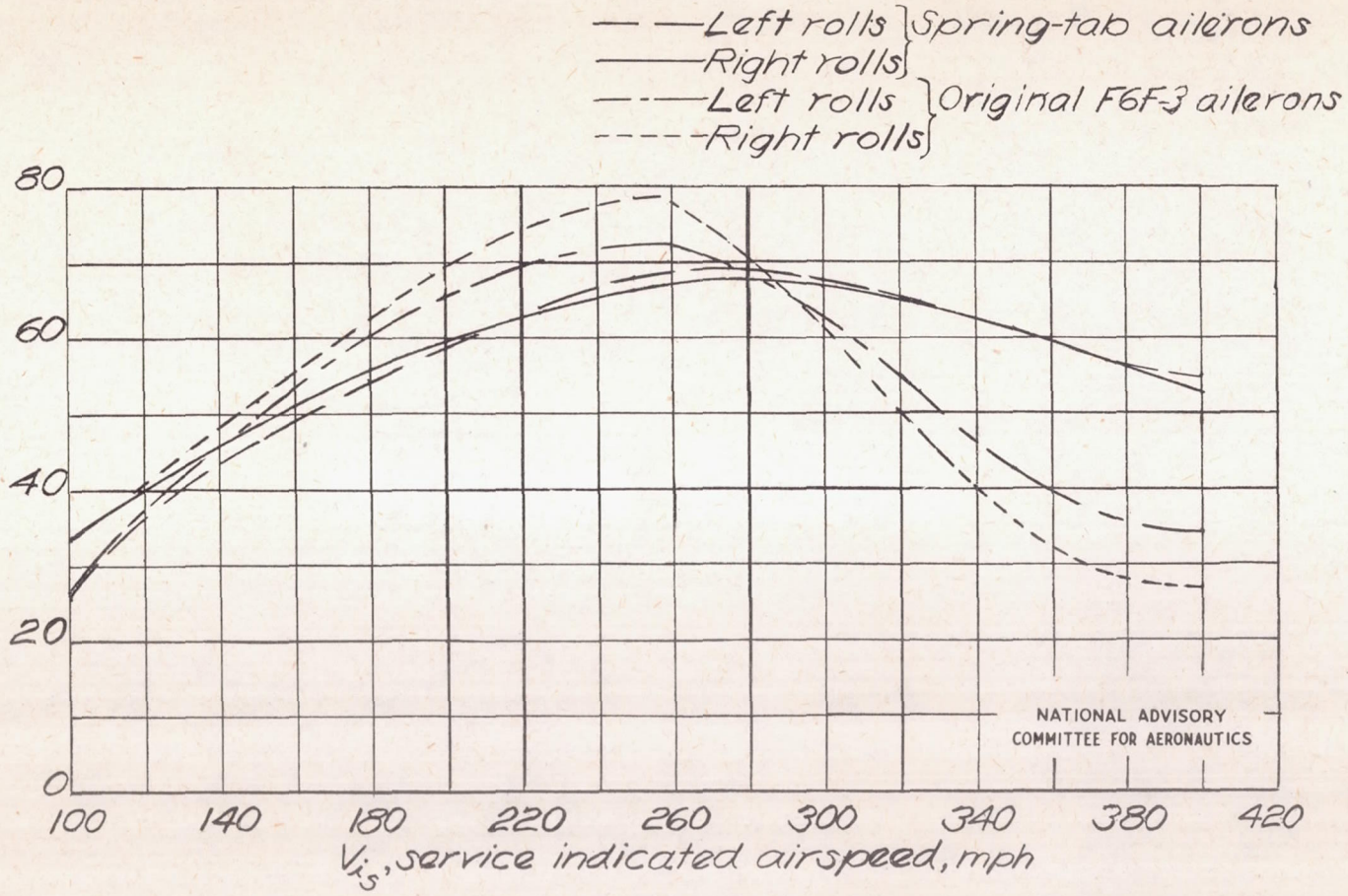
Figure 11.- Variation with correct service indicated airspeed of rolling velocity obtained at an altitude of 10,000 feet with full stick deflection or 30-pound stick force, whichever occurs first. F6F-3 airplane with spring-tab ailerons and with original F6F-3 ailerons.
