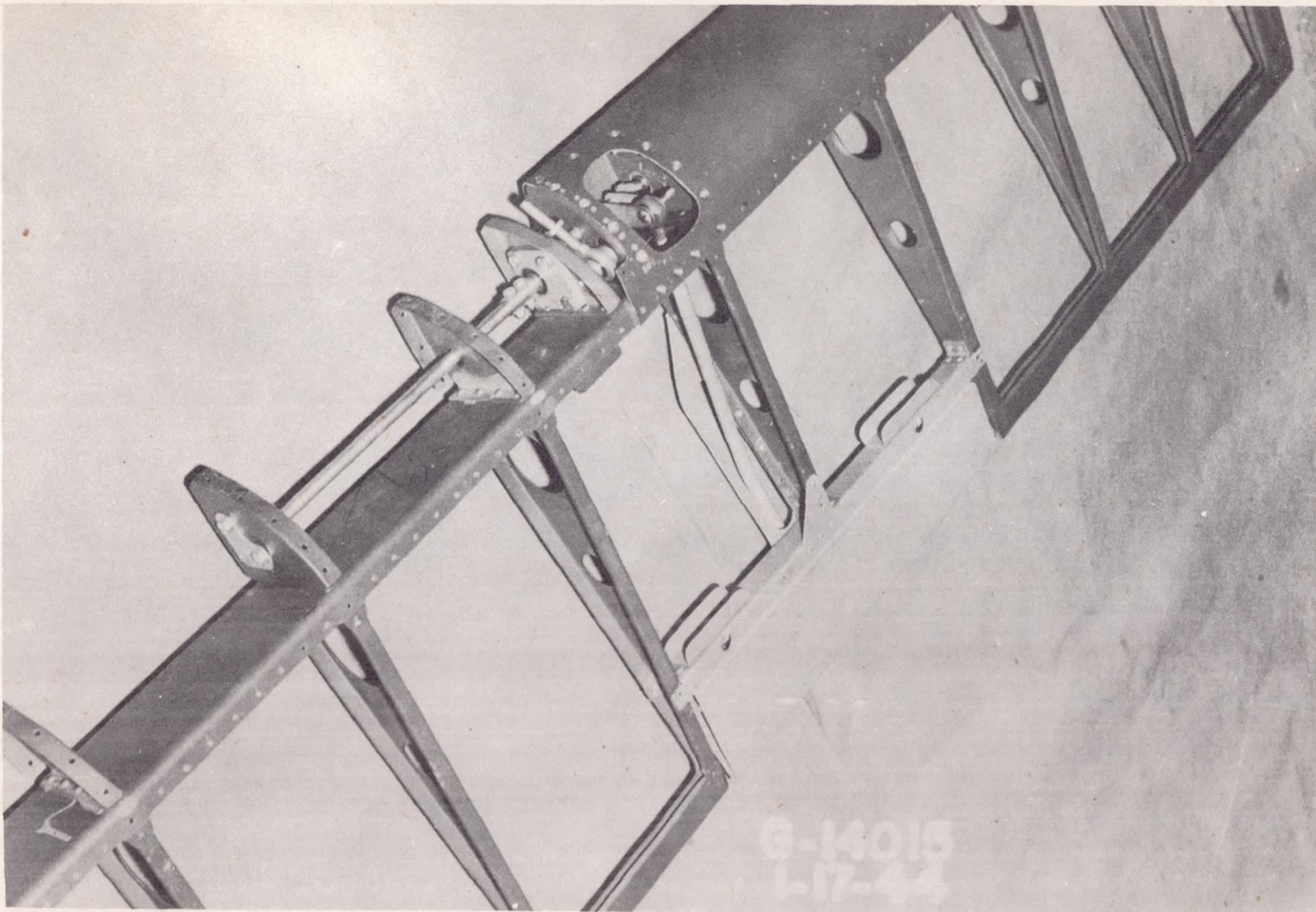
Figure 3.- Detail view of right spring-tab aileron. F6F-3 airplane. (Photograph furnished by Grumman Aircraft Engineering Corp.)
