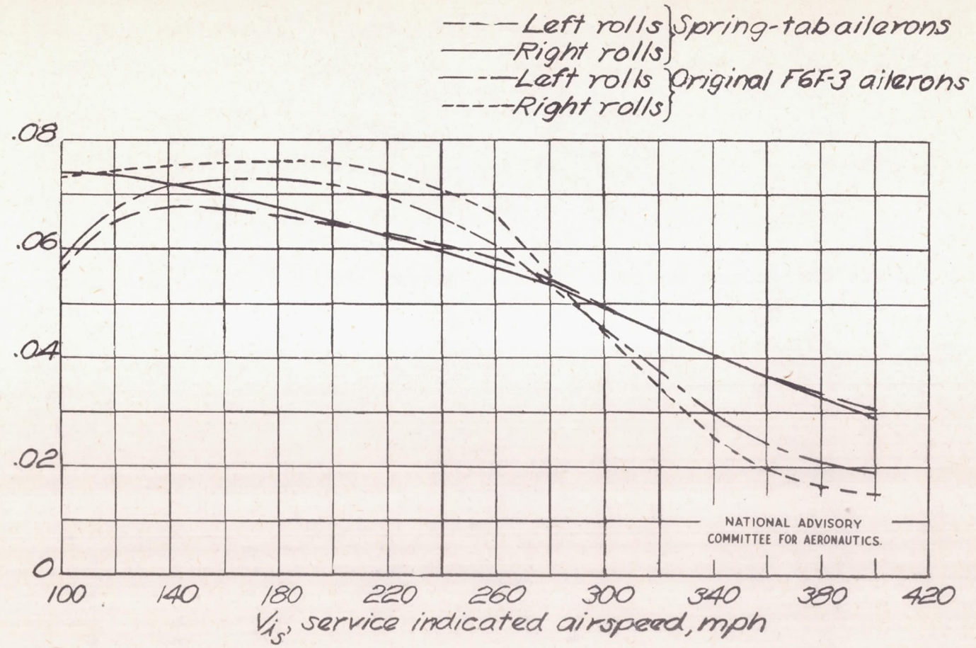
Figure 10.- Variation with correct service indicated airspeed of pb/2V obtained with full stick deflection or 30-pound stick force, whichever occurs first. F6F-3 airplane with spring-tab ailerons and with original F6F-3 ailerons.
