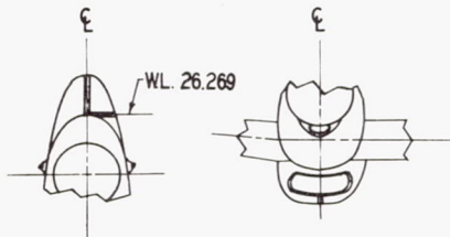
-CANOPY PRESSURE ORIFICE STATIONS- -RADIATOR PRESSURE ORIFICE STATIONS-
