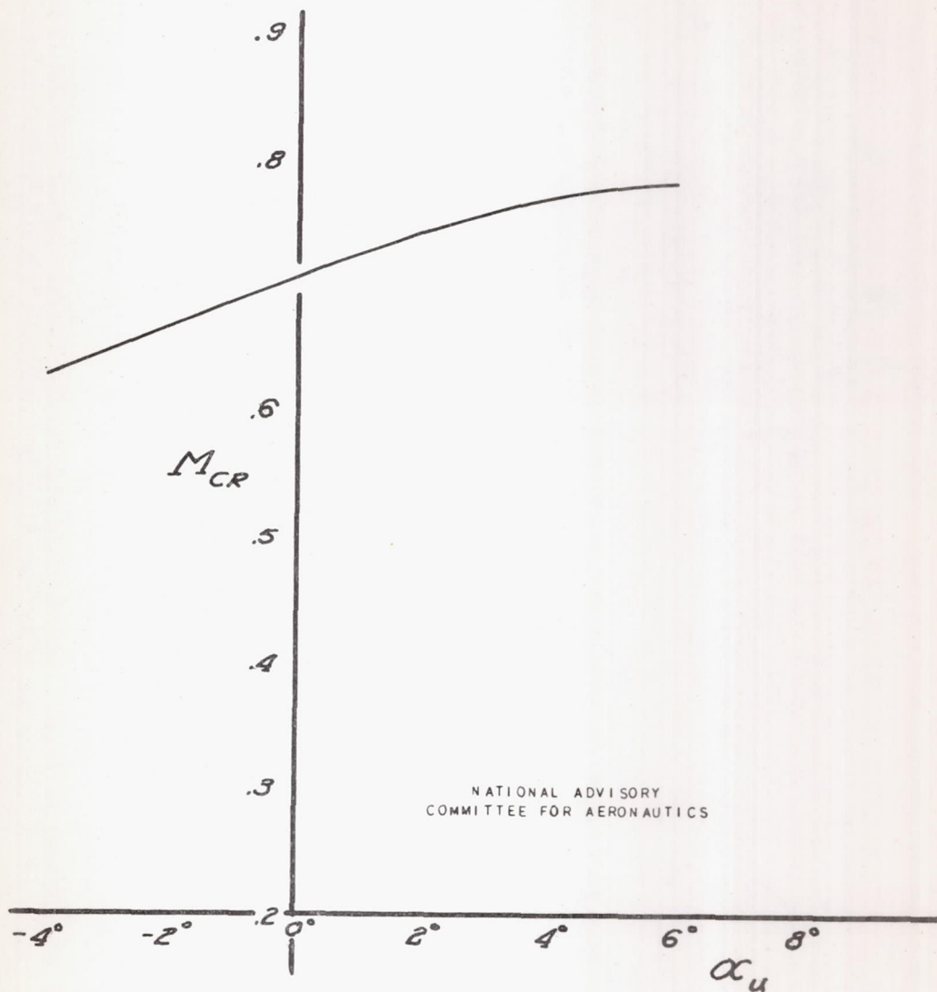
FIGURE 60:- VARIATION OF CRITICAL MACH NUMBER WITH ANGLE OF ATTACK OVER THE ENTRANCE OF THE COOLANT-RADIATOR DUCT ON THE MODEL. MODEL COMPLETE WITH AMES FILLETS AND PRESSURE-TUBE STAUT.
