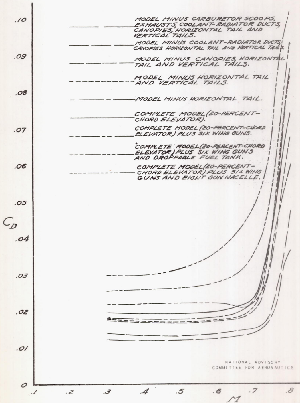
FIGURE 39:- VARIATION OF DRAG COEFFICIENT WITH MACH NUMBER FOR SEVERAL CONFIGURATIONS OF THE MODEL WITH AMES FILLETS. C_L, 0.0
