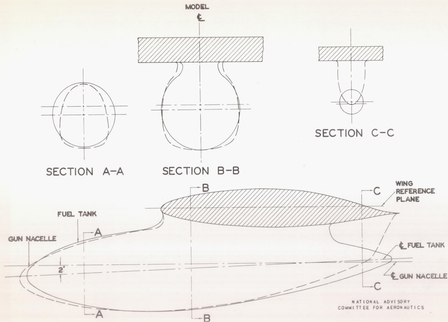
FIGURE 4:- DROPPABLE FUEL TANK AND EIGHT-GUN NACELLE ATTACHED TO THE WING.
