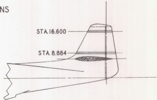
VERTICAL STABILIZER AND RUDDER -PRESSURE ORIFICE STATIONS-
