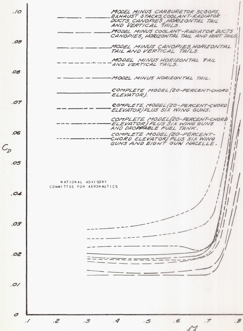
FIGURE 40:- VARIATION OF DRAG COEFFICIENT WITH MACH NUMBER FOR SEVERAL CONFIGURATIONS OF THE MODEL WITH AMES FILLETS. C_L, 0.2 .
