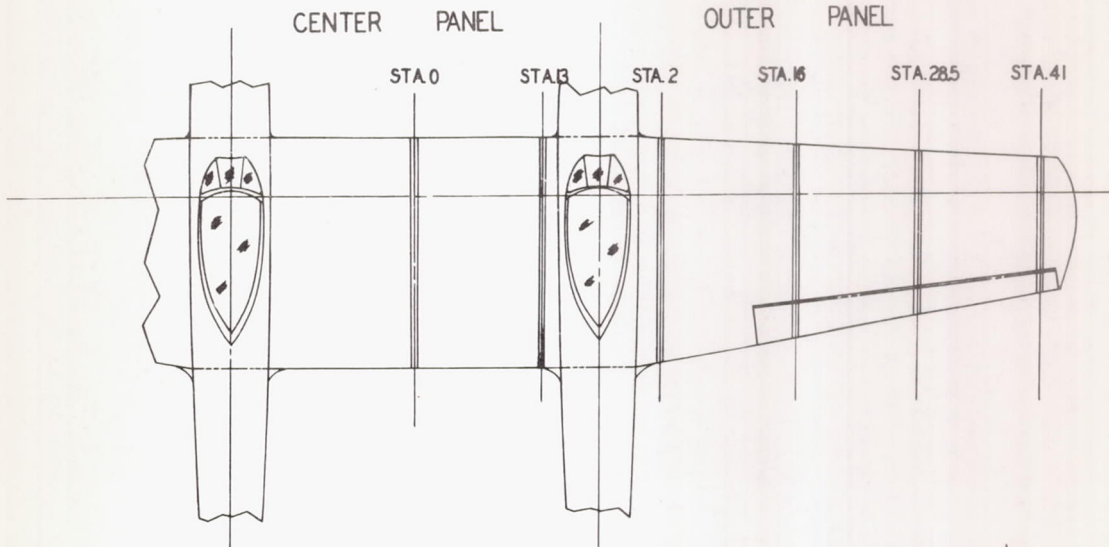
WING PRESSURE ORIFICE STATION LOCATIONS
