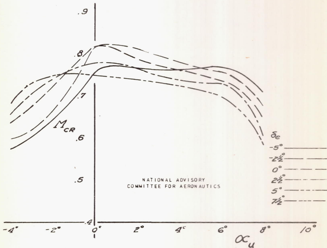
FIGURE 51:- VARIATION OF CRITICAL MACH NUMBER WITH ANGLE OF ATTACK FOR SEVERAL ELEVATOR DEFLECTIONS OF THE 32.8-PERCENT-CHORD ELEVATOR ON THE MODEL WITH THE MANUFACTURERS FILLETS, MODEL COMPLETE WITH PRESSURE-TUBE STRUT, HORIZONTAL-TAIL STATION 3.00 .
