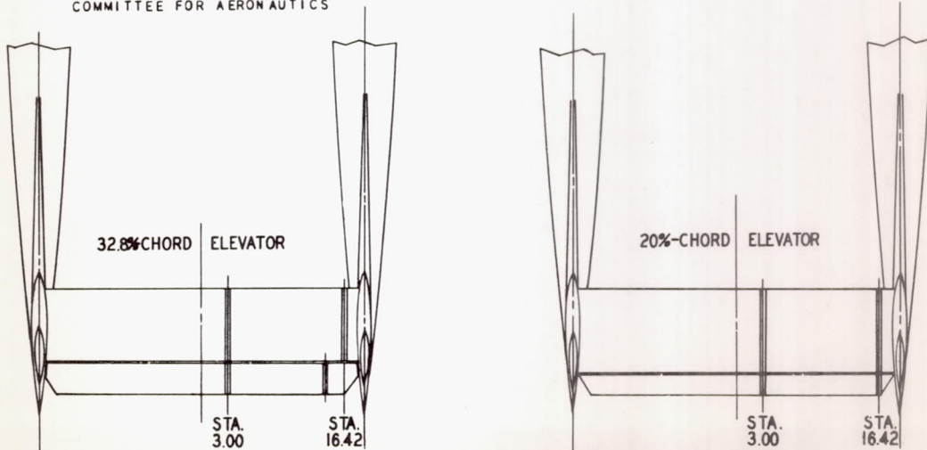
HORIZONTAL STABILIZER AND ELEVATOR PRESSURE ORIFICE STATIONS
