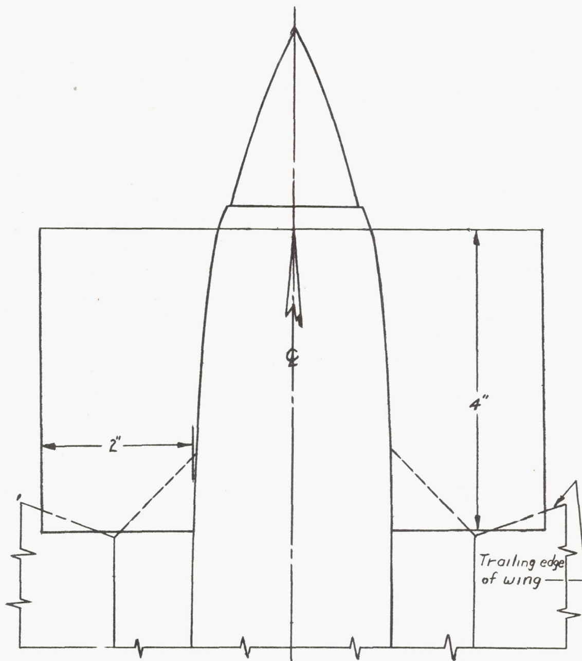
Figure 9. - Plan view of the 2-inch by 4-inch cowl fins tested on the 0.059-scale model of the XP-55 airplane. Cowl fins are in horizontal plane through thrust line. Dimensions are model scale.
