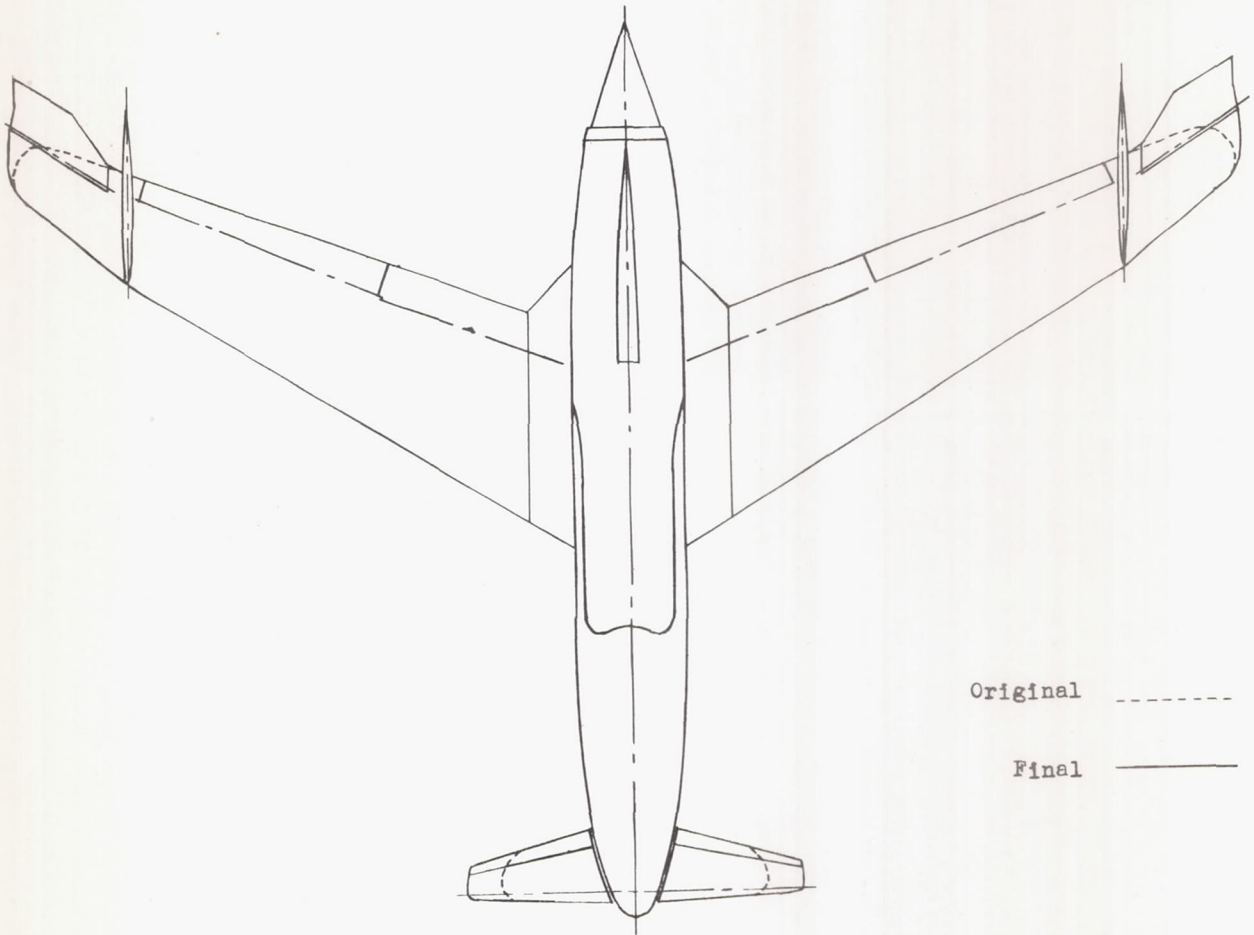
Figure 11.- Comparison of original and final configurations of the 0.059-scale model of the XP-55 airplane.
