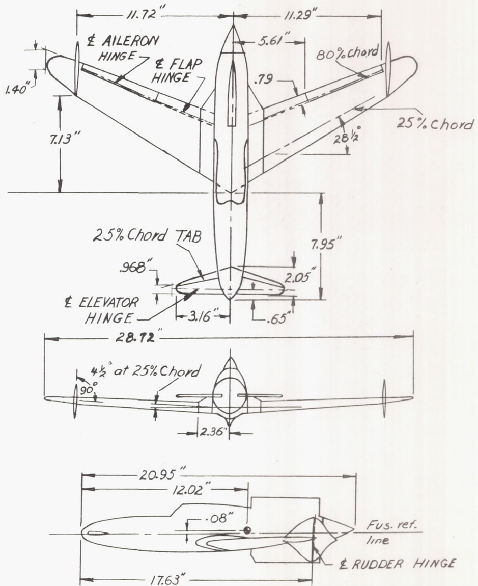
Figure 1.- The 0.059-scale model of the Curtiss-Wright XP-55 airplane tested in the 15-foot free-spinning tunnel. Wing root chord incidence, 4.25^\circ , leading edge up. Tip chord incidence, 0.75^\circ , leading edge up. Center-of-gravity location shown is for the normal loading with the landing gear retracted.
