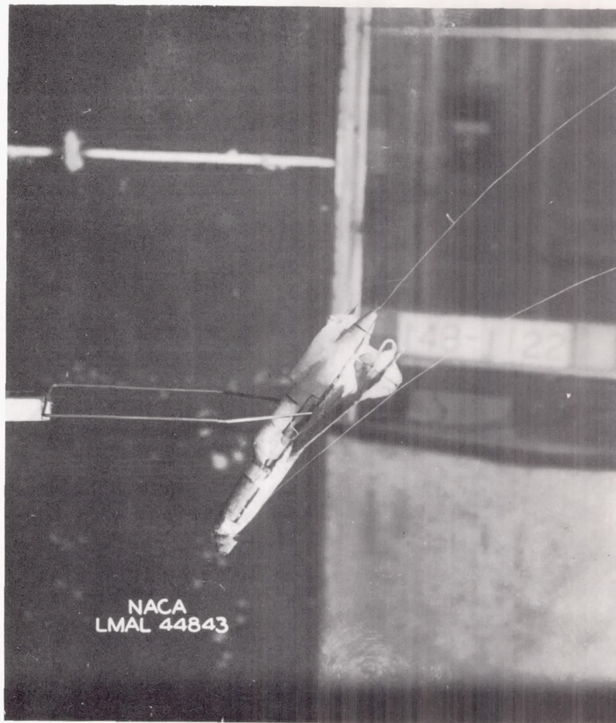
Figure 10.- The 0.059-scale model of the XP-55 airplane as mounted on the longitudinal-trim rig.
