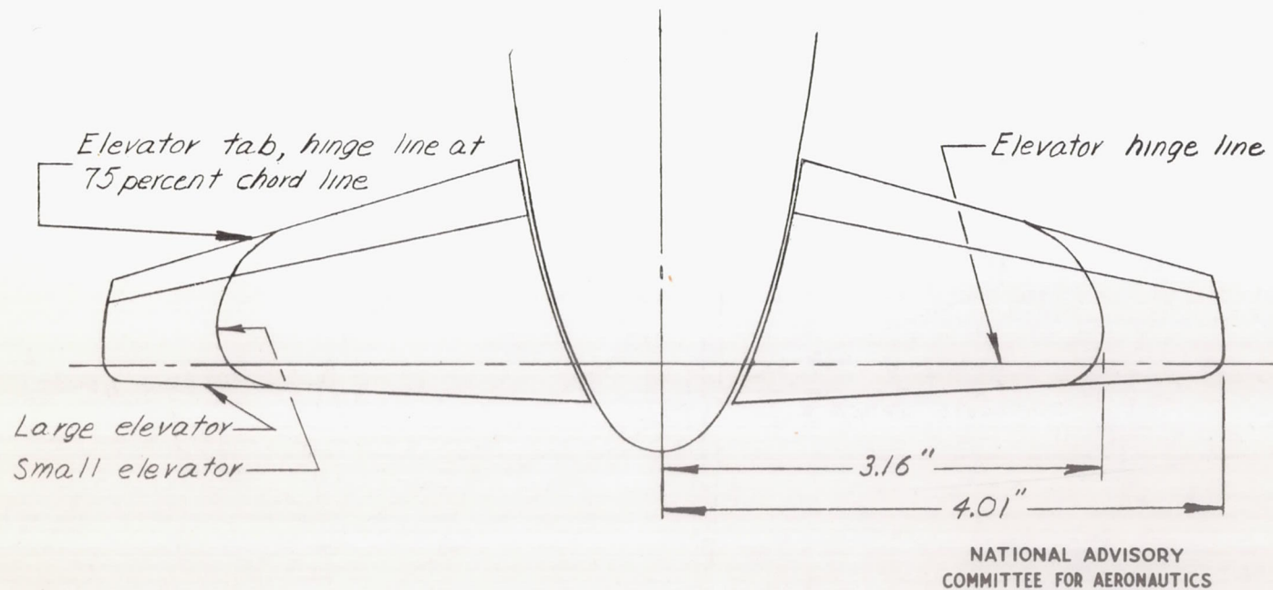
Figure 4.- Large and small elevators tested on the 0.059-scale model of the XP-55 airplane. Dimensions are model scale.
