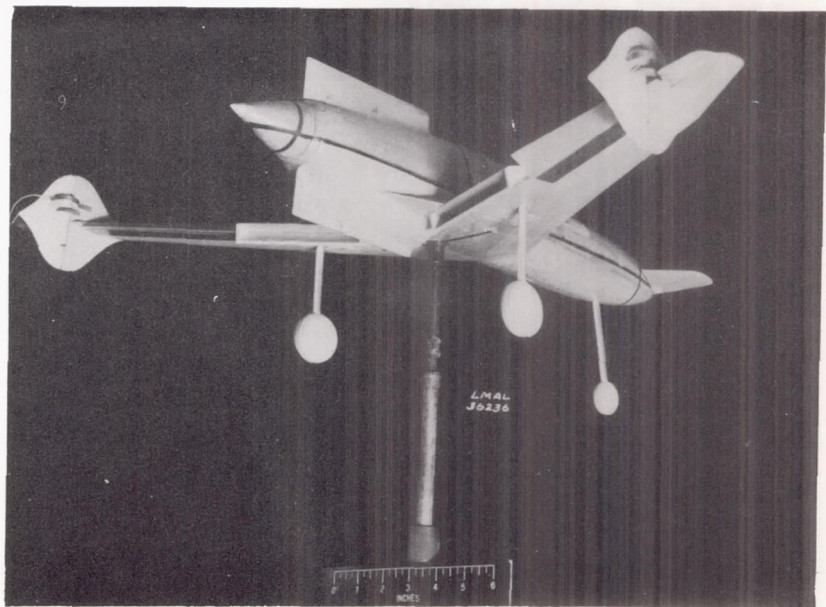
Figure 3.- The 0.059-scale model of the Curtiss-Wright XP-55 airplane in the clean and landing conditions.
