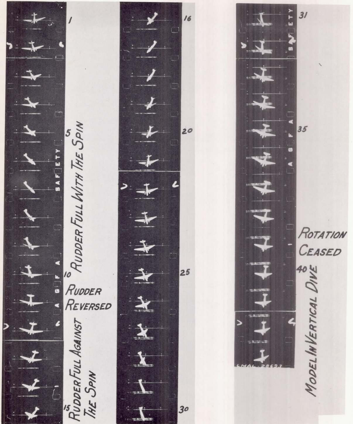
Figure 6.- Recovery from an elevator-neutral spin. Control settings: rudder as noted, elevator neutral, ailerons neutral. Recovered in 1 turn (frames 11 to 39).
