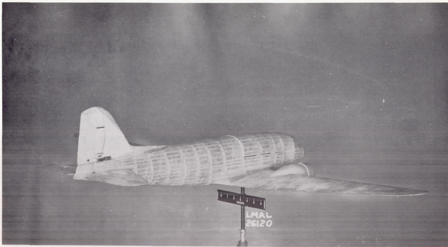
Figure 4.- Three-quarter rear view of the \frac{1}{23.75} -scale model of the Douglas DC-3 airplane.
