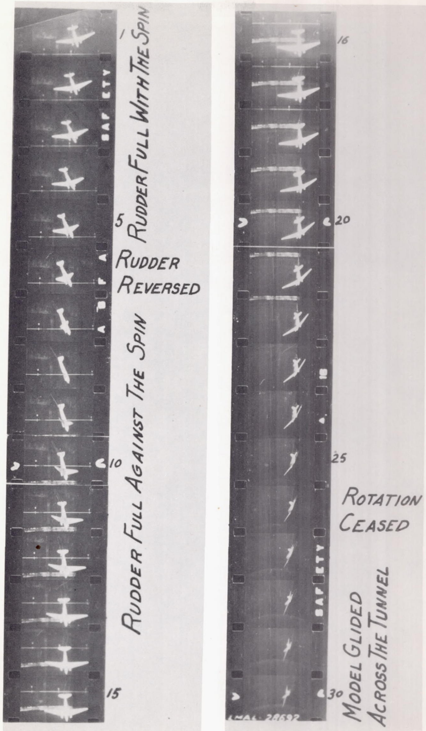
Figure 5.- Recovery from an elevator-up spin. Control settings: rudder as noted, elevator full up, ailerons neutral. Recovered in \frac{1}{2} turn (frames 6 to 26).
