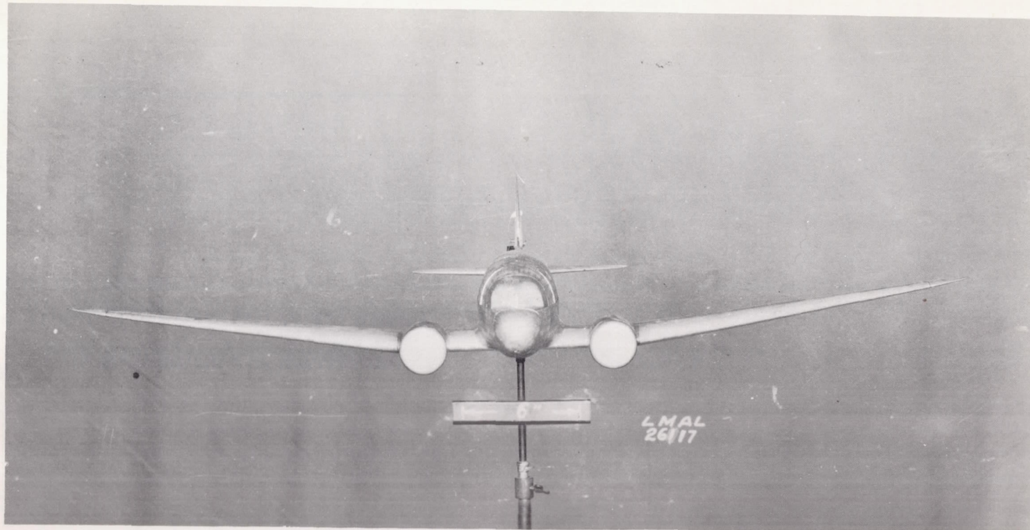
Figure 1.- Front view of the \frac{1}{23.75} -scale model of the Douglas DC-3 airplane.
