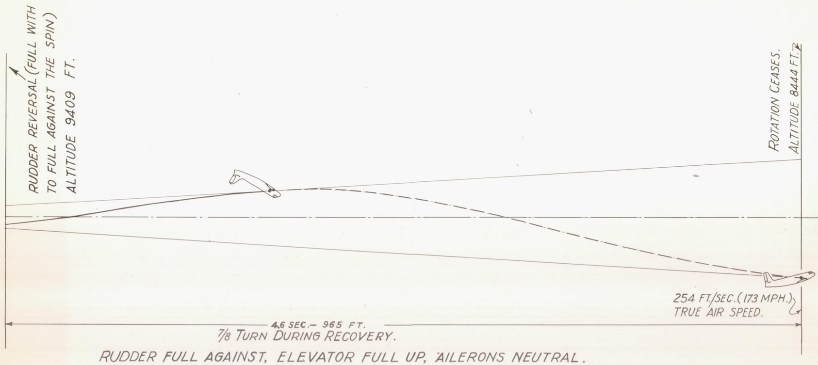
FIG. 9-(CONT.)- STEADY SPIN AND RECOVERY OF DC-3
