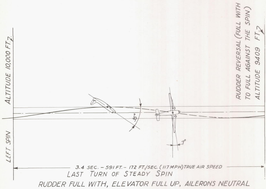
FIG. 9 - STEADY SPIN AND RECOVERY OF DC-3
