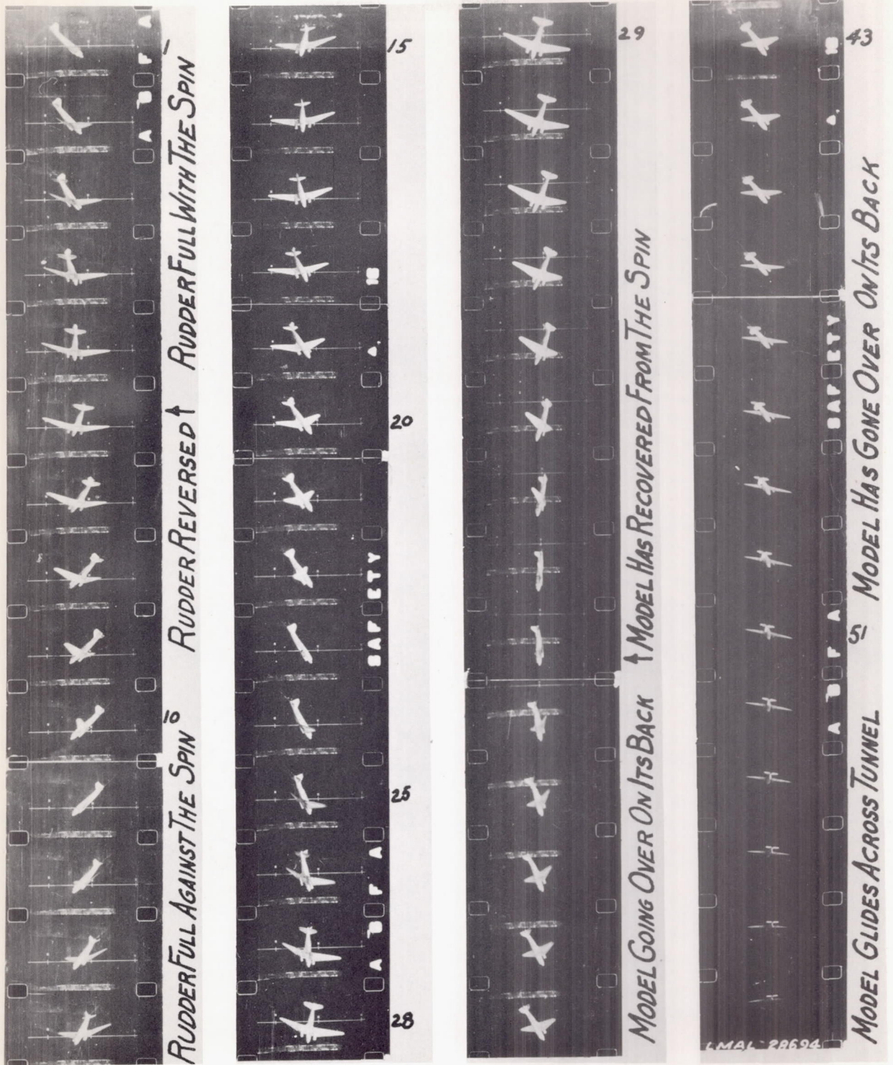
Figure 7.- Recovery from an elevator-down spin. Control settings: rudder as noted, elevator full down, ailerons neutral. Recovered in 1\frac{1}{4} turns (frames 6 to 37).
