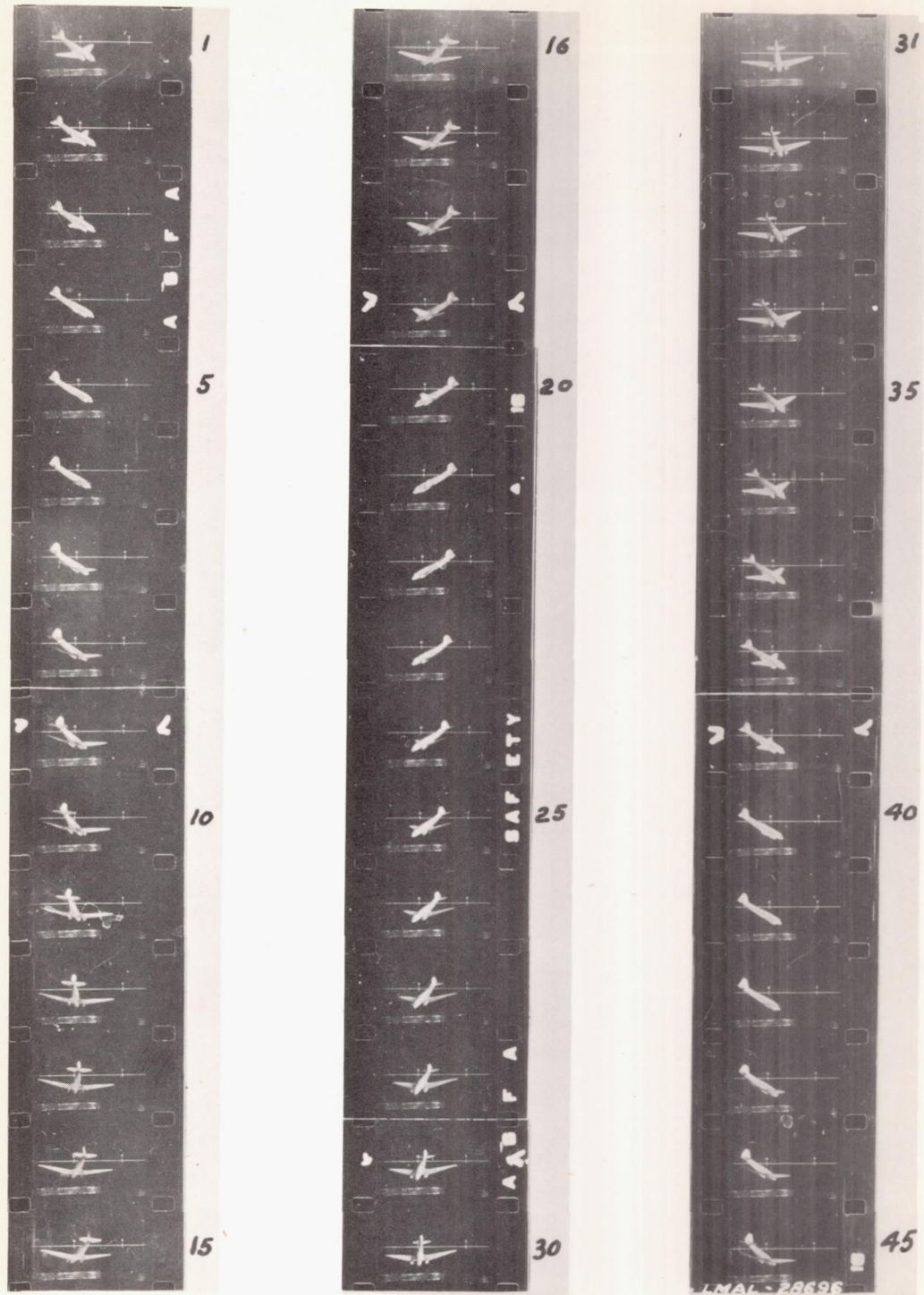
Figure 10.- Typical flat spin. Control settings: rudder full with the spin, elevator neutral, ailerons neutral. Full-scale values: \alpha = 63^\circ , \phi = 5^\circ , V = 121 ft/sec (82 mph), \Omega = 0.34 rev/sec, radius of spin = 3.5 ft.
