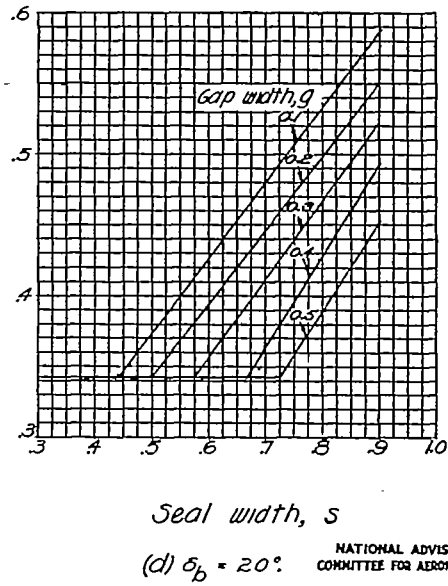
Figure 14.- Vertical clearance required for flexible seals with vertical-line backplates.
