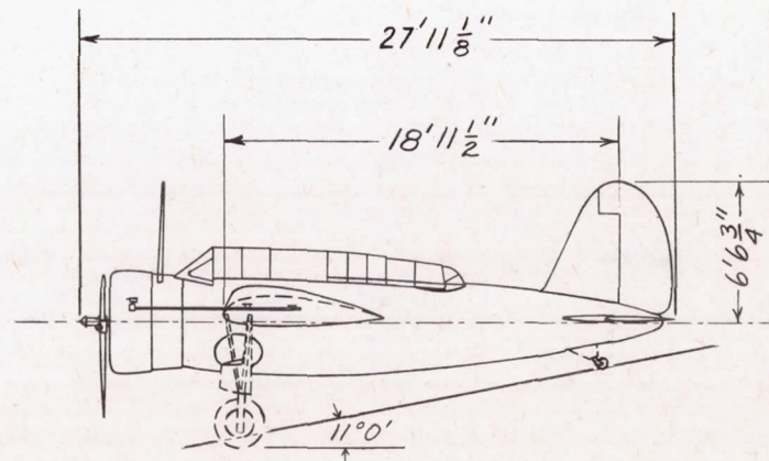
Figure 1.- Three-view drawing of Brewster XSBA-1 airplane with configuration 1.
