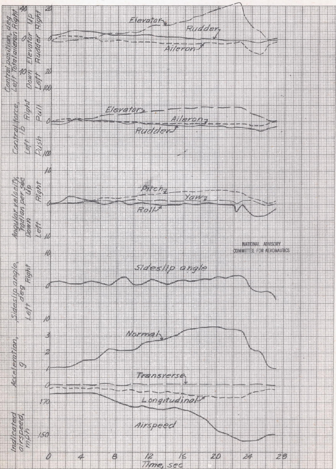
Figure 27.- Time history of a 3.5g right turn to the stall; Brewster XSBA-1 airplane with tail configuration 3; c.g. at 25.2 percent M.A.C.
