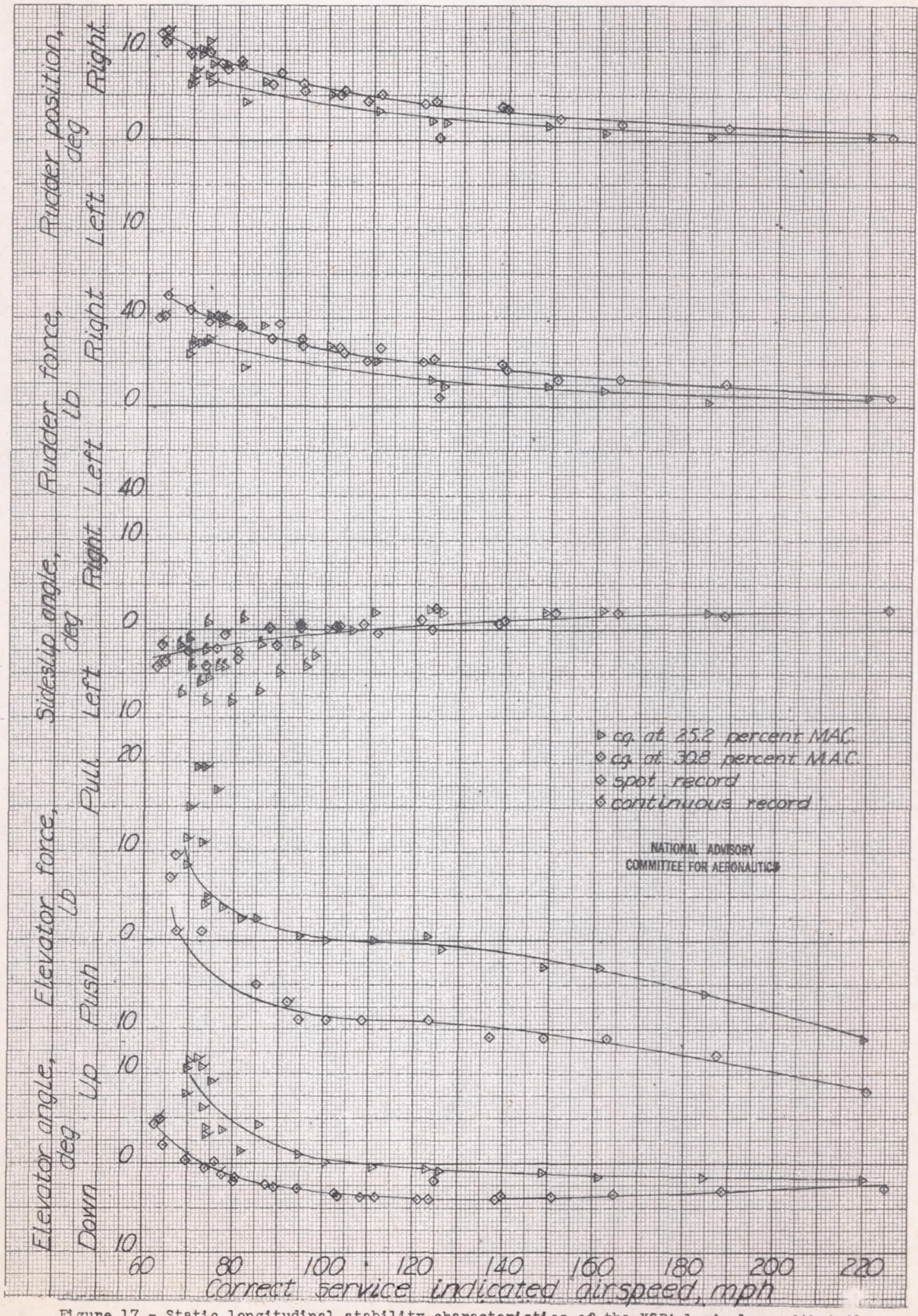
Figure 17.- Static longitudinal stability characteristics of the XSB-1 airplane with tail configuration 3 in the climbing condition.
