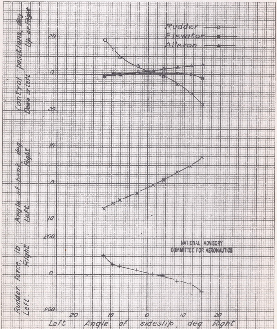
Figure 44.- Steady sideslip characteristics in the landing condition at 112 miles per hour (flaps down, landing gear down, power off); Brewster XSBA-1 airplane with tail configuration 3.
