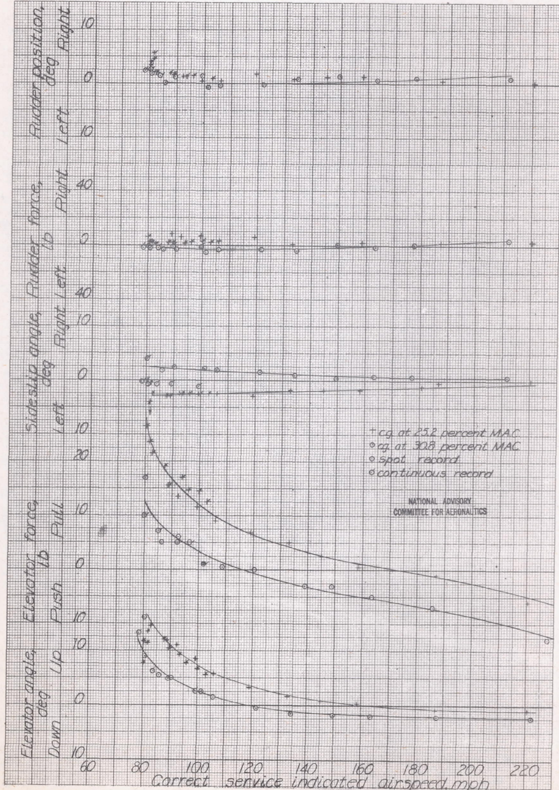
Figure 15.- Static longitudinal stability characteristics of the XSBA-1 airplane with tail configuration 3 in the gliding condition.
