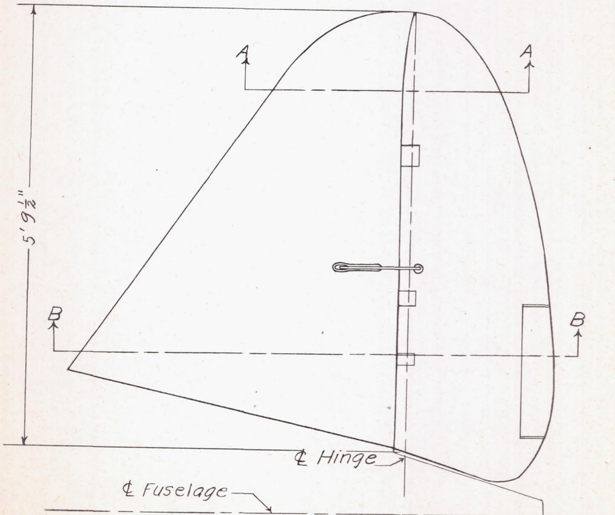
Figure 8.- Vertical tail configuration 3; Brewster XSBA-1 airplane.
