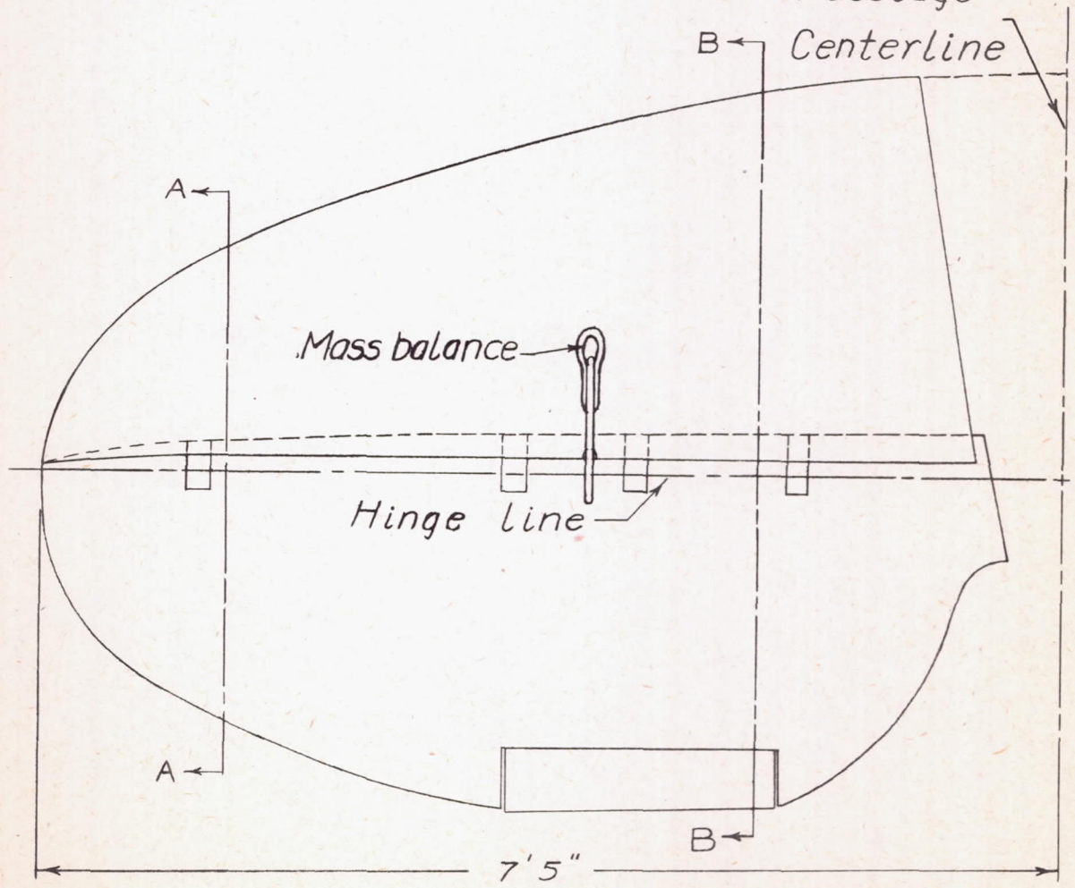
Figure 5.- Horizontal tail configuration number two. Brewster XSBA-1 airplane.
