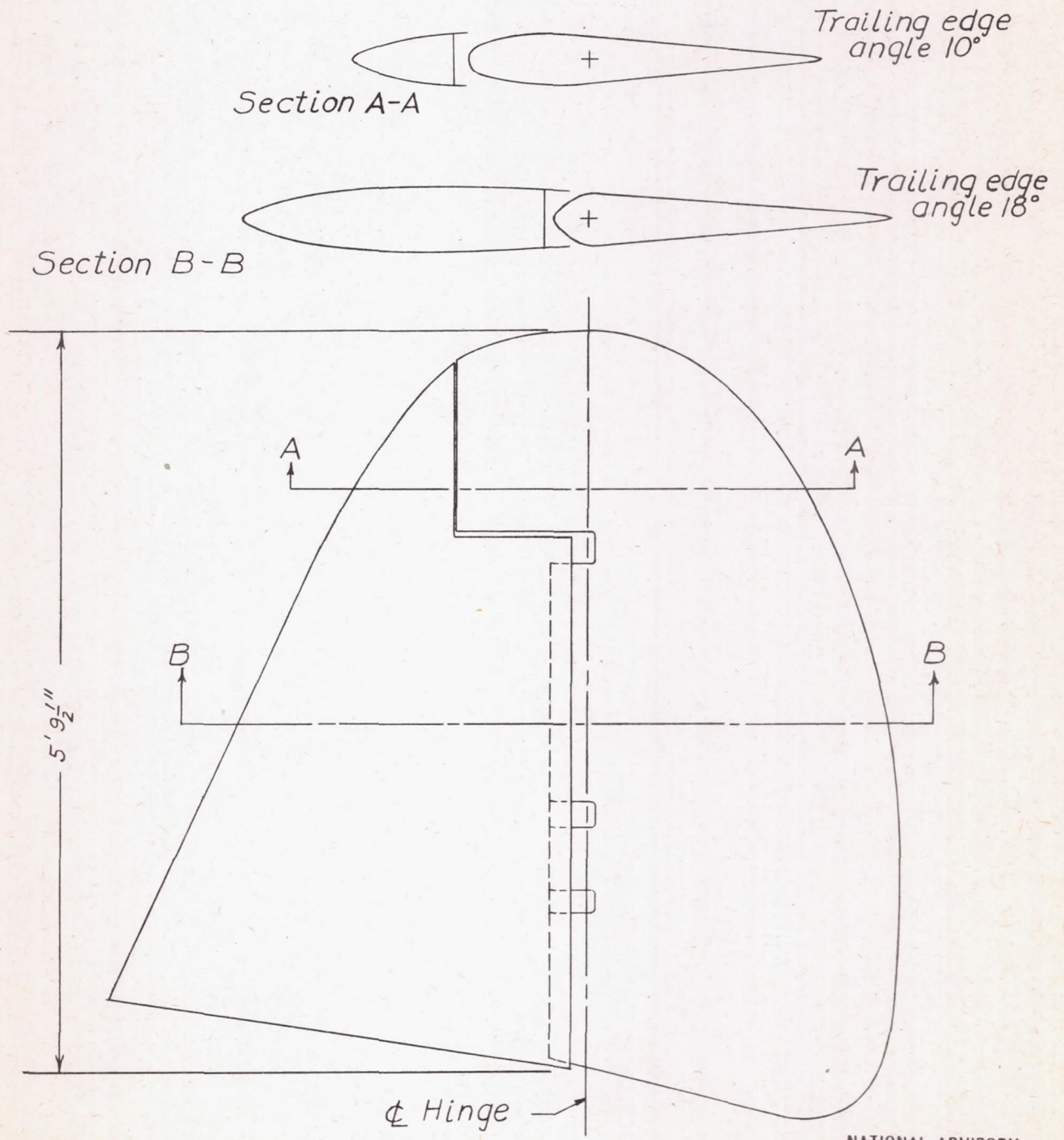
Figure 4.- Vertical tail configuration number one. Brewster XSB-1 airplane.
