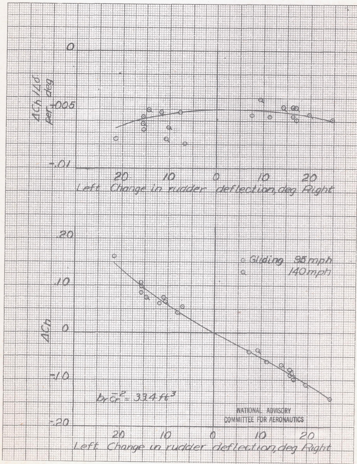
Figure 53.- Plots of \Delta C_h / \Delta \delta and \Delta C_h for constant \alpha against change of rudder deflection during rudder kicks; XSBA-1 airplane with tail configuration 2.
