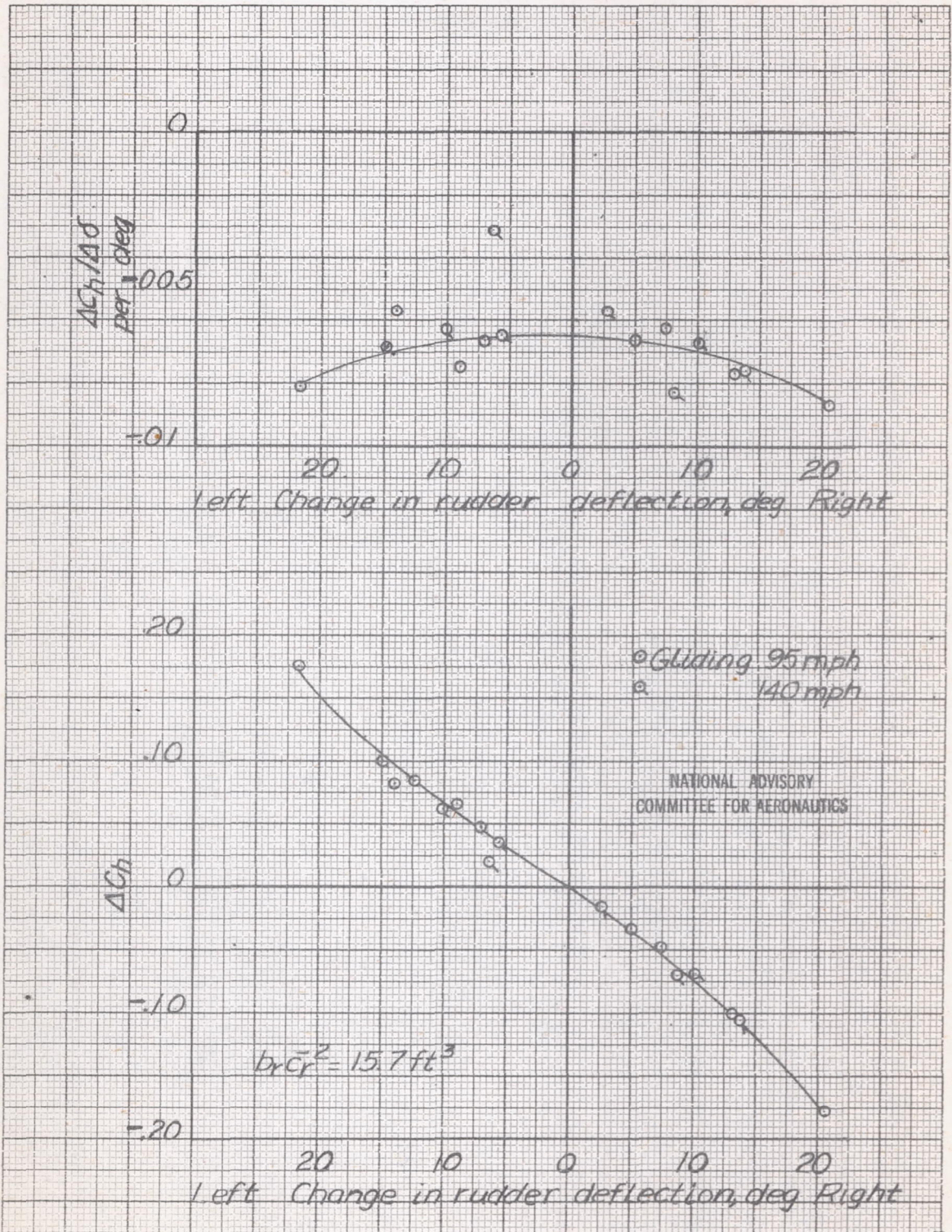
Figure 54.- Plots of \Delta C_h / \Delta \delta and \Delta C_h for constant \alpha against change of rudder deflection during rudder kicks; XSBA-1 airplane with tail configuration 3.
