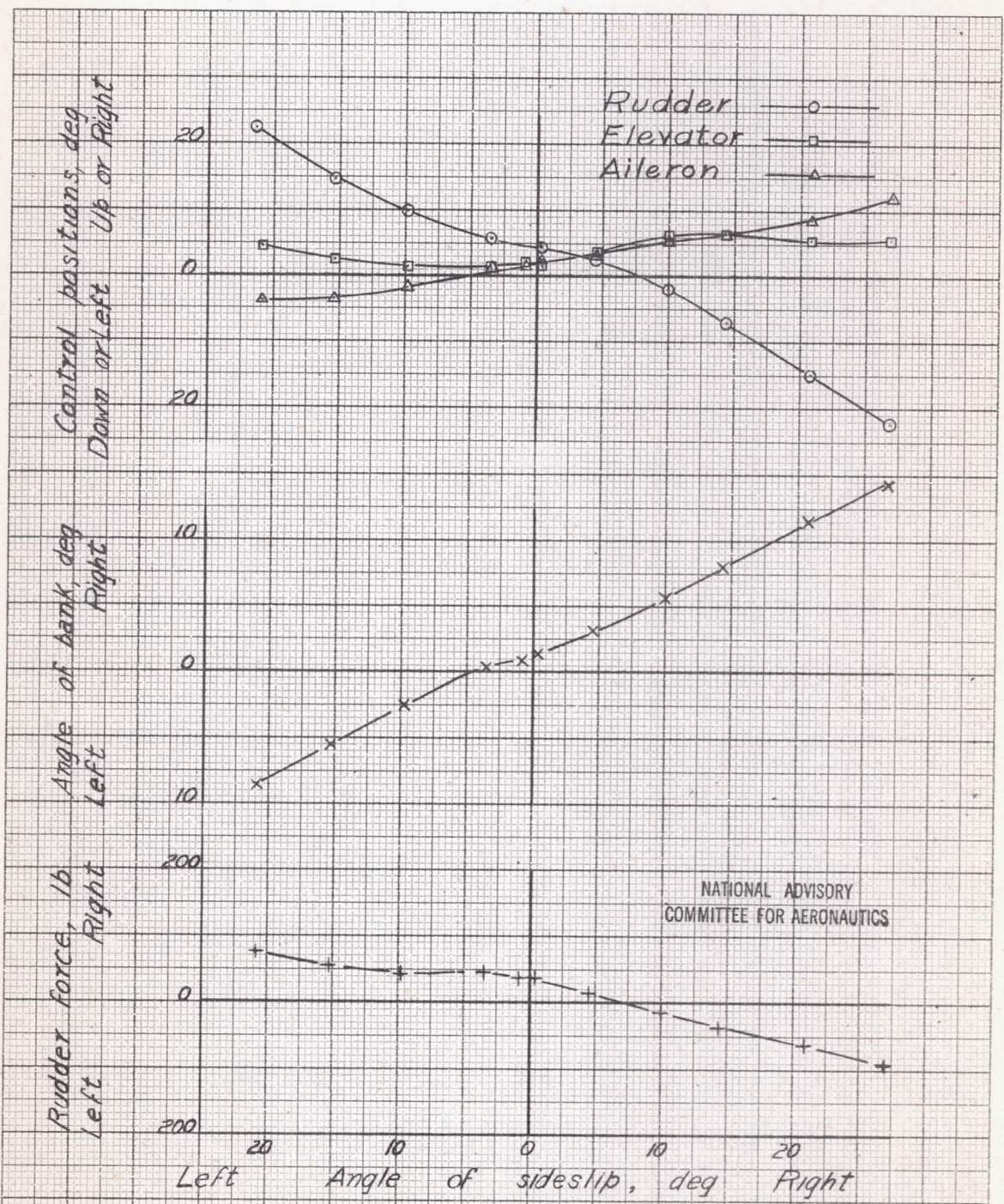
Figure 41.- Steady sideslip characteristics in the cruising condition at 87 miles per hour (flaps up, landing gear up, cruising power); Brewster XSBA-1 airplane with tail configuration 3.
