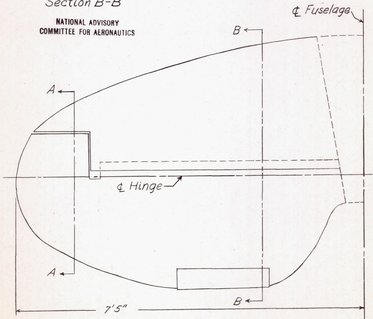
Figure 3.- Horizontal tail configuration number one. Brewster XSBA-1 airplane.
