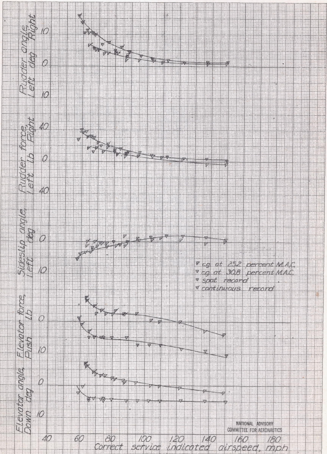
Figure 13.- Static longitudinal stability characteristics of the XSEA-1 airplane with tail configuration 3 in the approach condition.
