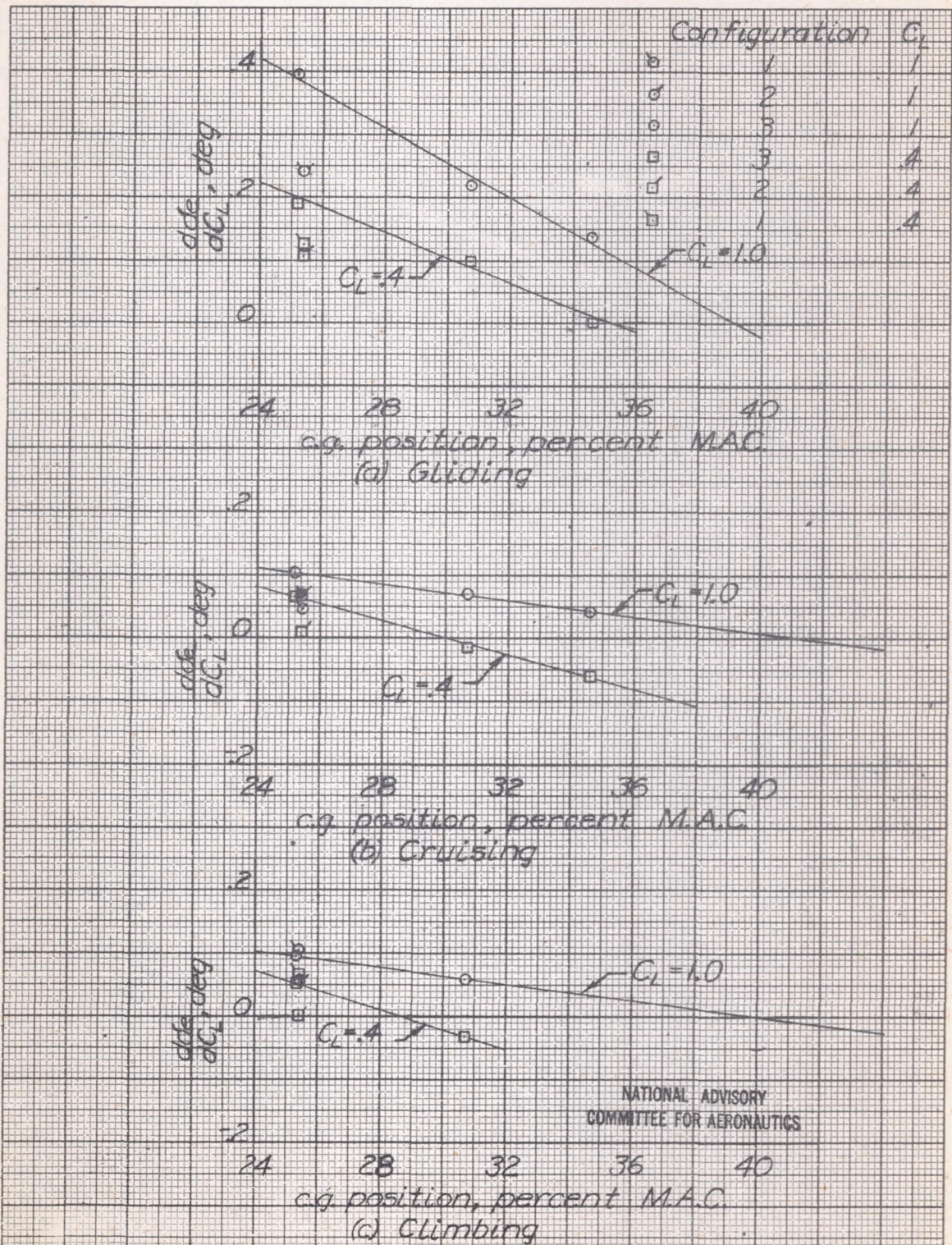
Figure 21.- Plots showing stick-fixed neutral points in various flight conditions for the XSBA-1 airplane.
