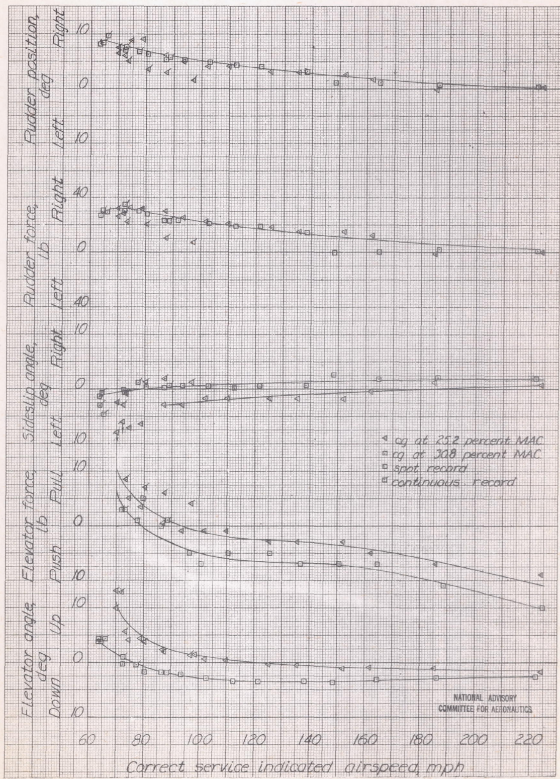
Figure 16.- Static longitudinal stability characteristics of the XSBA-1 airplane with tail configuration 3 in the cruising condition.
