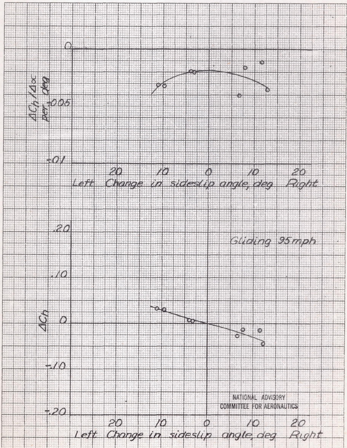
Figure 56.- Plots of \Delta C_h / \Delta \alpha and \Delta C_h against change of sideslip angle during rudder kicks; XSBA-1 airplane with tail configuration 3.
