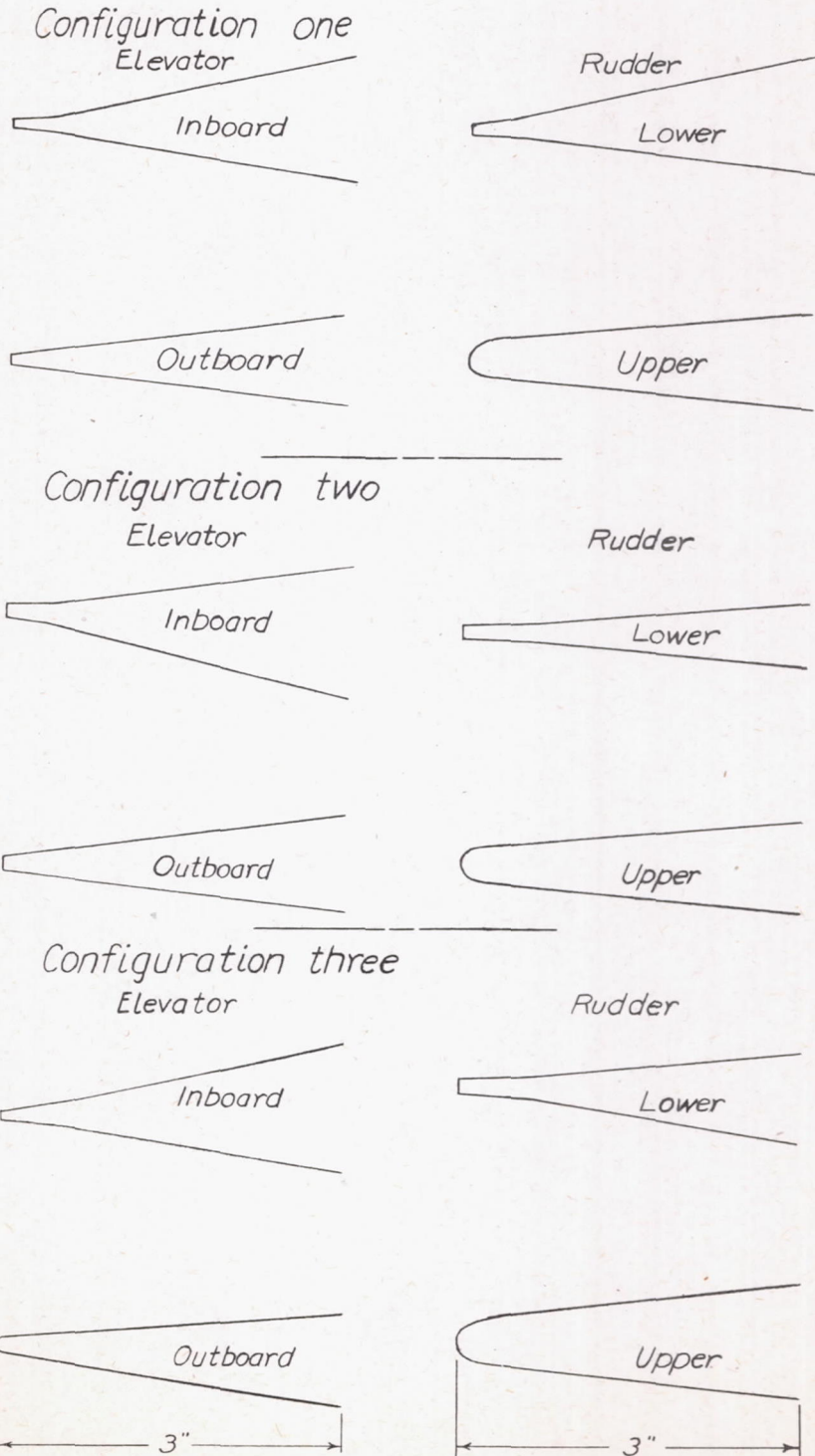
Figure 11.- Trailing edge sections of X8BA-1 tail surfaces at the stations indicated in figures 3 through 8.
