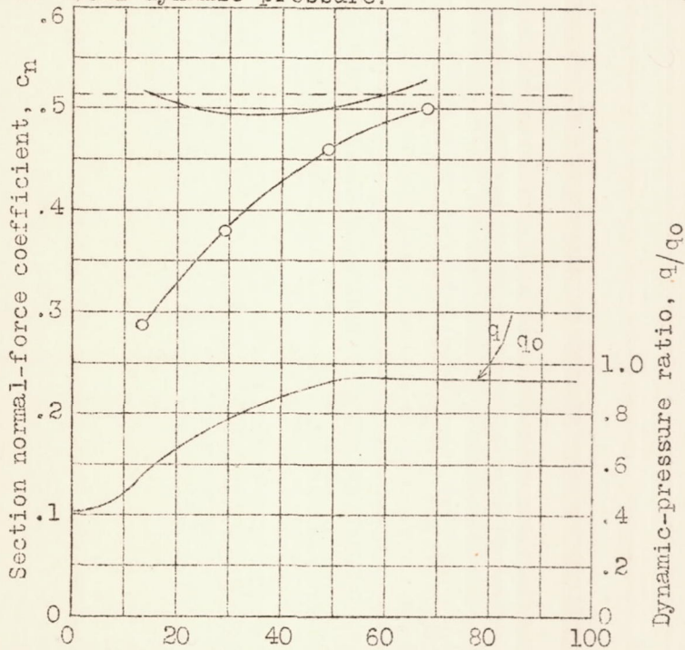
Figure 35.- Comparison of the measured and calculated normal-force distributions on the horizontal tail, \alpha_T, 15.6^\circ, \delta_e, 0^\circ .
