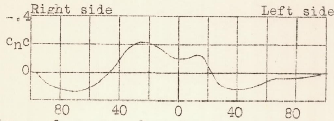
Figure 34.- Stabilizer span load distribution, \alpha_T, 0^\circ, \delta_e, 3^\circ .
