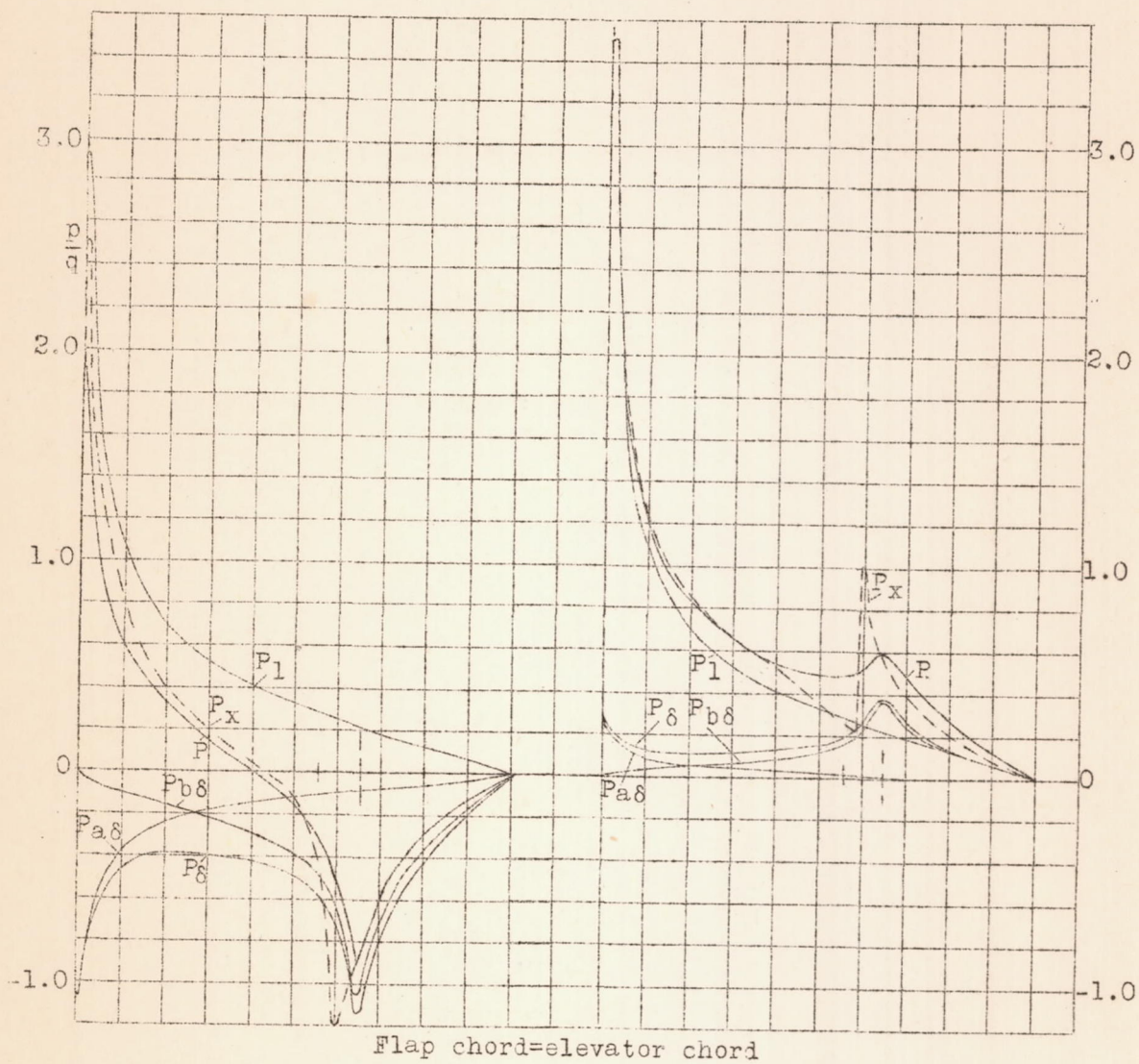
Figure 38.- Pressure distributions on rib 2. \alpha_{fl}, 15.6^\circ; \delta_e, -15^\circ. Figure 39.- Pressure distributions on rib 2. \alpha_{fl}, 15.6^\circ; \delta_e, 50^\circ.
