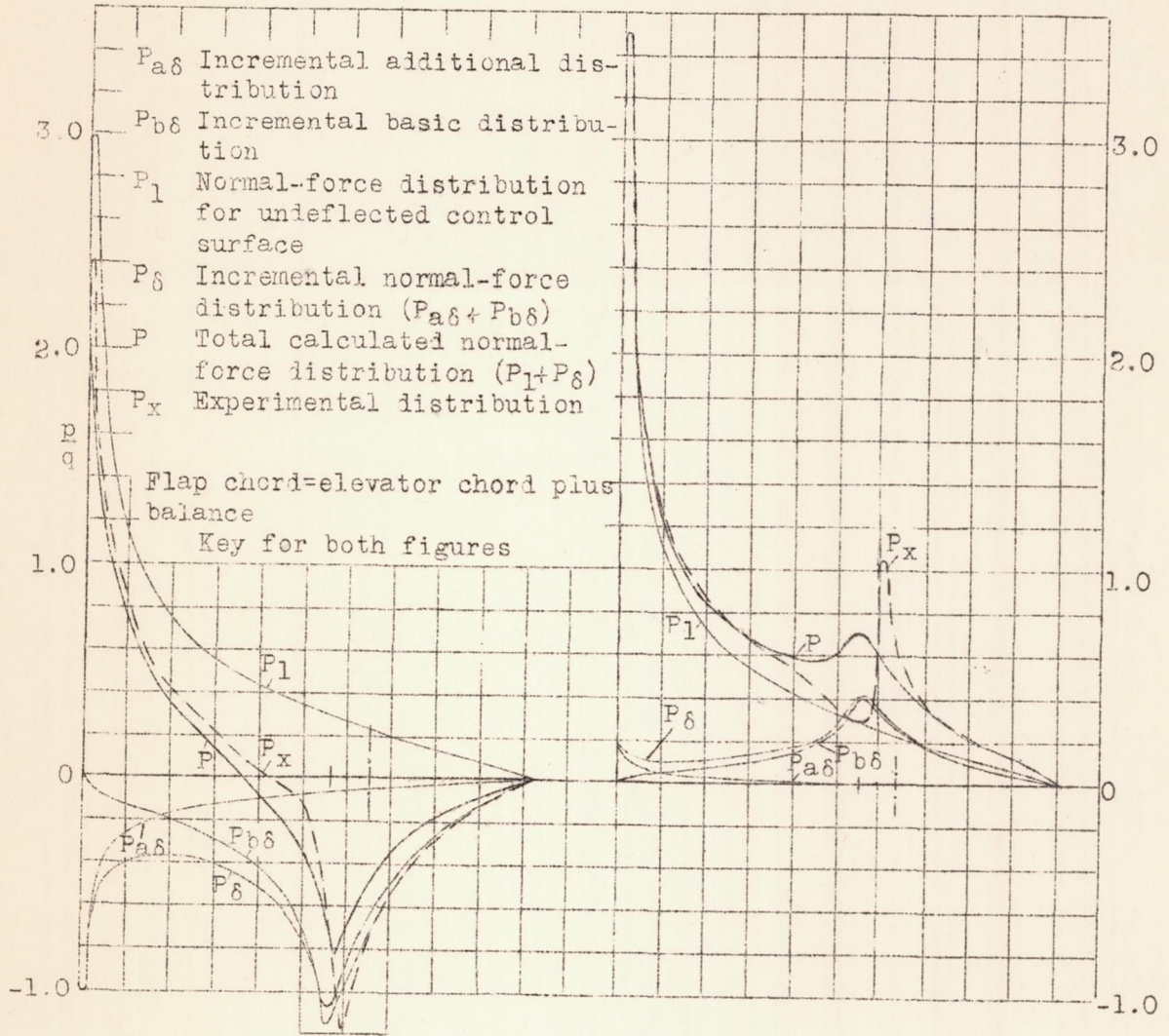
Figure 36.- Pressure distributions on rib 2, \alpha_T, 15.6^\circ; \delta_e, -15^\circ . Figure 37.- Pressure distributions on rib 2, \alpha_T, 15.6^\circ; \delta_e, 5^\circ .
