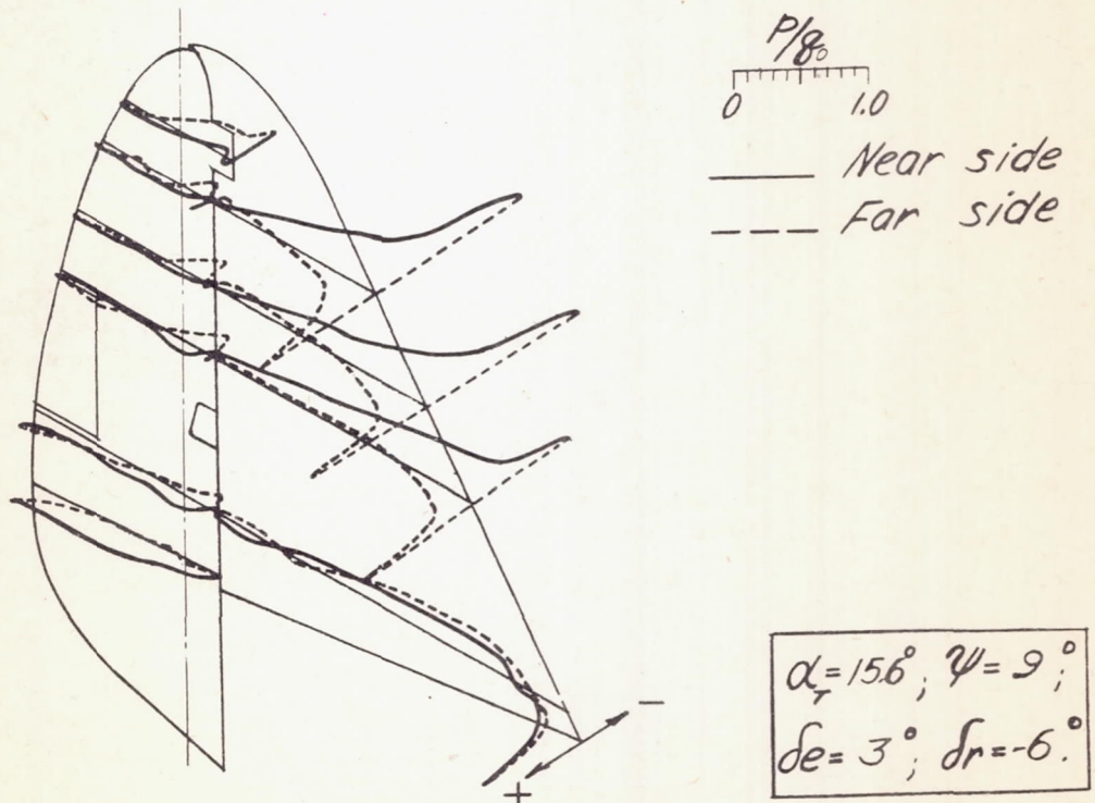
Figure 14. - Vertical tail surface pressure distribution.
