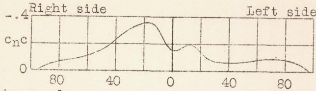
Figure 33.- Stabilizer span load distribution, \alpha_T, 0^\circ, \delta_e, 0^\circ .
