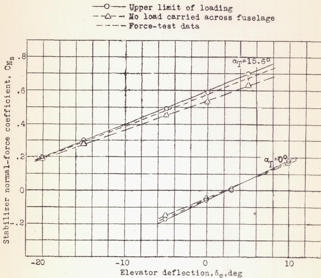
Figure 16.- Determination of stabilizer loading carried across fuselage.
