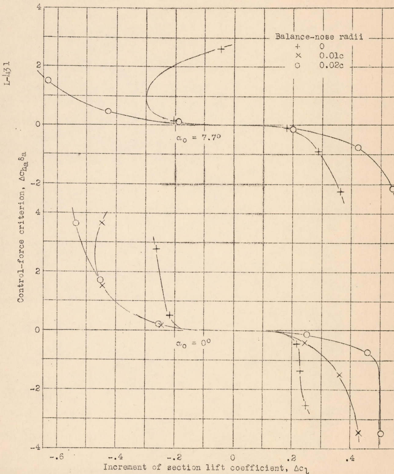
Figure 18.- Variation of \Delta Ch \delta a with \Delta Cl (by pressure distribution) showing effect of balance-nose radii. M = 0.358 ; gap = 0.0055c.
