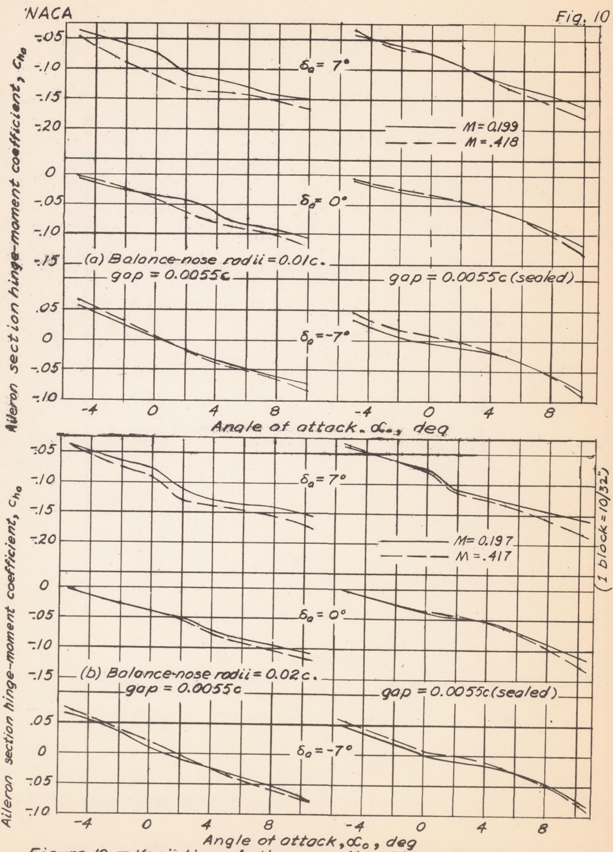
Figure 10. - Variation of aileron section hinge-moment coefficient with angle of attack.
