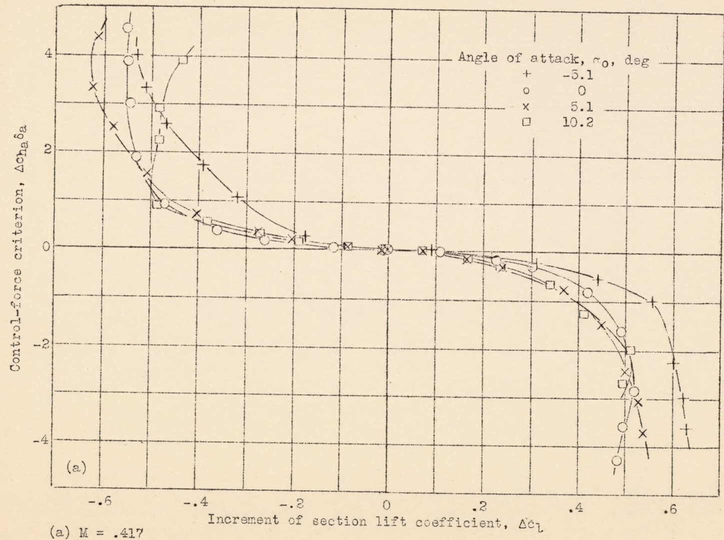
Figure 20(a,b).- Variation of control-force criterion with increment of section lift coefficient for the angle of attack range. Balance-nose radii = 0.02c; gap = 0.0055c.
