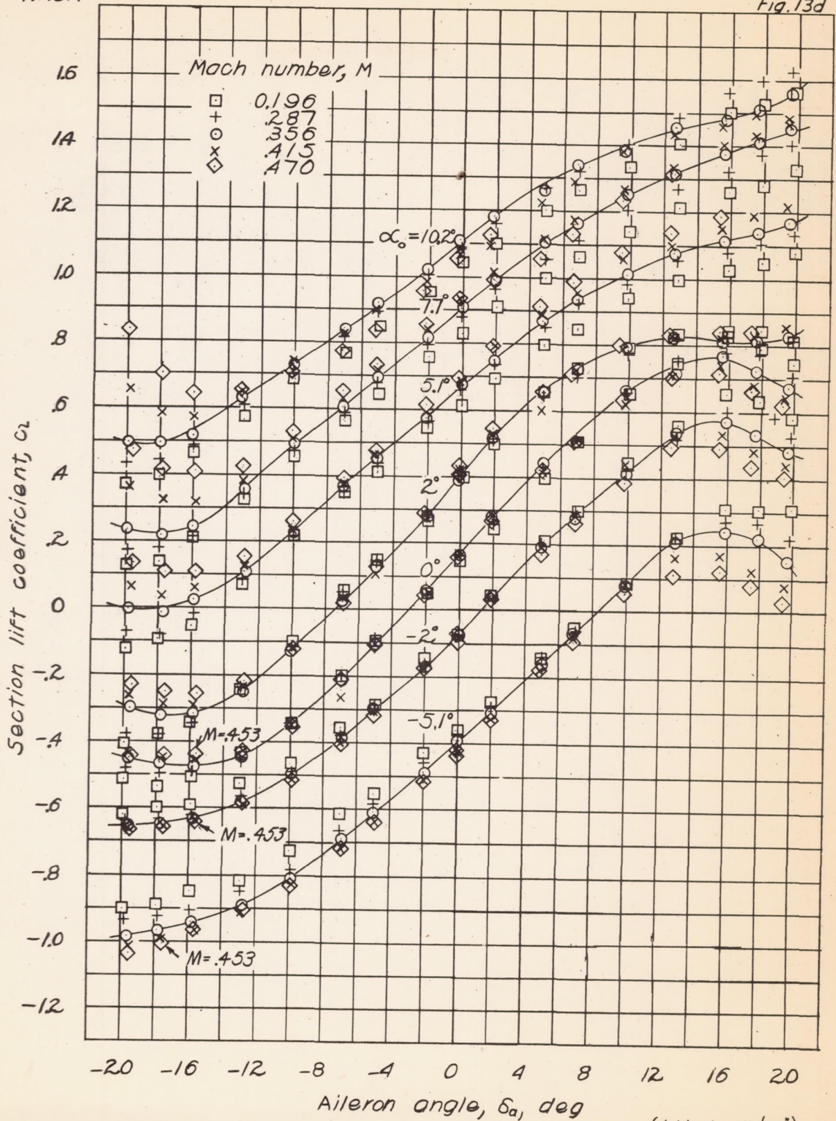
Figure 13. - Variation of section lift coefficient with aileron angle Balance nose radii = 0.02c. (Concluded)
