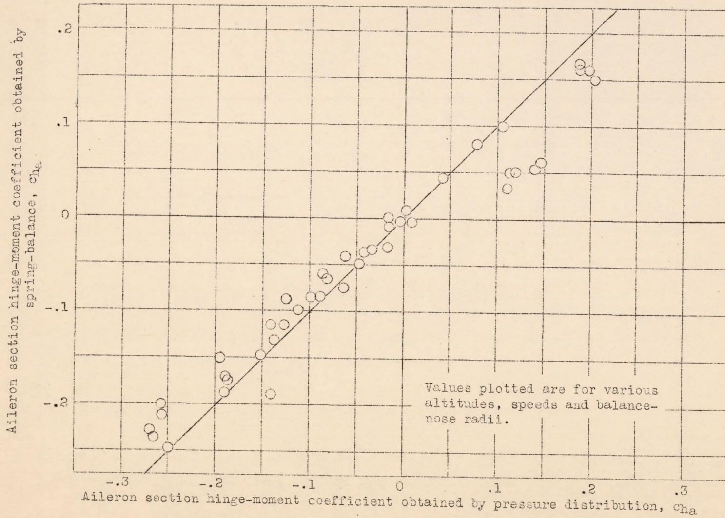
Figure 4.- A comparison between spring-balance and pressure-distribution section hinge-moment coefficients.
