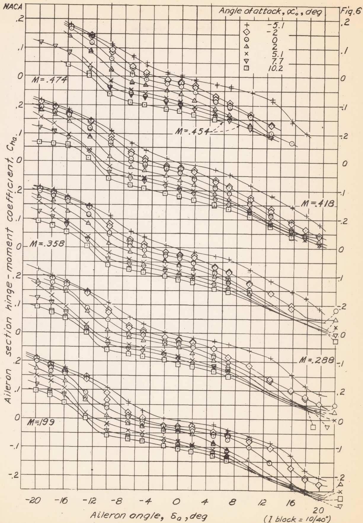
Figure 6. — Variation of aileron section hinge-moment coefficient with aileron angle. Balance-nose radii = 0.01c ; gap = 0.0055c .
