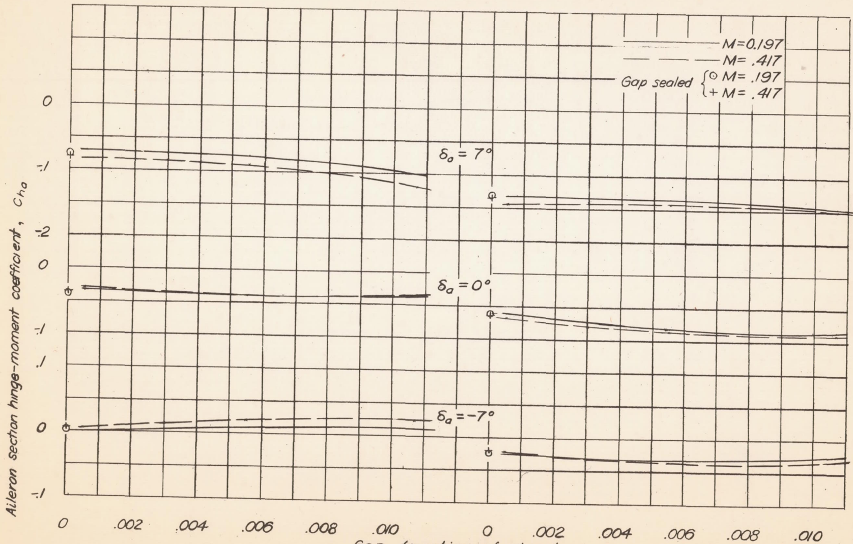
Figure 9.- Variation of aileron section hinge-moment coefficient with gap. (Continued)
