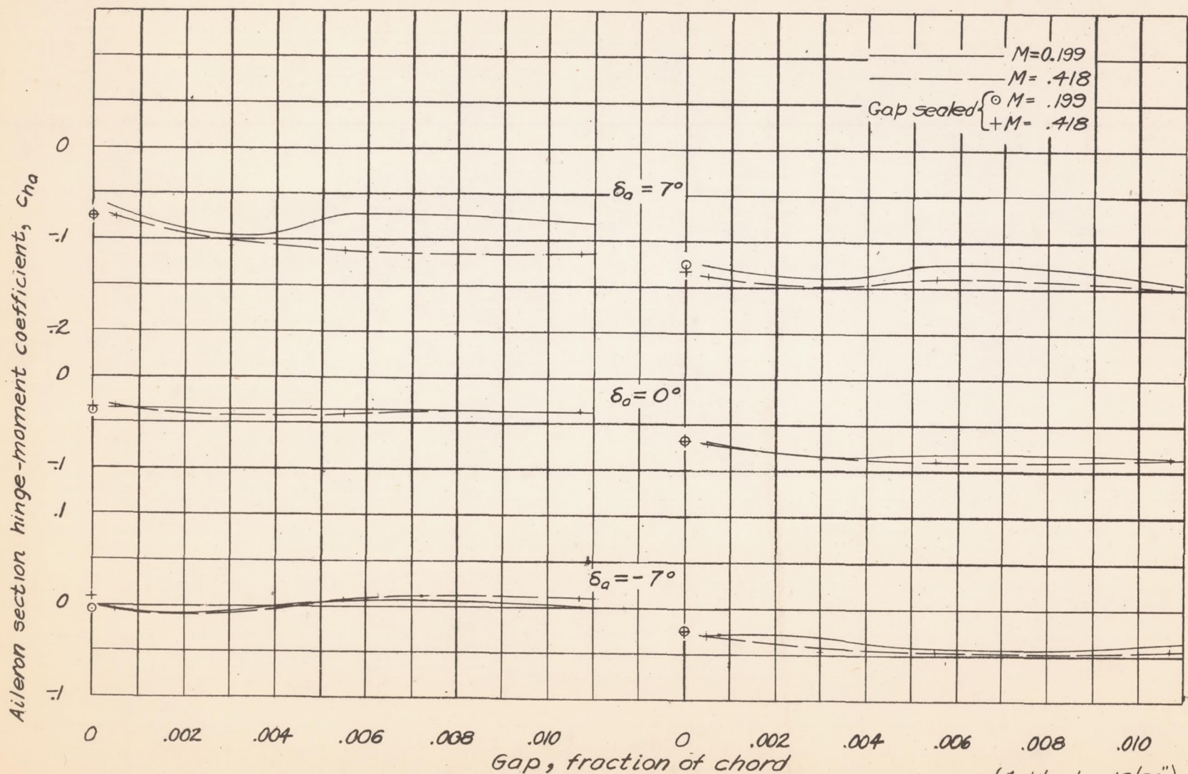
Figure 9.— Variation of aileron section hinge-moment coefficient with gap.
