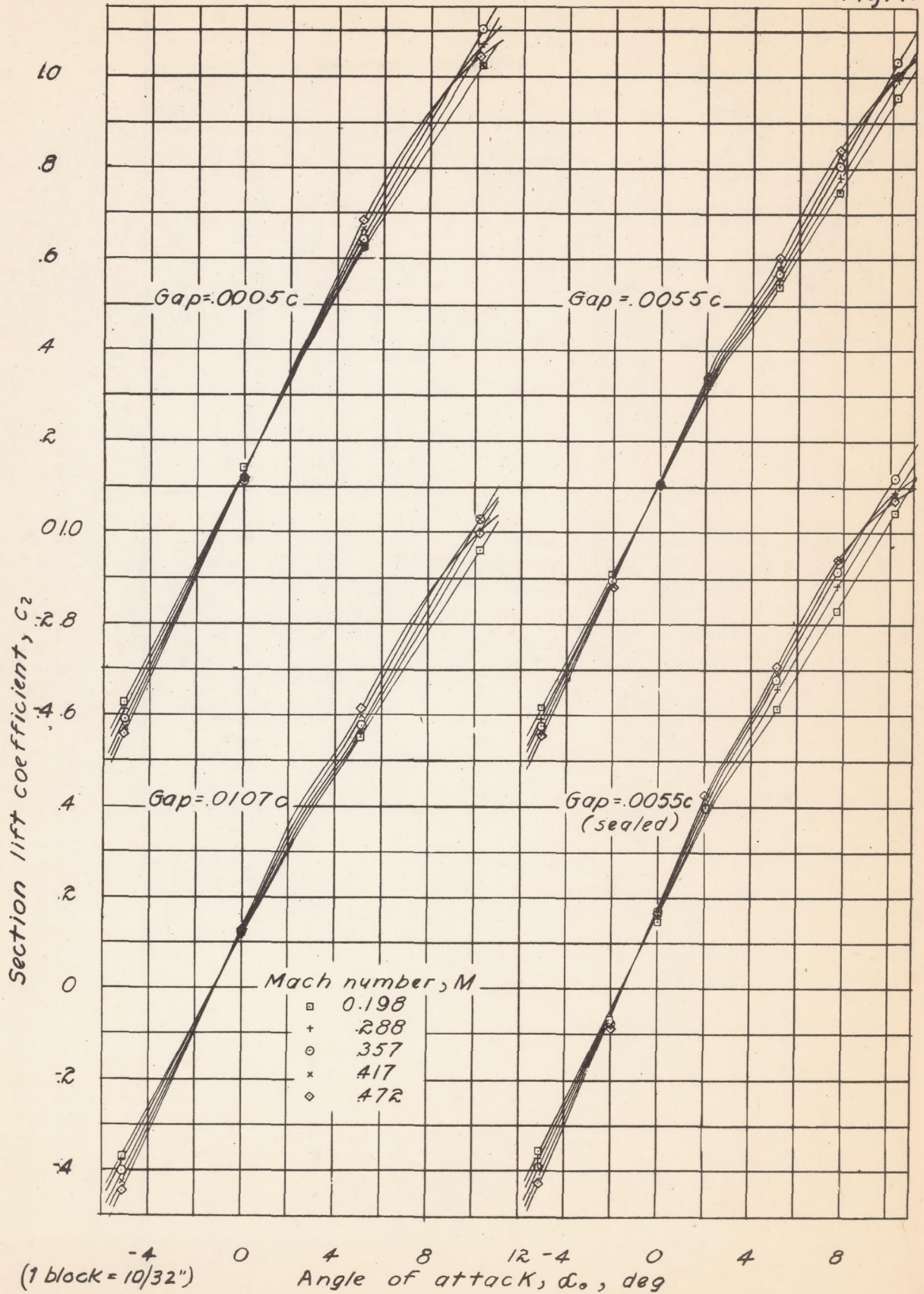
Figure 11.— Variation of section lift coefficient with angle of attack. Balance-nose radii = 0.02c ; \delta_0 = 0^\circ .
