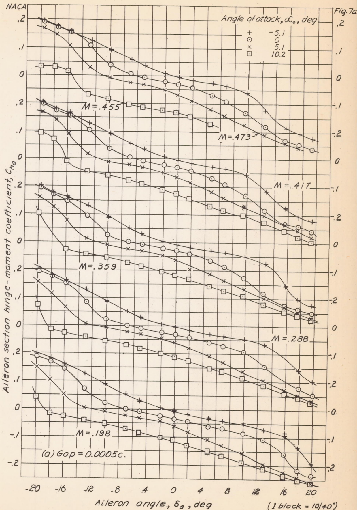
Figure 7. — Variation of aileron section hinge-moment coefficient with aileron angle. Balance-nose radii = 0.02c.
