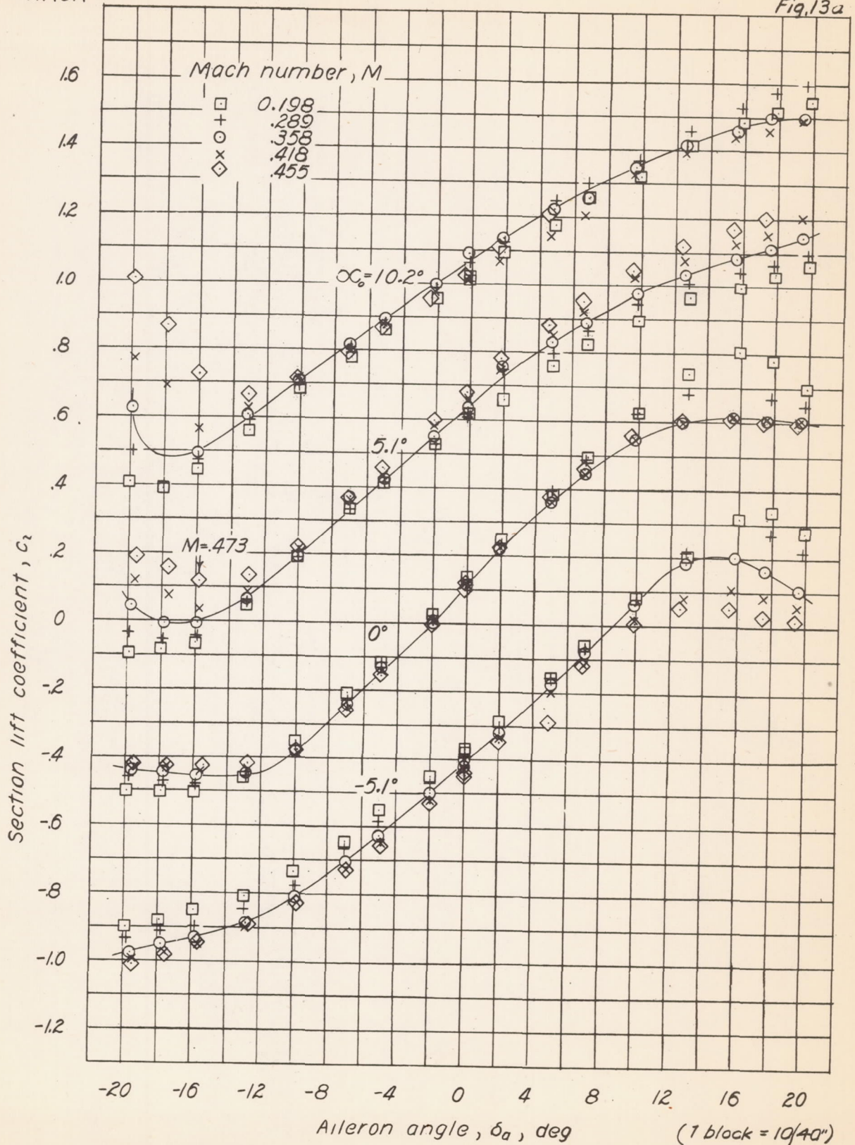
Figure 13. — Variation of section lift coefficient with aileron angle. Balance-nose radii = 0.02c.
