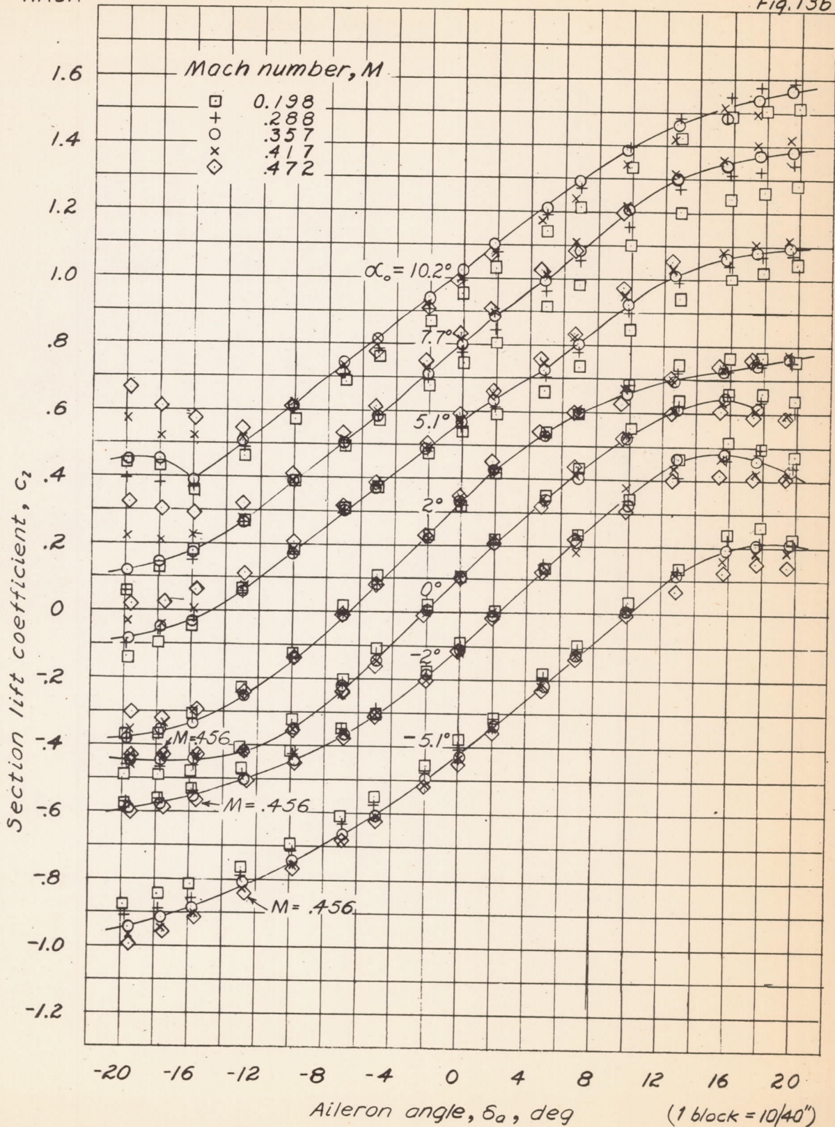
Figure 13. — Variation of section lift coefficient with aileron angle. Balance-nose radii = 0.02c. (Continued)
