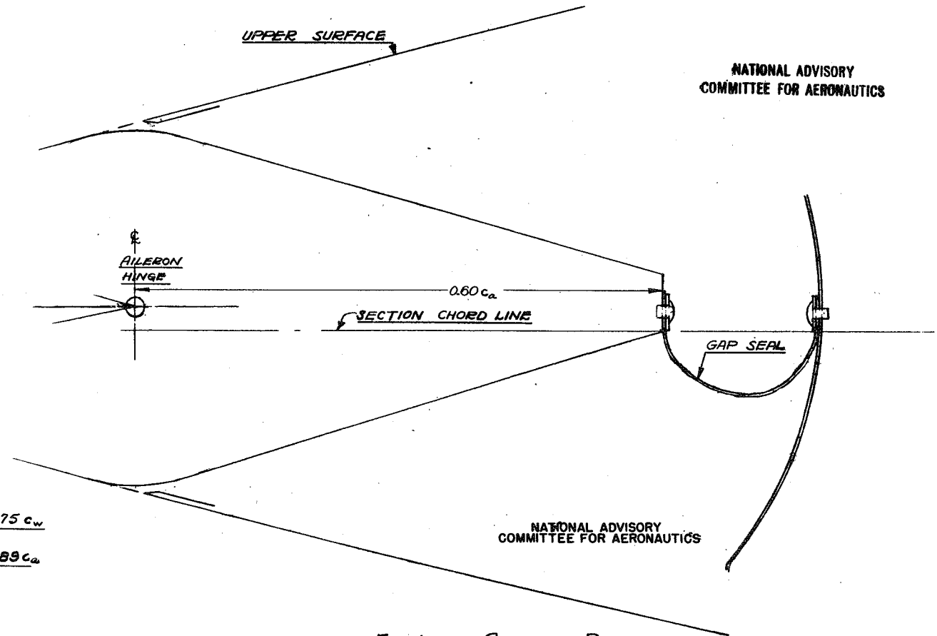
FIG. 1 AILERON BALANCE STA. 122 SCALE - FULL
