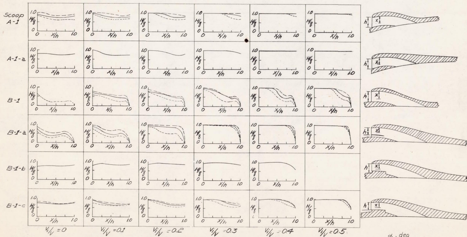
Figure 11.— Comparison of total pressures available in scoop entrances. (Measure with 60 ths scale)
