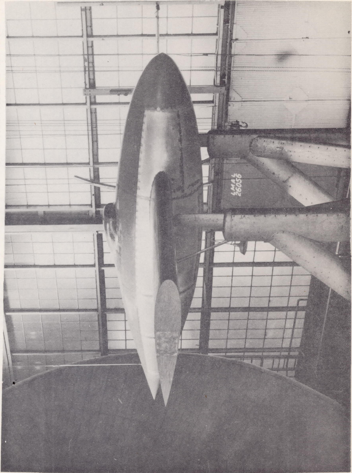
Figure 1.- Model with scoop B-1-c mounted in tunnel.
