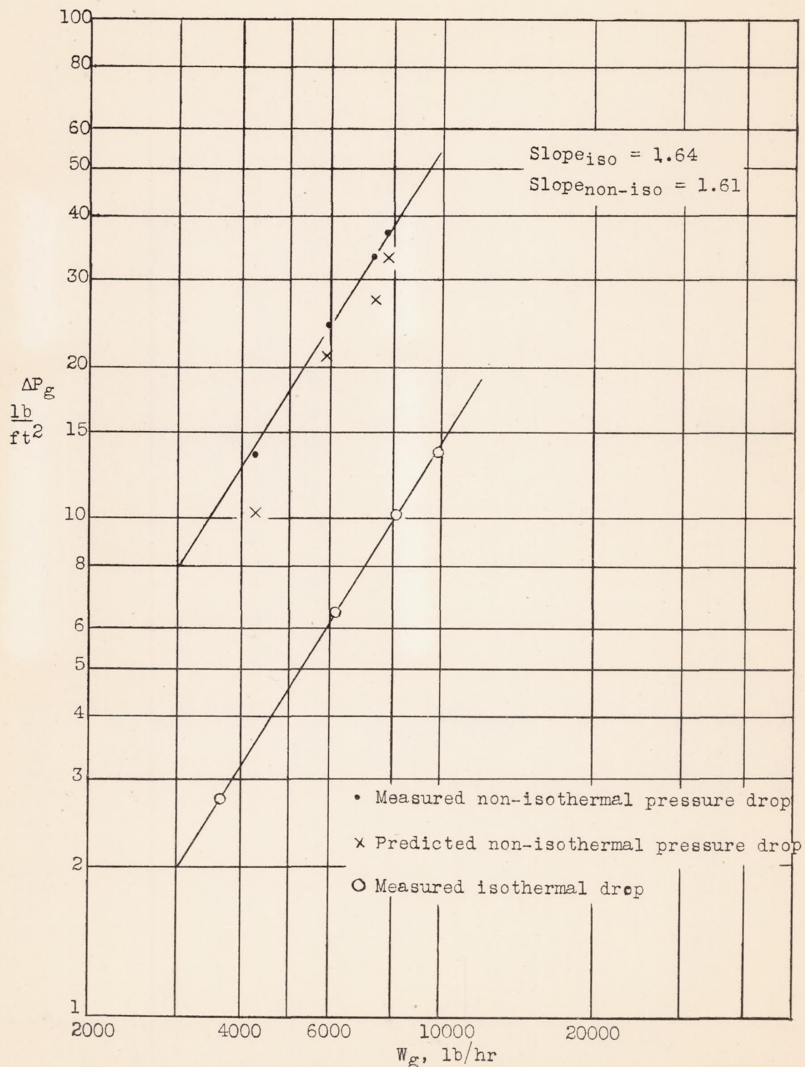
Figure 11.- Pressure drop on exhaust-gas side of Airesearch No. 2 heater as a function of exhaust-gas rate,
