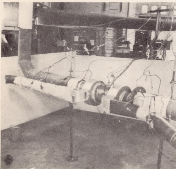
Figure 4.- Photograph of heater in test stand with air-shroud headers in normal position.
