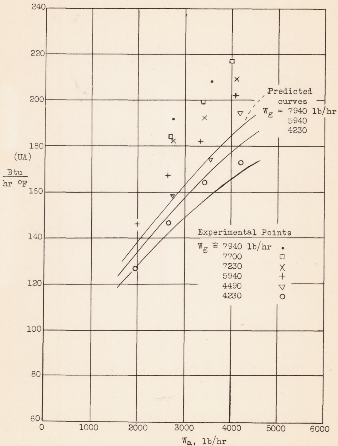
Figure 8.- Overall conductance of Airesearch No. 2 fluted-type heater as a function of ventilating-air rate.
