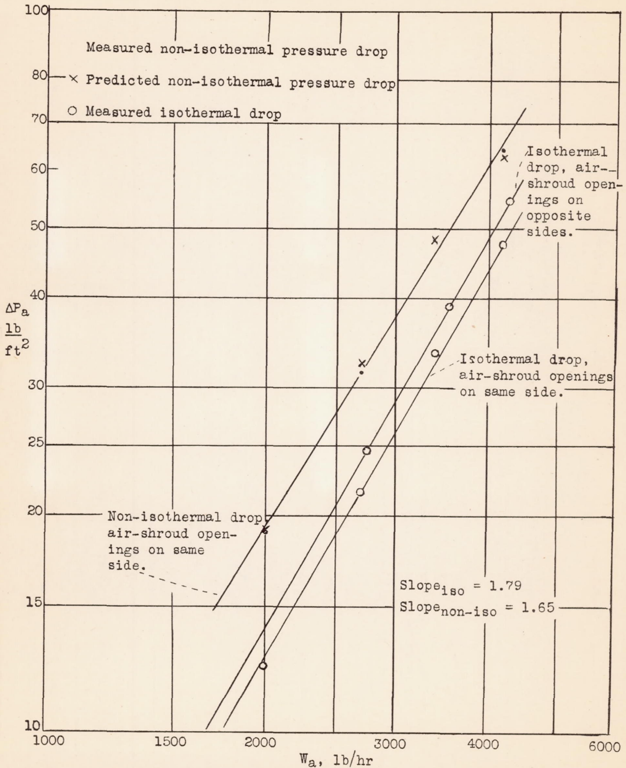
Figure 9.-- Pressure drop on air side of Airesearch No. 2 heater as a function of ventilating-air rate.
