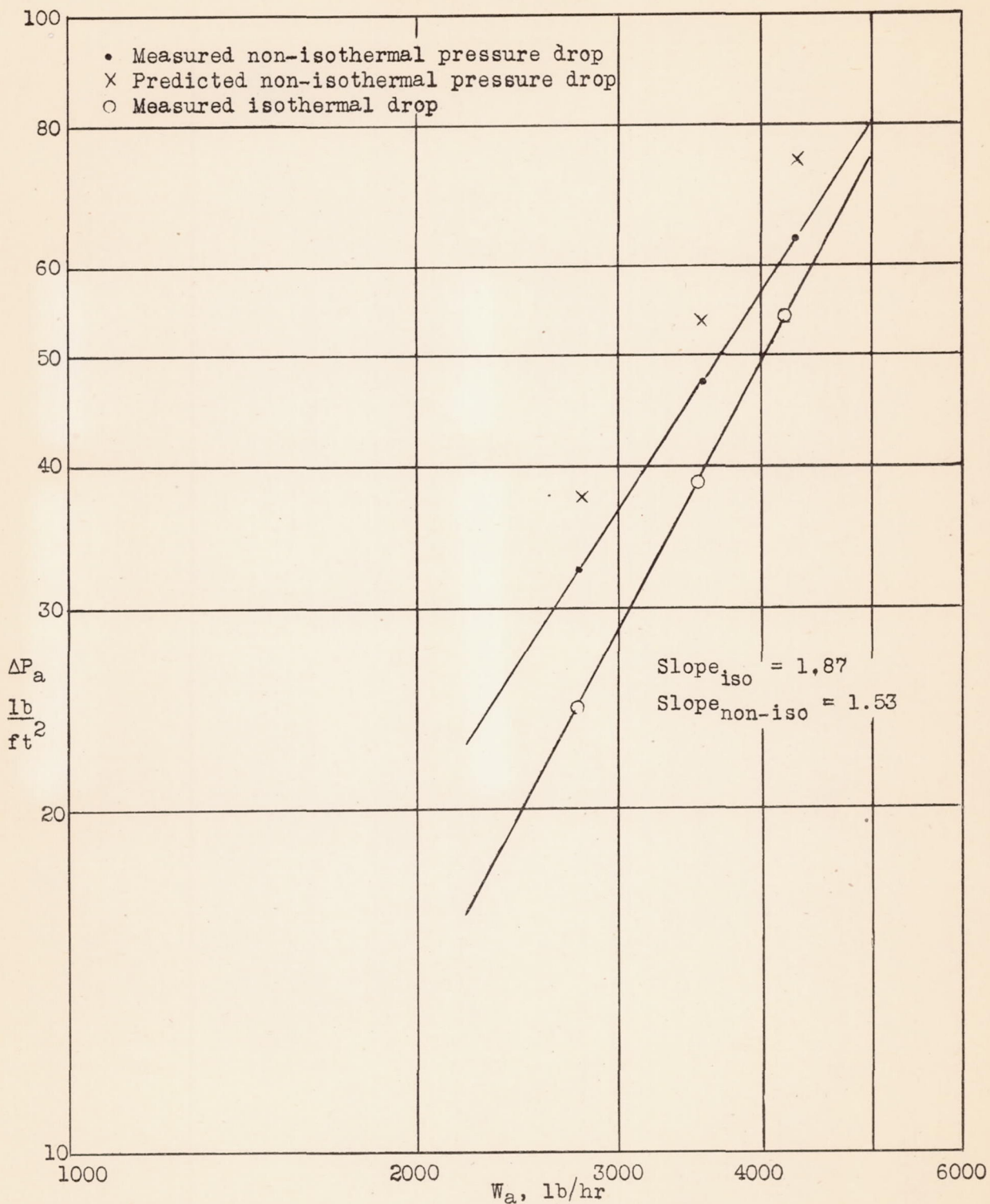
Figure 10.- Pressure drop on air side of Airesearch No. 2 heater as a function of ventilating-air rate. (Air-shroud openings on opposite sides.)
