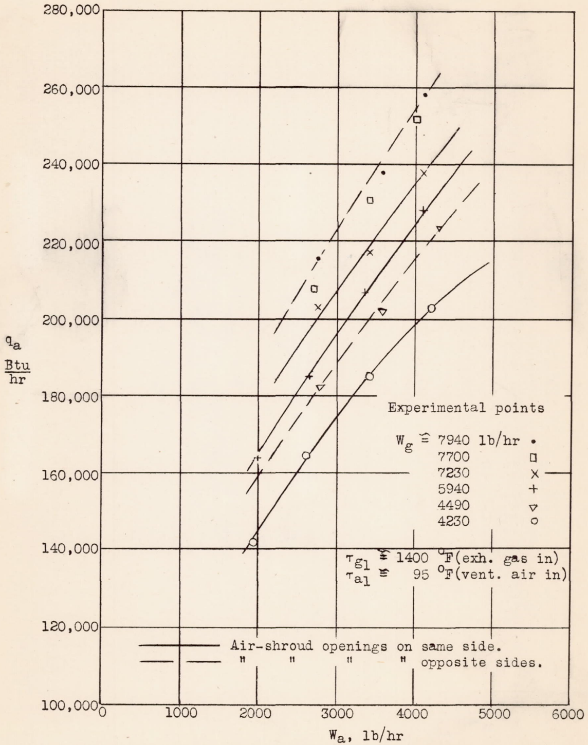
Figure 7.- Thermal output of Airesearch No.2 fluted-type heater as a function of ventilating-air rate.
