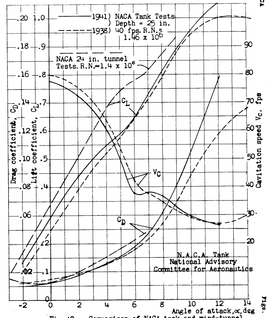
Fig. 19 .- Comparison of NACA tank and wind-tunnel tests on 16-509 section foil.
