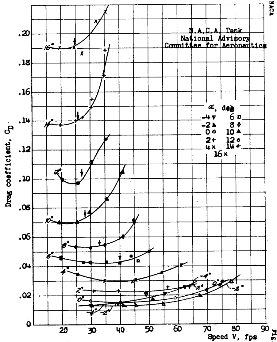
Fig.15 .- NACA 16-509 section hydrofoil. 30^\circ dihedral. Depth, 16.3 inches to 3/4 at tips.
