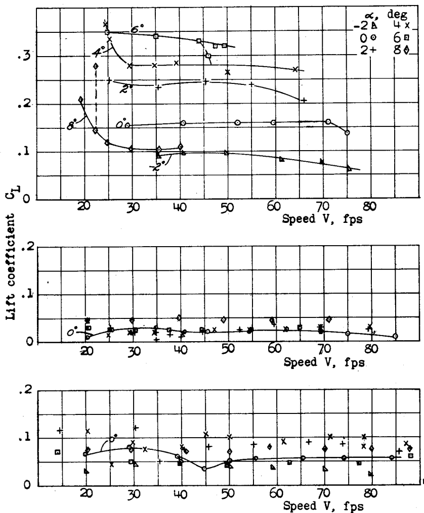
Fig. 8 .- NACA 16-509 section hydrofoil. 20° dihedral. Depths, c/4 at tips above water line, .46, 2.7, and 3.7 inches.
