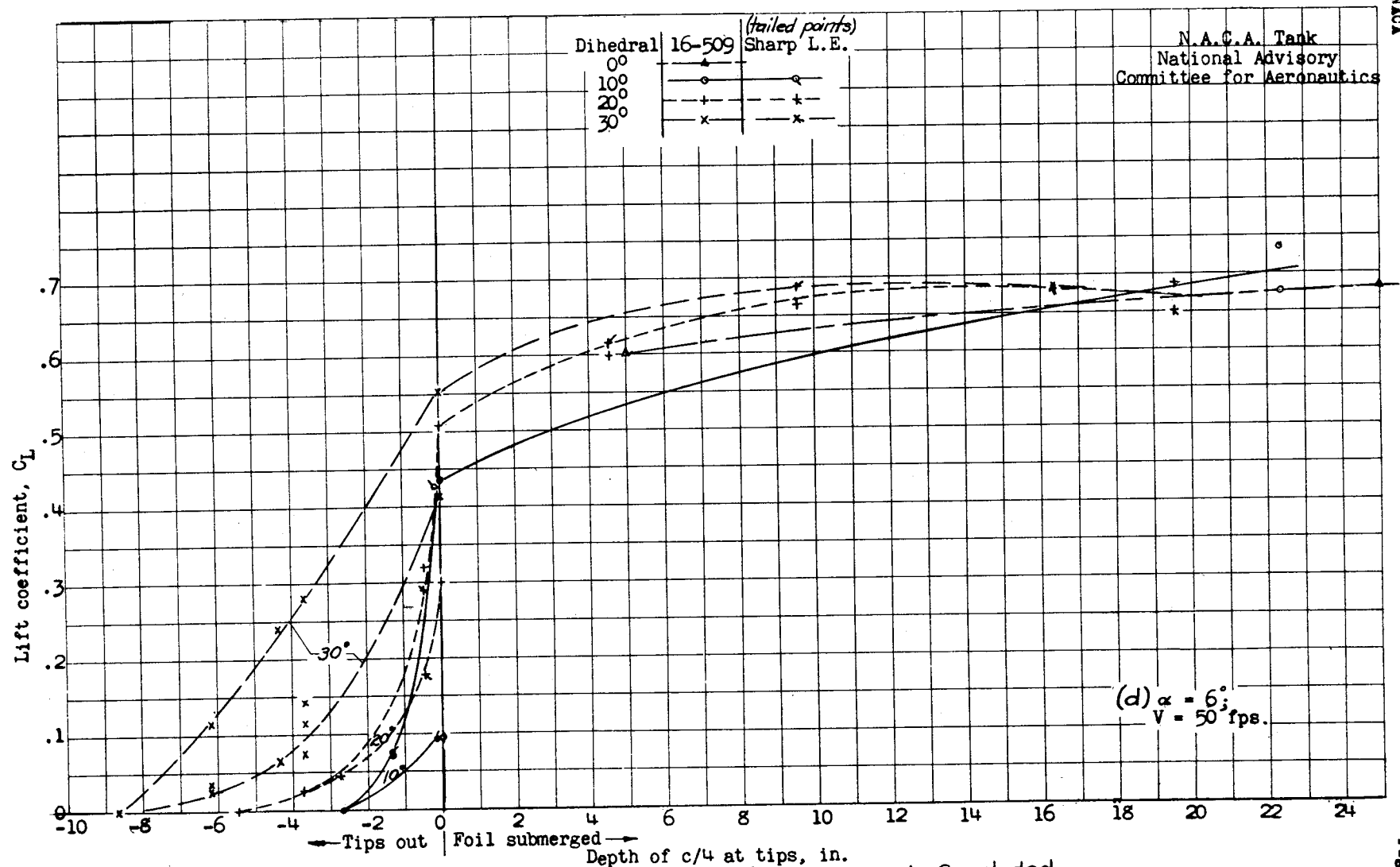
Fig. 16d.- Effect of depth on lift coefficient. Concluded.
