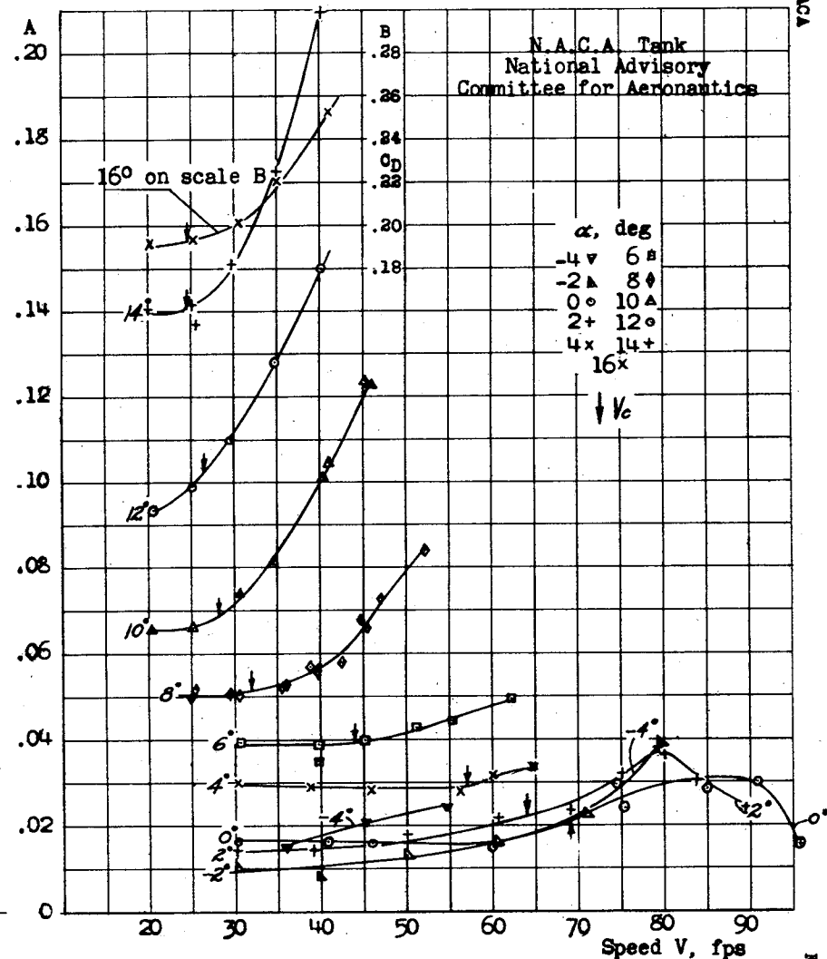
Fig. 12.- NACA 16-509 section hydrofoil. 20^\circ dihedral. Depth 19.5 inches to c/4 at tips.
