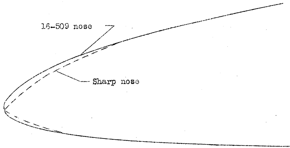
Enlarged nose sections
