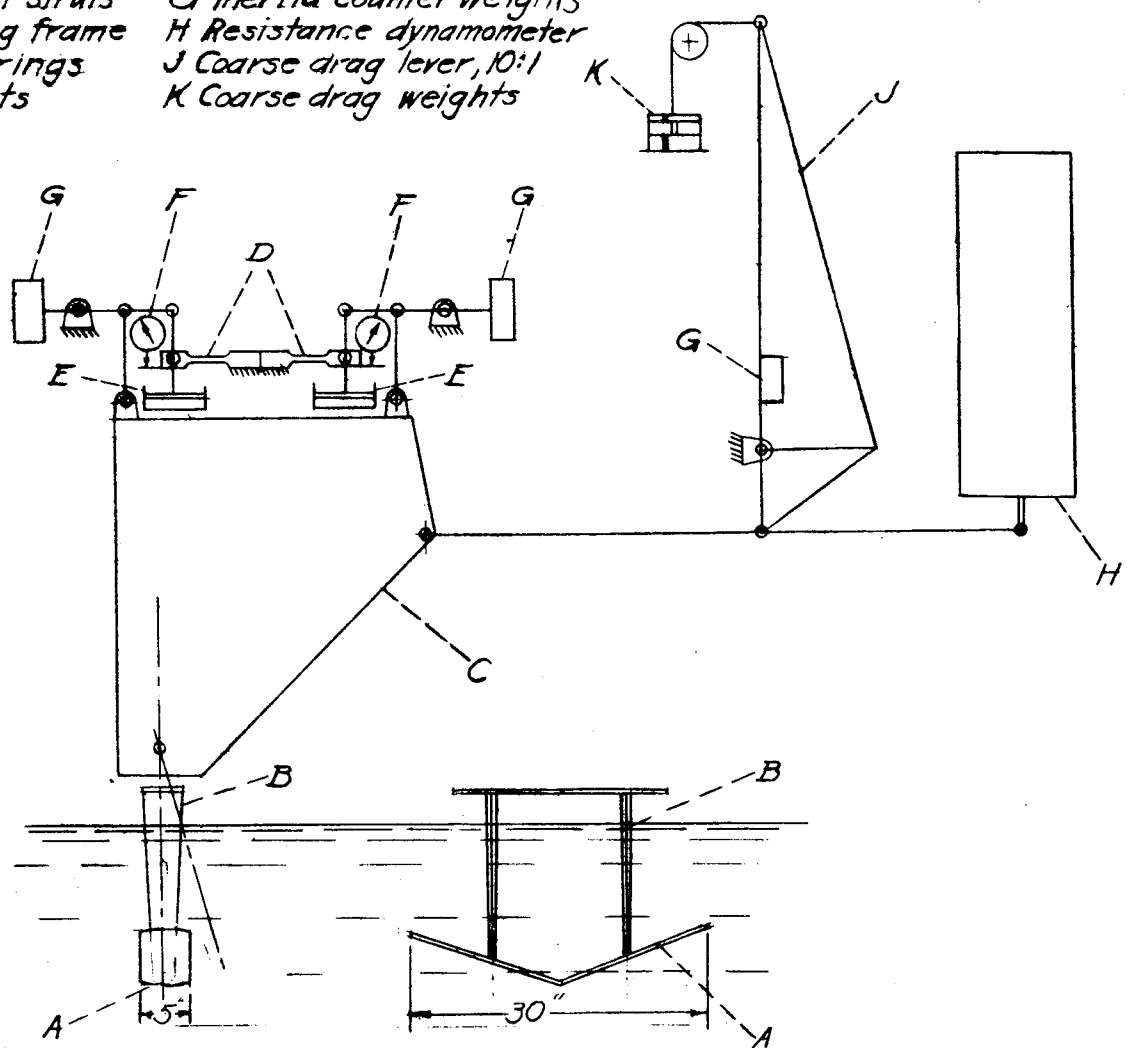
Fig. 2. — Diagrammatic sketch of hydrofoil dynamometer.
