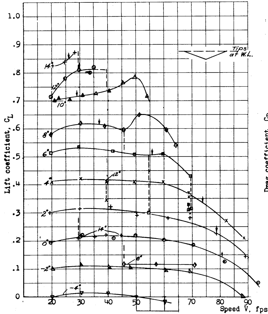
Fig. 9 .- 16-509 section hydrofoil. 20° dihedral. c/4 tips at water line.
