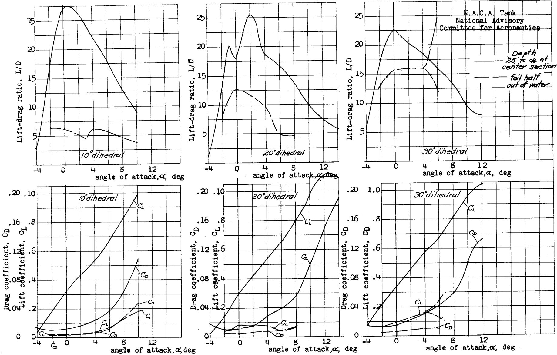
Fig. 20.- Characteristics of 16-509 section hydrofoils with dihedral angles of 10, 20, and 30 degrees at two depths. V = 40 fps DWH
