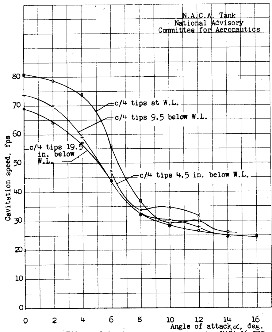
Fig. 17 .- Effect of depth on cavitation speed. NACA 16-509 section hydrofoil. 20^\circ dihedral.
