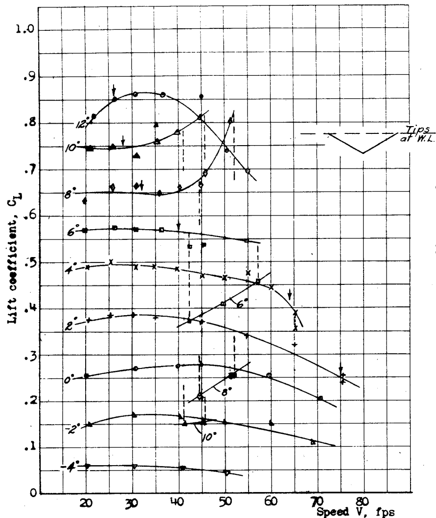
Fig.14 .- NACA 16-509 section hydrofoil. 30^\circ dihedral. Depths c/4 at tips at water line.
