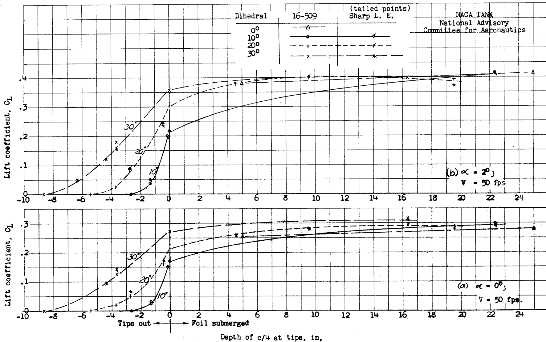
Fig. 16a,b.—Effect of depth on lift coefficient.
