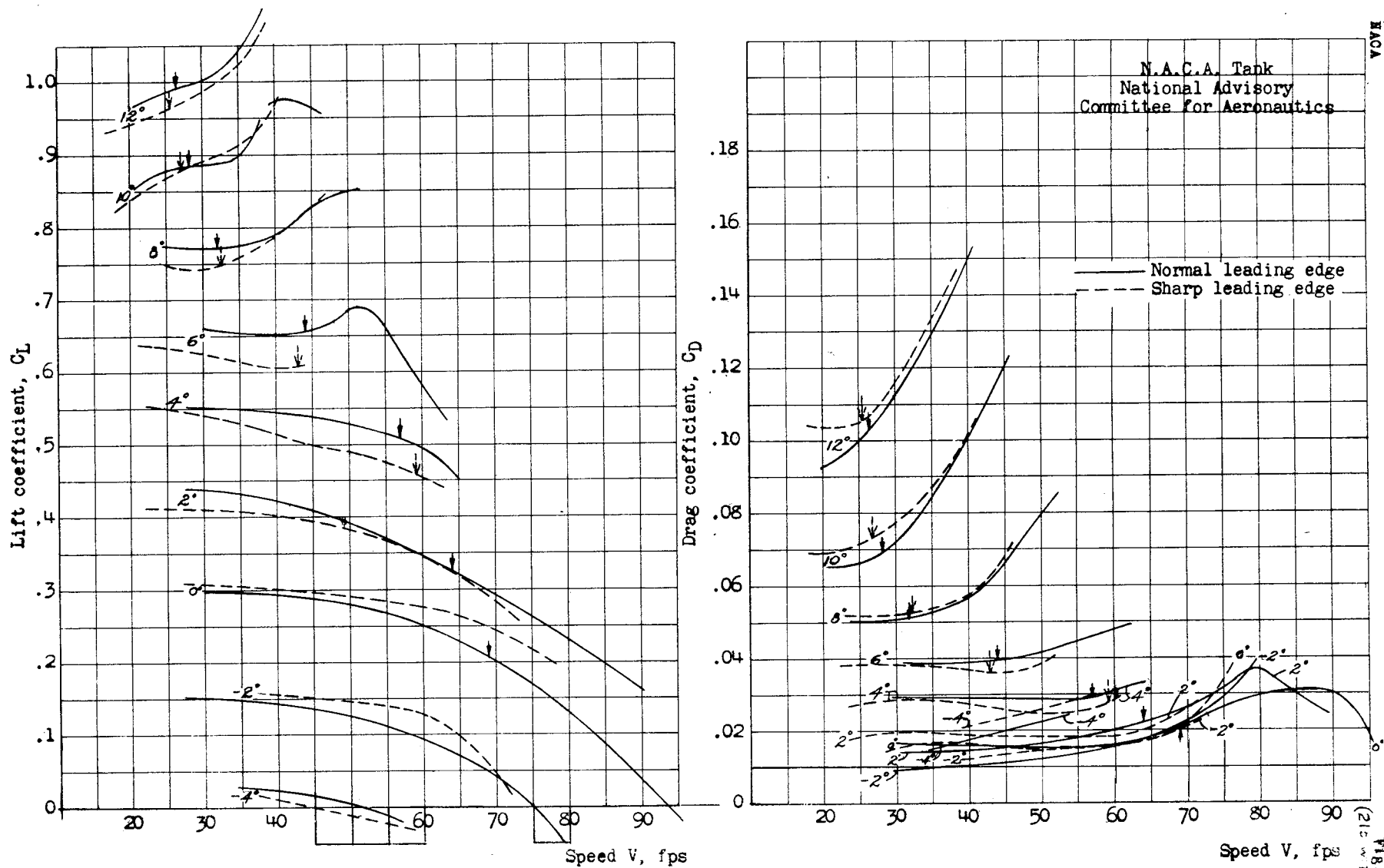
Fig. 21a. - Comparison of test results on normal and sharp leading edge hydrofoils. 20^\circ dihedral. Depth, 19.5 inches to c/4 at tips.
