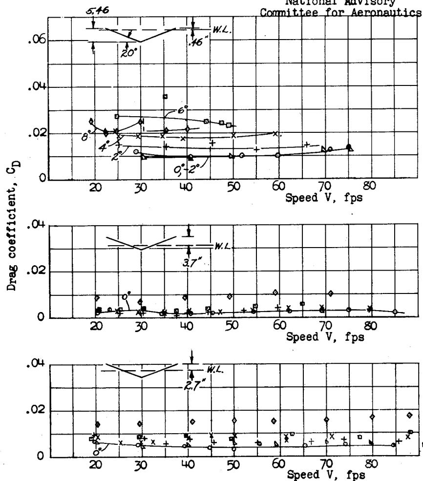
Fig. 8 .- NACA 16-509 section hydrofoil. 20° dihedral. Depths, c/4 at tips above water line, .46, 2.7, and 3.7 inches.
