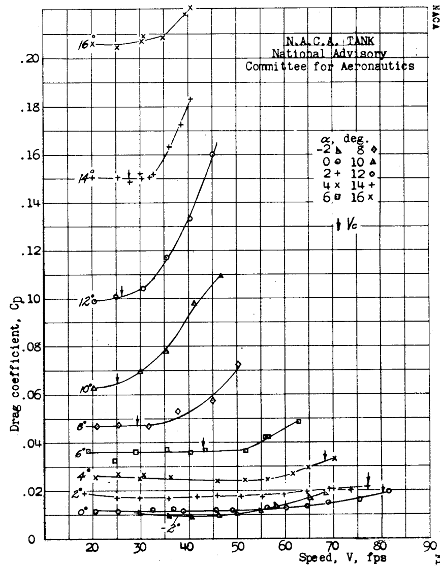
Fig. 4.- NACA 16-509 section hydrofoil. 0^\circ dihedral. Depth, 5 inches to c/4 .
