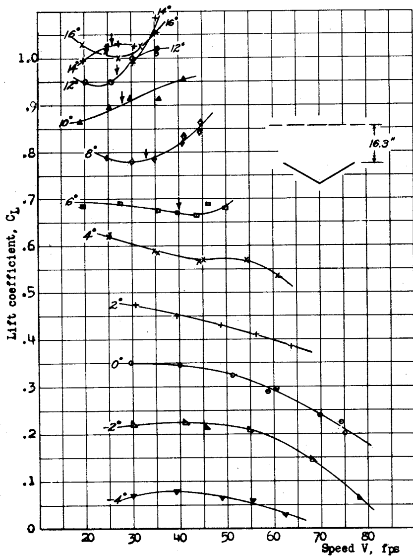
Fig.15 .- NACA 16-509 section hydrofoil. 30^\circ dihedral. Depth, 16.3 inches to 3/4 at tips.
