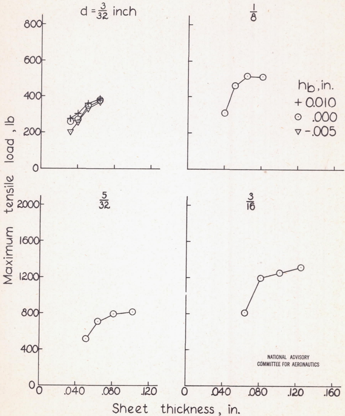
Figure 9.-Variation of maximum tensile load with sheet thickness for conventional machine-countersunk flush rivets; rivet-head angle = 100°
