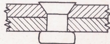
(b) Conventional countersunk rivet.
