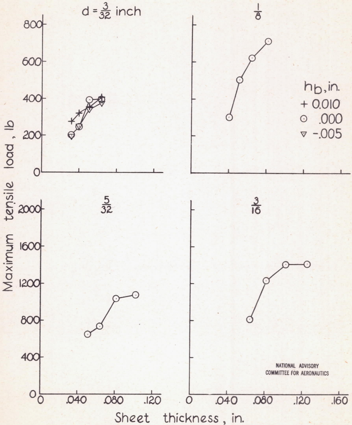
Figure 8.-Variation of maximum tensile load with sheet thickness for conventional machine-countersunk flush rivets; rivet-head angle = 78°.
