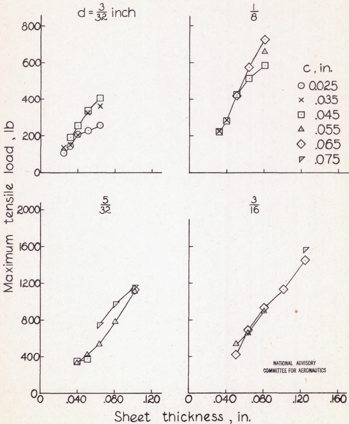
Figure 5. - Variation of maximum tensile load with sheet thickness for NACA machine-countersunk flush rivets ; rivet-head angle = 60°
