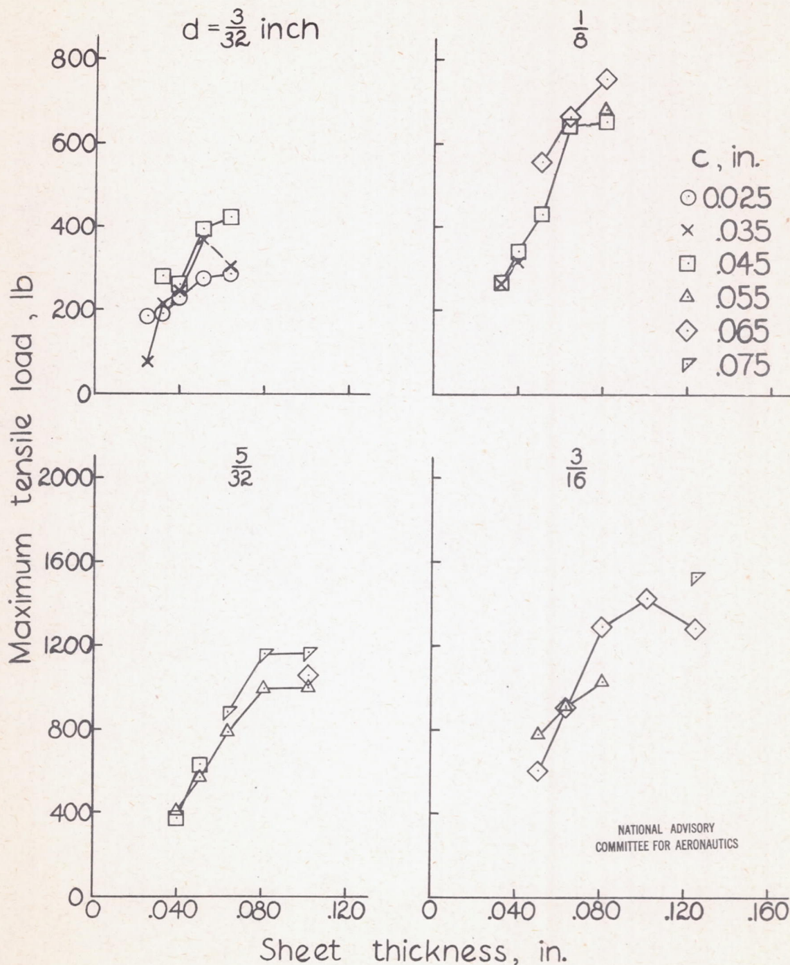
Figure 6.-Variation of maximum tensile load with sheet thickness for NACA machine-countersunk flush rivets ; rivet-head angle = 82°.
