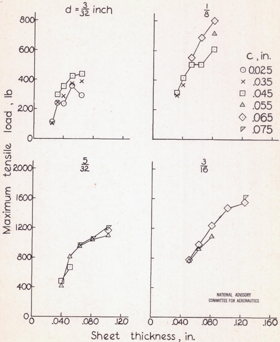
Figure 7.-Variation of maximum tensile load with sheet thickness for NACA machine-countersunk flush rivets ; rivet-head angle = 100°.
