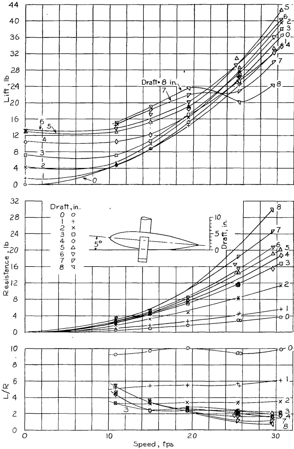
Figure 6.- Lift and resistance characteristics of streamline body with hydrofoil. \tau = 5^\circ .
