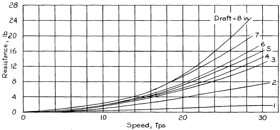
Figure 8.- Effective lift and resistance characteristics of streamline body. \tau = 5^\circ .
