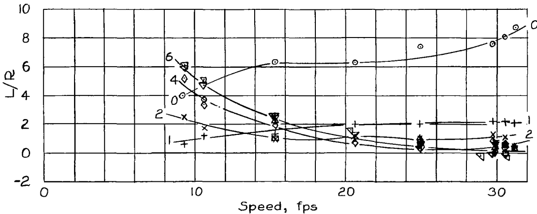
Figure 5.- Lift and resistance characteristics of streamline body with hydrofoil. \tau = 0^\circ .
