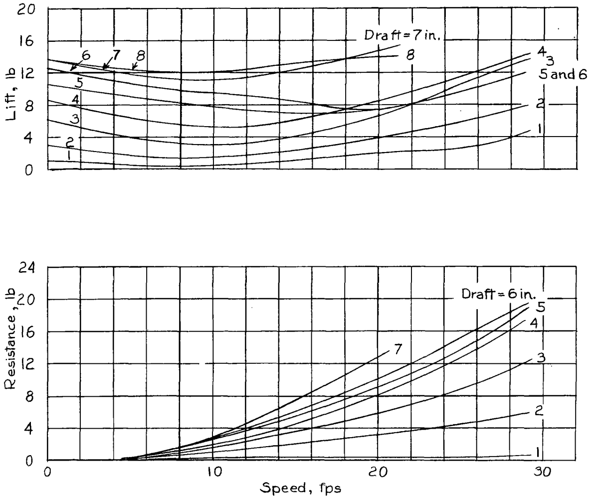
Figure 9.- Effective lift and resistance characteristics of streamline body. \tau = 10^\circ .
