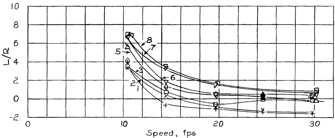
Figure 4.- Lift and resistance characteristics of streamline body. \tau = 10^\circ .
