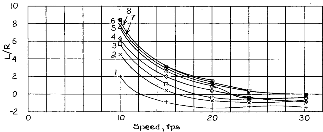
Figure 3.- Lift and resistance characteristics of streamline body. \tau = 5^\circ .
