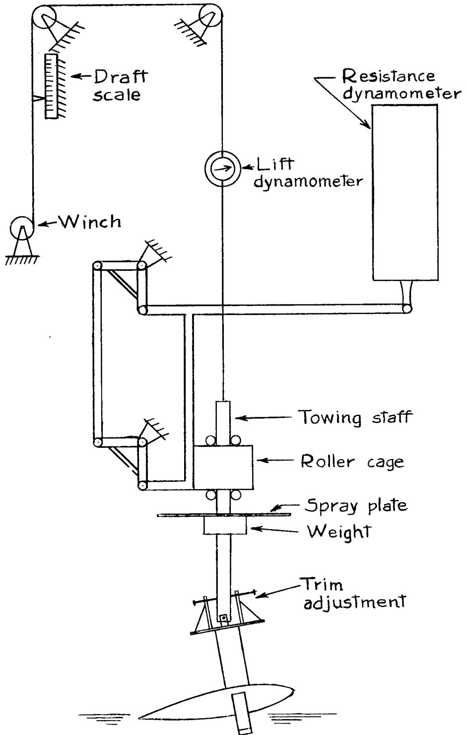
Figure 2.- Diagrammatic sketch of towing gear.
