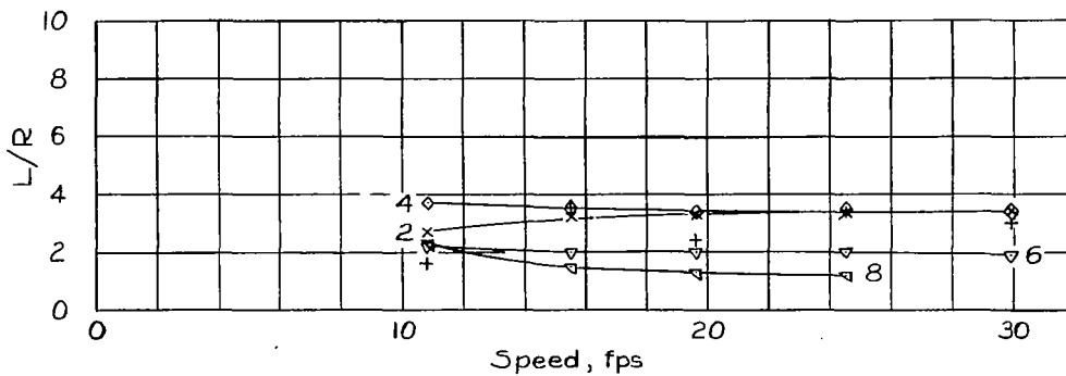
Figure 10.- Lift and resistance characteristics of \frac{1}{5} -size model of PBV-type outboard float, NACA model 104-A; trim = 13°. (Data taken from unpublished tests.)
