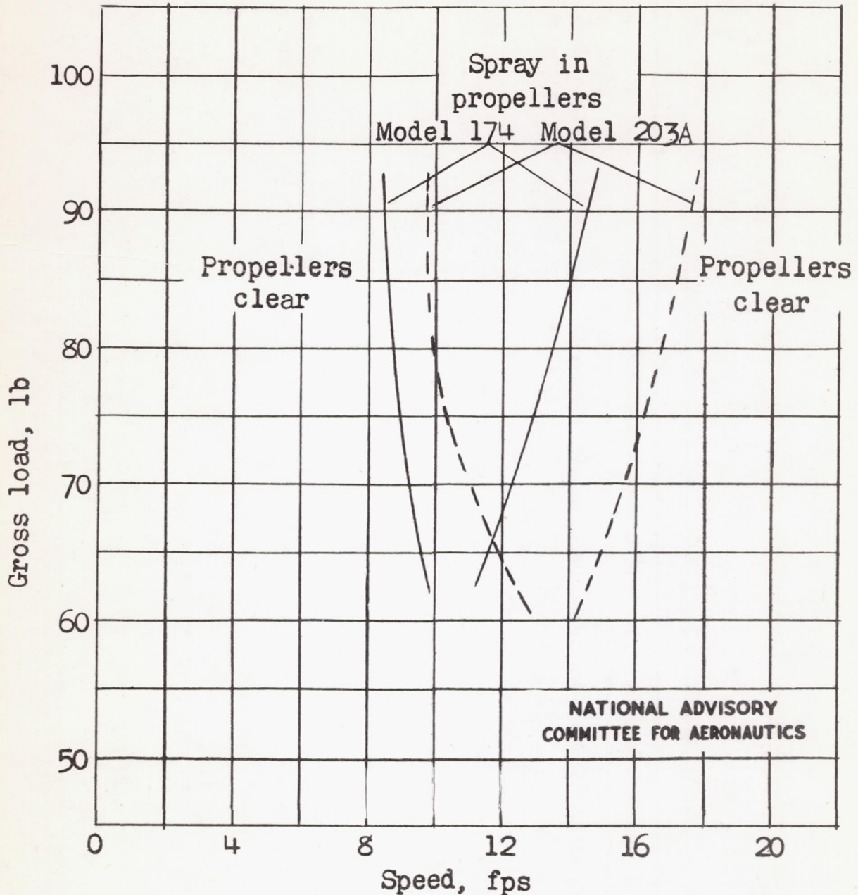
Figure 8 .- Model 174. Speed range over which spray enters propellers. Full power, 4,200 rpm; center of gravity, 28 percent M.A.C.; flap deflection, 20°; elevator deflection, -10°.
