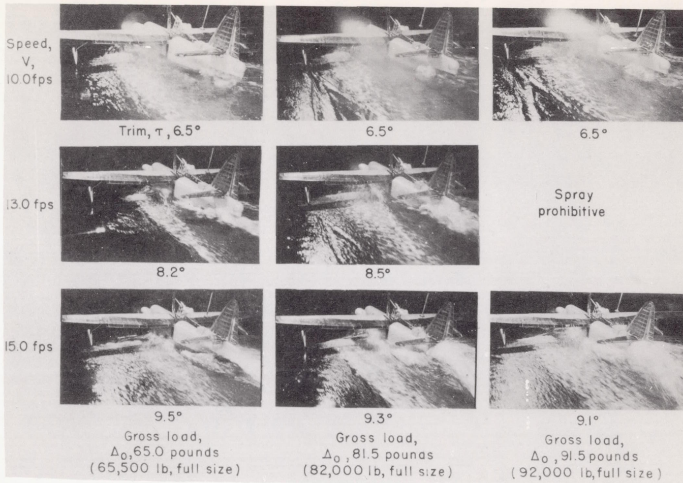
Figure 11.- Model 174. Spray characteristics, flap and tail assembly. Full power, 4,200 rpm; center of gravity, 28 percent M.A.C.; flap deflection, 20^\circ ; elevator deflection, -10^\circ .
