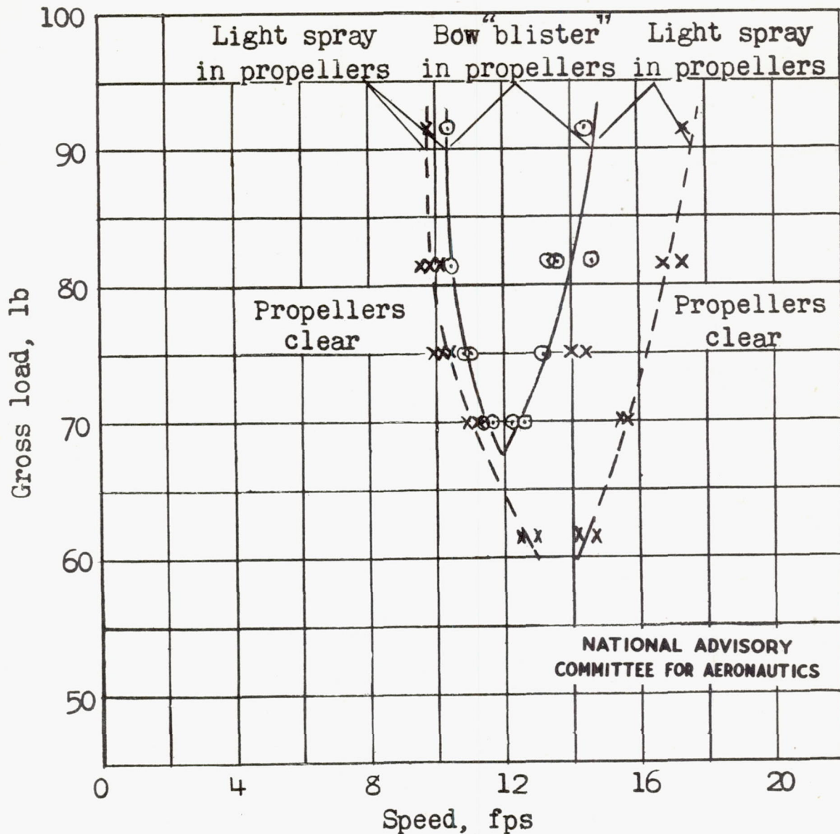
Figure 6 .- Model 203A. Speed range over which spray enters the propellers. Full power, 4,550 rpm; center of gravity, 28 percent M.A.C.; flap deflection, 20°; elevator deflection, -10°.
