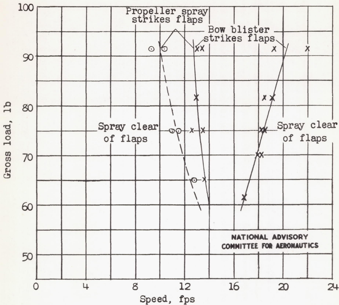
Figure 12.- Model 203A . Speed range over which spray strikes the flaps. Full power, 4,500 rpm; center of gravity, 28 percent M.A.C.; flap deflection, 20°; elevation deflection, -10°.
