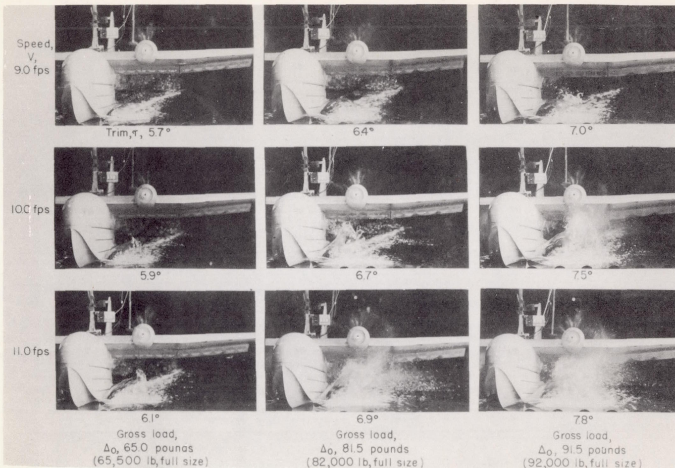
Figure 7.- Model 203A. Spray characteristics, bow. Full power, 4,550 rpm; center of gravity, 28 percent M.A.C.; flap deflection, 20°; elevator deflection, -10°.
