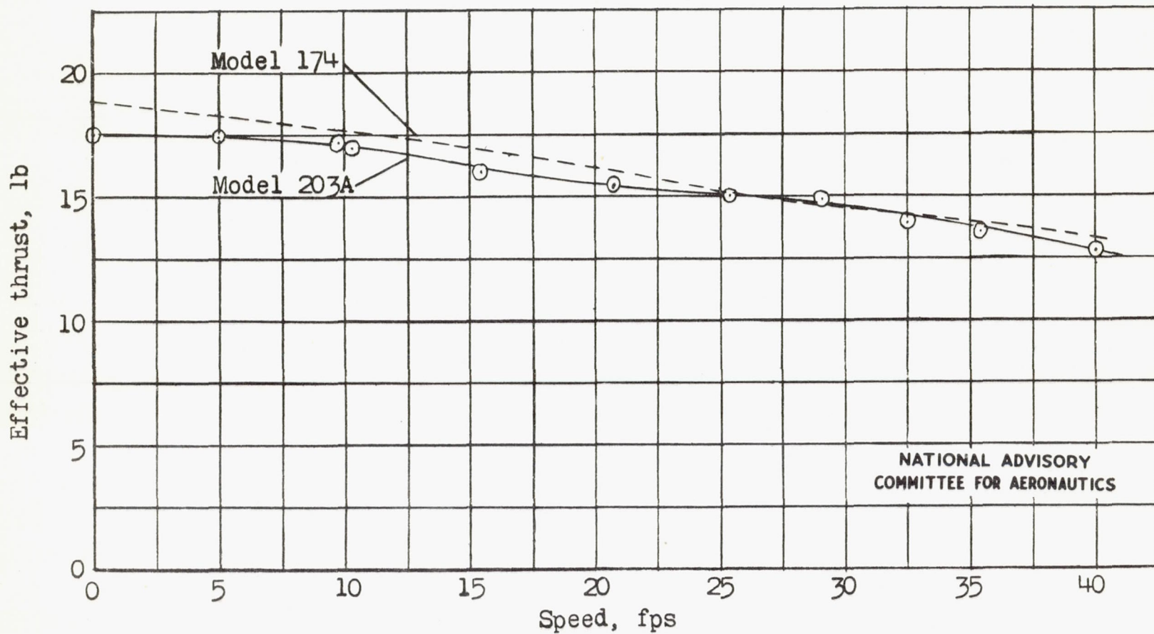
Figure 4 .- Model 203A. Variation of effective thrust with speed. Full power, 4,550 rpm; blade angle, 14^{\circ} ; flap deflection, 0^{\circ} ; trim, 0^{\circ} .
