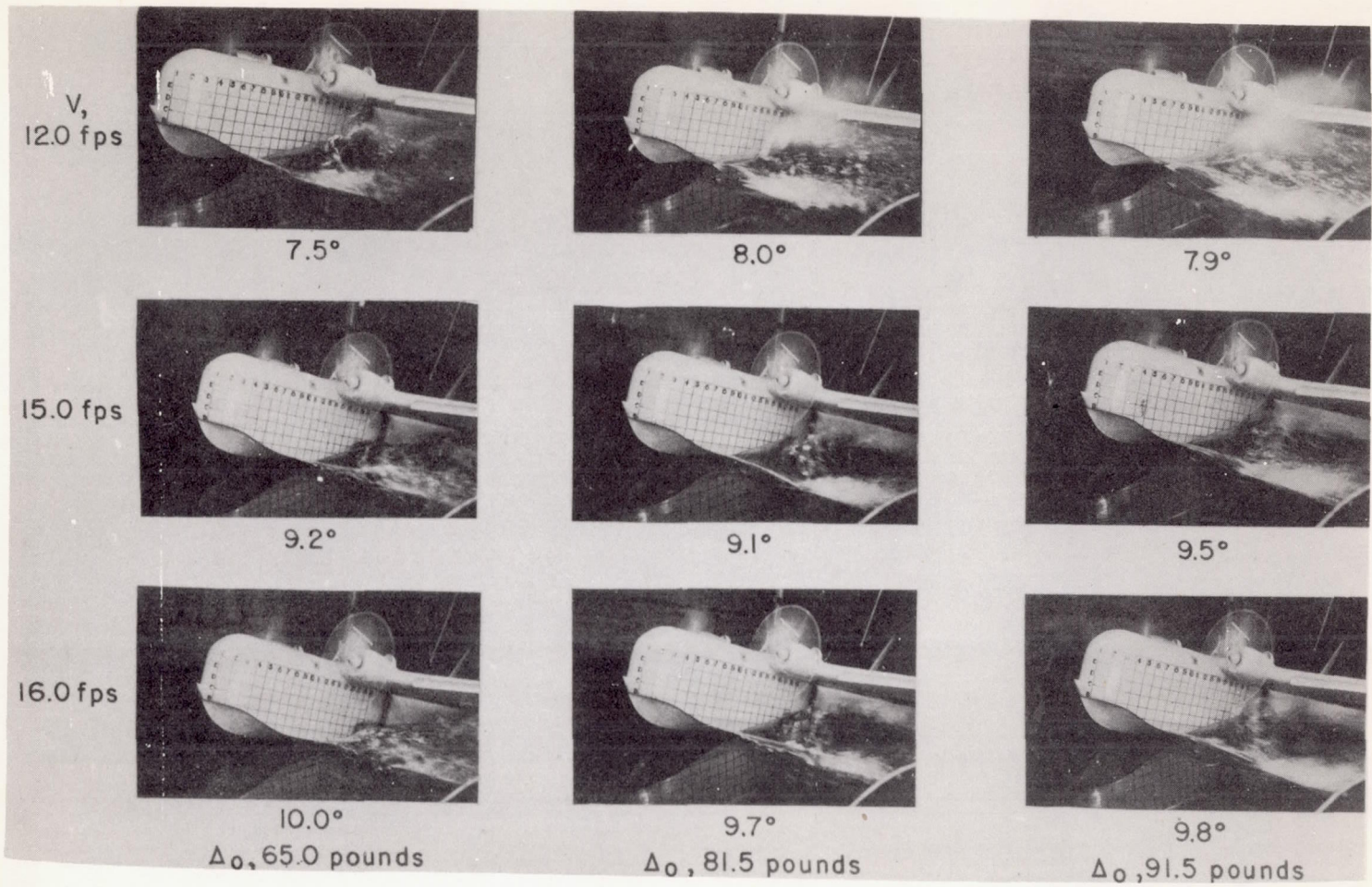
Figure 9.- Model 174. Concluded.
