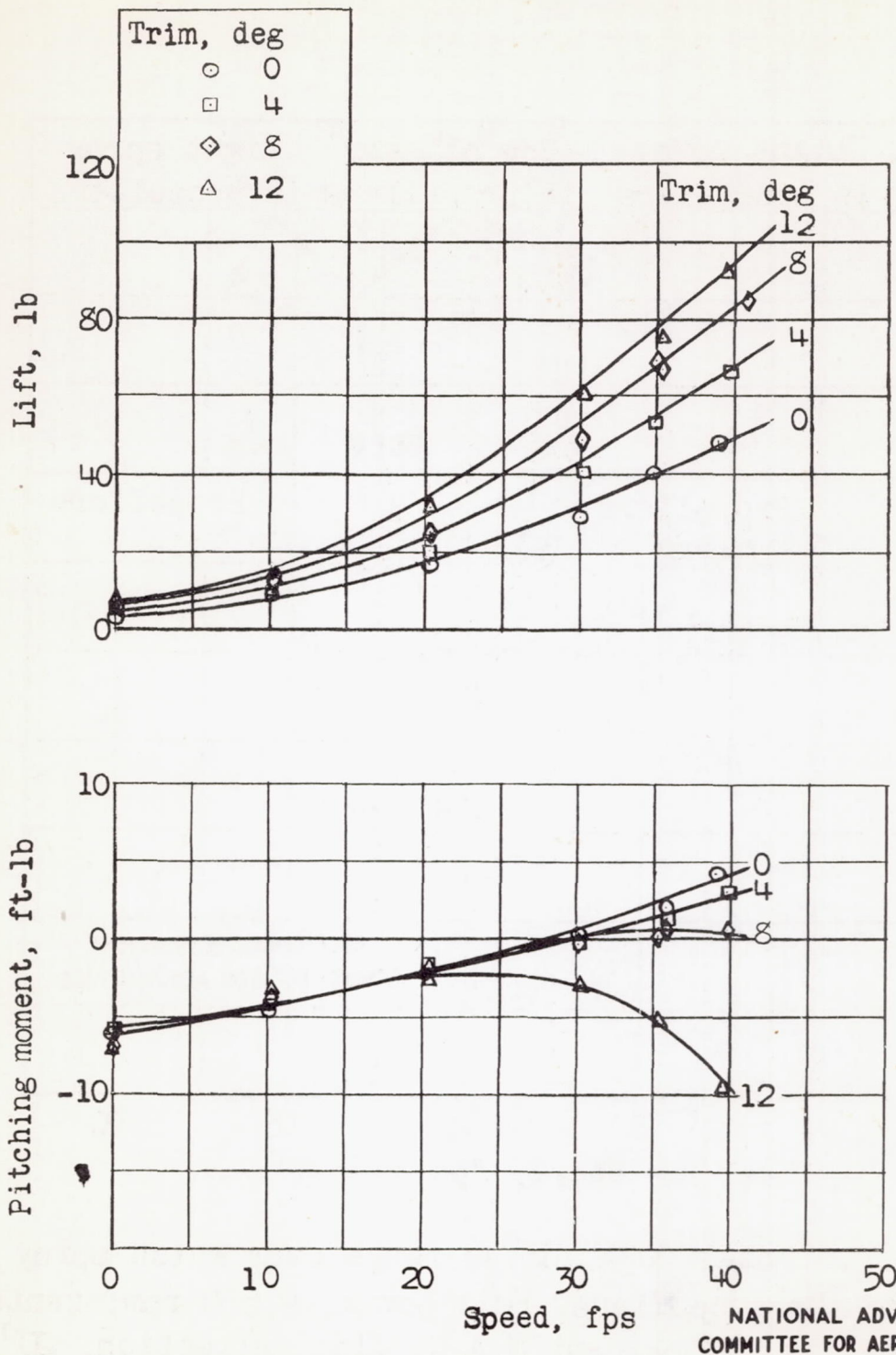
Figure 5 .- Model 203A. Variation in aerodynamic lift and pitching moment with speed. Full power, 4,550 rpm; center of gravity, 24 percent M.A.C.; flap deflection, 20^{\circ} ; elevator deflection, -10^{\circ} .
