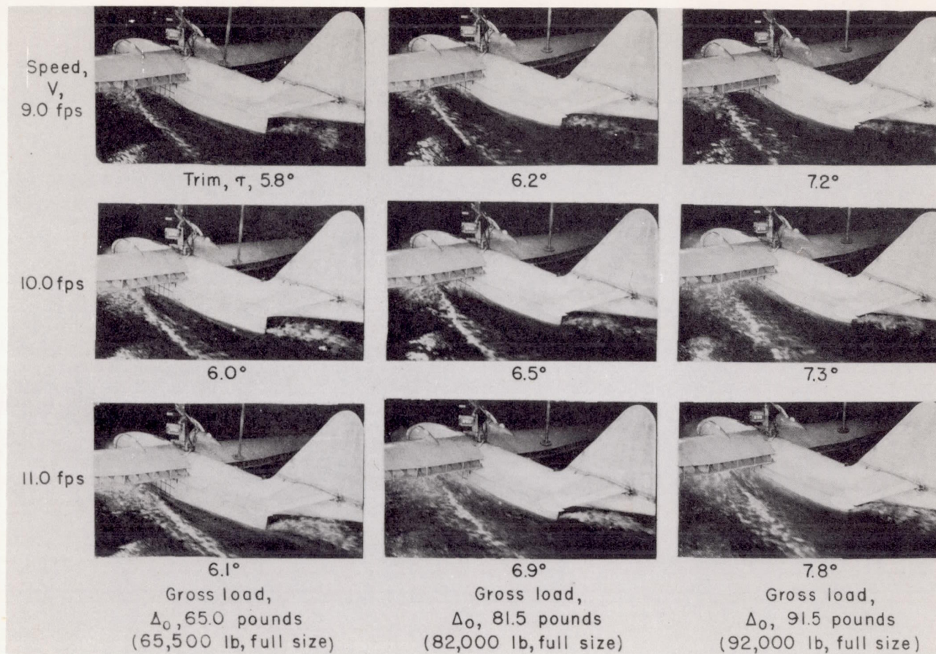
Figure 10.- Model 203A. Spray characteristics, flap and tail assembly. Full power, 4,550 rpm; center of gravity, 28 percent M.A.C.; flap deflection, 20°; elevator deflection, -10°.
