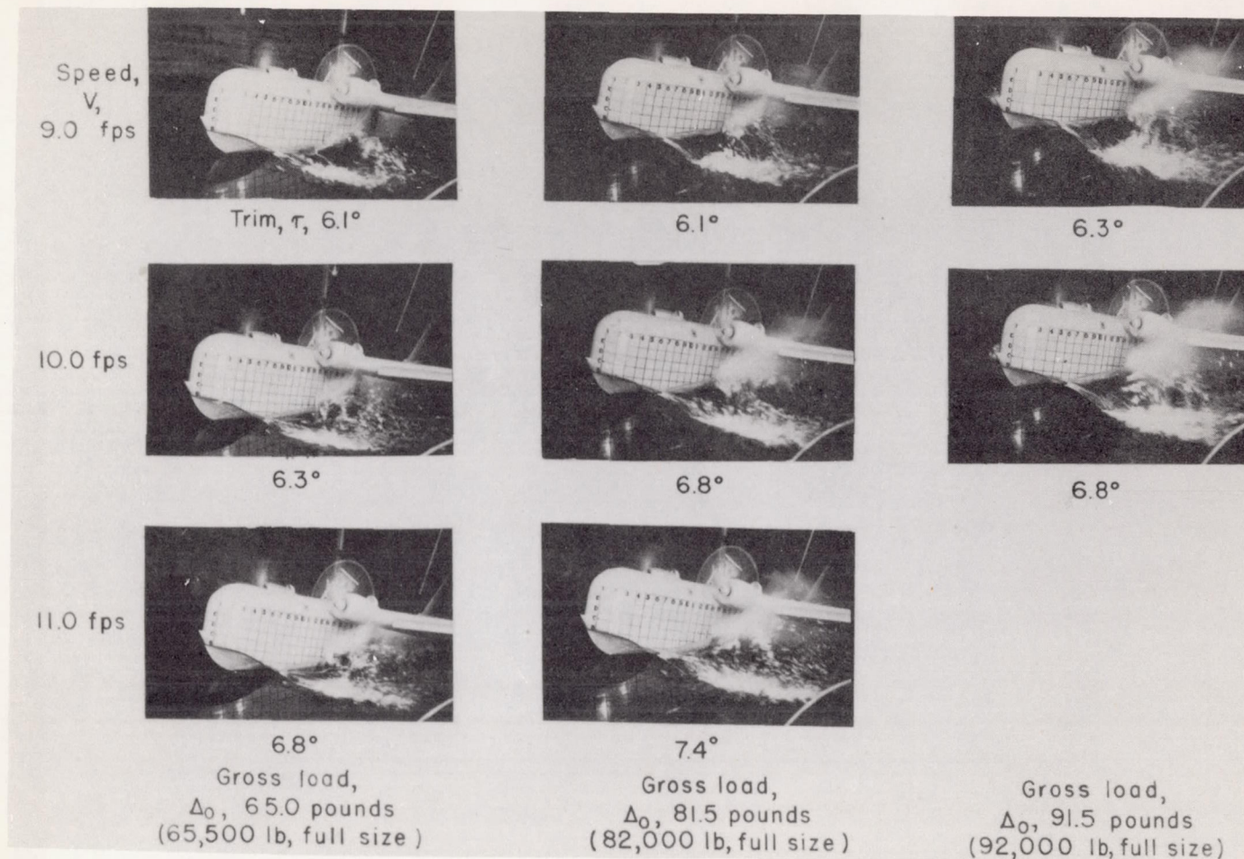
Figure 9.- Model 174. Spray characteristics, bow. Full power, 4,200 rpm; center of gravity, 28 percent M.A.C.; flap deflection, 20°; elevator deflection, -10°.
