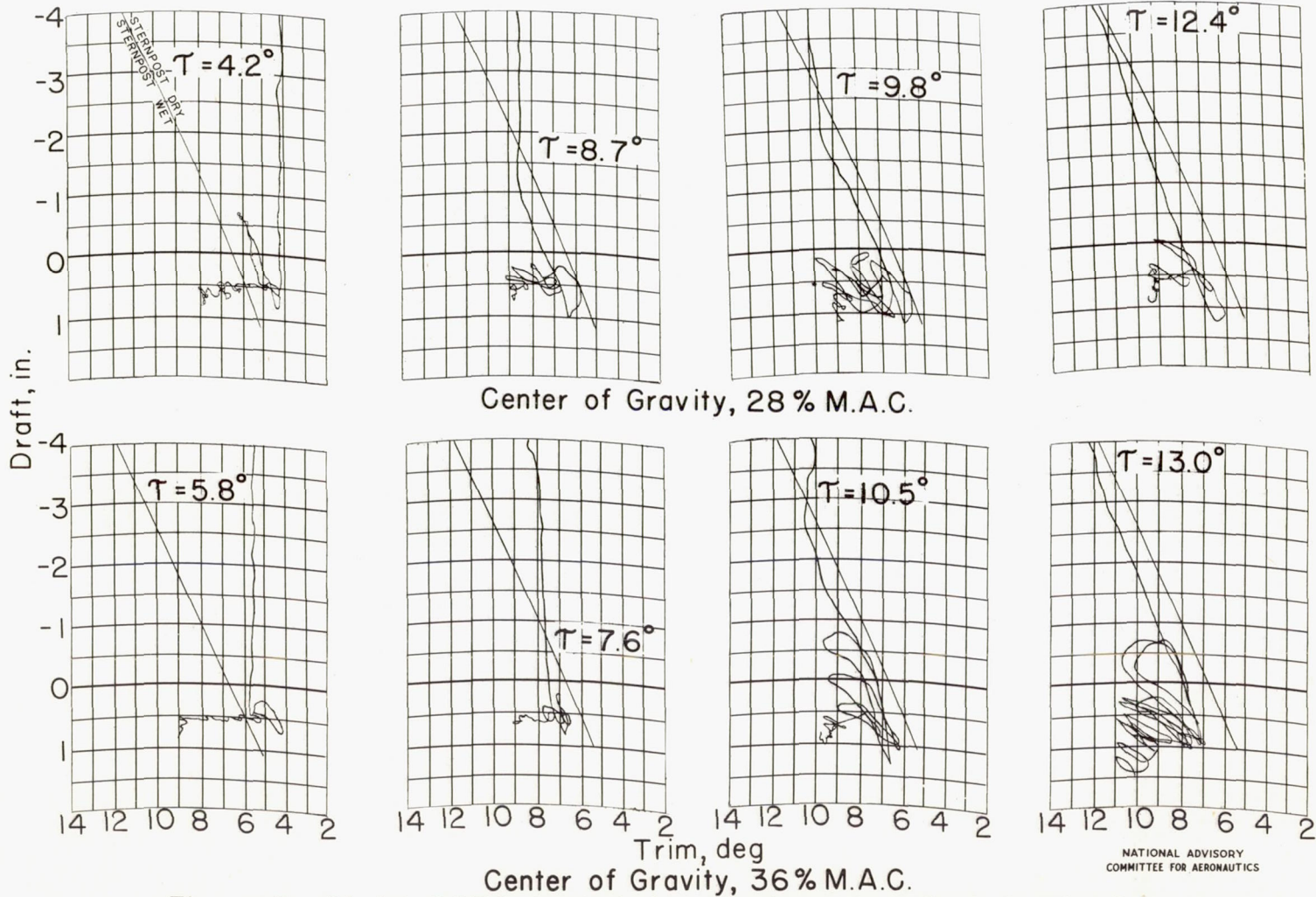
Figure 9.-Model 203C-I. Variation of trim and draft during landing. Gross load, 81.5 pounds; 1/4 power; flap deflection, 20°.
