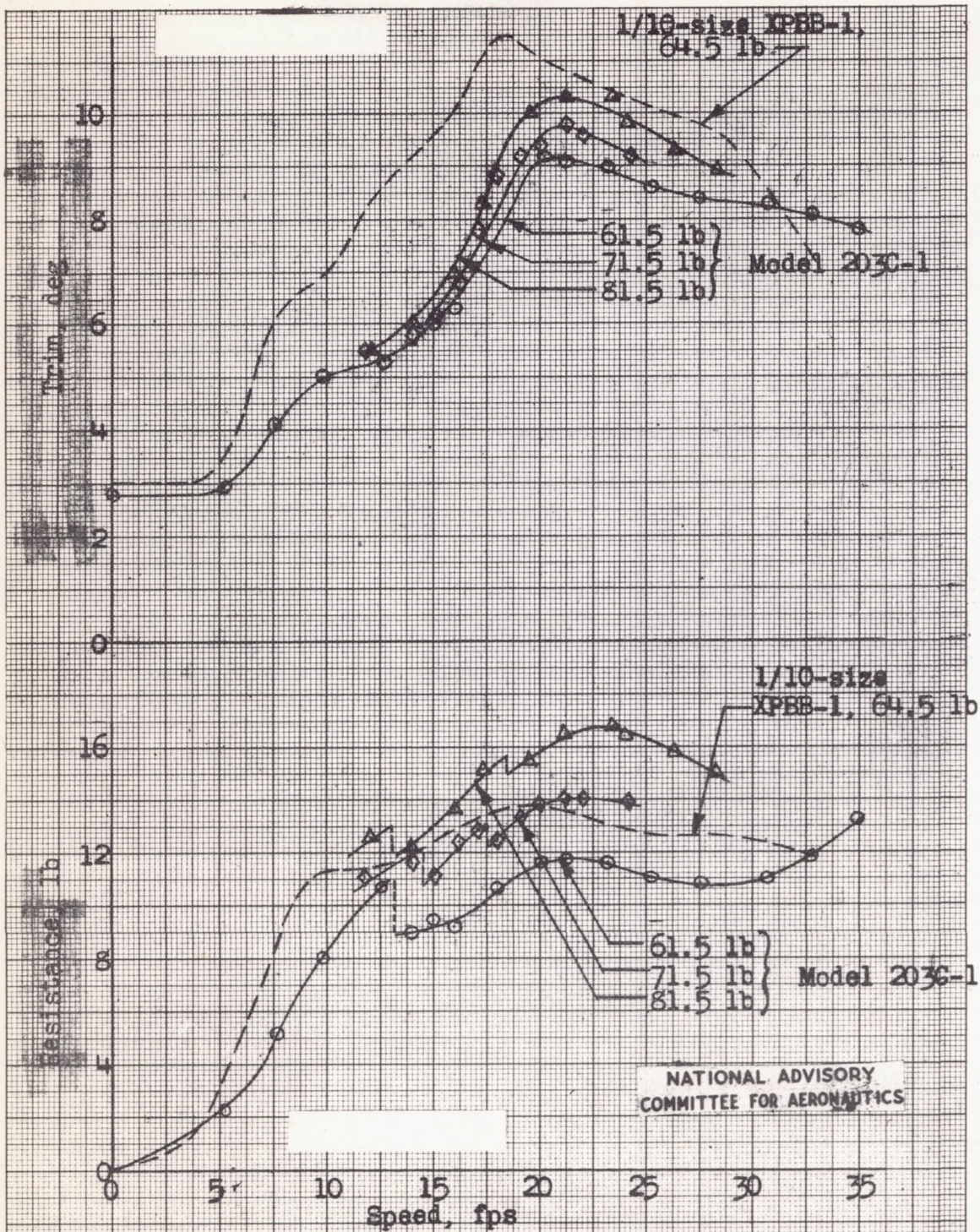
Figure 10.- Model 2030-1, total resistance and trim, Center of gravity 28 percent mean aerodynamic chord; elevator deflection, -10 degrees.
