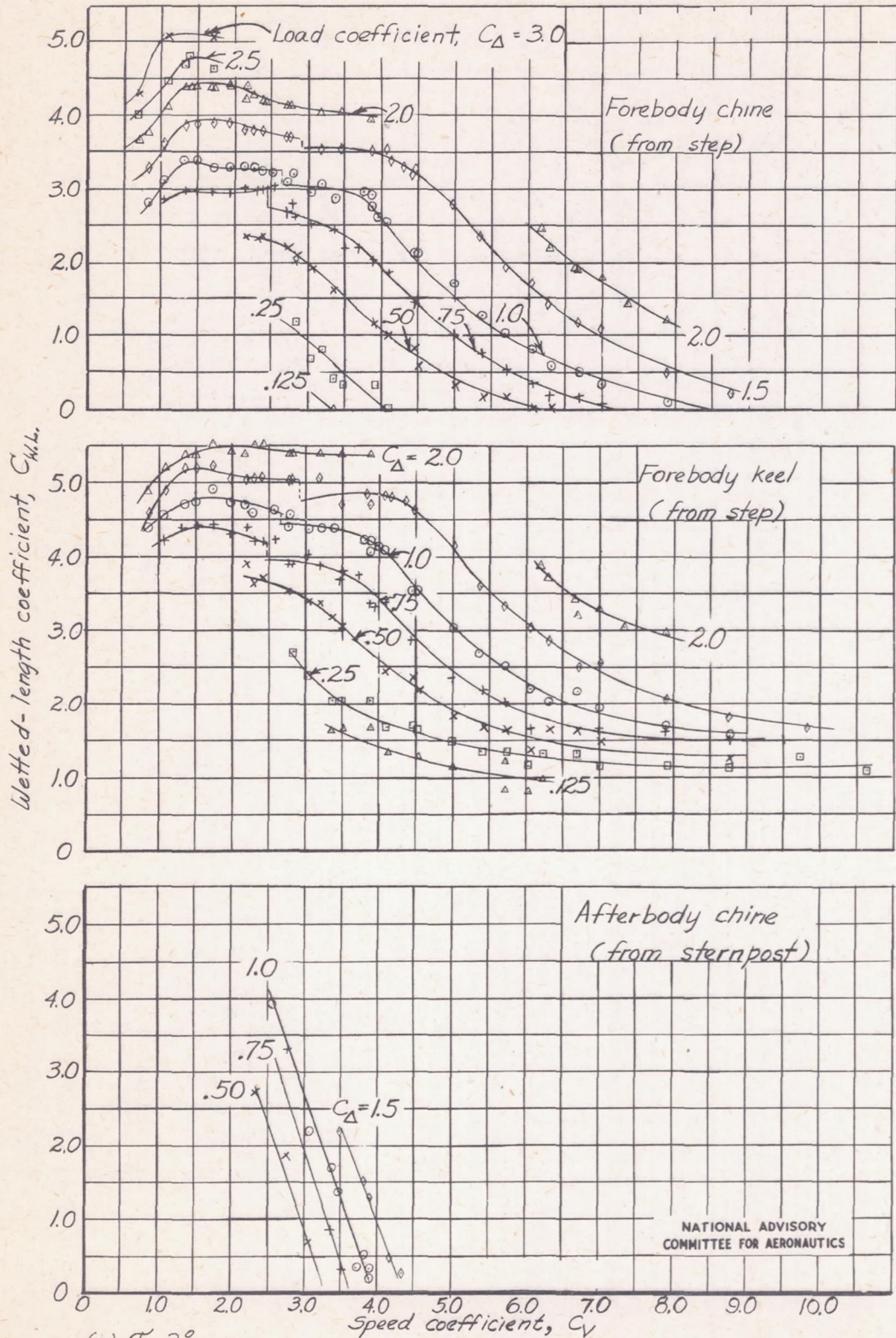
Figure 8.- Model 185. Wetted-length characteristics.
