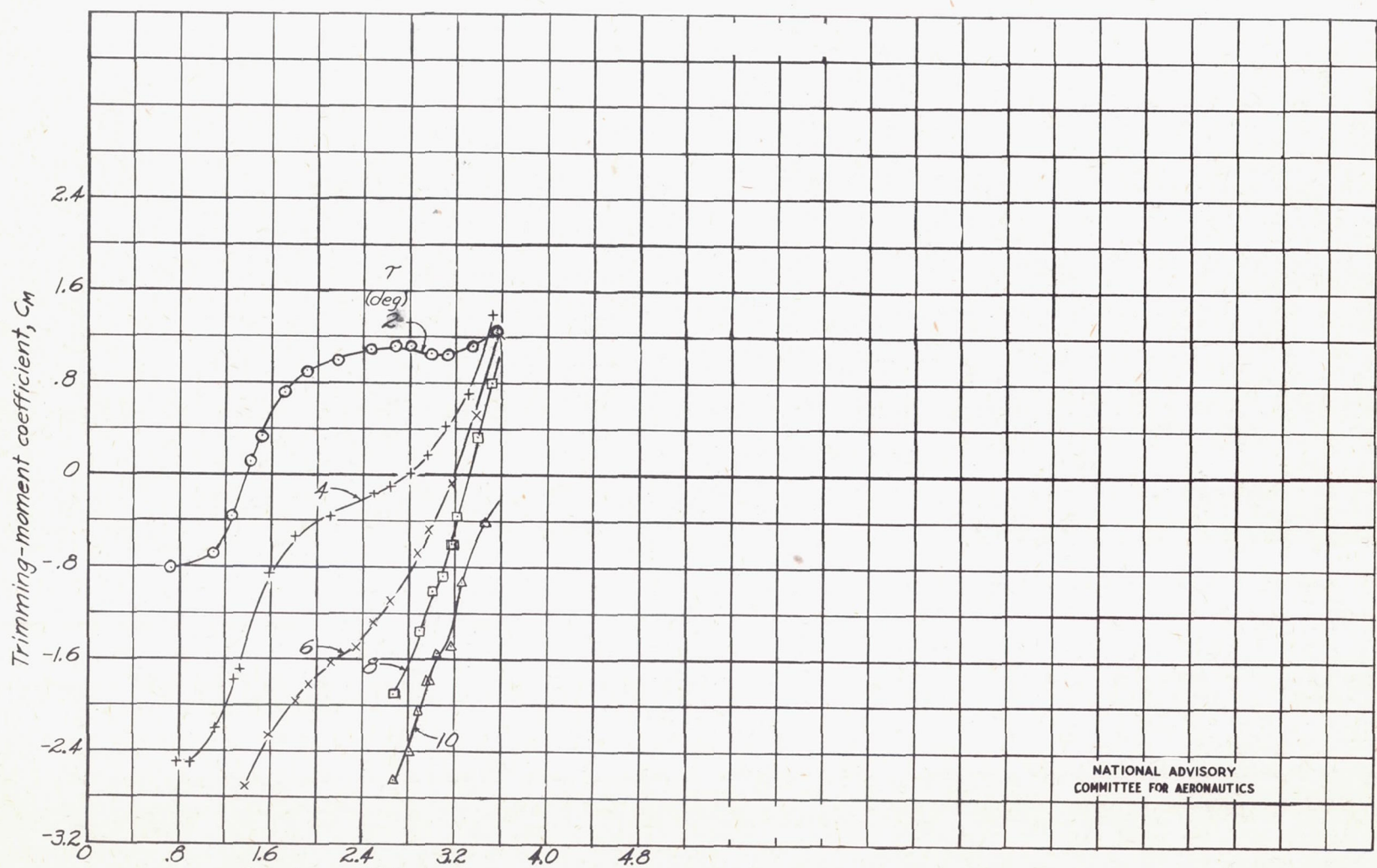
Speed coefficient, C_v (a) Load coefficient, C_L = 4.0 . Figure 5.- Model 185. Trimming-moment characteristics.
