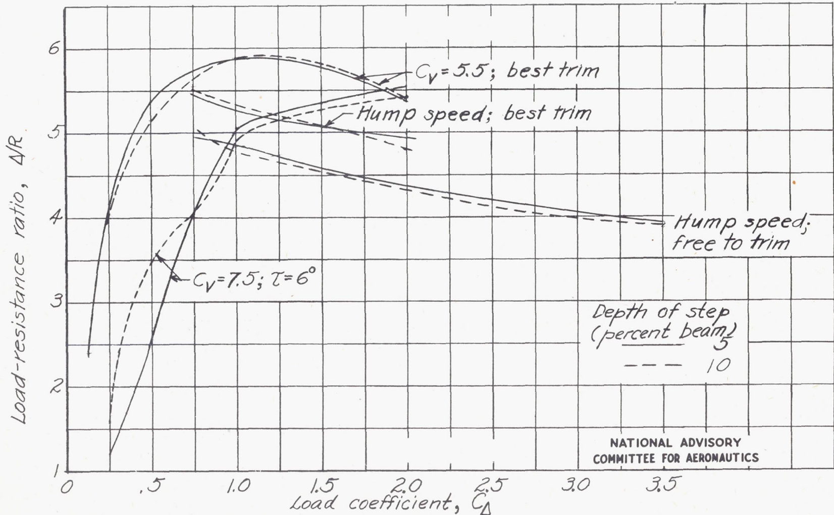
Figure 14.-Variation of load-resistance ratio with load for two depths of step.
