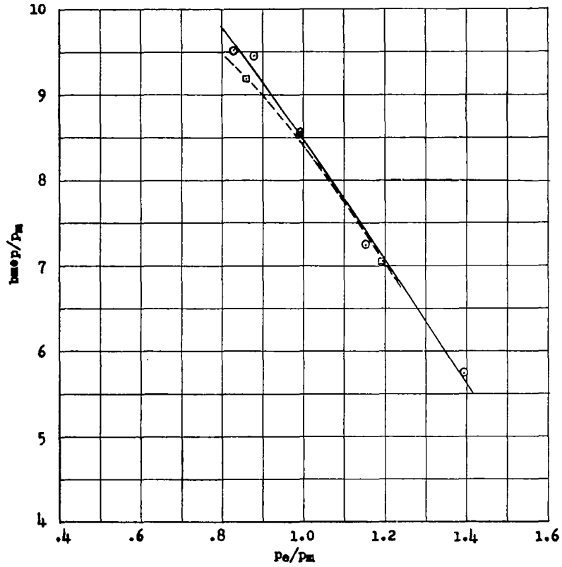
(b) Engine speed, 2000 rpm. Figure 7. - Continued.
