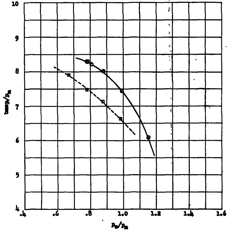
(e) Engine speed, 3500 rpm.
