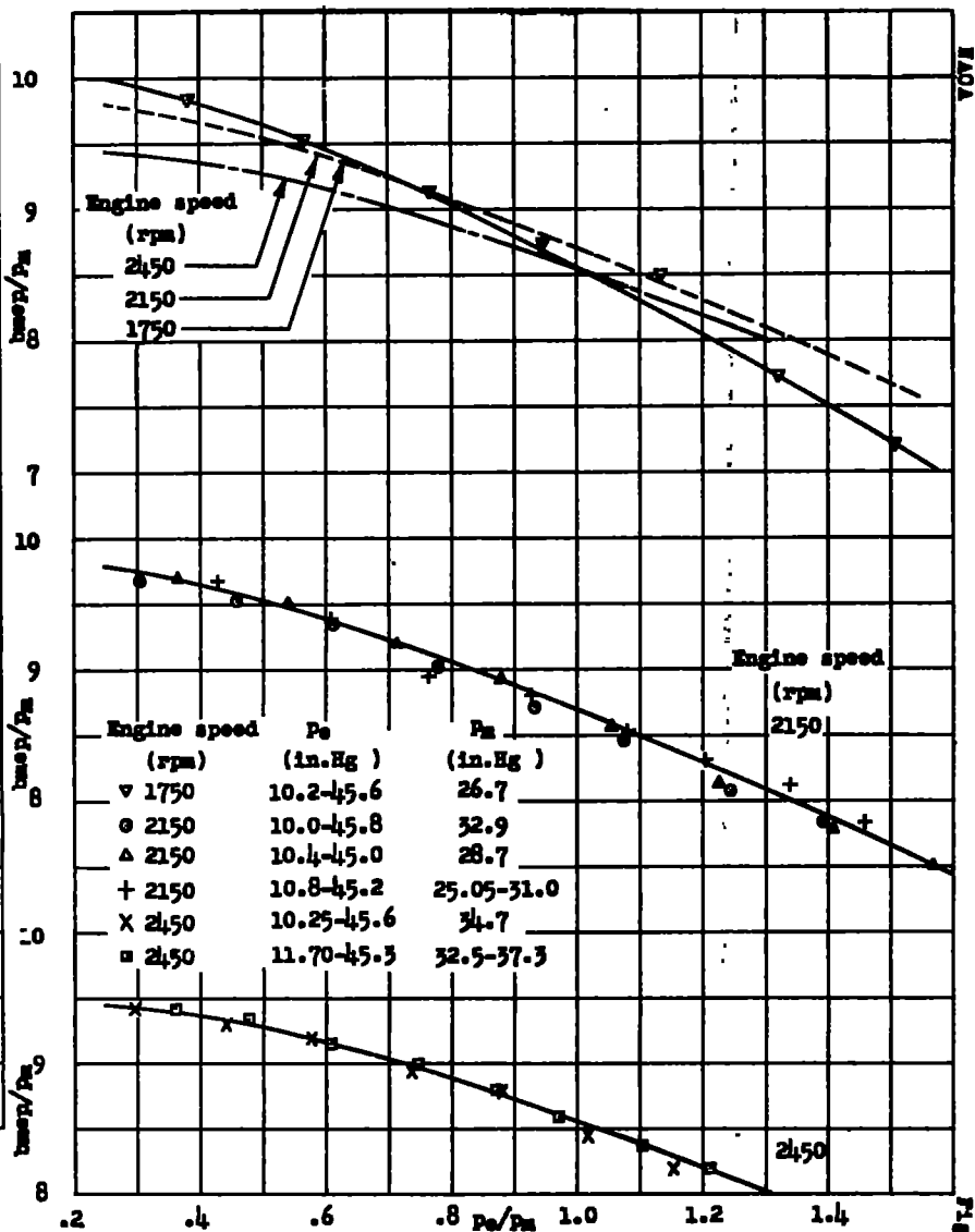
Figure 3. - Effect of exhaust back pressure on engine power for Pratt & Whitney R-1830-64 engine. Ratio of impeller tip speed to engine speed, 26.2 feet; compression ratio, 6.5.
