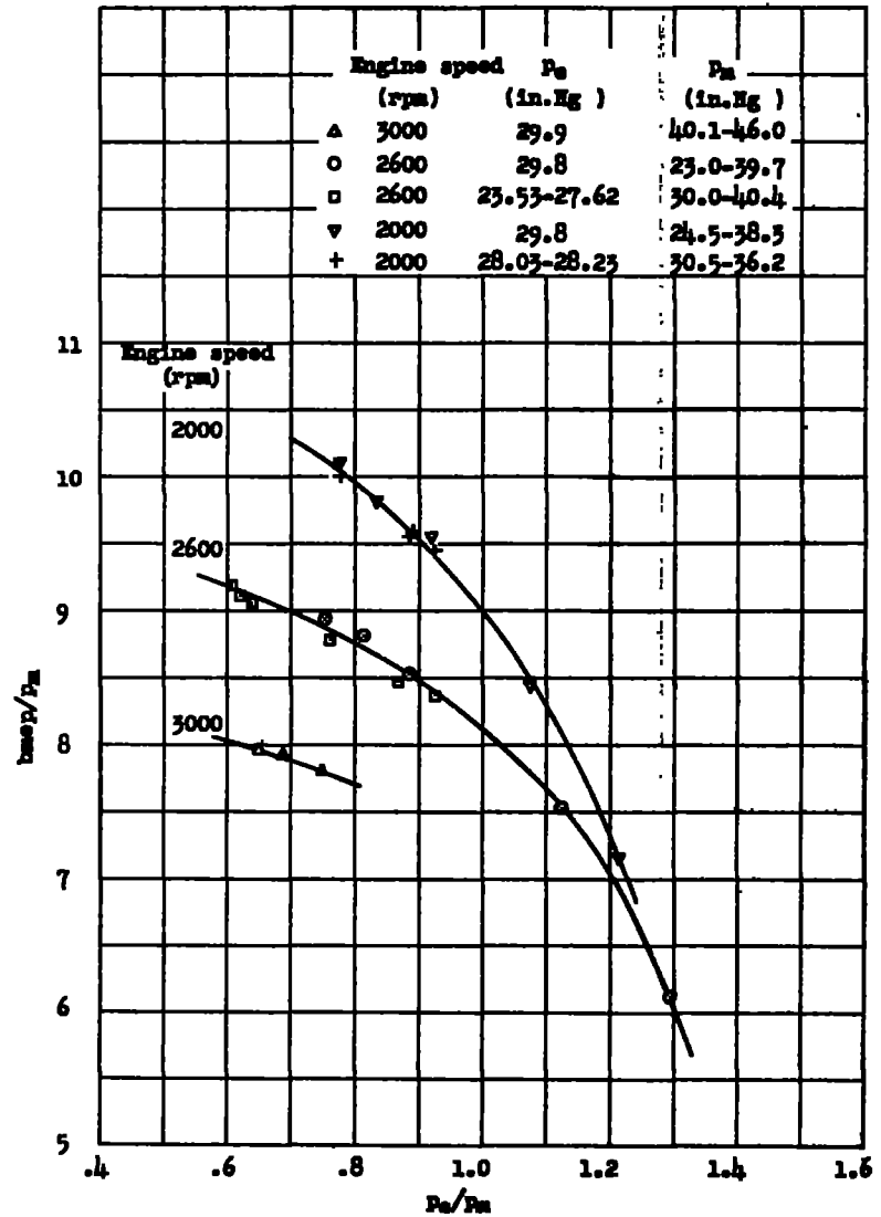
Figure 5. - Effect of exhaust back pressure on engine power for Allison XV-1710-6 engine. Ratio of impeller tip speed to engine speed, 21.9 feet; compression ratio, 6.65.
