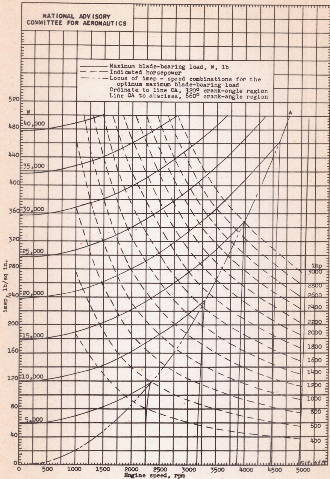
(a) Compression ratio, 5.50. Figure 14. - Maximum load on blade bearing of a production V-type engine for all values of indicated mean effective pressure and engine speed at various compression ratios. (Constant maximum-load curves.) Effective bearing area, 3.44 square inches.
