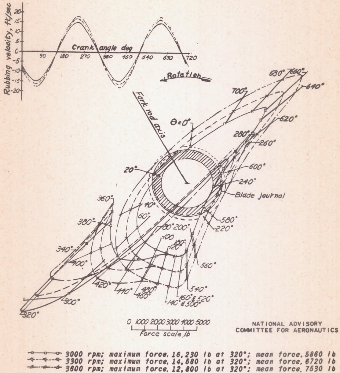
Figure 5. - Polar diagrams showing the magnitude of the resultant force on the blade journal of a V-type engine and its direction with respect to the fork-rod axis at an indicated mean effective pressure of 242 pounds per square inch.
