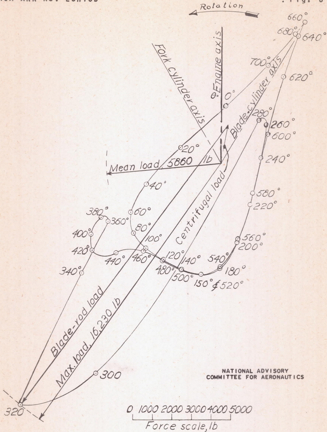
Figure 3. - Polar diagram showing the magnitude of the resultant force on the blade journal of a V-type engine and its direction with respect to the engine axis. Engine speed, 3000 rpm; indicated mean effective pressure, 242 pounds per square inch.
