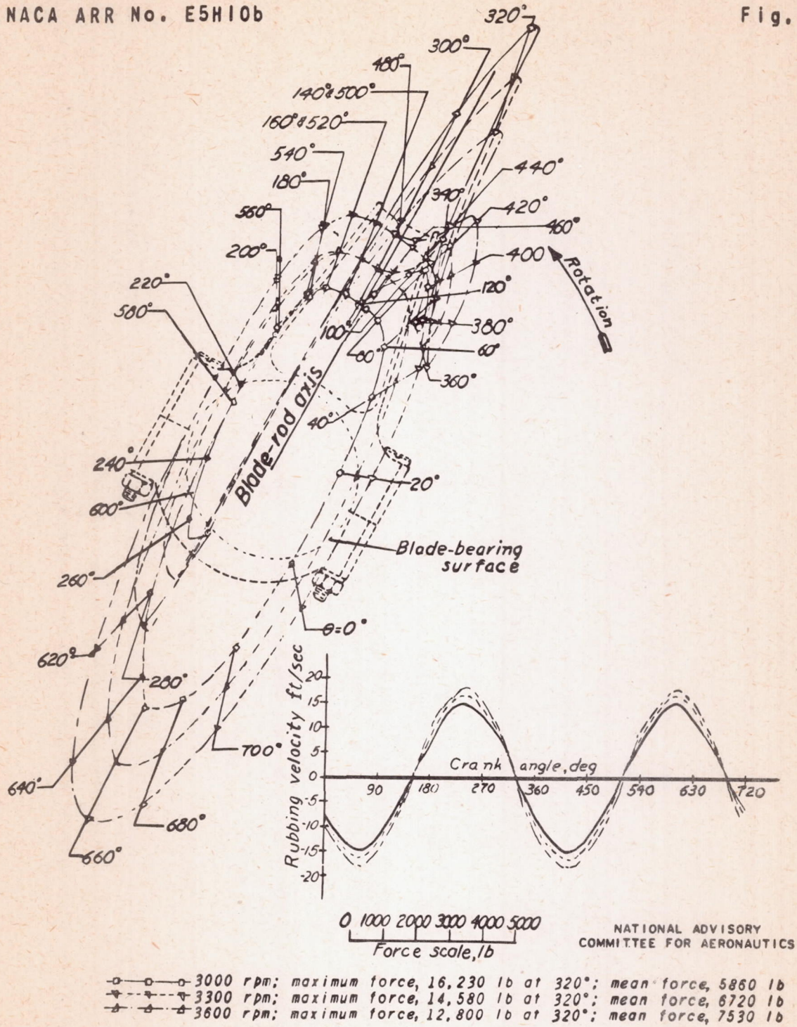
Figure 7. - Polar diagrams showing the magnitude of the resultant force on the blade bearing of a V-type engine and its direction with respect to the blade-rod axis at an indicated mean effective pressure of 242 pounds per square inch.
