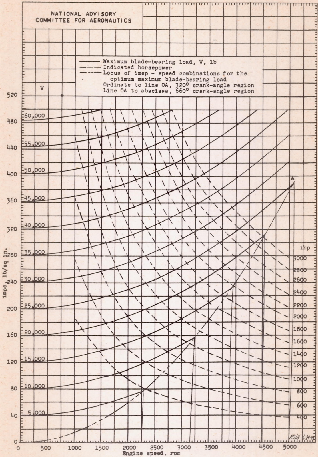
(c) Compression ratio, 8.50. Figure 14. - Concluded.
