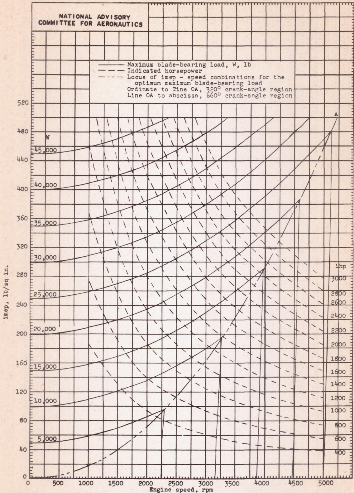
Figure 9. - Maximum load on blade bearing of a production, V-type engine for all values of indicated mean effective pressure and engine speed at a compression ratio of 6.65. (Constant maximum-load curves.) Effective bearing area, 3.44 square inches.
