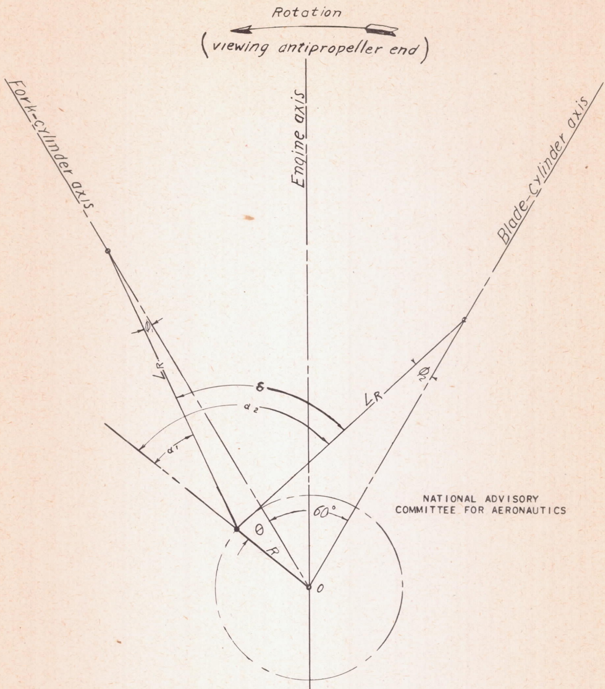
Figure 1. - Schematic diagram of the mechanism of a 12 cylinder V-type engine.
