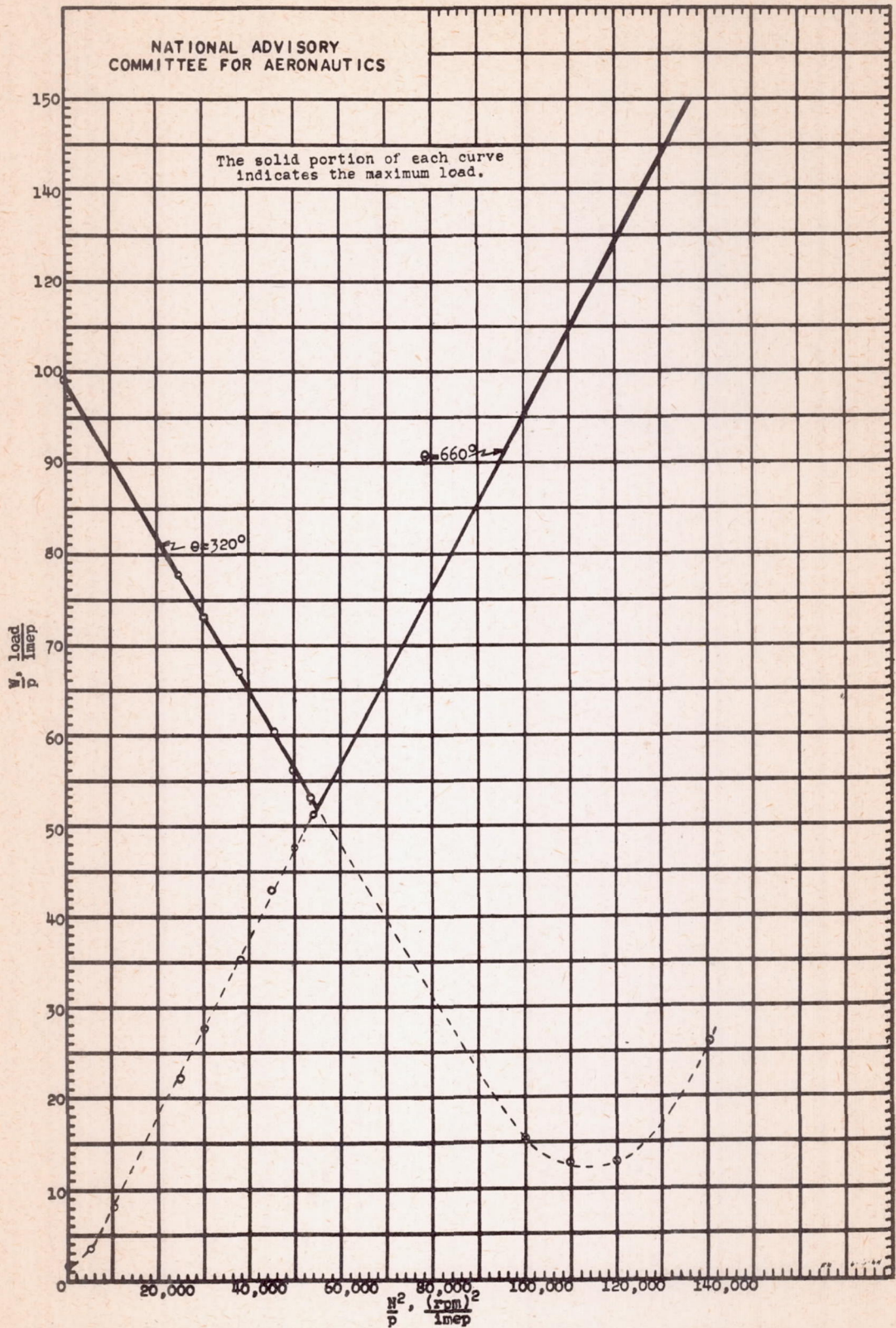
Figure 8. - Representative plot showing the variations of W/p with N^2/p at crank angles of 320^\circ and 660^\circ for a V-type engine.
