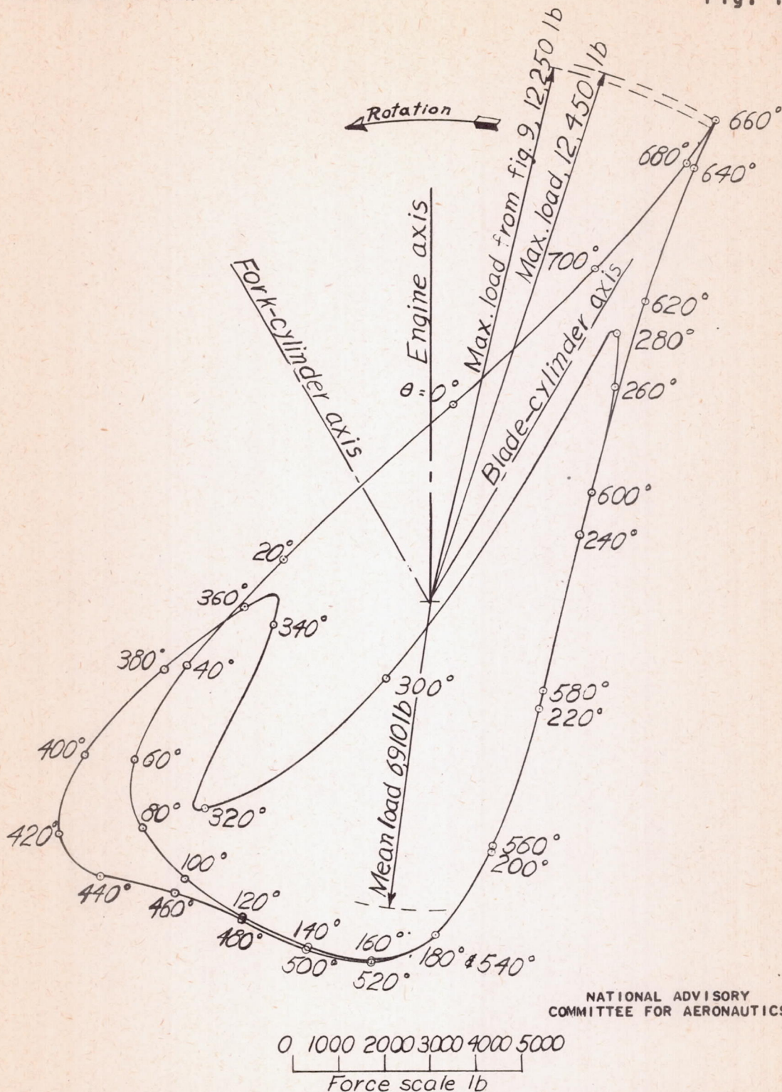
Figure 13. - Polar diagram showing the magnitude of the resultant force on the blade journal of a V-type engine and its direction with respect to the engine axis. Engine speed, 3600 rpm; indicated mean effective pressure, 182 pounds per square inch.
