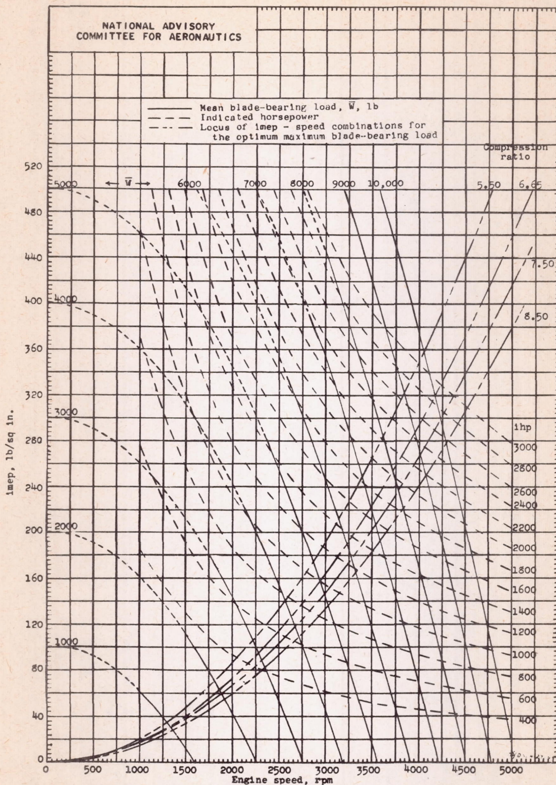
Figure 11. - Mean load on blade bearing of a production V-type engine for all values of indicated mean effective pressure and engine speed. (Constant mean-load curves.) Effective bearing area, 3.44 square inches.
