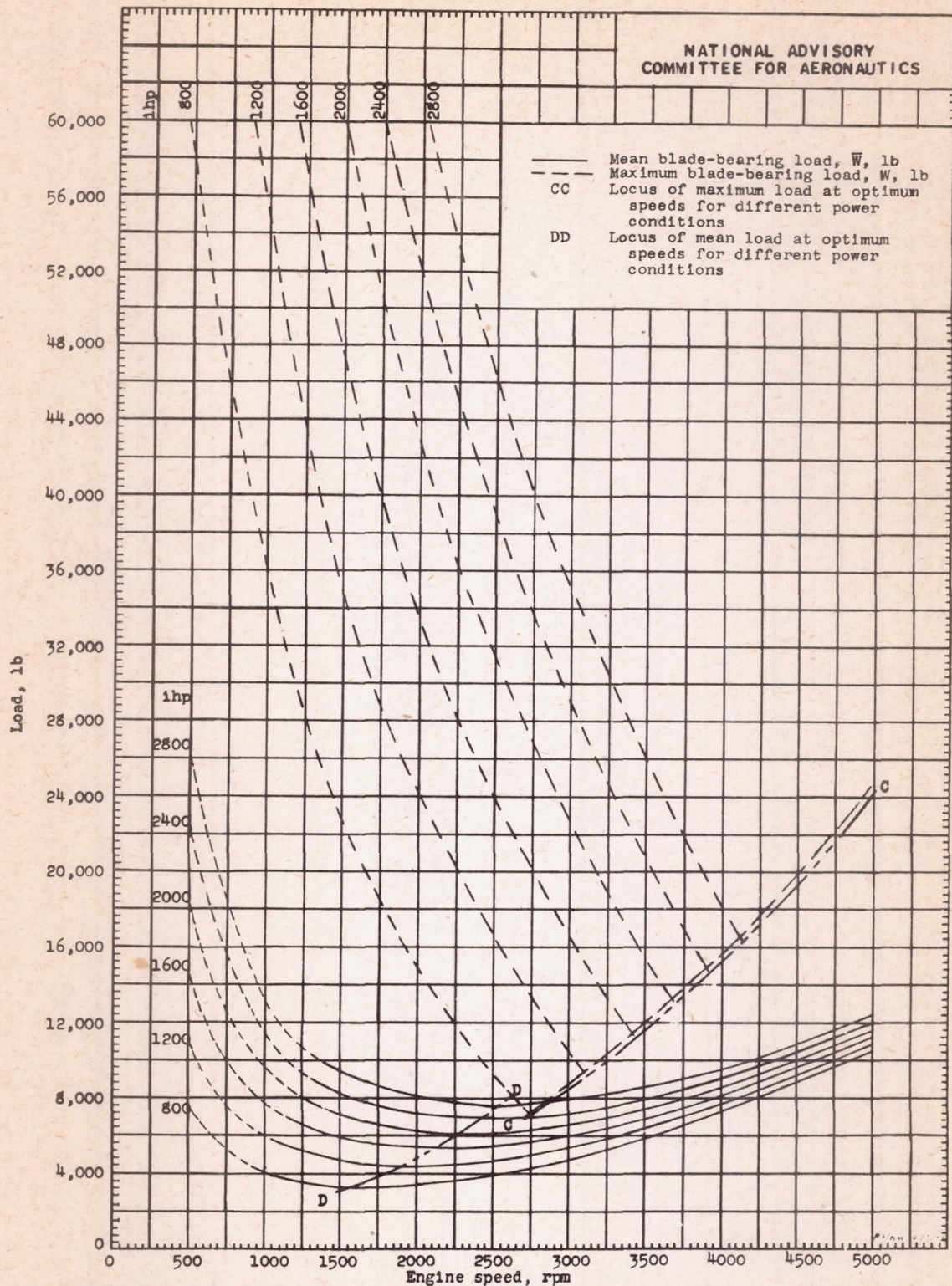
Figure 12. - Mean and maximum load on blade bearing of a V-type engine for all values of indicated horsepower and engine speed at a compression ratio of 6.65. (Constant indicated-horsepower curves.) Effective bearing area, 3.44 square inches.
