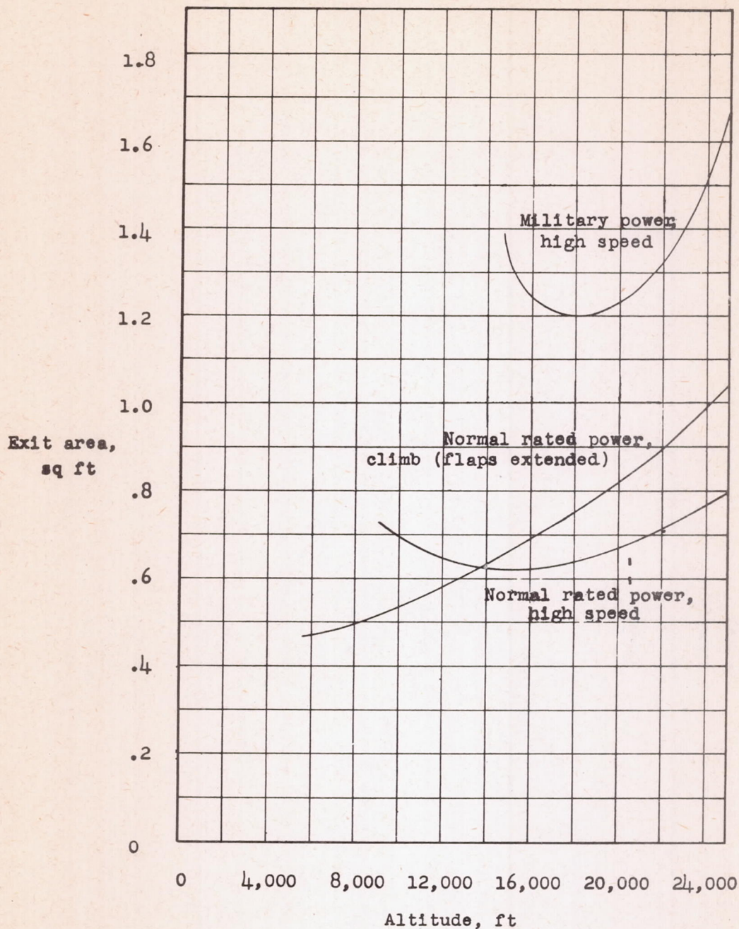
Figure 7.- Intercooler duct exit area.
