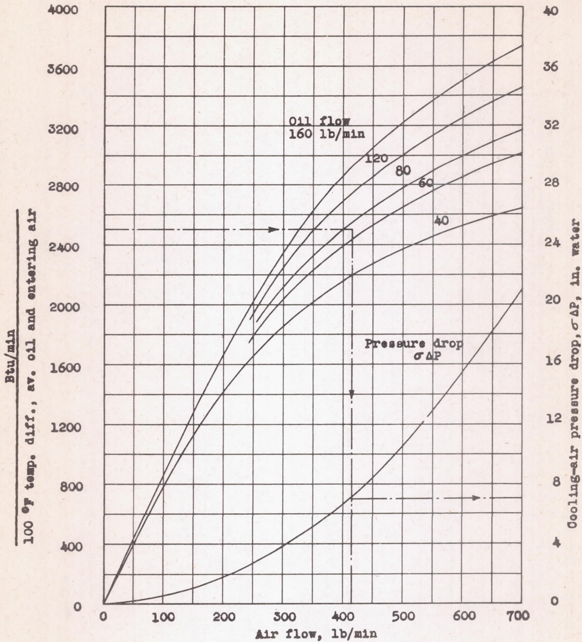
Figure 4.- The characteristics of an oil cooler. Diameter, 13 inches; depth, 9 inches.
