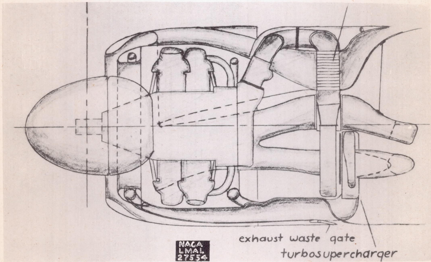
Figure 2.- Power plant installation.
