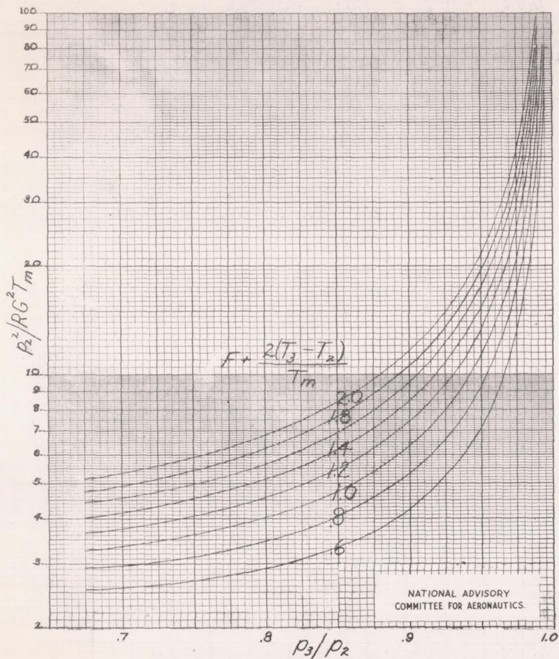
(a) Small values of p_3/p_2 .
