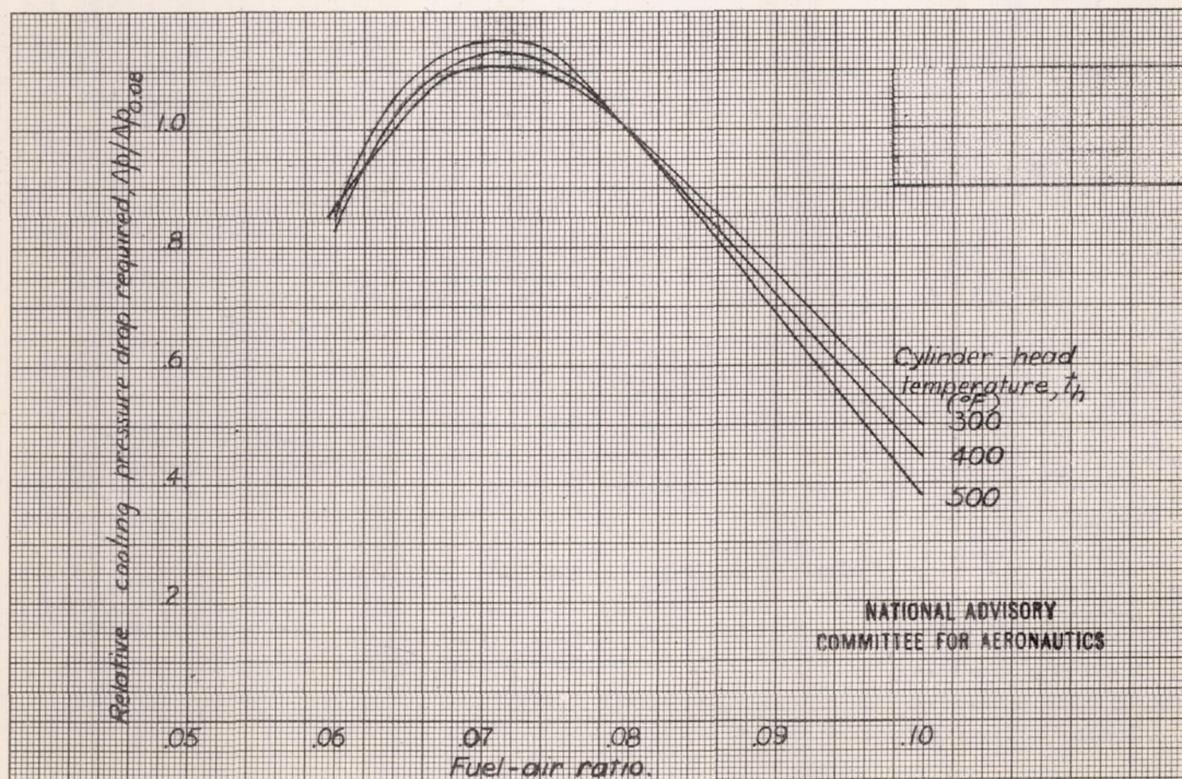
Figure 2.- Effect of fuel-air ratio on sea-level cooling pressure drop. Values are given relative to pressure drop required for fuel-air ratio of 0.08.
