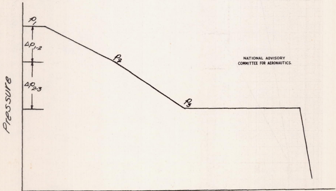
Figure 4.- Diagram of cooling-air flow path and pressure drops.
