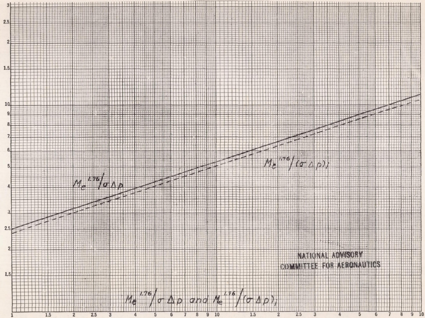
Figure 12.-Cooling correlation curve for the example engine.
