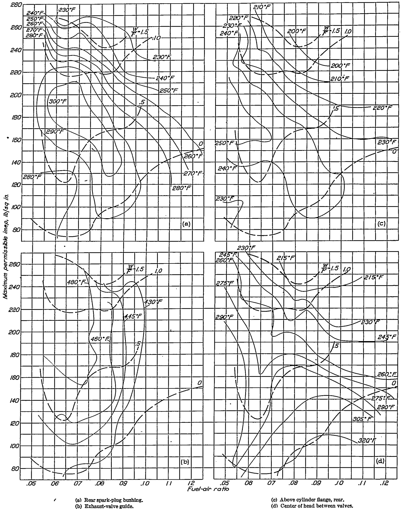
FIGURE 13.—Relation between fuel-air ratio, maximum permissible indicated mean effective pressure, engine temperatures, and water-fuel ratios of 0, 0.5, 1.0, and 1.5. Cylinder displacement, 202 cubic inches; engine speed, 2000 rpm; spark advance, 20°; compression ratio, 7.0; Inlet-air temperature, 250° F; cooling pressure drop, 14.0 inches water; fuel, 80-octane number.
