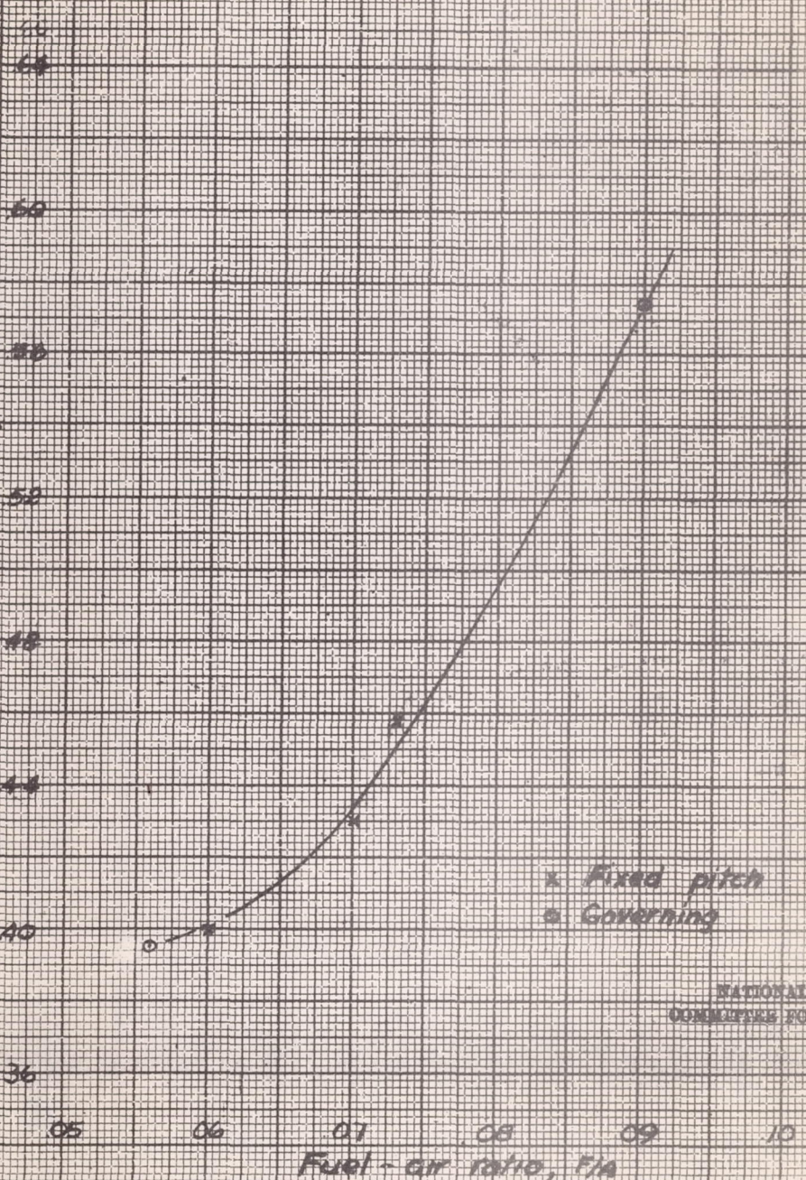
Figure 6. - Variation of brake specific fuel consumption with fuel-air ratio for constant power approximately 660 horsepower.
