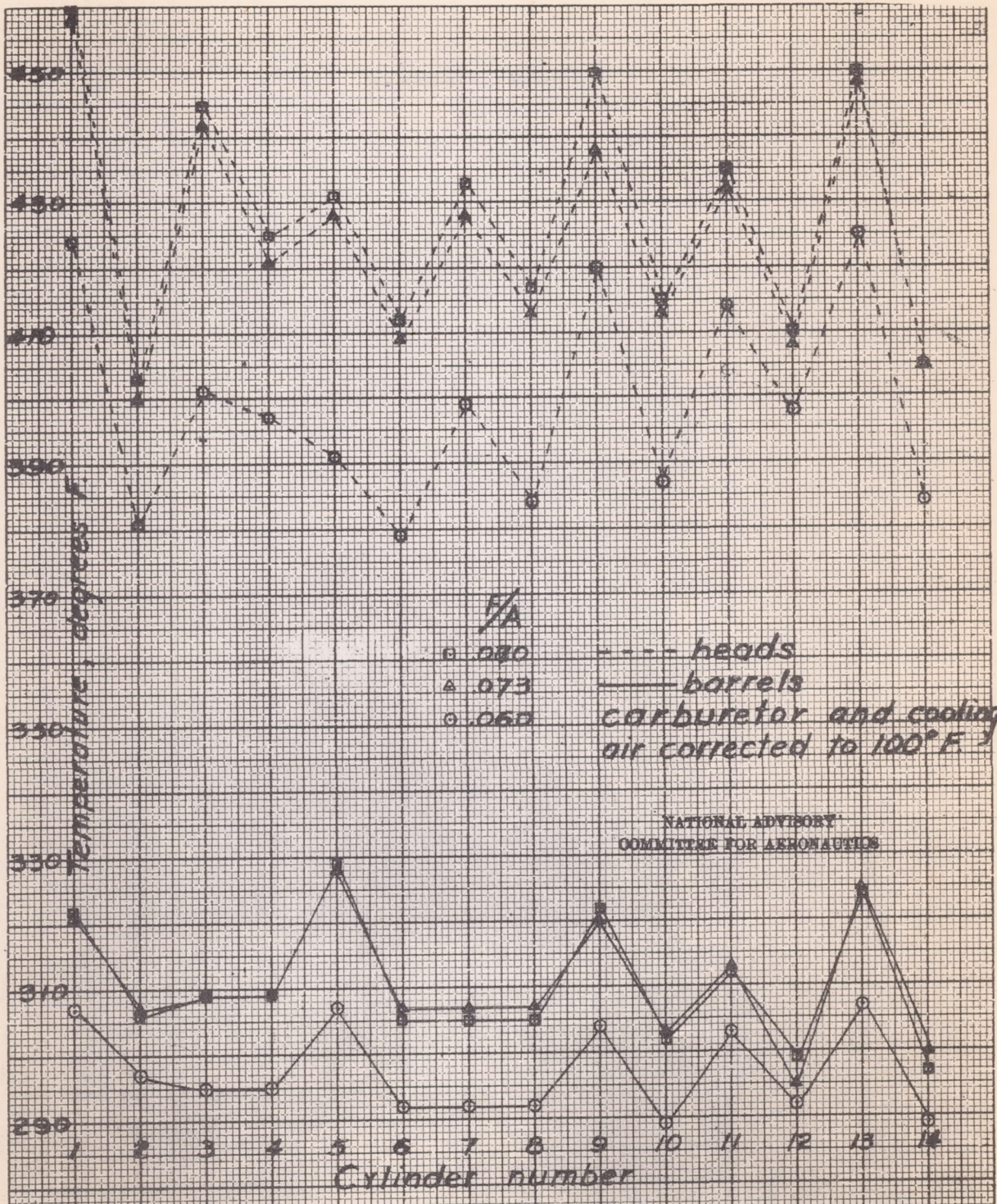
Figure 5. - Distribution of the head and barrel temperatures on the 1830-A engine installation for three fuel-air ratios. Constant power at 2230 rpm; \phi = 21^\circ at 42-inch radius.
