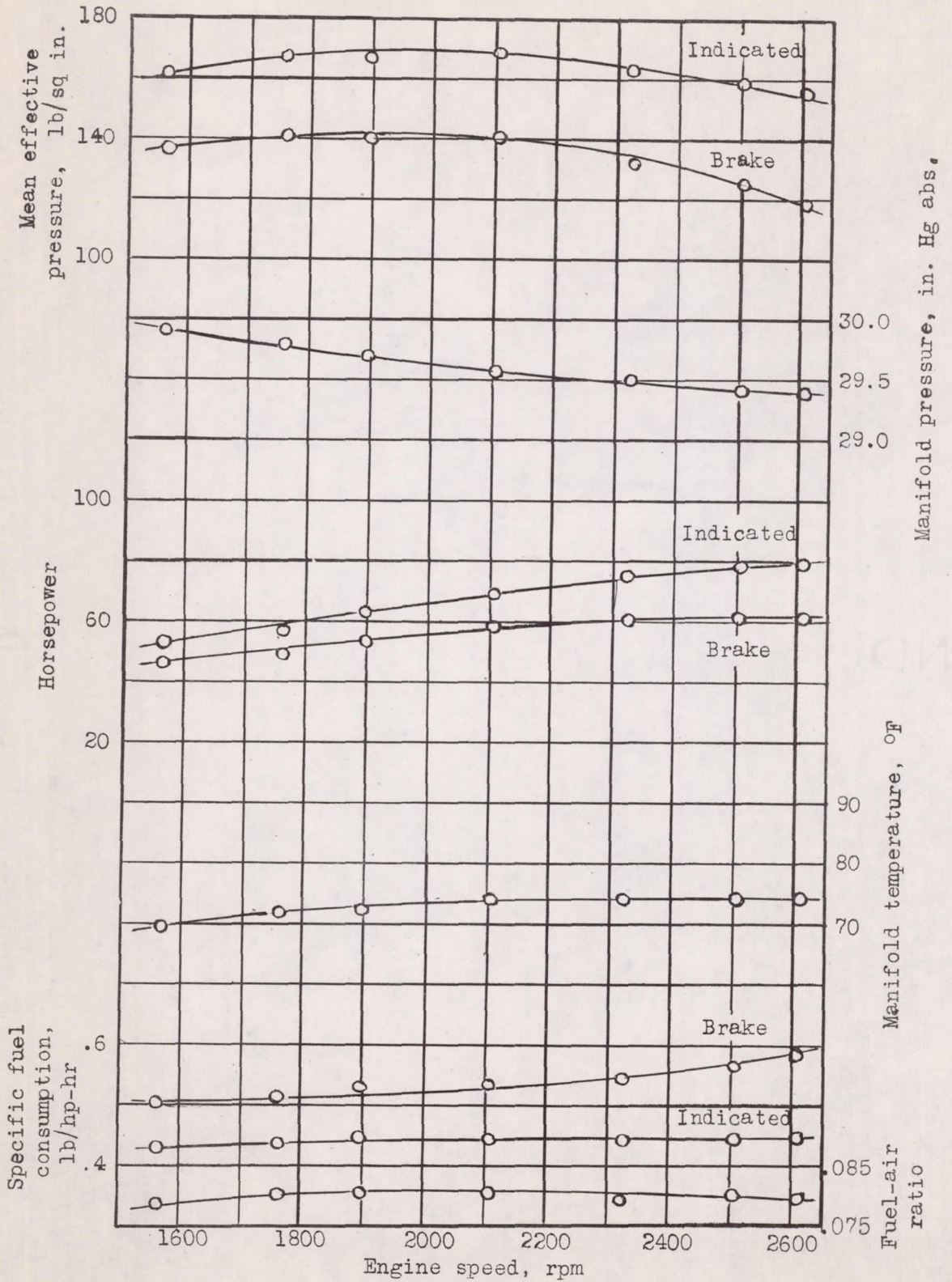
Figure 12.- Variation of performance with engine speed.
