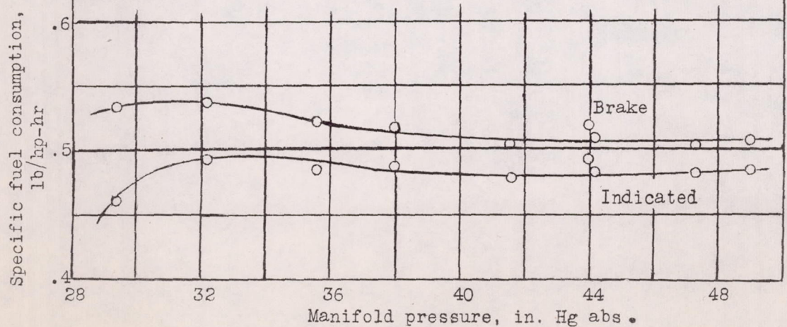
Figure 14.- Variation of performance with manifold pressure.
