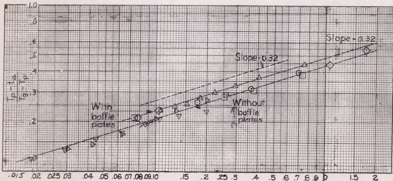
Fig. 10.- Variation of (T_p - t_a) / (T_g - T_p) with (W_c)^{1.76} / (\Delta p p_i / \rho) and (W_t)^{1.14} / W_c
