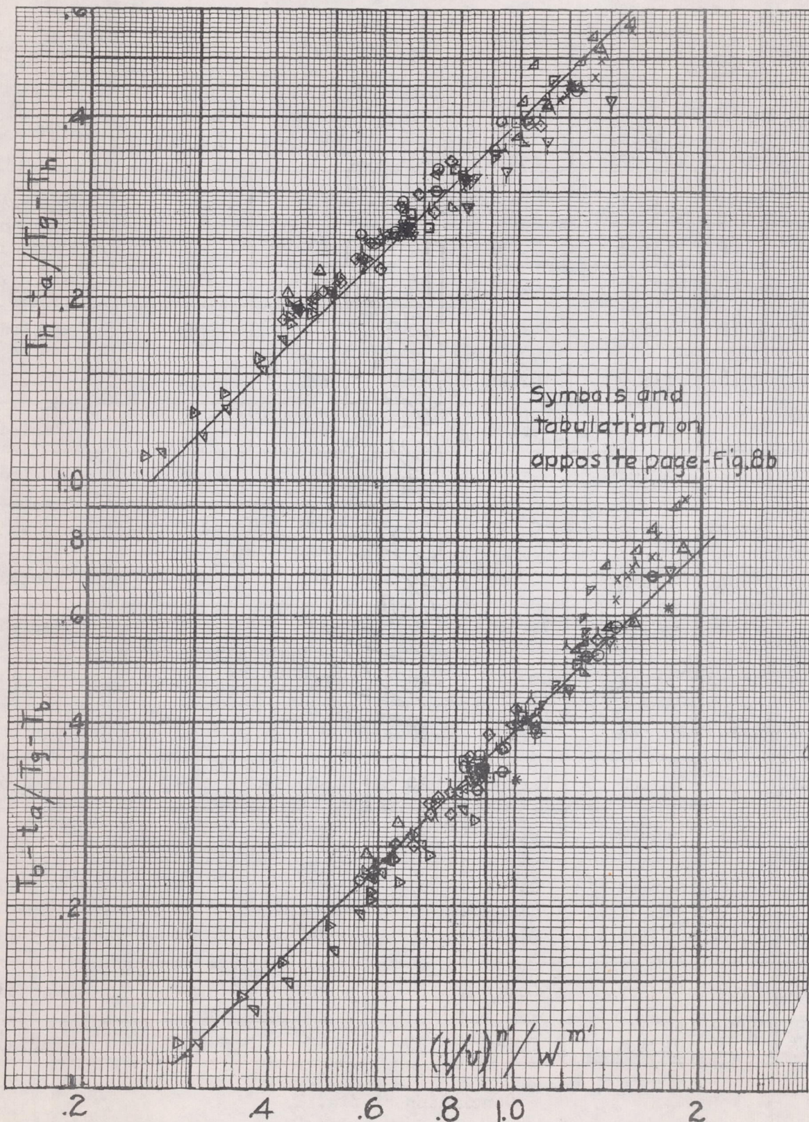
Figure 8.- Variation of (T_h - t_a) / (T_g - T_h) and (T_b - t_a) / (T_g - T_b) with (I/v)^{n_1} / W^{m_1} for single-cylinder engine.
