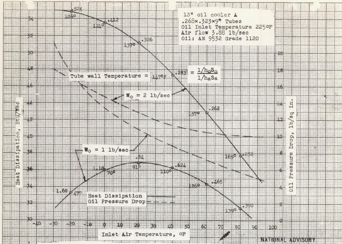
Figure 2.- Congealing tests of 13" oil cooler A.
