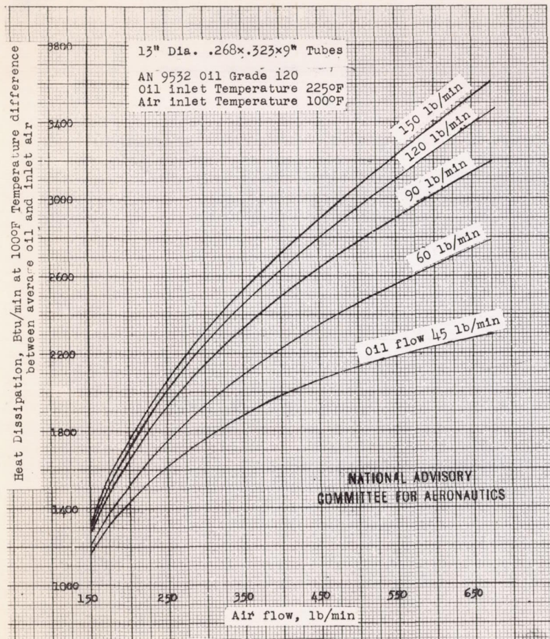
Figure 11.- Performance characteristics of 13" oil cooler .
