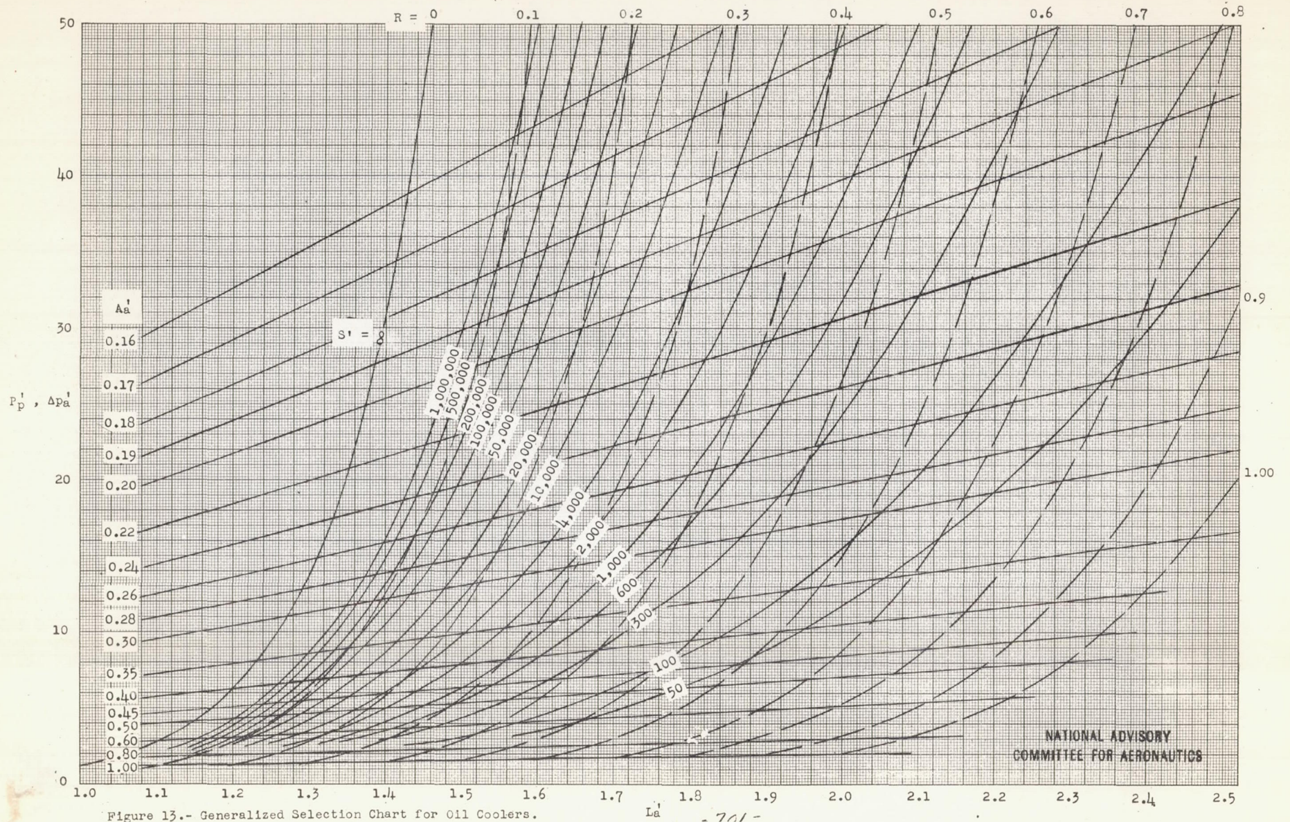
Figure 13.- Generalized Selection Chart for Oil Coolers.
