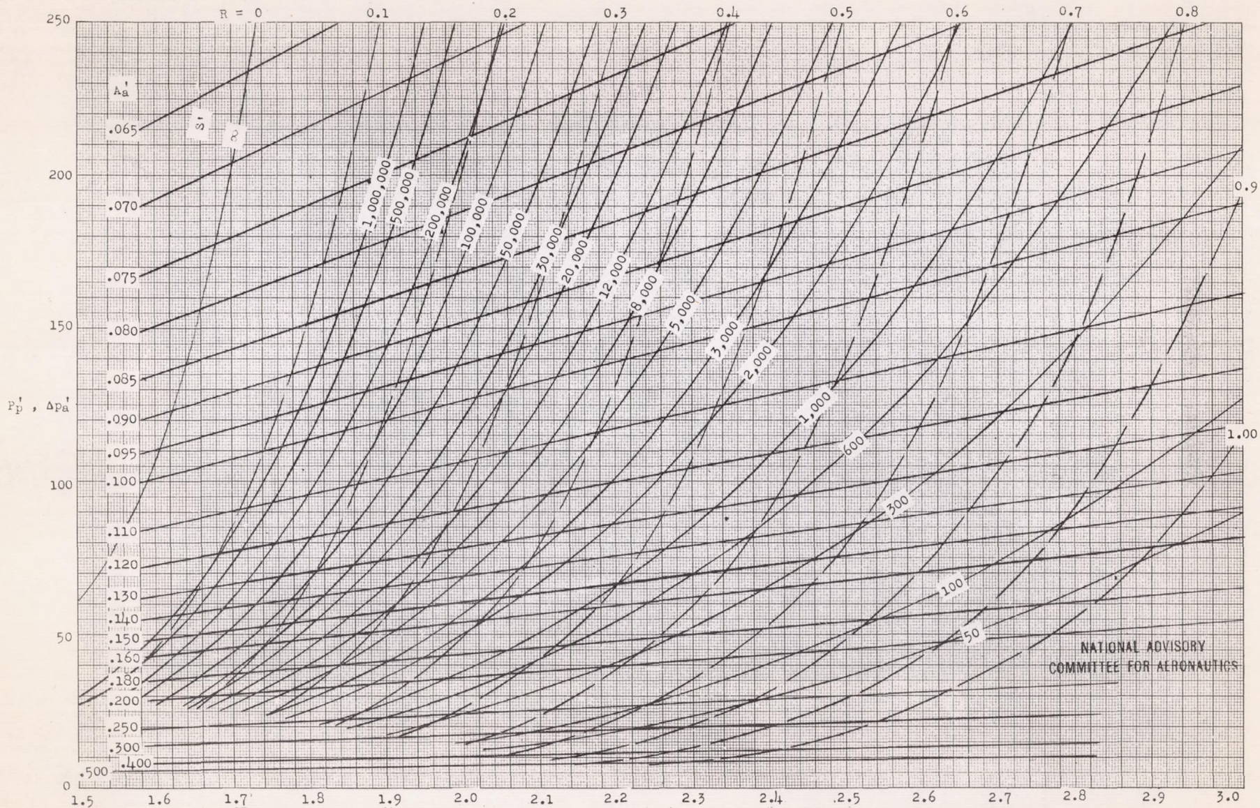
Figure 13.- Concluded, Generalized Selection Chart for Oil Coolers
