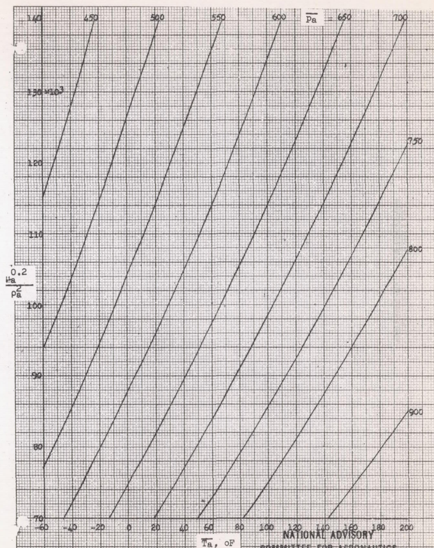
Figure 15.- Concluded, \frac{\rho_a^{0.2} V_a}{\rho_a} as a function of T_a and \bar{p}_a
