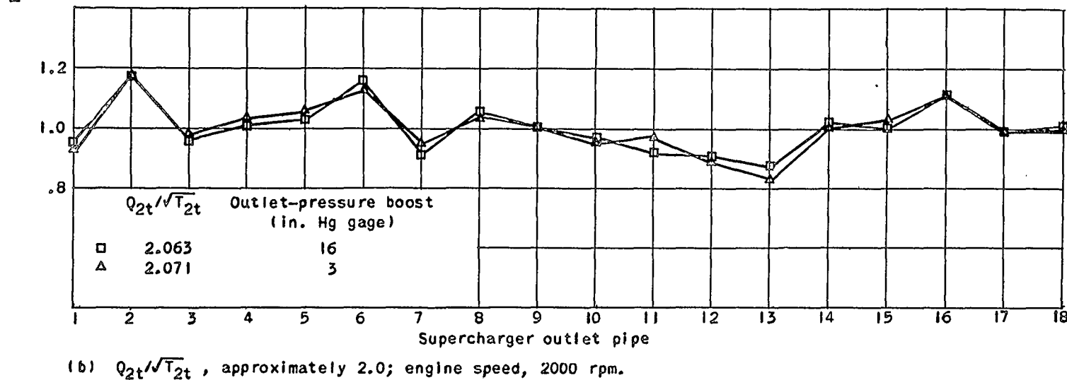
Figure 9. - Effect of outlet pressure on air-flow distribution in supercharger outlets with NACA 18-vane diffuser. Carburetor-throttle angle, 66°.
