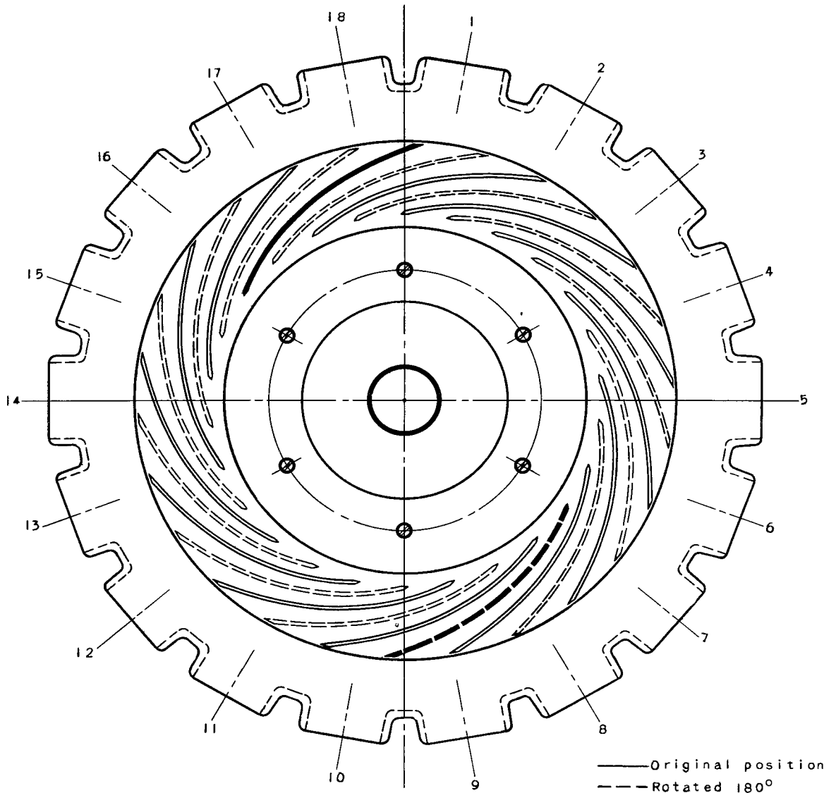
Figure 2. - Sketch of standard 13-vane diffuser in original position and rotated 180° showing relation of diffuser vanes and supercharger outlets.
