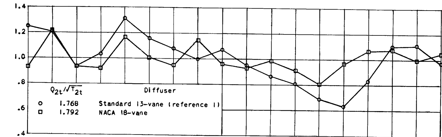
(c) Q_{2t}/\sqrt{T_{2t}} , approximately 1.8; engine speed, 2400 rpm.
