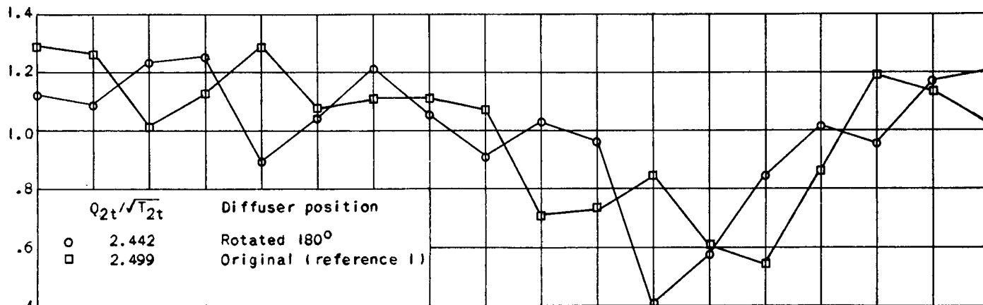
(c) Q_{2t}/\sqrt{T_{2t}} , approximately 2.5; engine speed, 2400 rpm.
