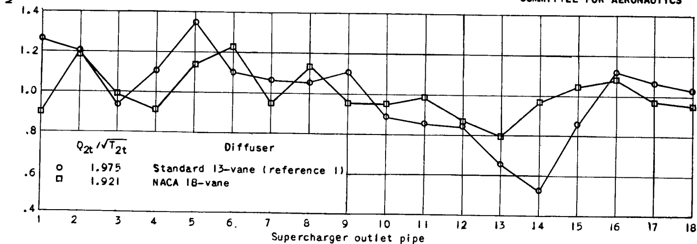
(d) Q_{2t}/\sqrt{T_{2t}} , approximately 1.95; engine speed, 2400 rpm.
