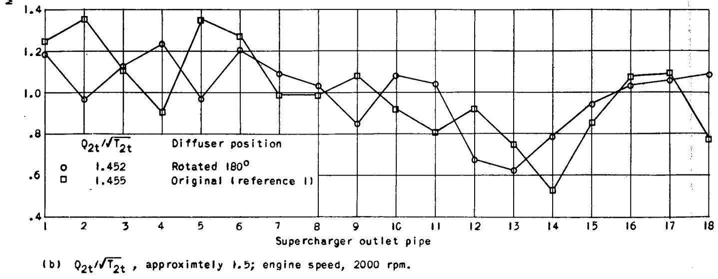
Figure 5. - Effect of rotating standard 13-vane diffuser 180° on air-flow distribution in supercharger outlets. Reference outlet pressure, 6 inches mercury gage; carburetor-throttle angle, 66°.
