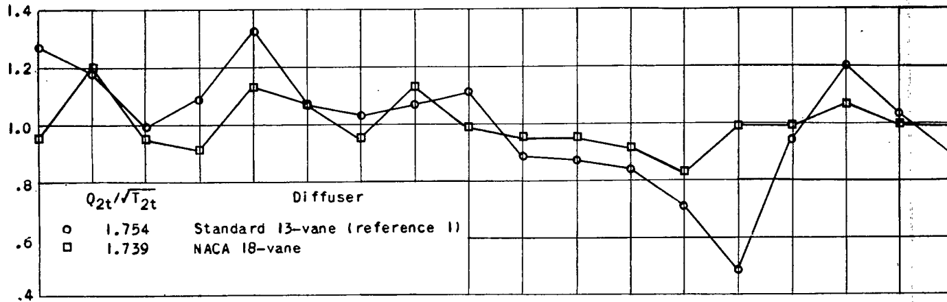
(a) Q_{2t}/\sqrt{T_{2t}} , approximately 1.7; engine speed, 2000 rpm.
