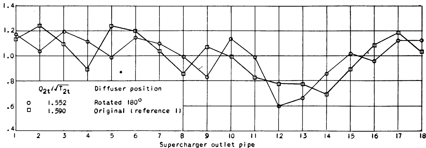
(d) Q_{2t}/\sqrt{T_{2t}} , approximately 1.6; engine speed, 2400 rpm.
