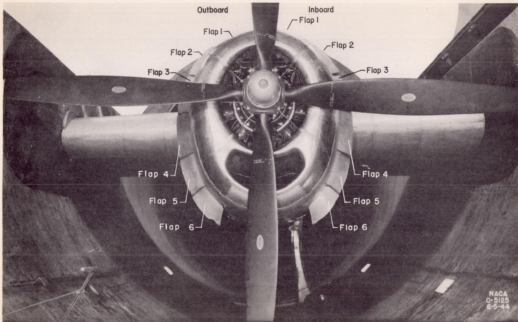
Figure 1. - Front view of power-plant installation in altitude wind tunnel. Production configuration.
