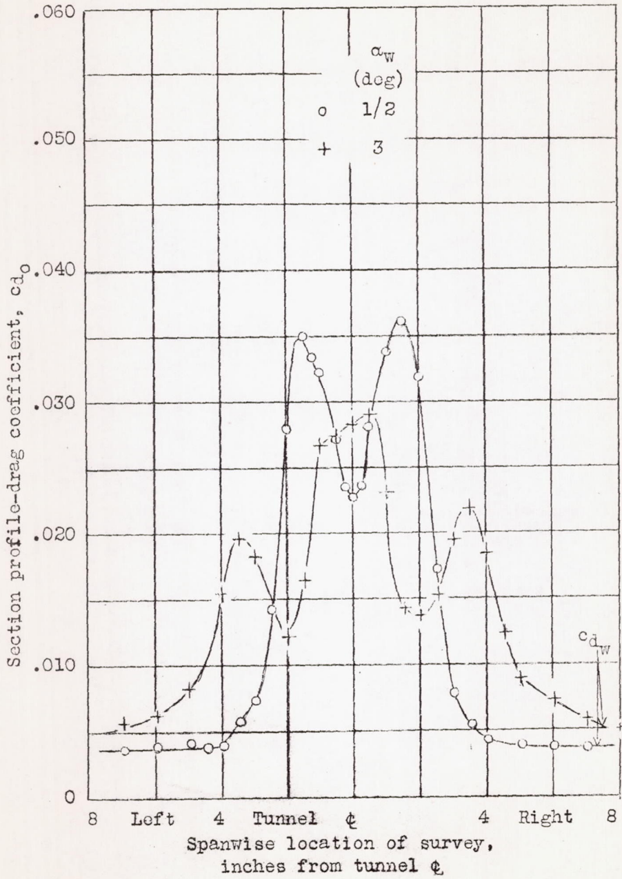
Figure 3.- Typical spanwise drag plot. Nacelle in smooth condition; R_w, 6.5 \times 10^6 .
