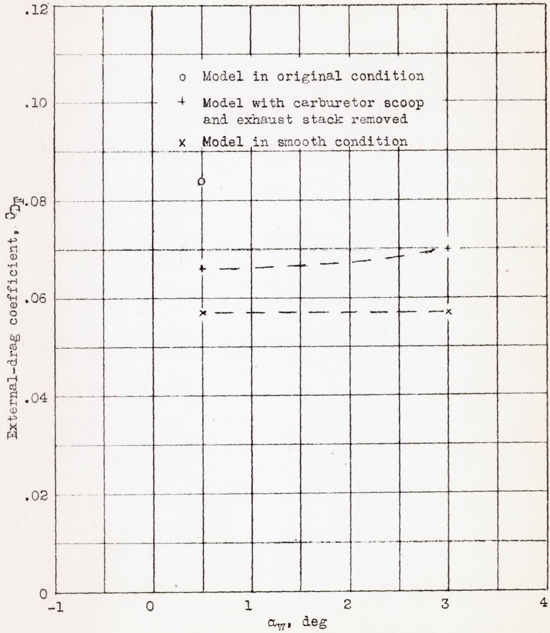
Figure 4.- Nacelle external-drag coefficients. R_w, 6.5 \times 10^6 .
