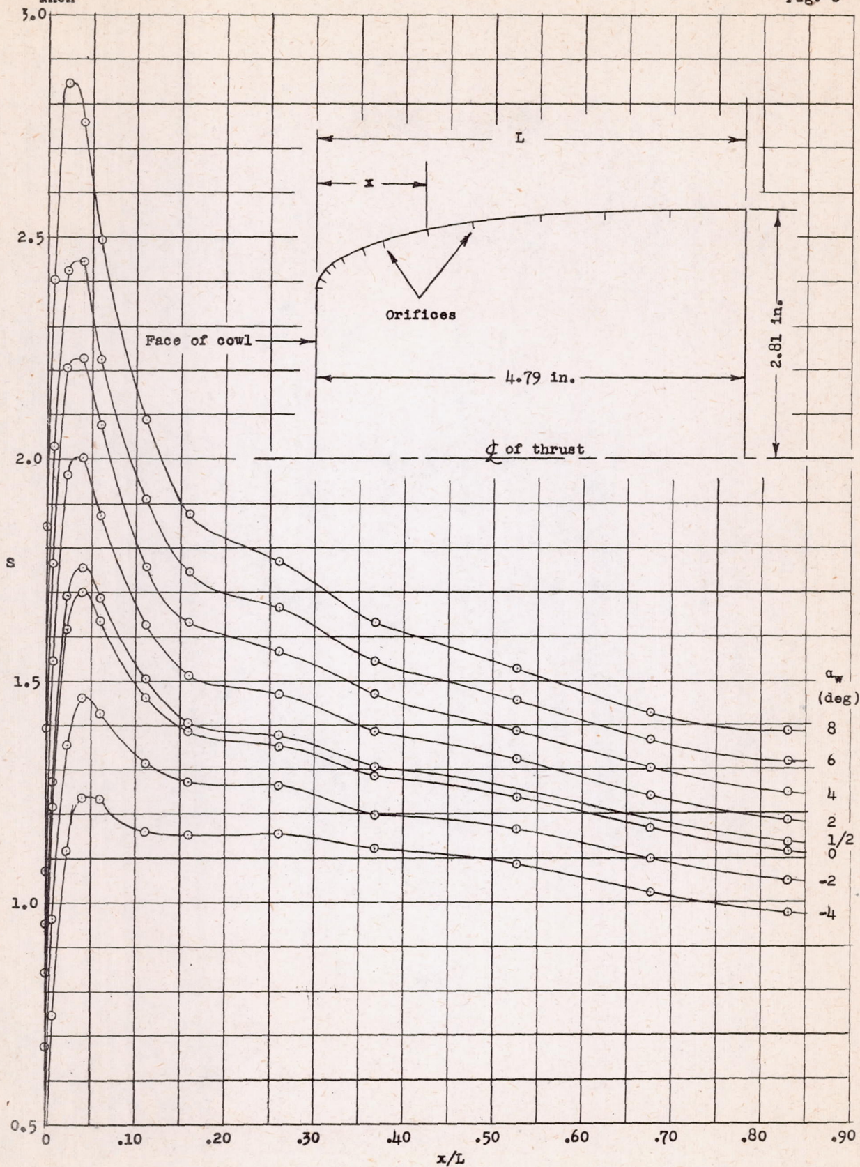
Figure 6.- Pressure distribution over top of cowl. R_w, 6.5 \times 10^6 . (Angles of attack are those of wing which has 1/2^\circ incidence to nacelle thrust line.)
