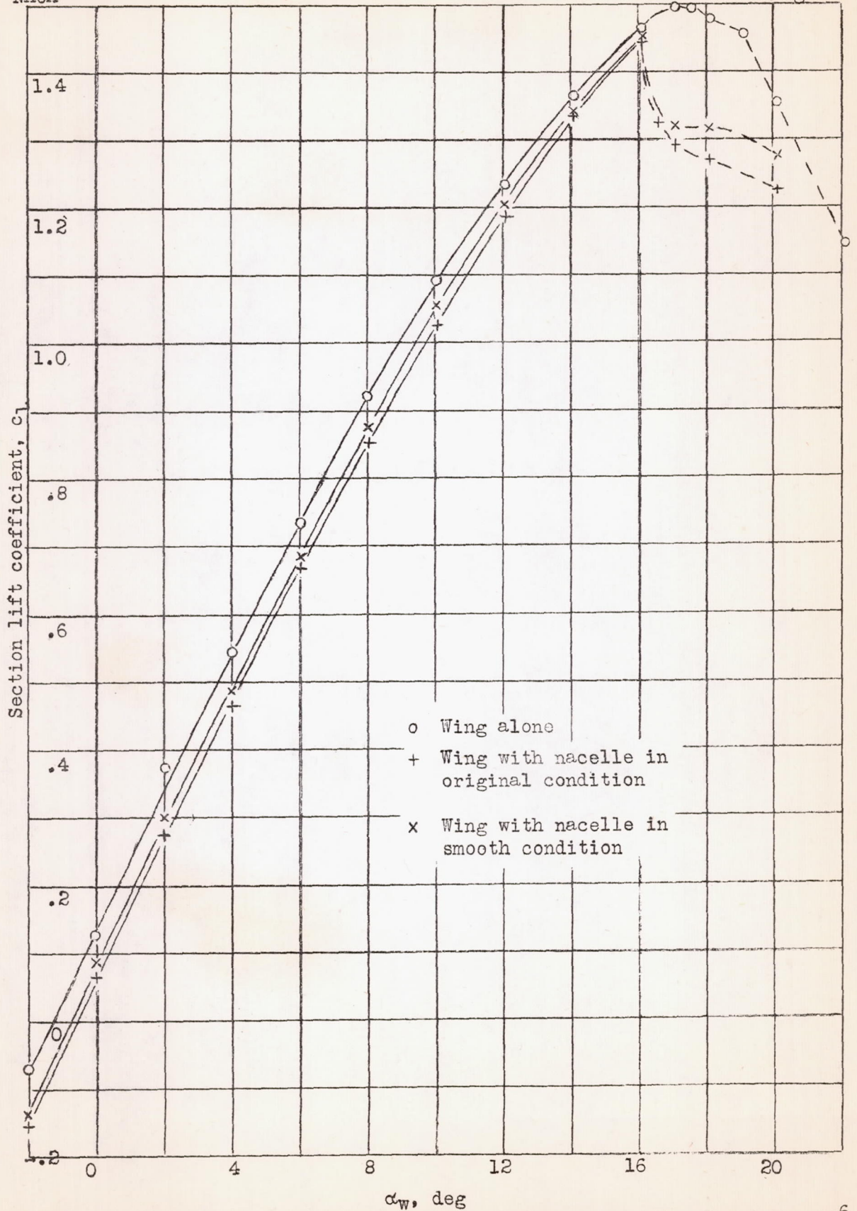
Figure 5.- Lift comparison of wing with and without nacelle. R_w, 6.5 \times 10^6 .
