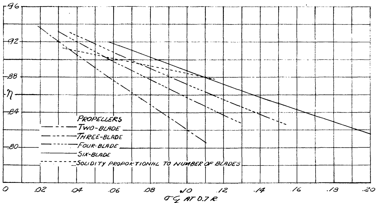
FIGURE 9.—OPTIMUM EFFICIENCY AGAINST \sigma_{c_2} AT 0.7 RADIUS FOR V/nD = 2.5 . ELEMENT 4/D_0 = 60 .
