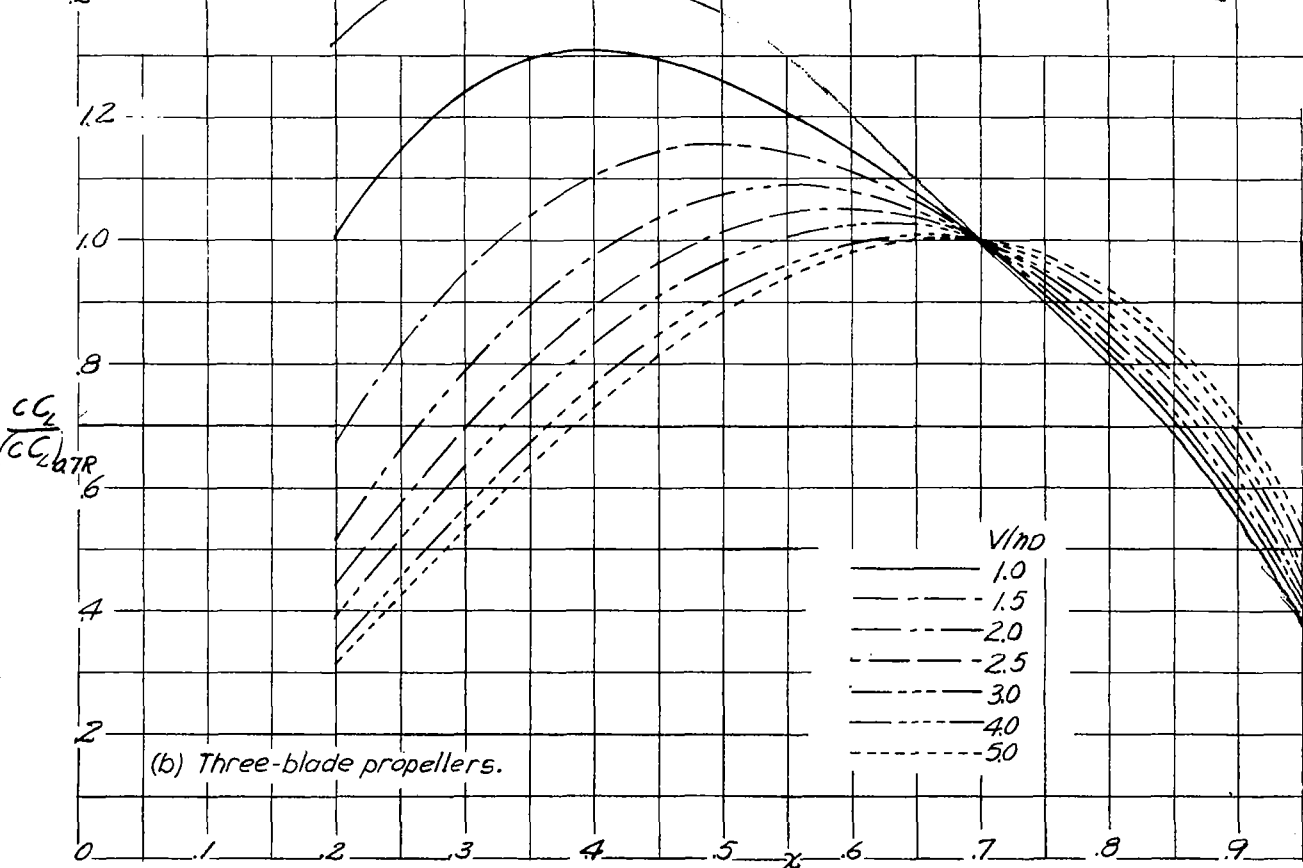
Figure 3.- Ratio of load coefficient to load coefficient at 0.7 radius for optimum load (a to d) distribution for propellers operating at several values of V/hD
