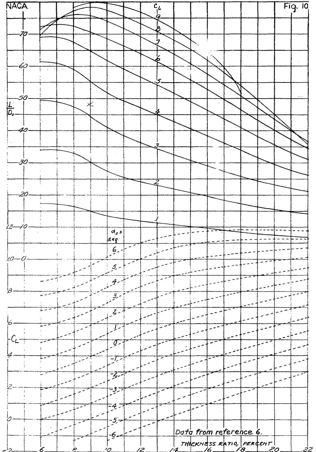
FIGURE 10.- CHARACTERISTICS OF CLARK Y AIRFOILS CORRECTED TO INFINITE ASPECT RATIO
