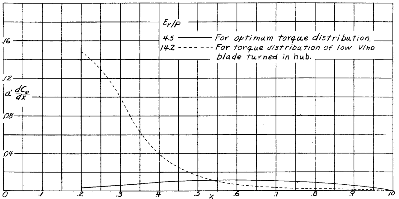
Figure 12.— Curves of d \frac{dC_g}{dx} against x . V/nd=5.0
