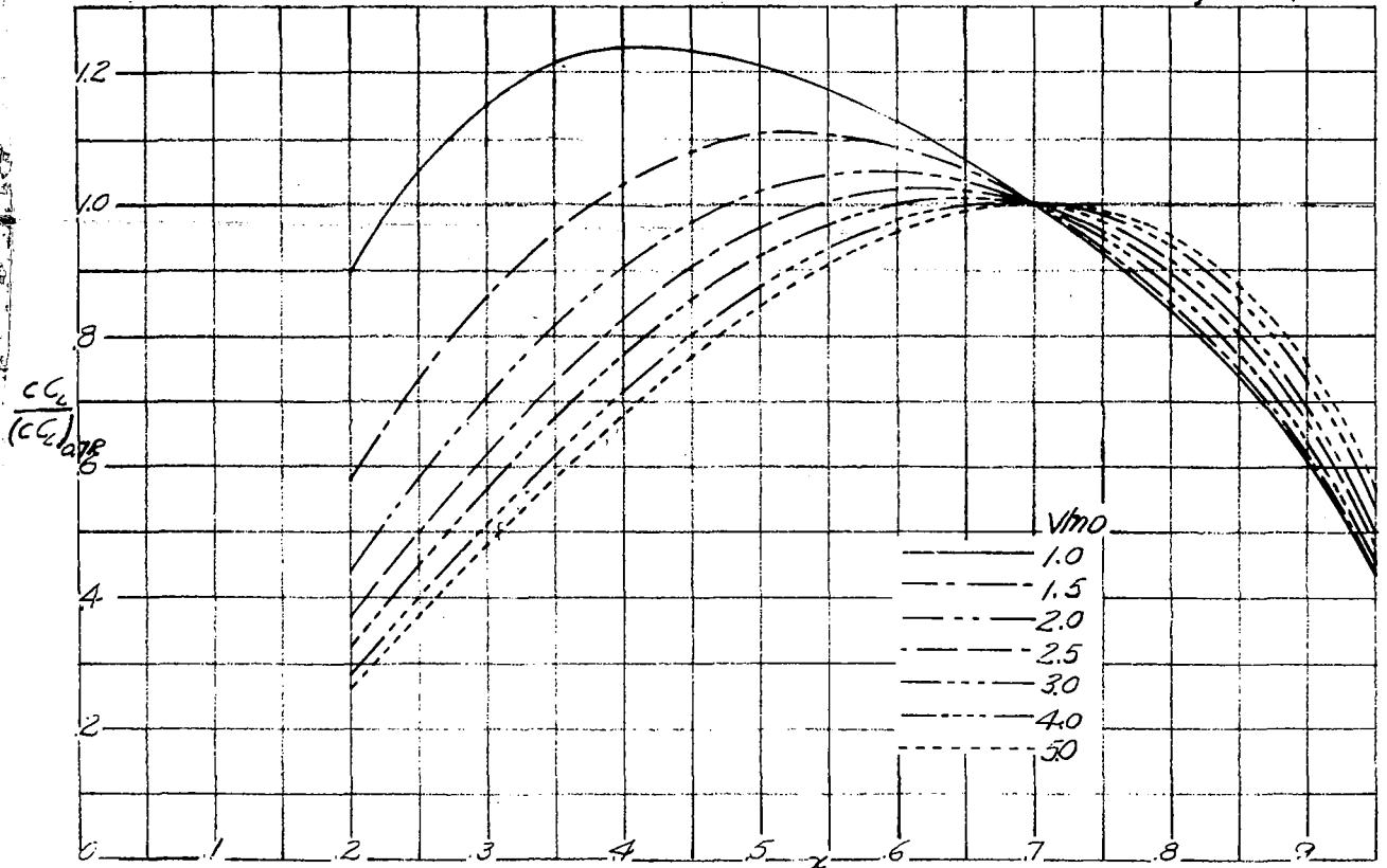
(c) FOUR-BLADE PROPELLERS. FIGURE 3.-CONTINUED
