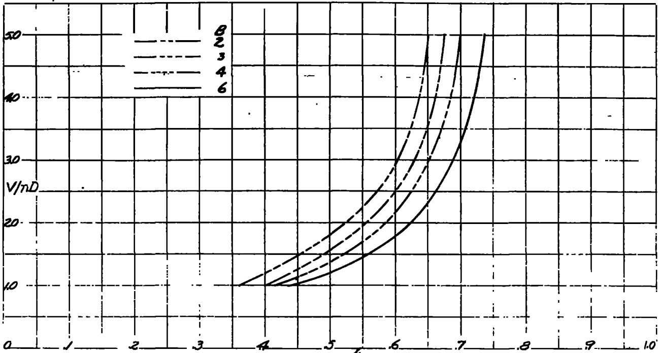
FIGURE 4.- CURVE SHOWING RADIAL LOCATION OF MAXIMUM VALUE OF ELEMENT LOAD COEFFICIENT c_Q FOR OPTIMUM THRUST DISTRIBUTION IN TERMS OF V/nD .
