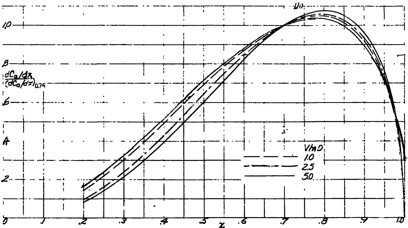
FIGURE 6.- RATIO OF dC_Q/dx TO dC_Q/dx AT 0.75 RADIUS FOR SEVERAL VALUES OF V/nD FOR A THREE-BLADE PROPELLER.
