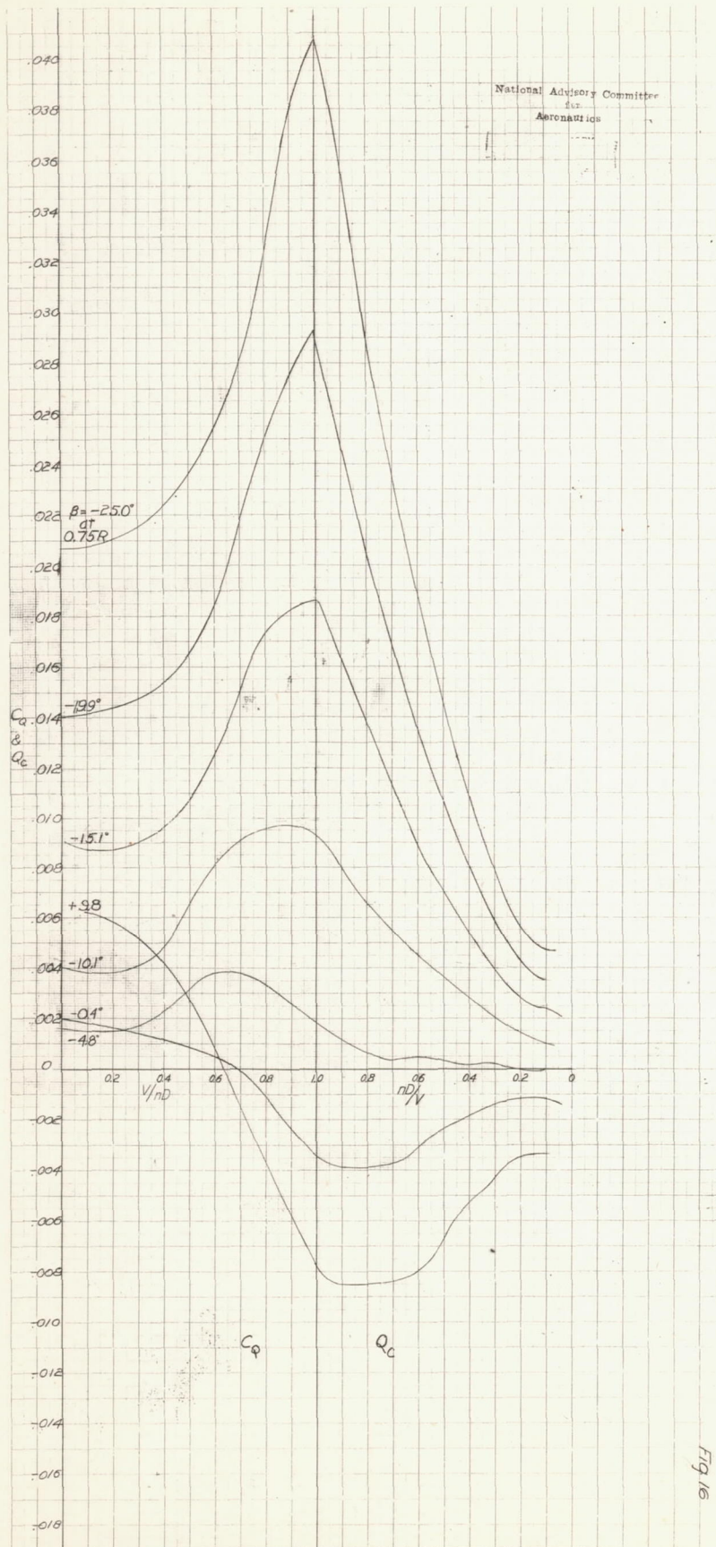
Figure 16-Torque-coefficient curves for propeller 6267 A-18, Clark Y blade section throughout
