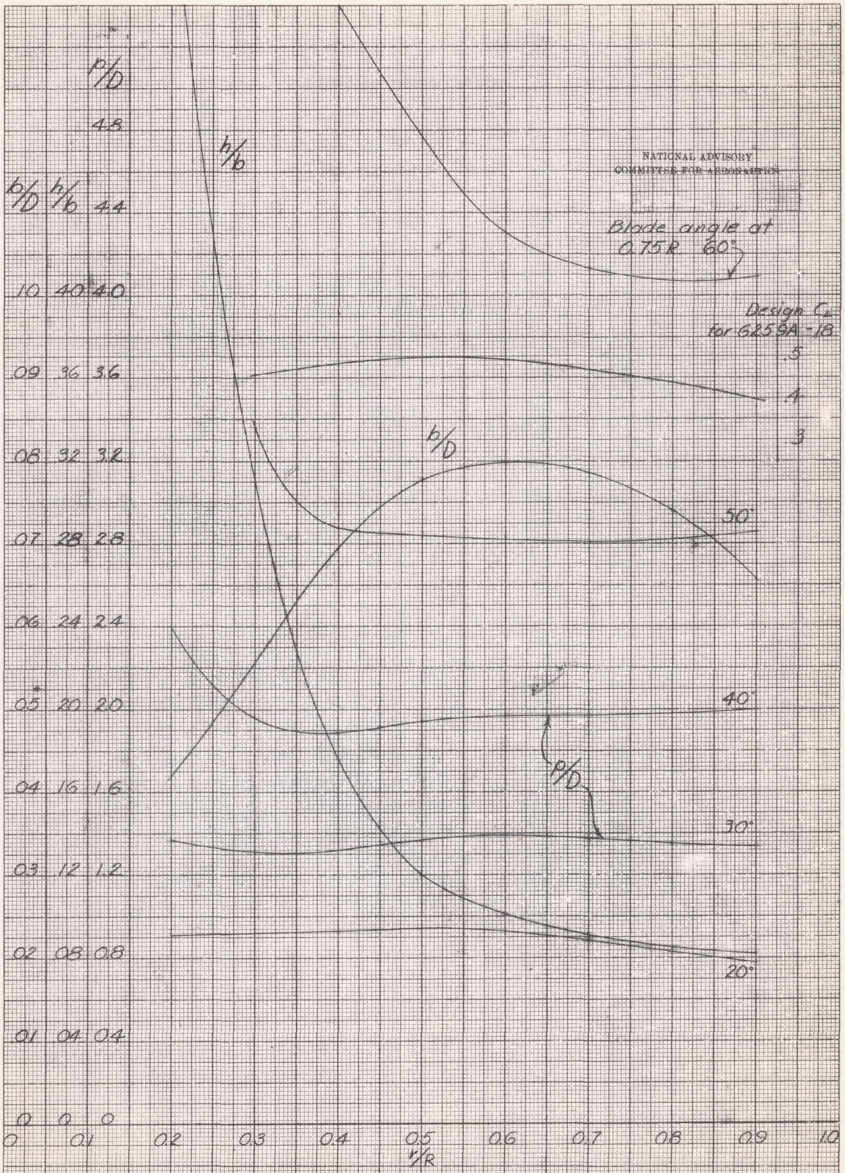
Figure 1 Blade form curves for Hamilton Standard propellers 6259A-1B & 6267A-1B. D, diameter; R, radius to tip; r, station radius; b, section chord; h, section thickness; p, geometric pitch.
