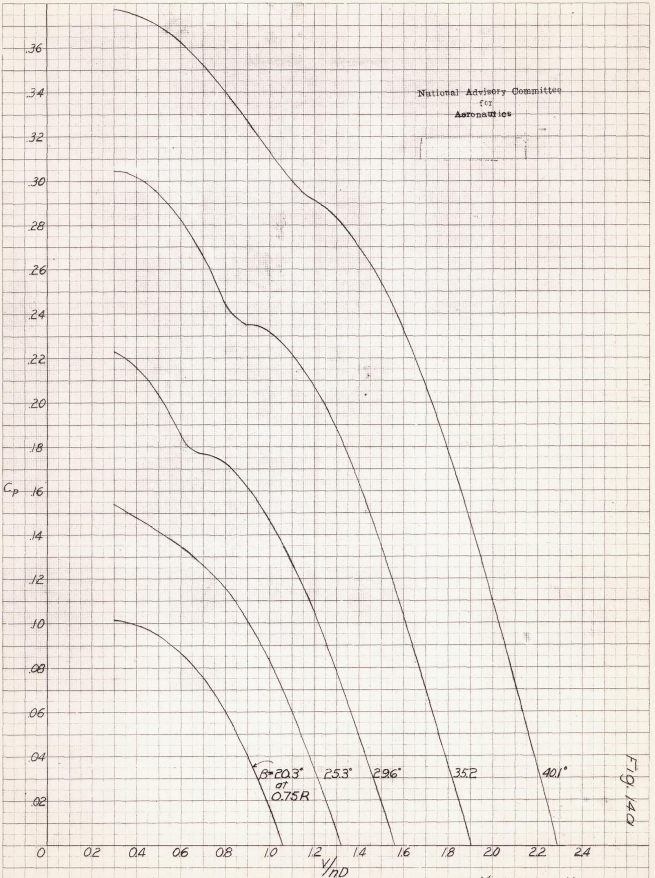
Figure 14a—Power-coefficient curves for propeller 6267A-18, Clark Y blade section throughout
