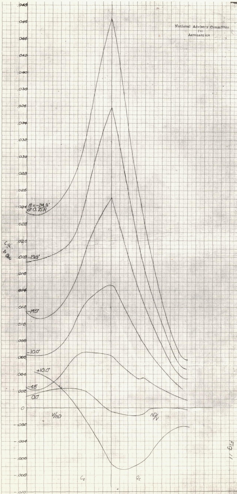
Figure 11 - Torque-coefficient curves for propeller 6259 A-18, NACA 16 blade section throughout
