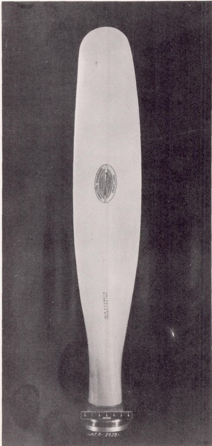
Figure 3.- Photograph showing plan form of the propeller blades tested.
