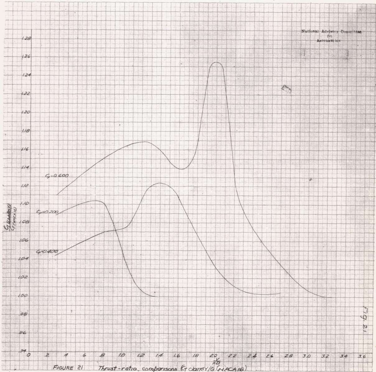
FIGURE 21 Thrust-ratio comparisons ( C_l CLARK Y/G (NACA 16))
