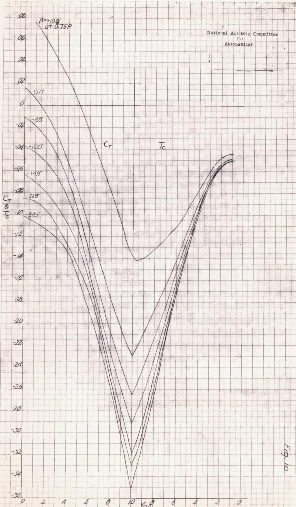
Figure 10. Thrust-coefficient curves for propeller 6259 A-18, NACA blade section throughout
