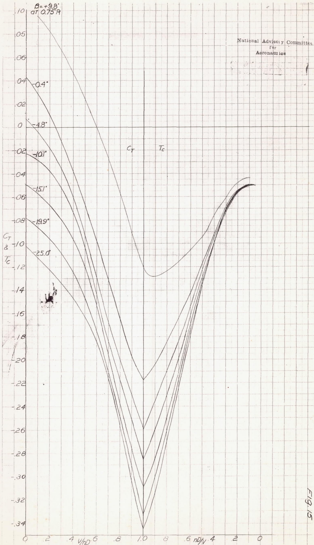
Figure 15-Thrust-coefficient curves for propeller 6267 A-18, Clark Y blade section throughout
