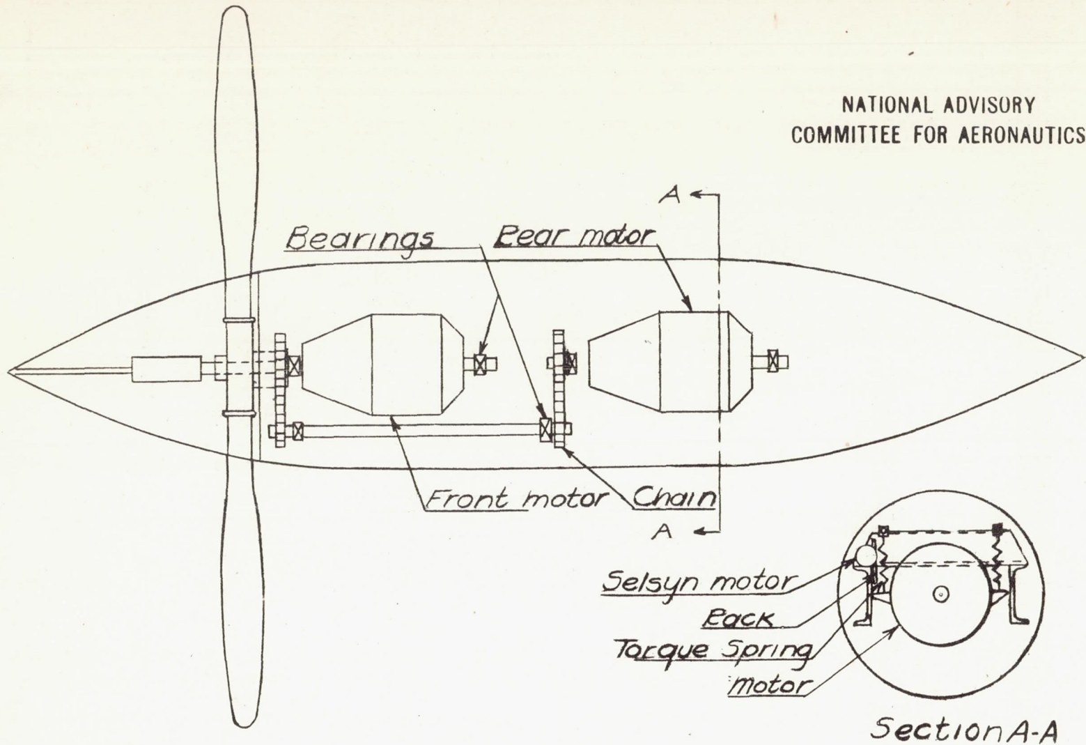
Figure 6.- propeller drive mechism.
