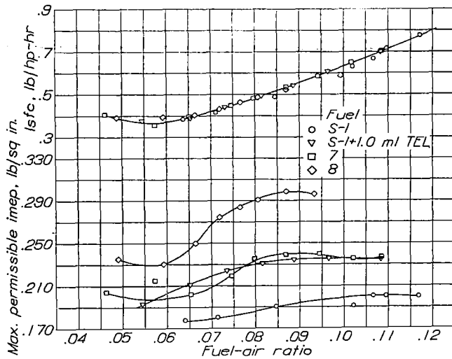
Figure 8.-Effect of fuel-air ratio on the maximum permissible performance of fuels 7,8, S-1, and S-1+1 ml TEL. Lycoming 0-1230 cylinder; engine speed, 2000 rpm; spark advance, 27°; coolant temperature, 250°F; compression ratio, 7.0; inlet-air temperature, 250°F.
