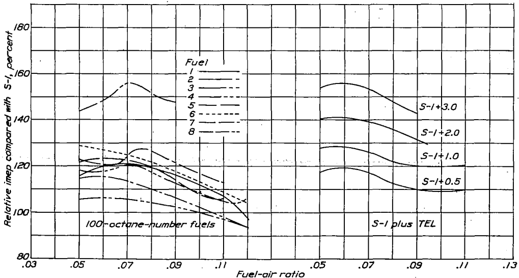
Figure 20.- Average relative indicated mean effective pressure with respect to S-1 for NACA fuels and S-1 plus tetraethyl lead.
