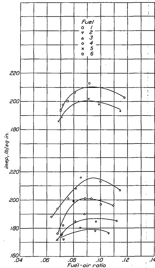
Figure 12.- Data showing relation between fuel-air ratio and maximum permissible indicated mean effective pressure for NACA fuels 1 to 6 in G.F.R. engine. (Data from Standard Oil Development Co.) Engine speed, 1800rpm; spark advance 30°; inlet-air temperature, 110°F; jacket temperature, 350°F; piston bore 2 5/8 inches; compression ratio, 6.5; engine displacement, 24.3 cubic inches.
