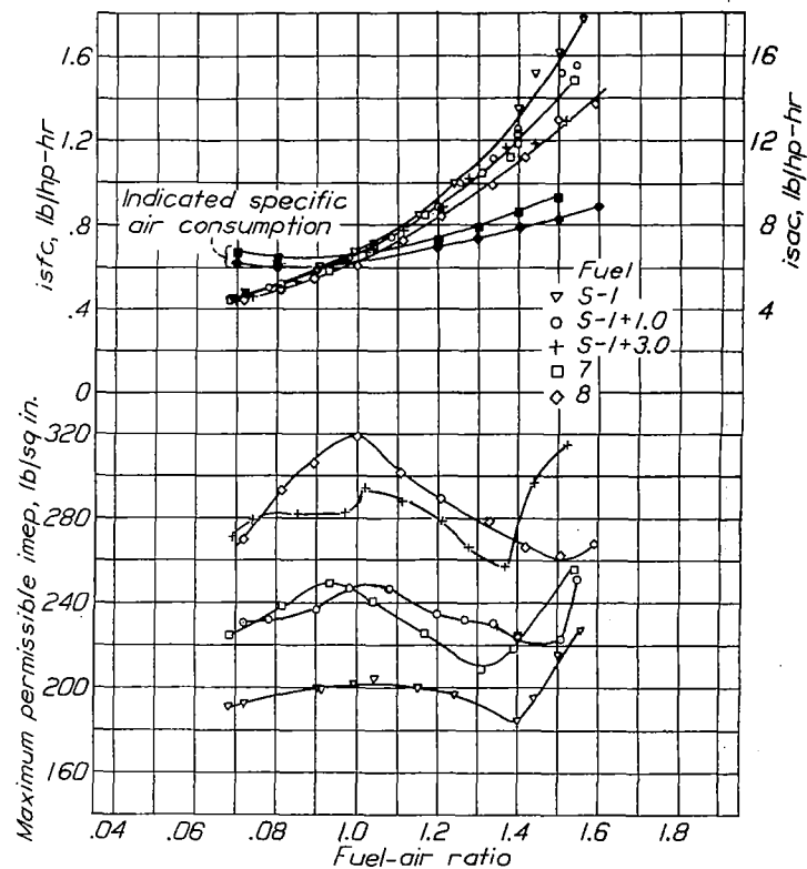
Figure 17.-Relation between estimated fuel-air ratio, maximum permissible imep, indicated specific fuel consumption, and indicated specific air consumption for S-1, S-1+1.0 ml tetraethyl lead, S-1+3.0 ml tetraethyl lead, and NACA fuels 7 and 8 in E.G.C. 17.6 cylinder. Engine speed, 2700 rpm; spark advance, 20°; inlet air temperature, 225°F; inlet coolant temperature, 240°F; compression ratio, 7.7. (Data from Ethyl Gasoline Corporation)
