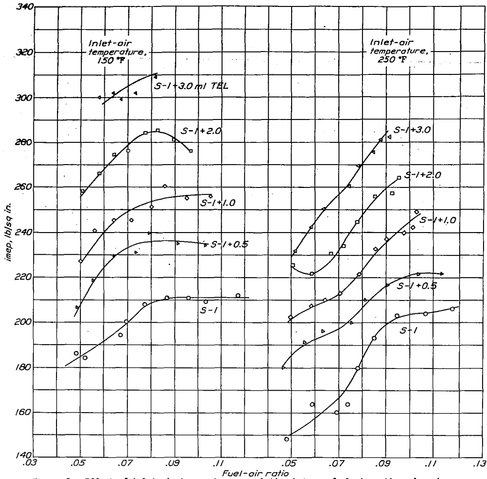
Figure 6.- Effect of inlet-air temperature on relation between fuel-air ratio and maximum permissible indicated mean effective pressure for S-1 and S-1 plus tetraethyl lead. Lycoming O-1230 cylinder; engine speed, 2000 rpm; spark advance, 27°; coolant inlet temperature, 250°F; compression ratio, 7.0.
