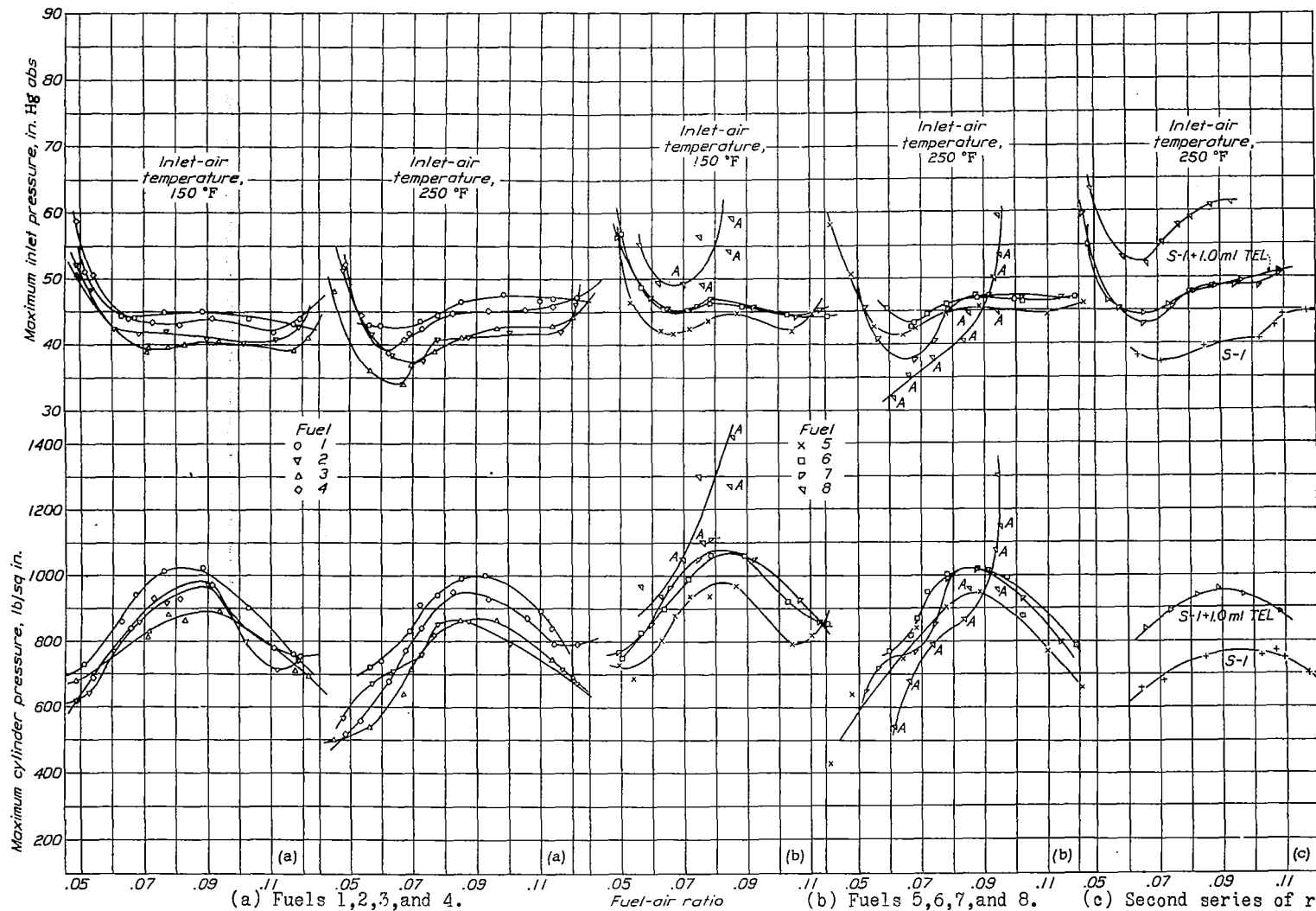
Figure 9.- Relation between fuel-air ratio and maximum permissible inlet pressure and between fuel-air ratio and maximum cylinder pressure at this inlet pressure for NACA fuels. Lycoming O-1230 cylinder; engine speed, 2000 rpm; spark advance, 27°; coolant inlet temperature, 250°F; compression ratio, 7.0.
