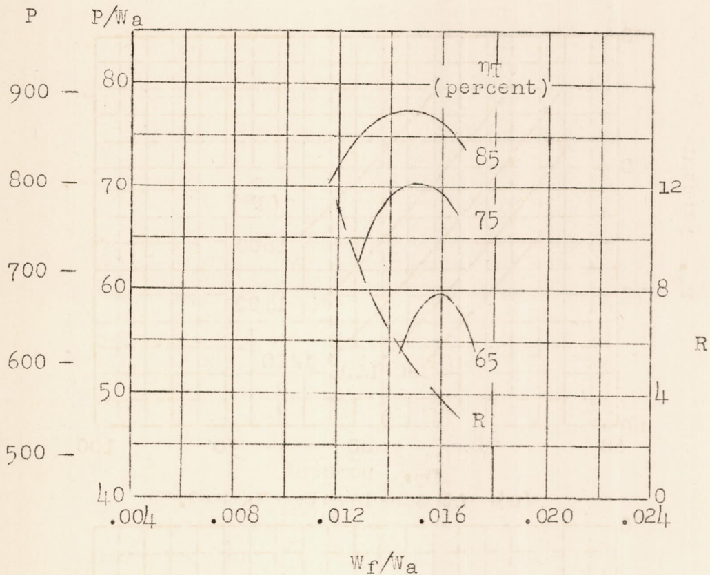
Figure 6.- Effect of fuel-air ratio on thrust power and pressure ratio. Altitude, 40,000 feet; V_0 = 880 feet per second; t_{max} = 1500^\circ F ; \eta_c = 75 percent.
