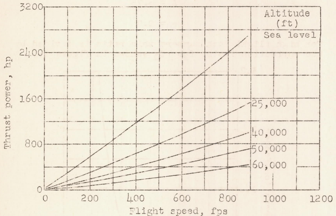
Figure 16.- Engine power output. t_{\max} = 1500^{\circ} F; \eta_c = \eta_T = 85 percent.
