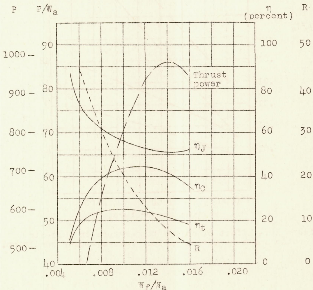
Figure 11.- Changes in thermal, jet, and over-all efficiencies and thrust power with fuel-air ratio. Altitude, 40,000 feet; V_0 = 880 feet per second; \eta_c = \eta_T = 85 percent.
