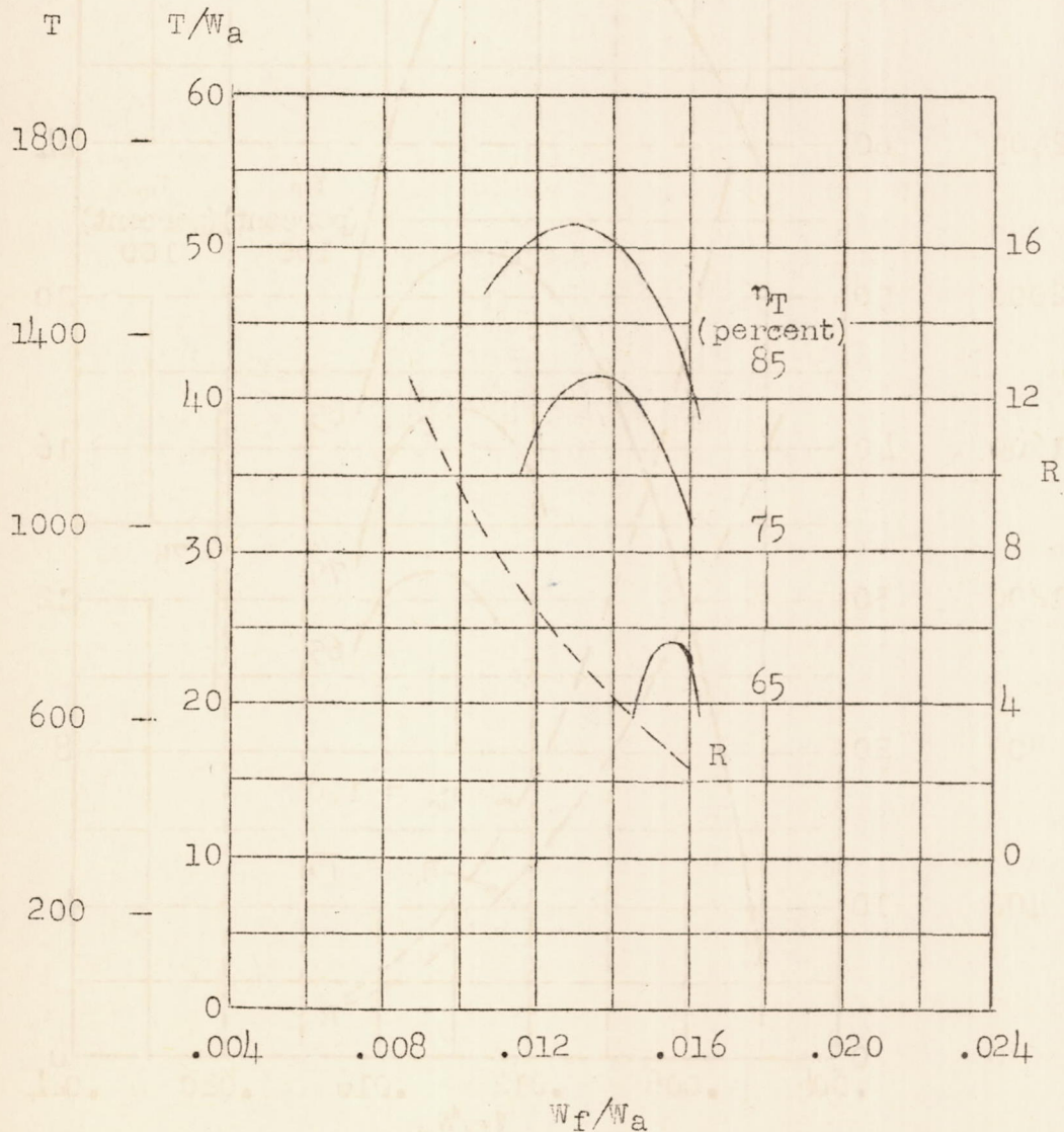
Figure 4.- Effect of fuel-air ratio on thrust and pressure ratio. At sea level; V_0 = 0 ; t_{max} = 1500^\circ F ; \eta_c = 75 percent.
