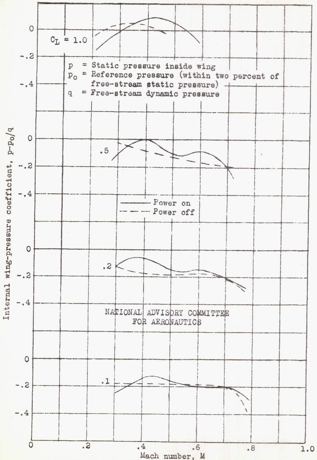
Figure 22.- Variation of wing internal-pressure coefficient with Mach number. P-39N-1 airplane.
