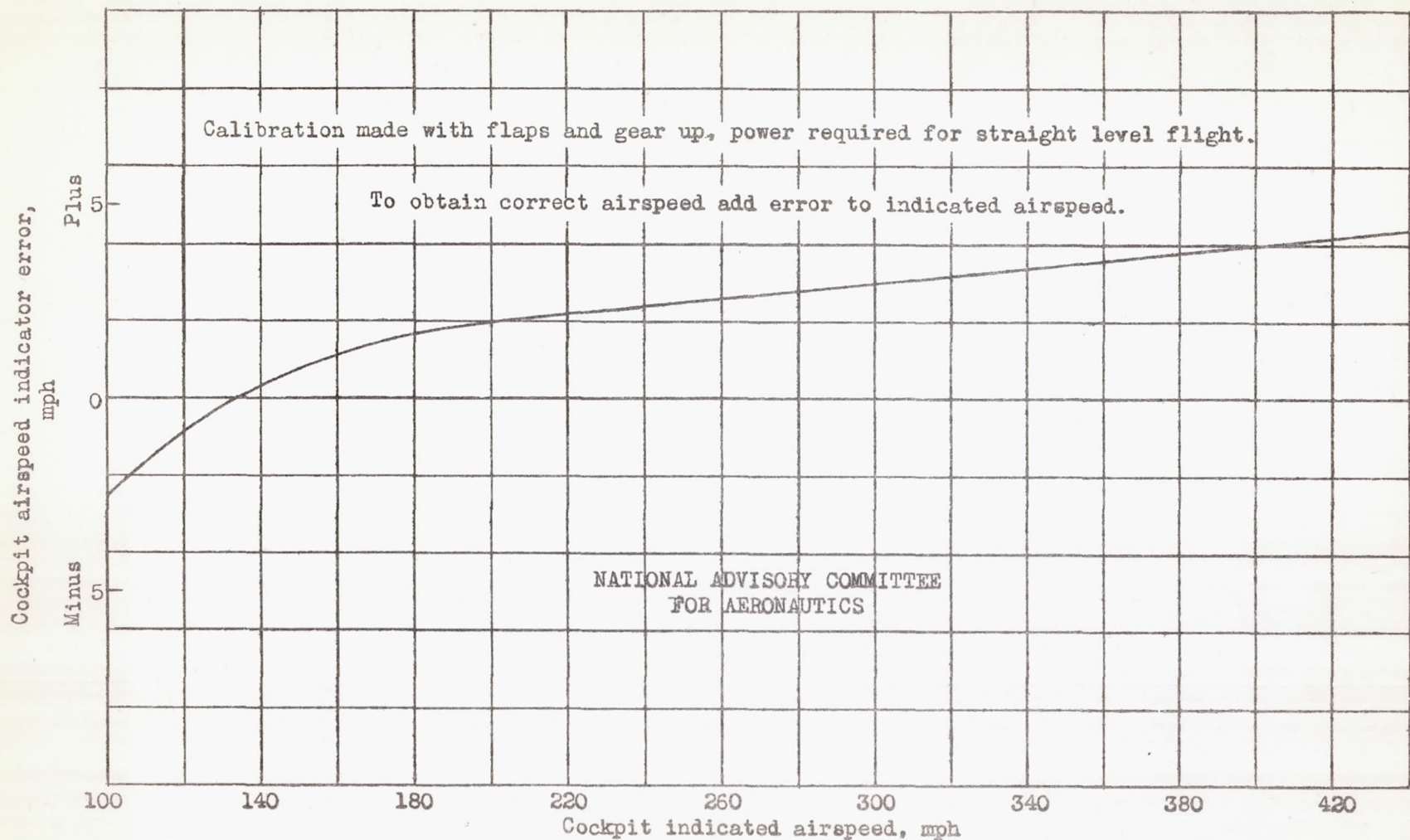
Figure 6.- Calibration of service airspeed-measuring system. P-39N-1 airplane.
