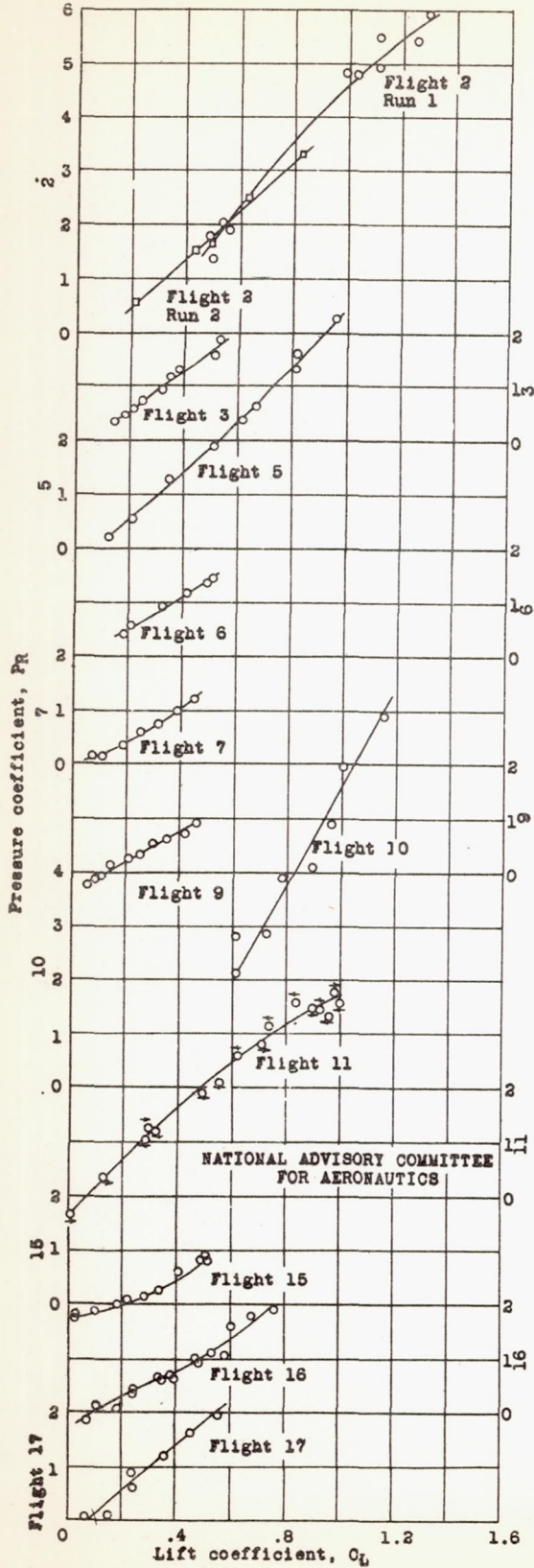
Figure 12.- Variation of resultant pressure coefficient for orifice station B-3 with airplane lift coefficient during the power-on test flights. P-39N-1 airplanes.
