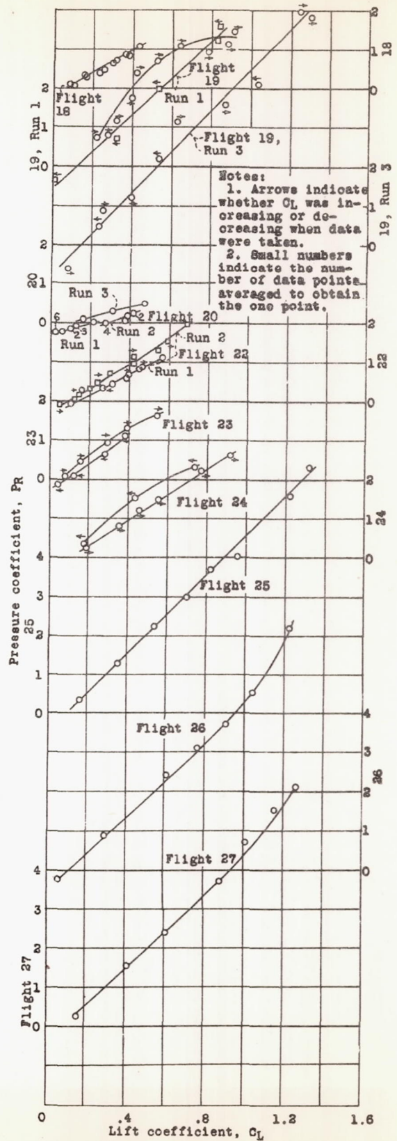
Figure 12.- Variation of resultant pressure coefficient for orifice station B-3 with airplane lift coefficient during the power-on test flights. P-39N-1 airplanes.
