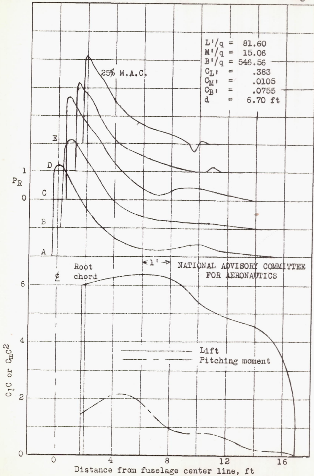
Figure 16.- Concluded. (v) Lift coefficient = 1.0, Mach number = .65. P-39N-1.
