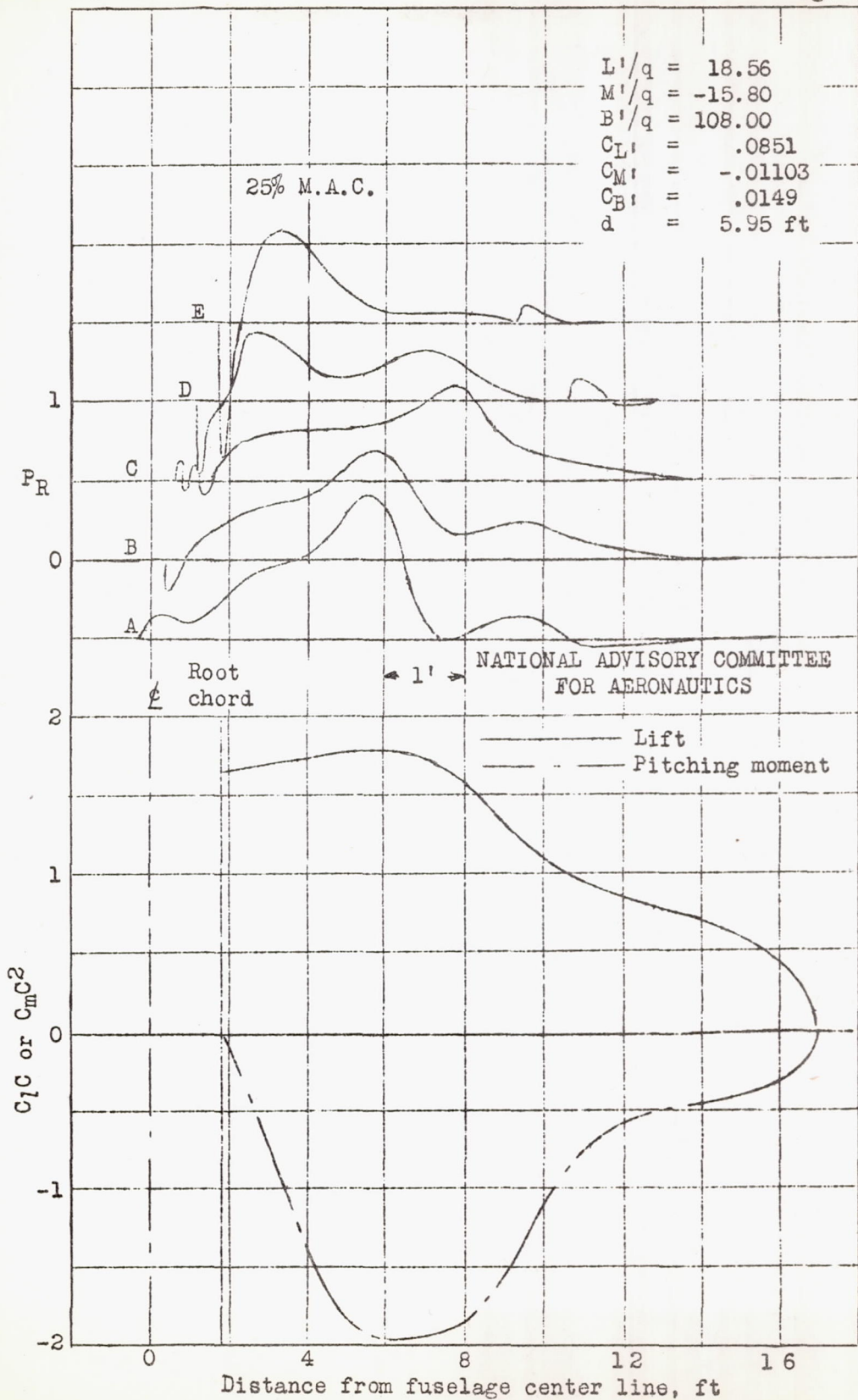
Figure 15.- Continued. (1) Lift coefficient = .20, Mach number = .78. P-39N-1.
