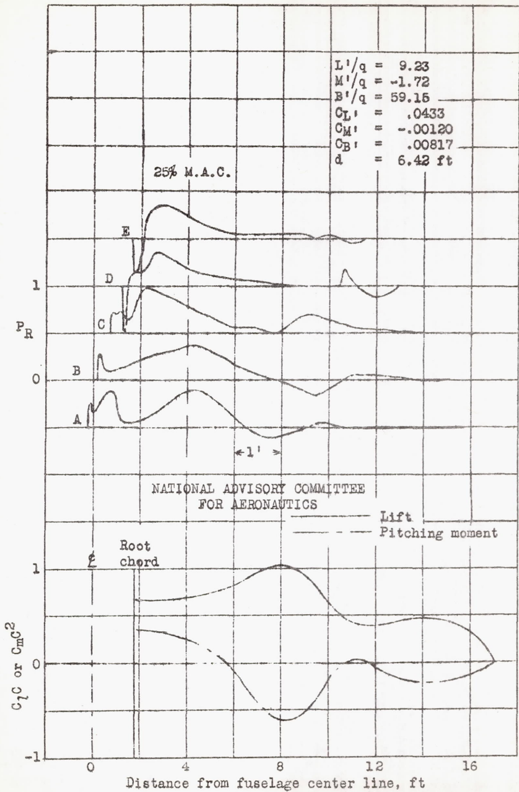
Figure 16.- Pressure distribution on the right wing in power-off flight. P-39N-1 airplane. (a) Lift coefficient = .10, Mach number = .30.
