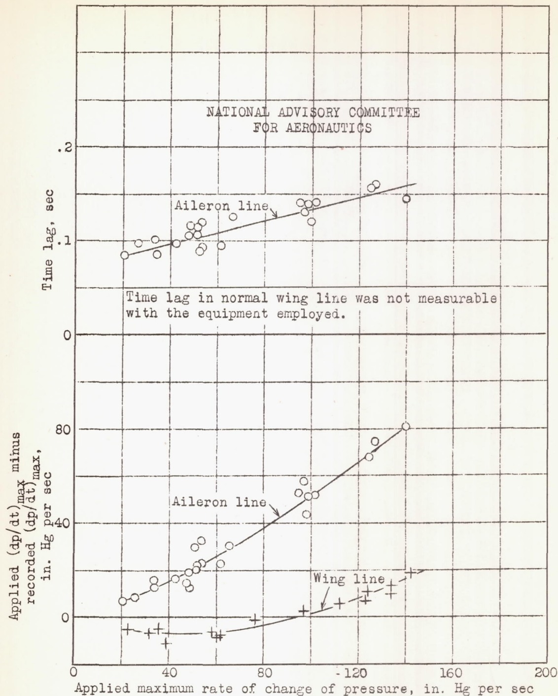
Figure 25.- Lag in typical wing pressure lines. F-39N-1 airplane.
