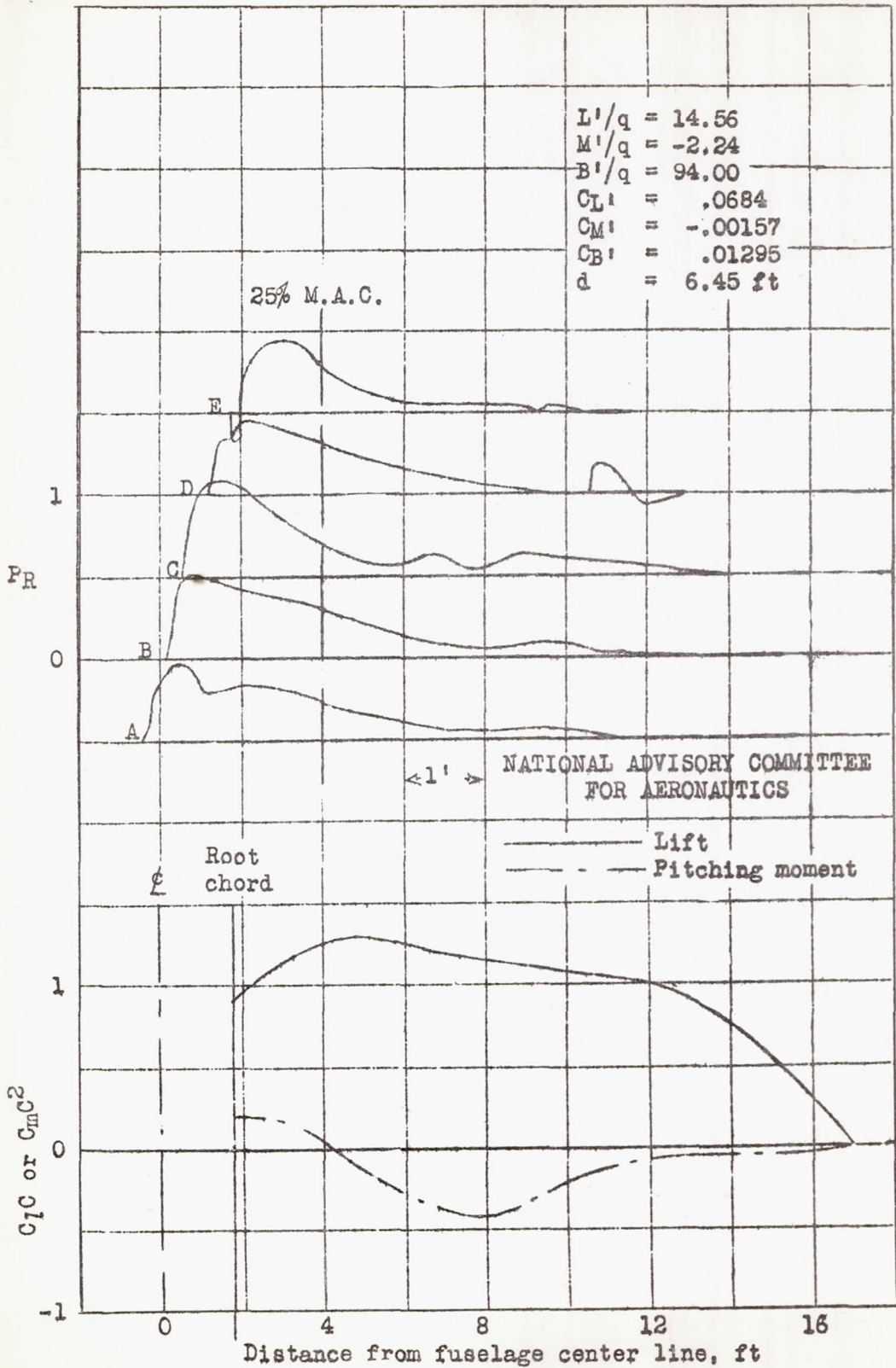
Figure 15.- Continued. (i) Lift coefficient = .20, Mach number = .50. P-39N-1.
