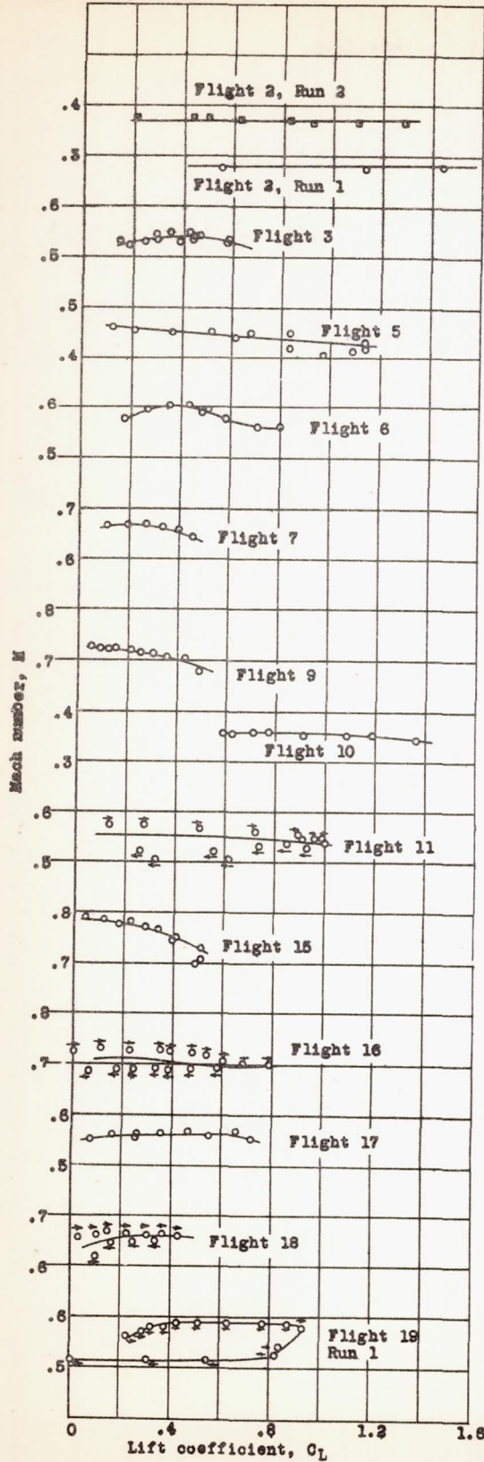
Figure 13.-Variation of Mach number with airplane lift coefficient during the power-on test flights. P-39W-1 airplane.
