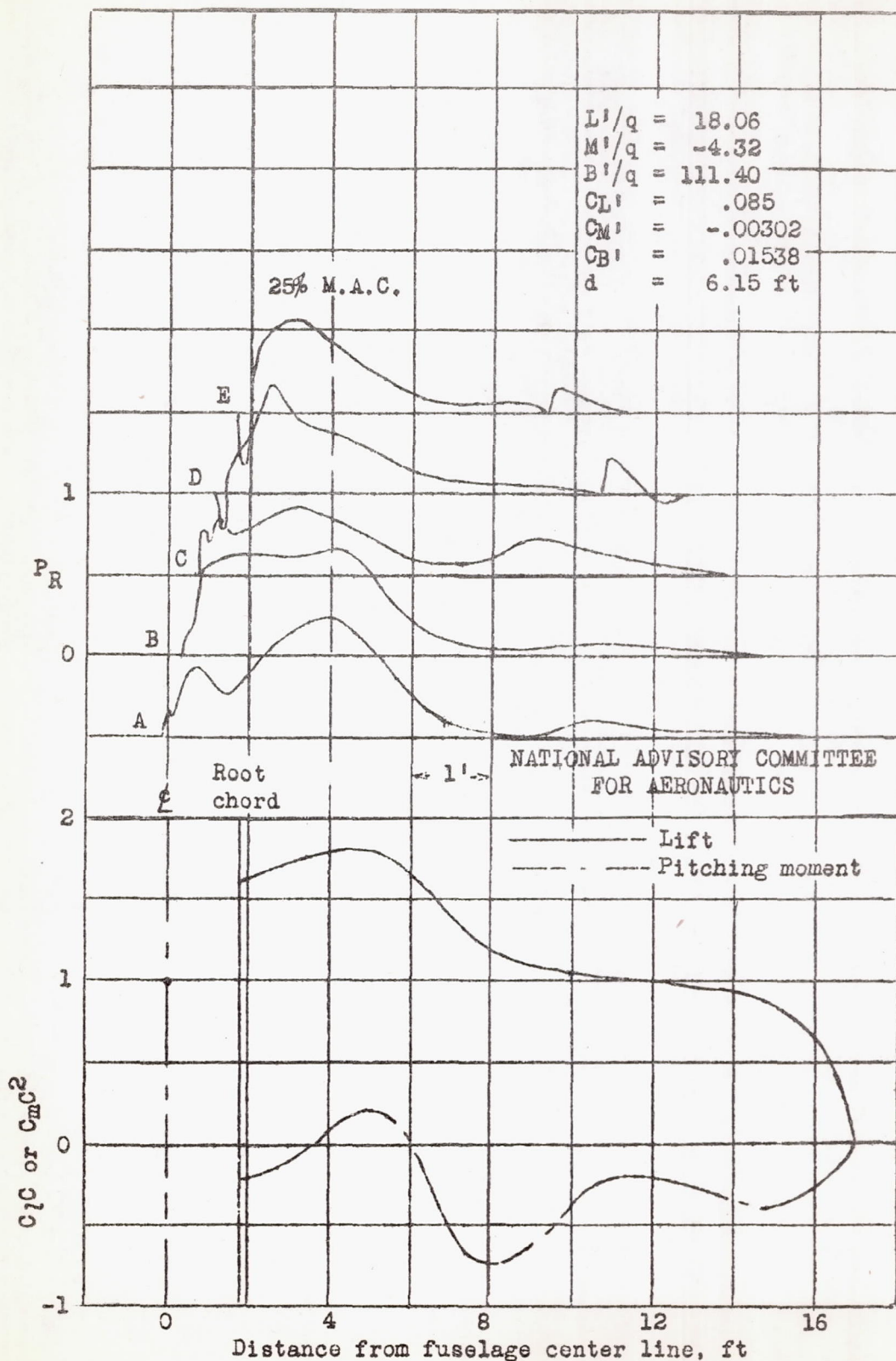
Figure 16. Continued. (k) Lift coefficient = .20, Mach number = .70, P-39N-1.
