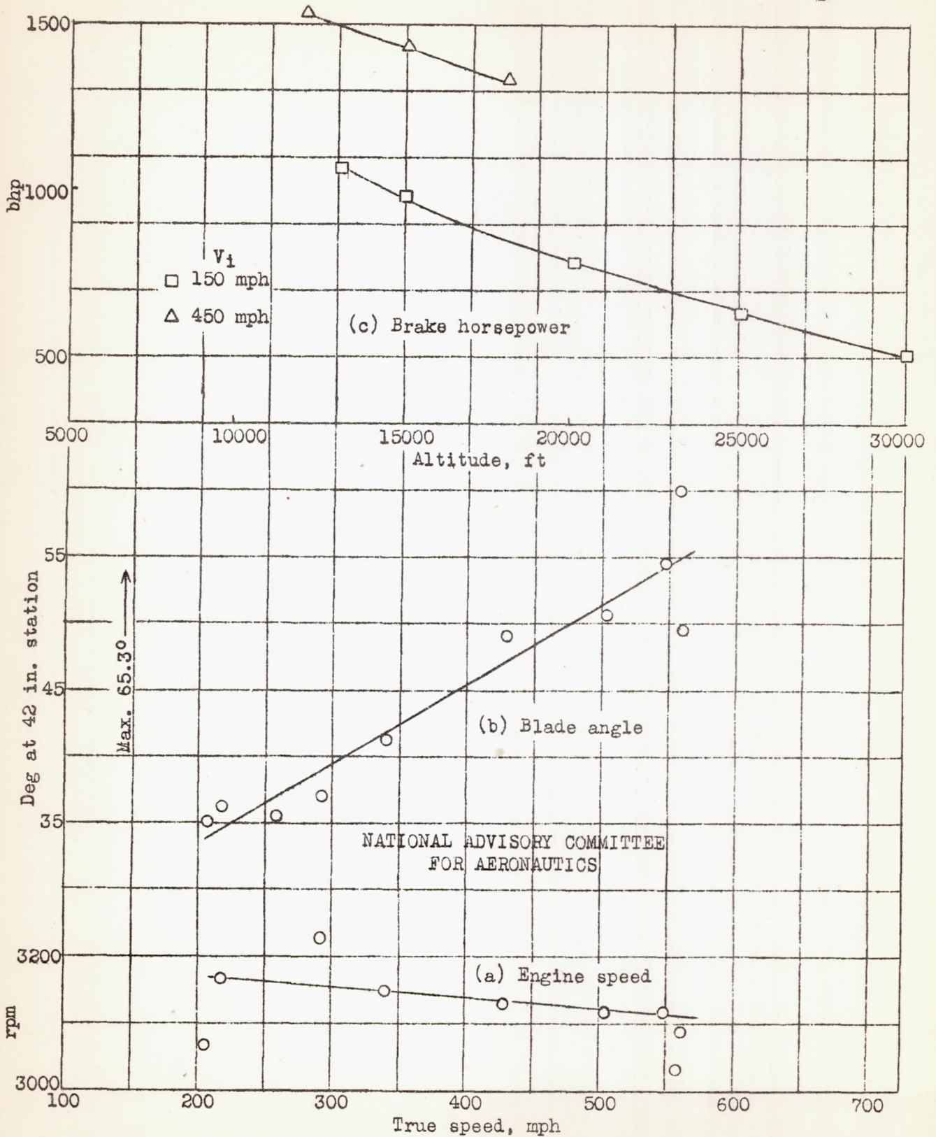
Figure 11.- Engine speed, propeller-blade angle, and brake horsepower for a power setting of full throttle and 3000 rpm. P-39M-1 airplane.
