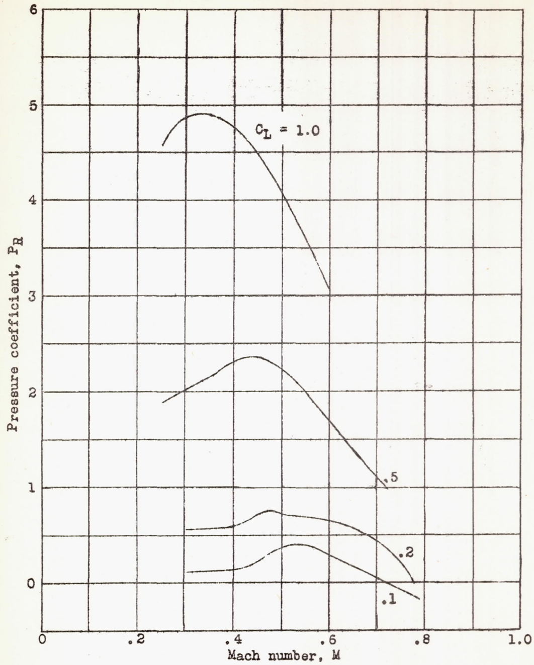
Figure 14.- Variation of resultant pressure coefficient with Mach number for orifice B-3, as measured in power-on flight. P-39N-1 airplane.
