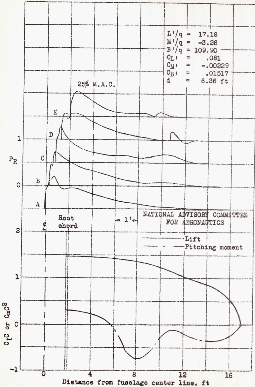
Figure 16.- Continued. (i) Lift coefficient = .20, Mach number = .50. F-39N-1.
