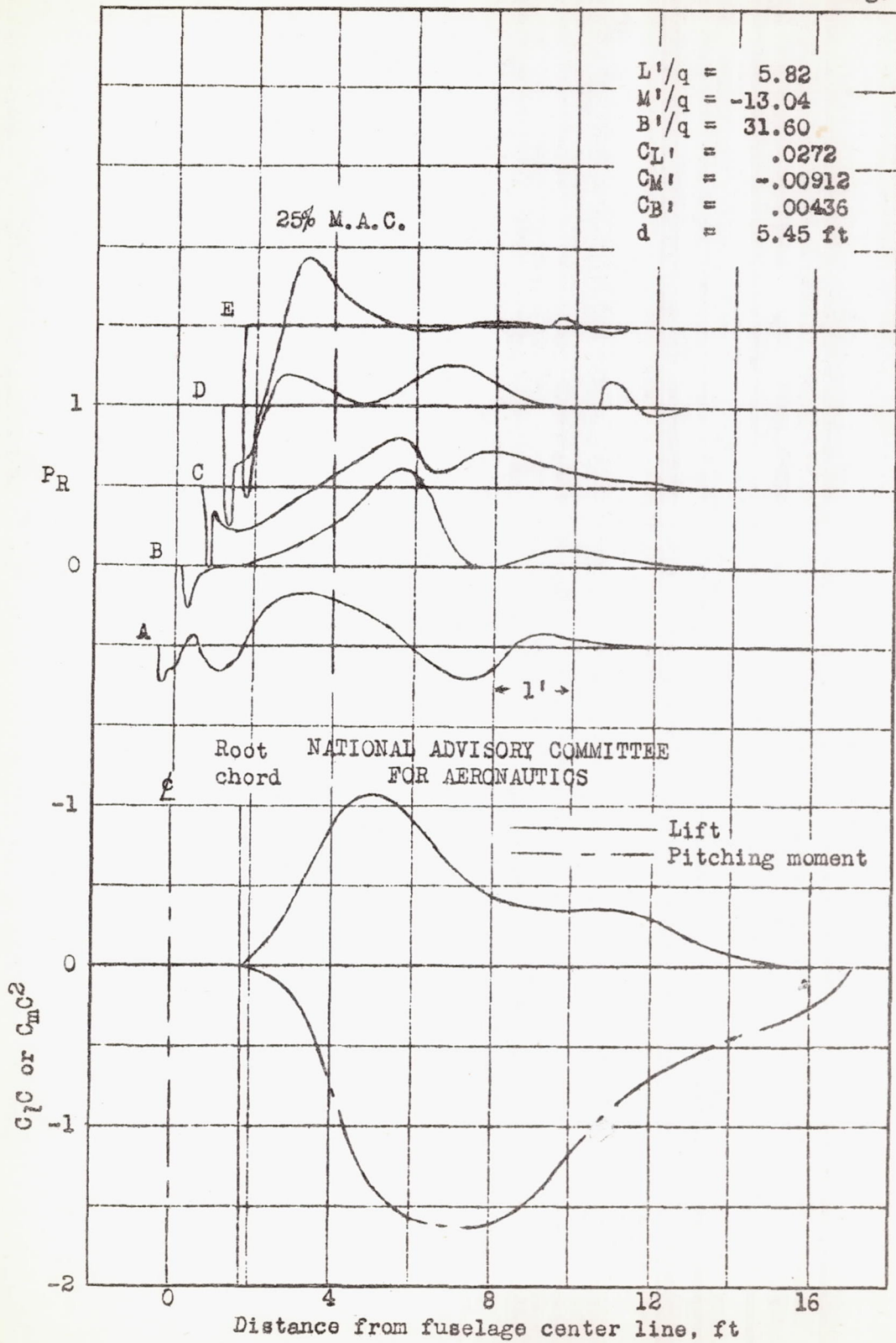
Figure 16.- Continued. (f) Lift coefficient = .10, Mach number = .78. P-39N-1.
