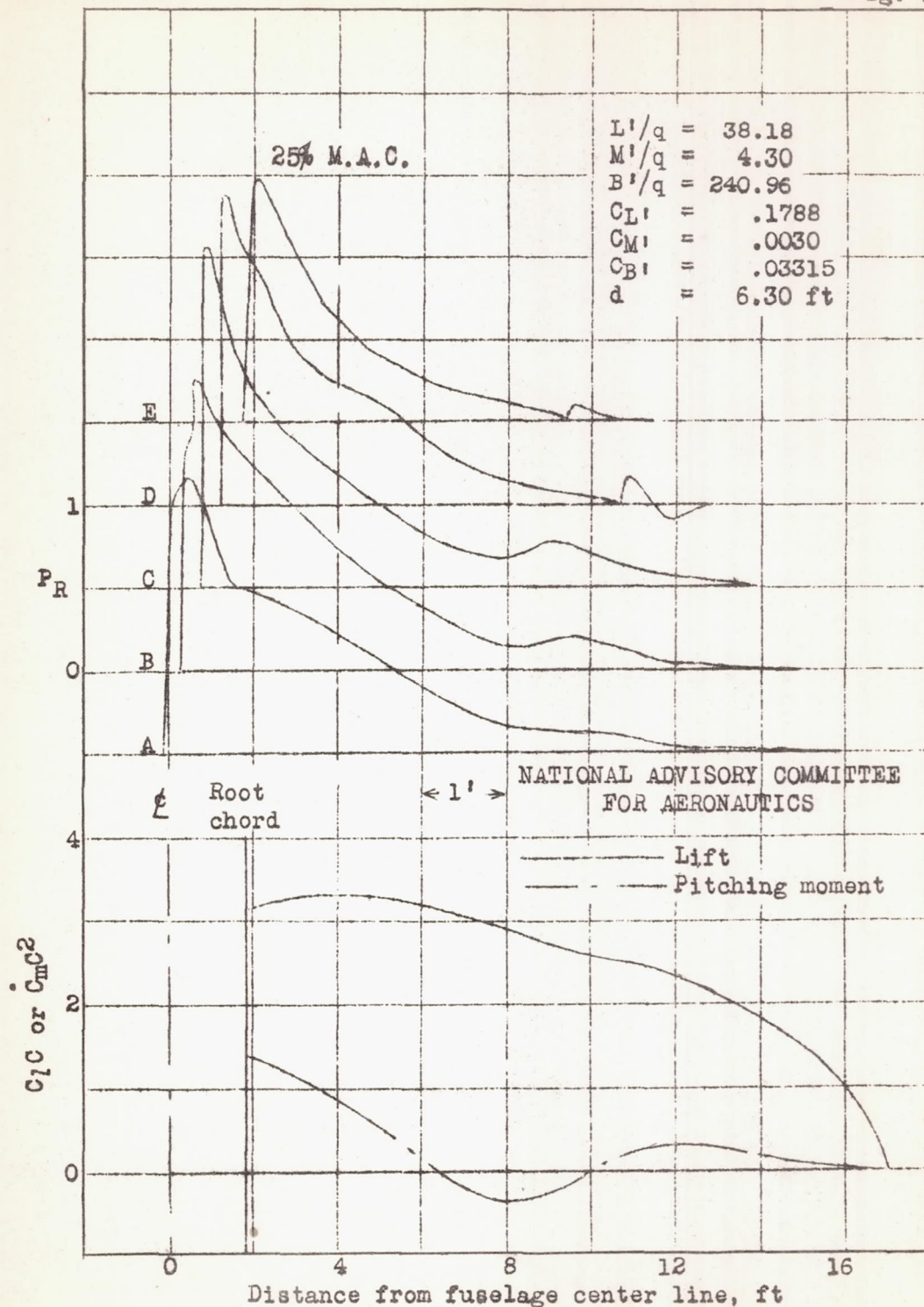
Figure 15.- Continued. (o) Lift coefficient = .50, Mach number = .50. P-39N-1.
