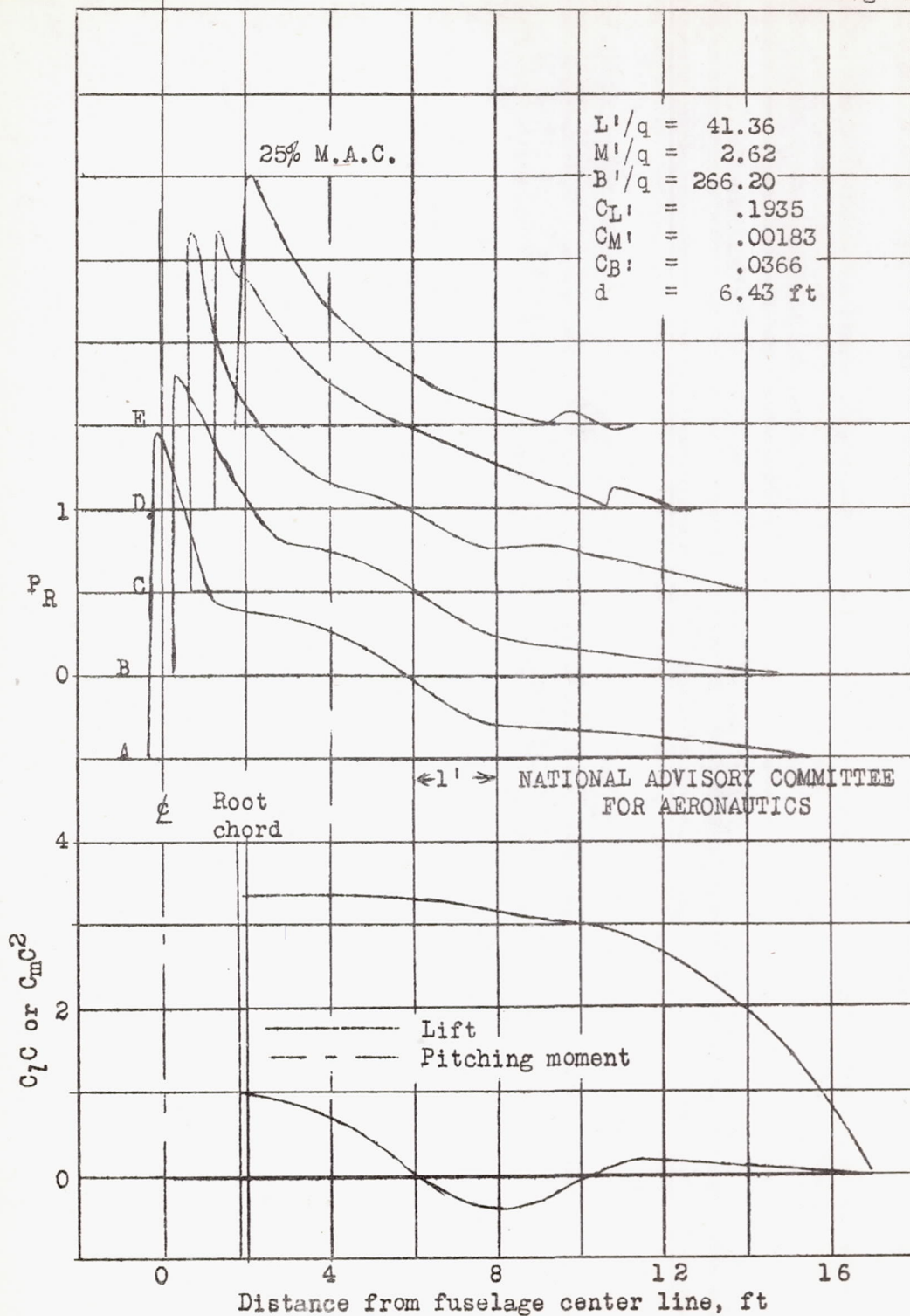
Figure 15.- Continued. (m) Lift coefficient = .50, Mach number = .30. P-39N-1.
