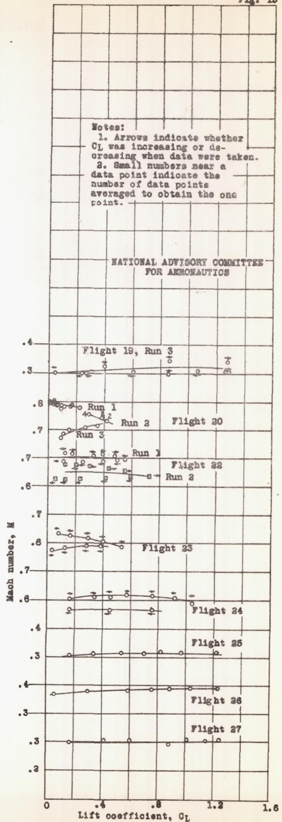
Figure 13.-Variation of Mach number with airplane lift coefficient during the power-on test flights. P-39W-1 airplane.
