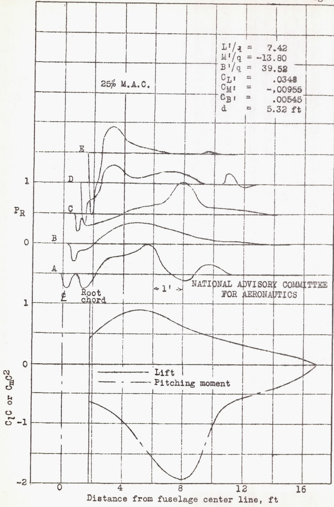
Figure 15.- Continued. (f) Lift coefficient = .10, Mach number = .78. P-39N-1.
