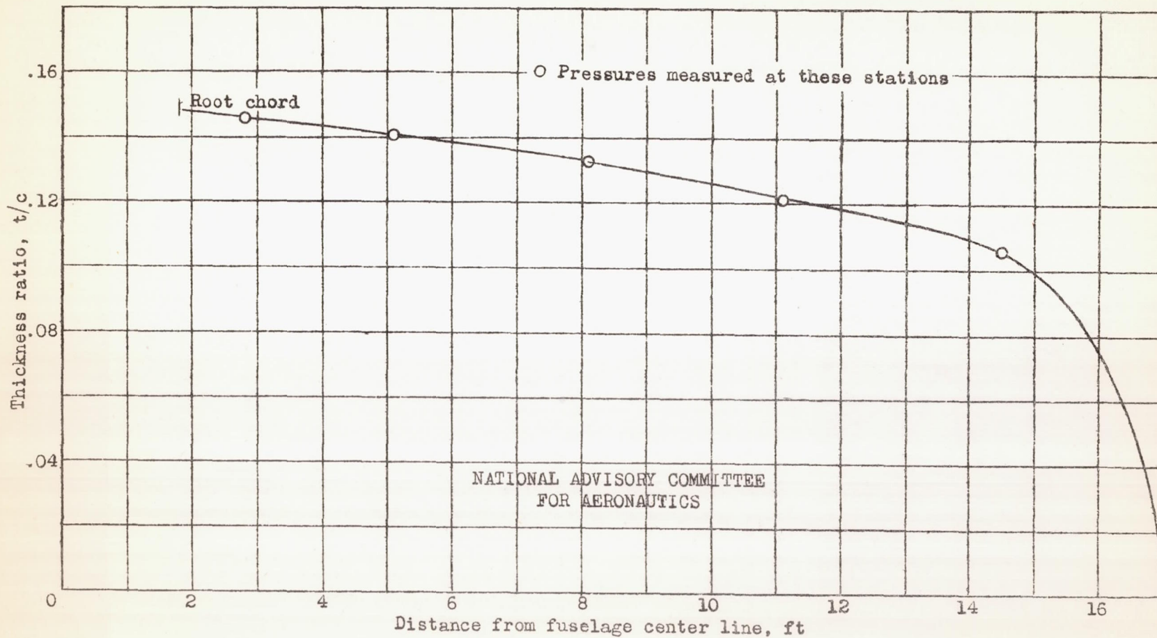
Figure 4.- Variation of thickness ratio along span of right wing. P-39N-1 airplane.
