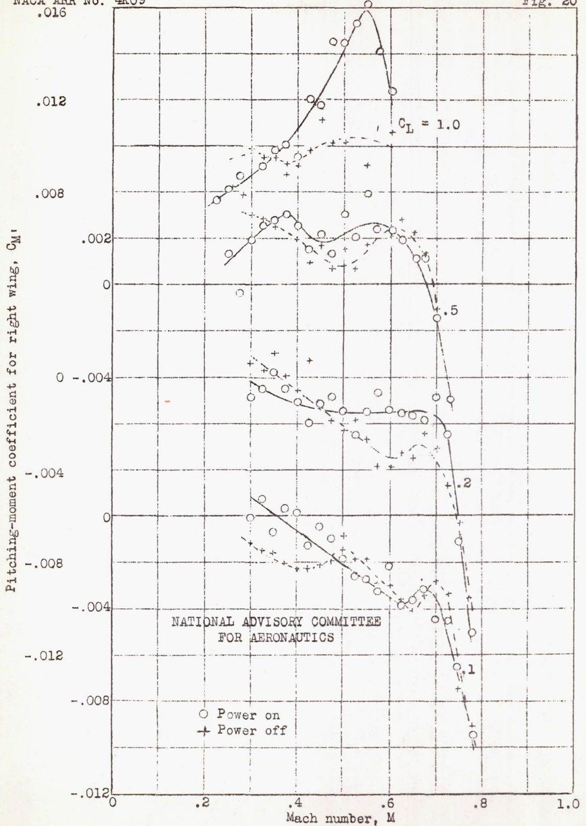
Figure 20.- Variation of right-wing-panel pitching-moment coefficient with Mach number. P-39N-1 airplane.
