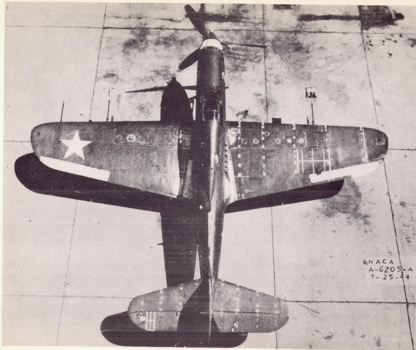
Figure 2.- Top view, P-39N-1 airplane as instrumented for flight tests.
