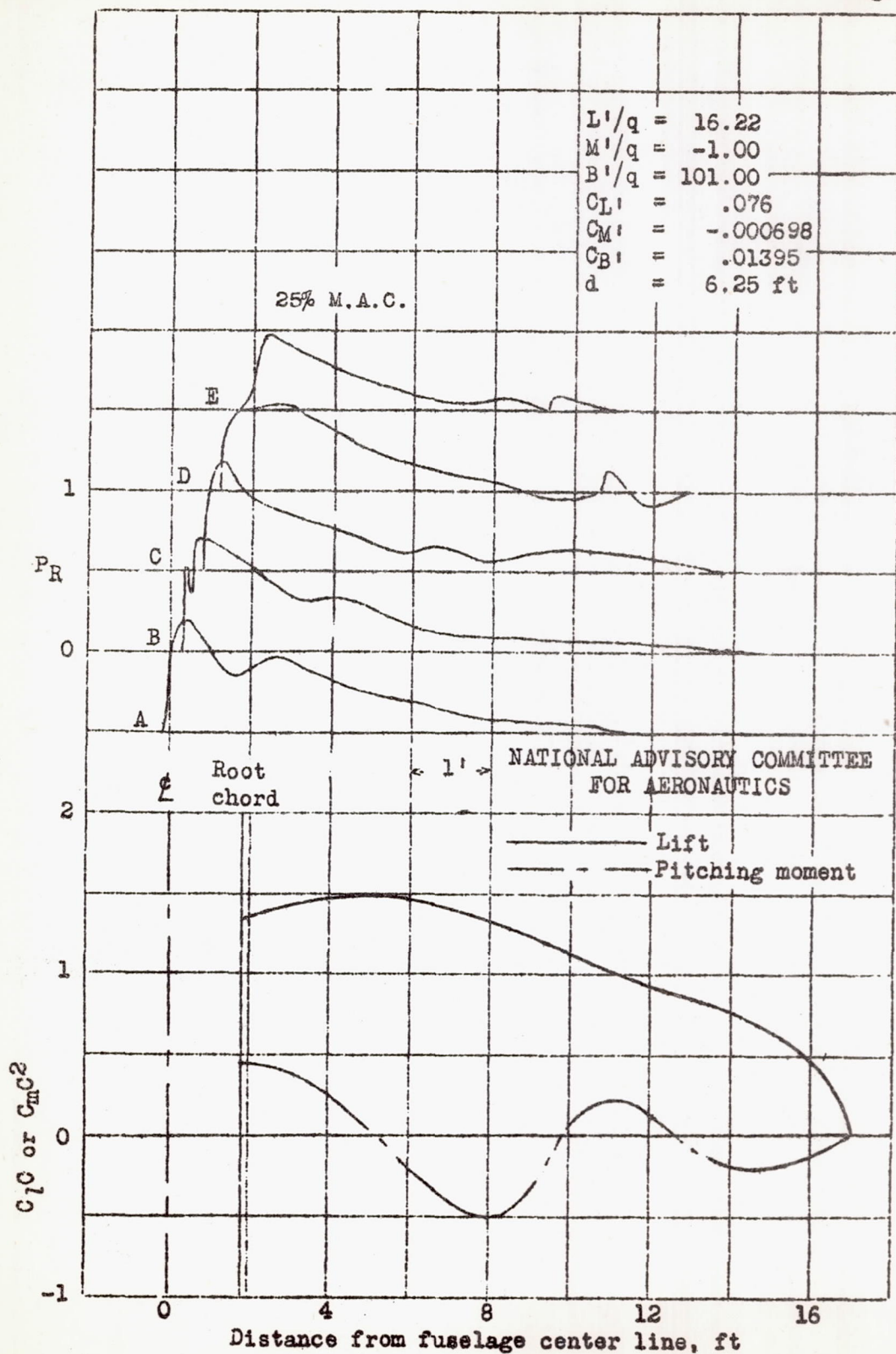
Figure 16.- Continued. (h) Lift coefficient = .20, Mach number = .40. P-39N-1.
