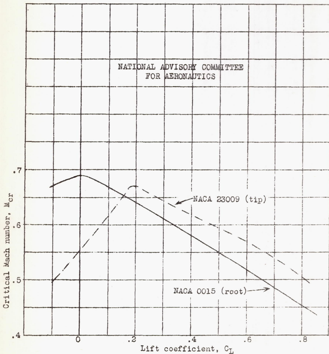
Figure 21.- Calculated values of critical Mach number for the specified root and tip wing sections on the P-39N-1 airplane.
