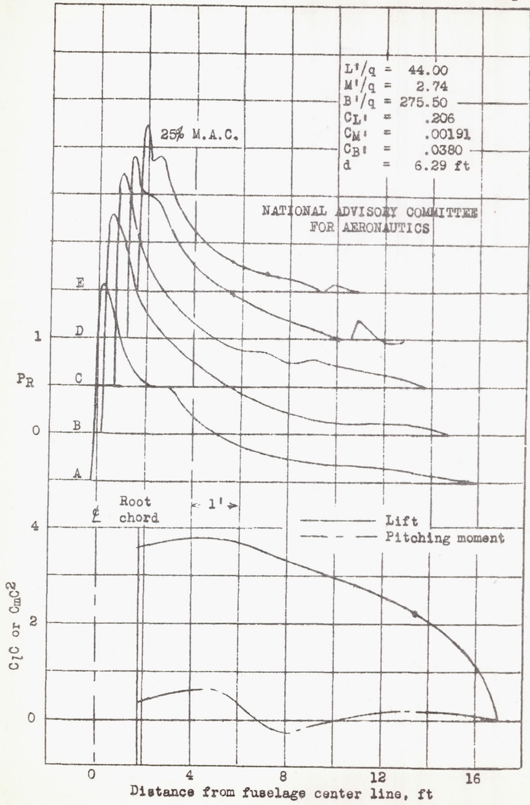
Figure 16.- Continued. (n) Lift coefficient = .50, Mach number = .40. P-39N-1.
