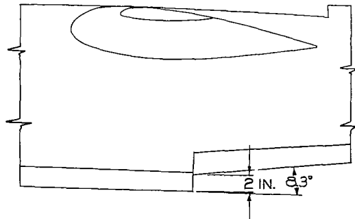
WING INCIDENCE OF BASIC MODEL DECREASED 2.5° AND ANGLE OF AFTERBODY KEEL INCREASED 1.5° DEPTH OF STEP = 2 IN (0.14 BEAM). MODEL 134C
