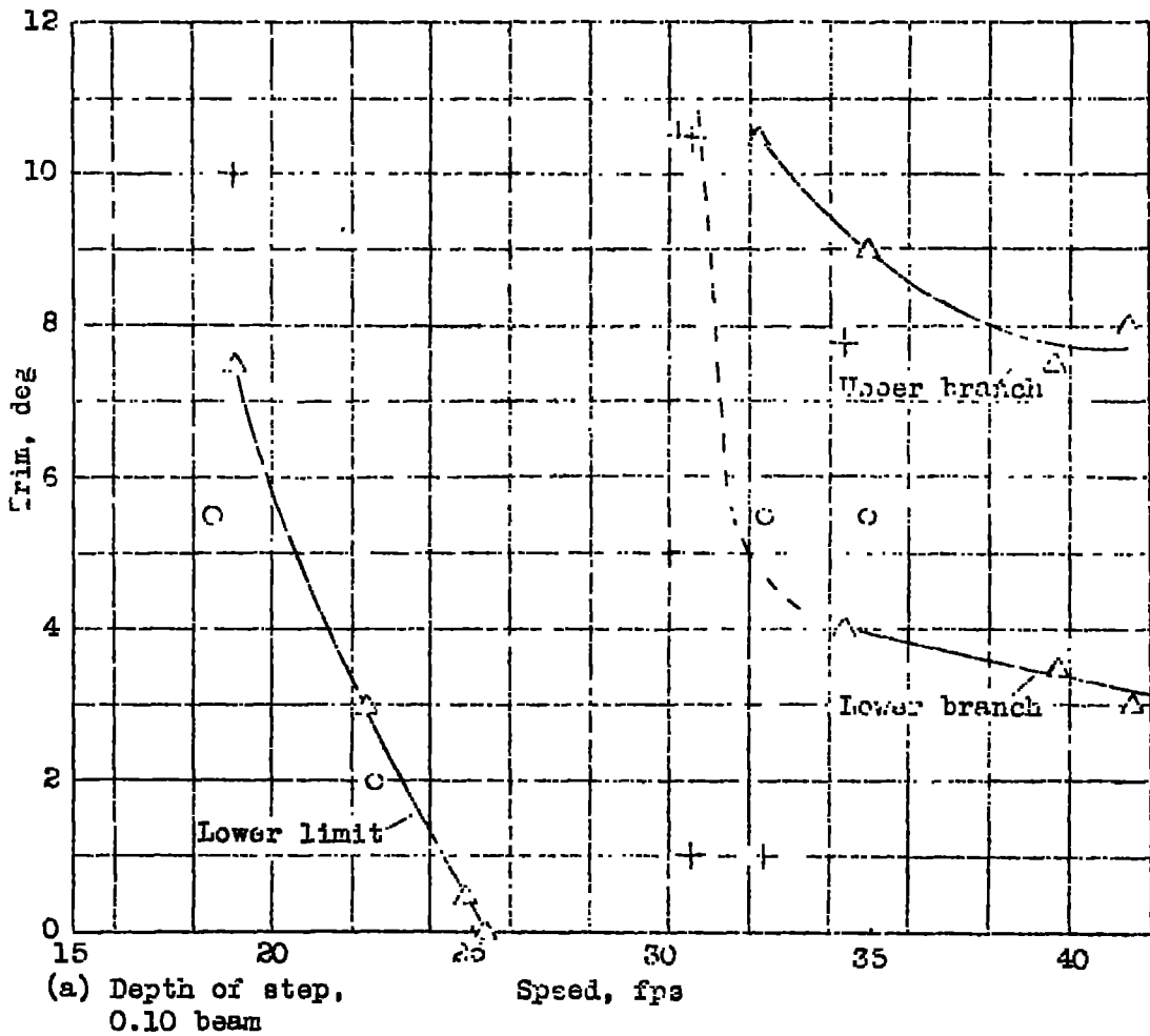
Figure 7 (a,b).- Model 134PF-2. Variation of trim limits with speed. C_{\Delta 0} = 0.87 .
