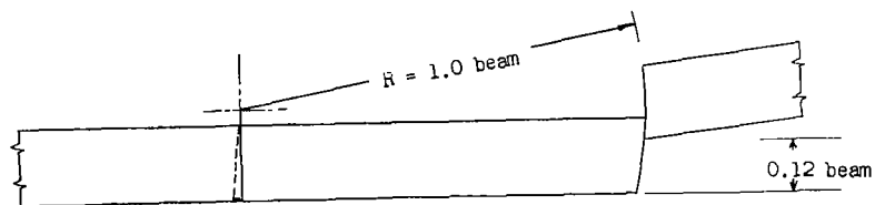
(b) Flap deflected to form step.
