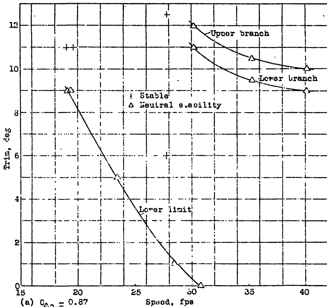
Figure 8 (a,b).-- Model 134PF-3. Variation of trim limits with speed. Depth of step = 0.14 beam.
