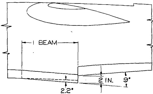
BASIC MODEL WITH PLANING FLAP. DEPTH OF STEP INCREASED TO 2 IN (0.14 BEAM). MODEL 134-PF-3
