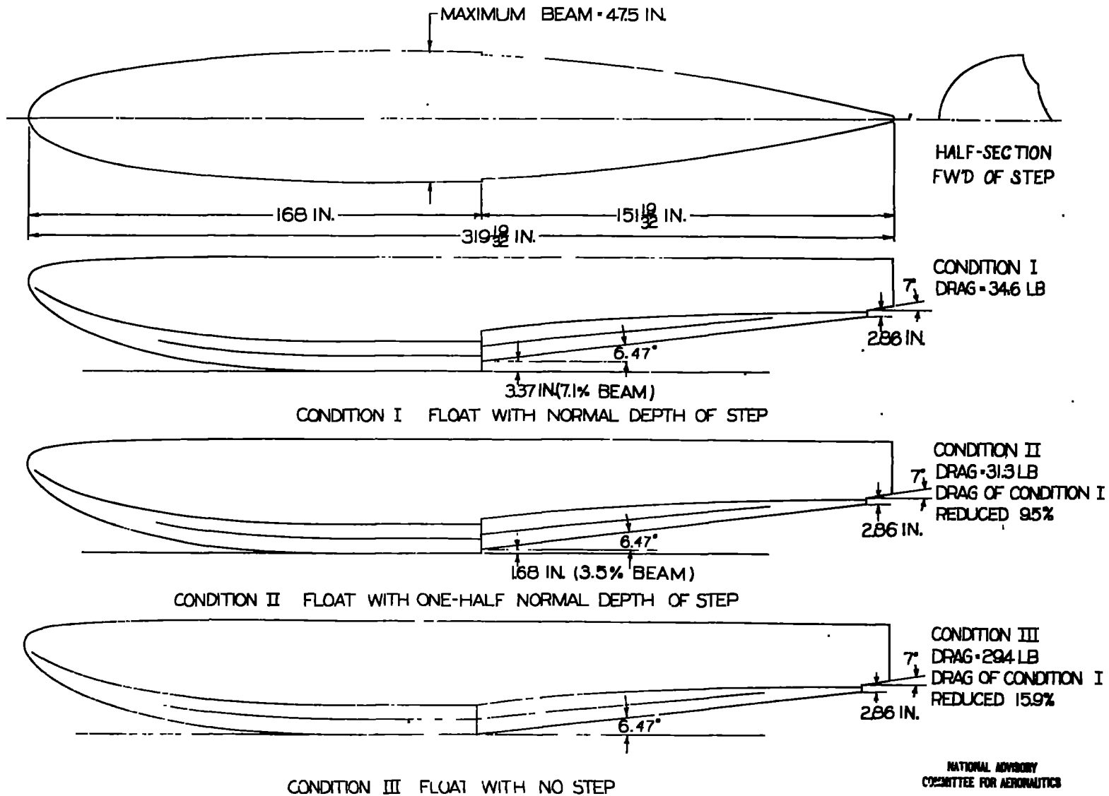
FIGURE 1.-MODIFICATIONS TO A FLOAT FOR THE PURPOSE OF SHOWING THE EFFECT OF THE DEPTH OF STEP ON AIR DRAG AT ZERO PITCH ( V=100 MPH; q=25.6 \frac{LB}{SQ FT} ).
