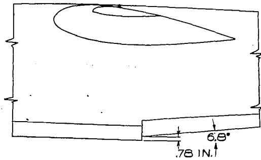
BASIC MODEL MODEL 134A
