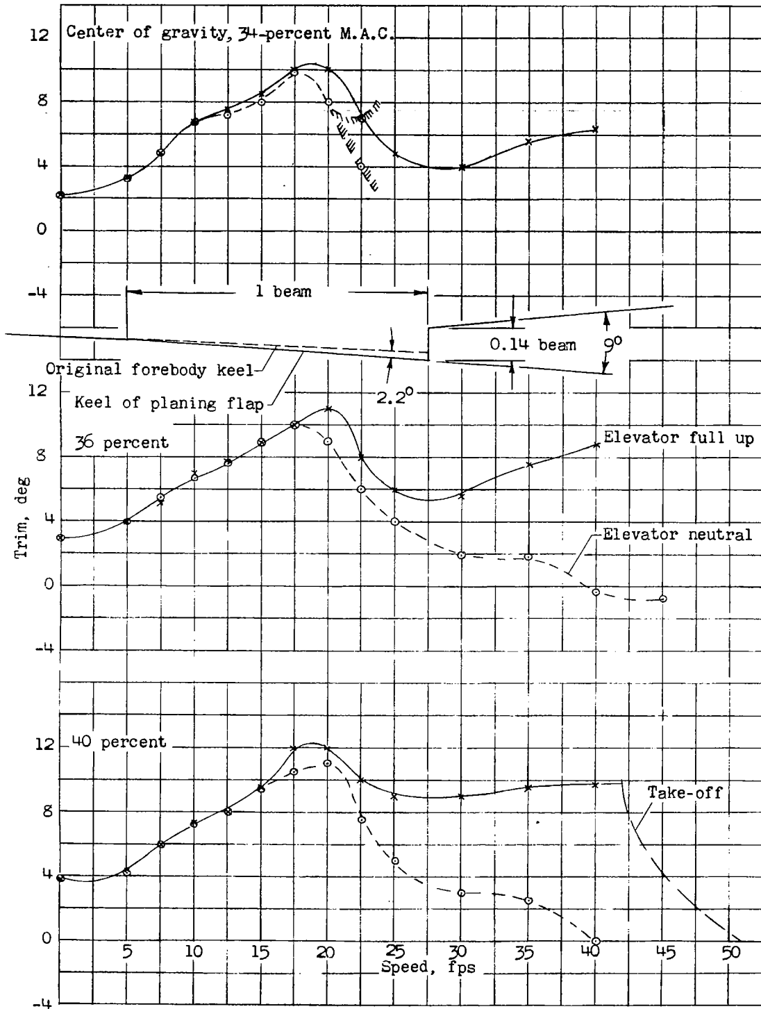
Figure 11.- Model 134PF-3. Variation of trim with speed. Step depth = 0.14 beam, stabilizer 5° up. C_{D0} = 0.87 . Angle of planing flap = 2.2°; chord = 1 beam.
