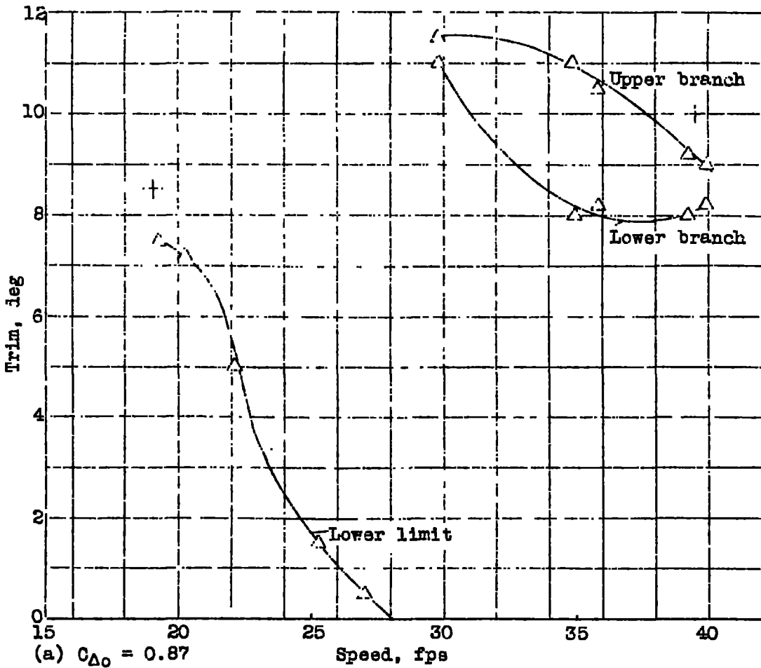
Figure 9 (a,b).- Model 134PF. Variation of trim limits with speed. Depth of step = 0.14 beam.
