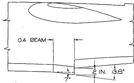
BASIC MODEL WITH PLANING FLAP. DEPTH OF STEP INCREASED TO 2 IN (0.14 BEAM). MODEL 134-PF-2
