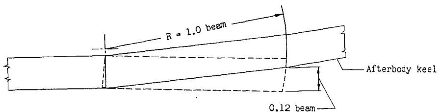
(c) Arrangement having larger angle of afterbody keel. Here the keel and chine of the flap when retracted are inclined at an angle between that of the forebody and afterbody. Dotted lines show flap deflected 2^\circ below forebody keel.
