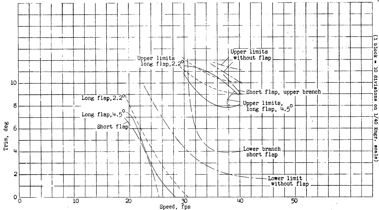
Figure 10.- Comparison of the trim limits of stability for the basic model and for the model fitted with three different planing flaps. C_{\Delta_0} = 0.87 ; depth of step = 0.14 beam; angle of keel of afterbody = 5.5^\circ to base line.
