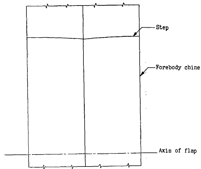
(e) Plan form of step. The departure from the conventional, straight transverse form is small.
