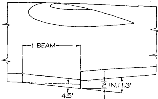
BASIC MODEL WITH PLANING FLAP. DEPTH OF STEP INCREASED TO 2 IN (0.14 BEAM). MODEL 134-PF
