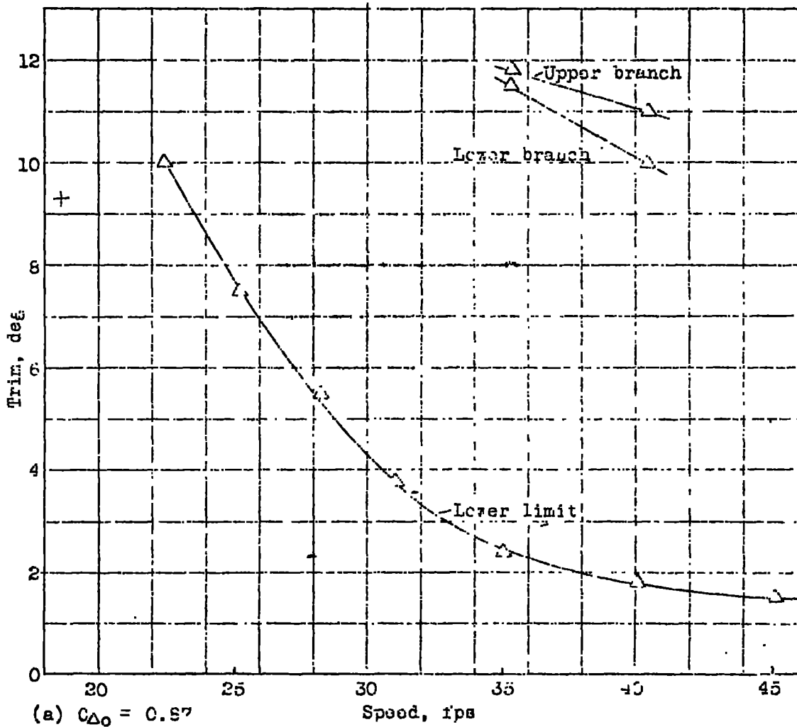
(a) C_{\Delta 0} = 0.87 Figure 6 (a,b).-- Model 134C. Variation of trim limits with speed. Angle of incidence of wing decreased 2\frac{1}{2}^\circ . Model without planing flap.
