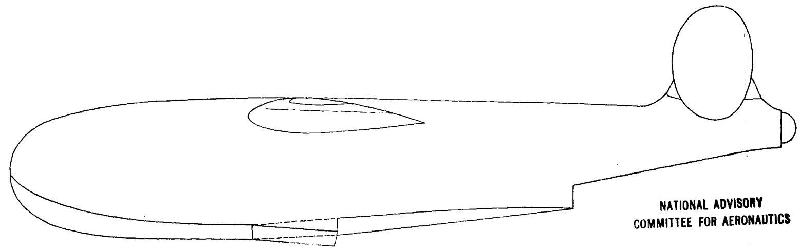
Figure 2.- Profile of model showing flap deflected. Dotted lines indicate flap in retracted position.
