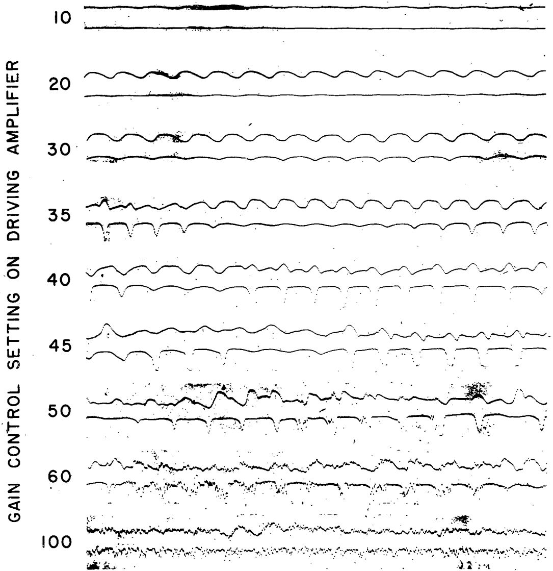
Figure 35.- Oscillograms of u-fluctuations showing development of turbulence from oscillations produced by vibrating ribbon at position 2.5 feet downstream from ribbon. Ribbon 3 feet from leading edge of plate. Simultaneous records at 0.014 inch from surface, upper trace; and 0.114 inch from surface, lower trace. Frequency 70 cps. U_0 = 50 ft per sec.
