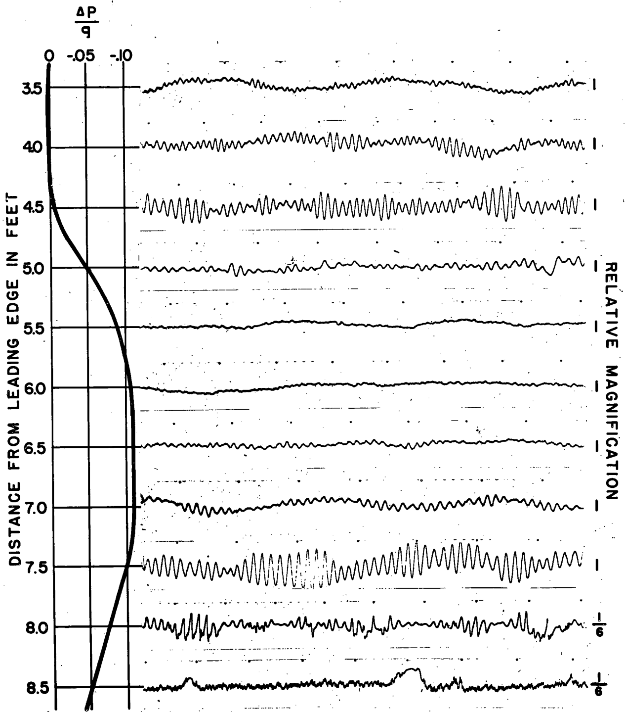
Figure 29.- Oscillograms of u-fluctuations showing effect of pressure gradient on boundary-layer oscillations, Distance from surface = 0.021 inch. U_0 = 95 ft per sec. Time interval between dots = \frac{1}{30} sec.
