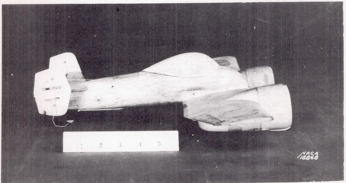
Figure 3.- Side view of 1/22-scale model of Grumman XF5F-1 airplane.
