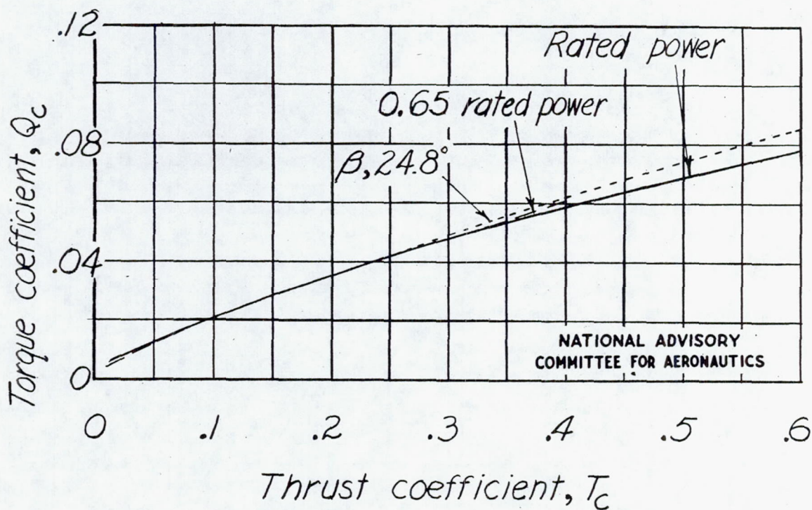
Figure 5.- Comparison of variation of T_c with Q_c for constant-power operation and for the propeller with blade angle fixed at 24.8^\circ at 0.75 radius.
