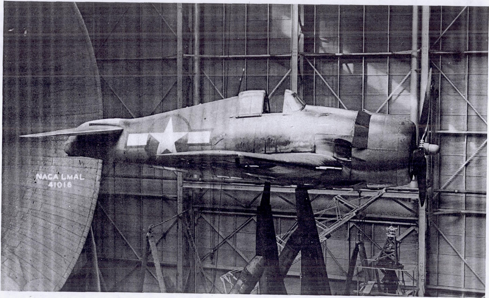
Figure 3.- Three-quarter side view of airplane with vertical tail removed and tail fairing installed.
