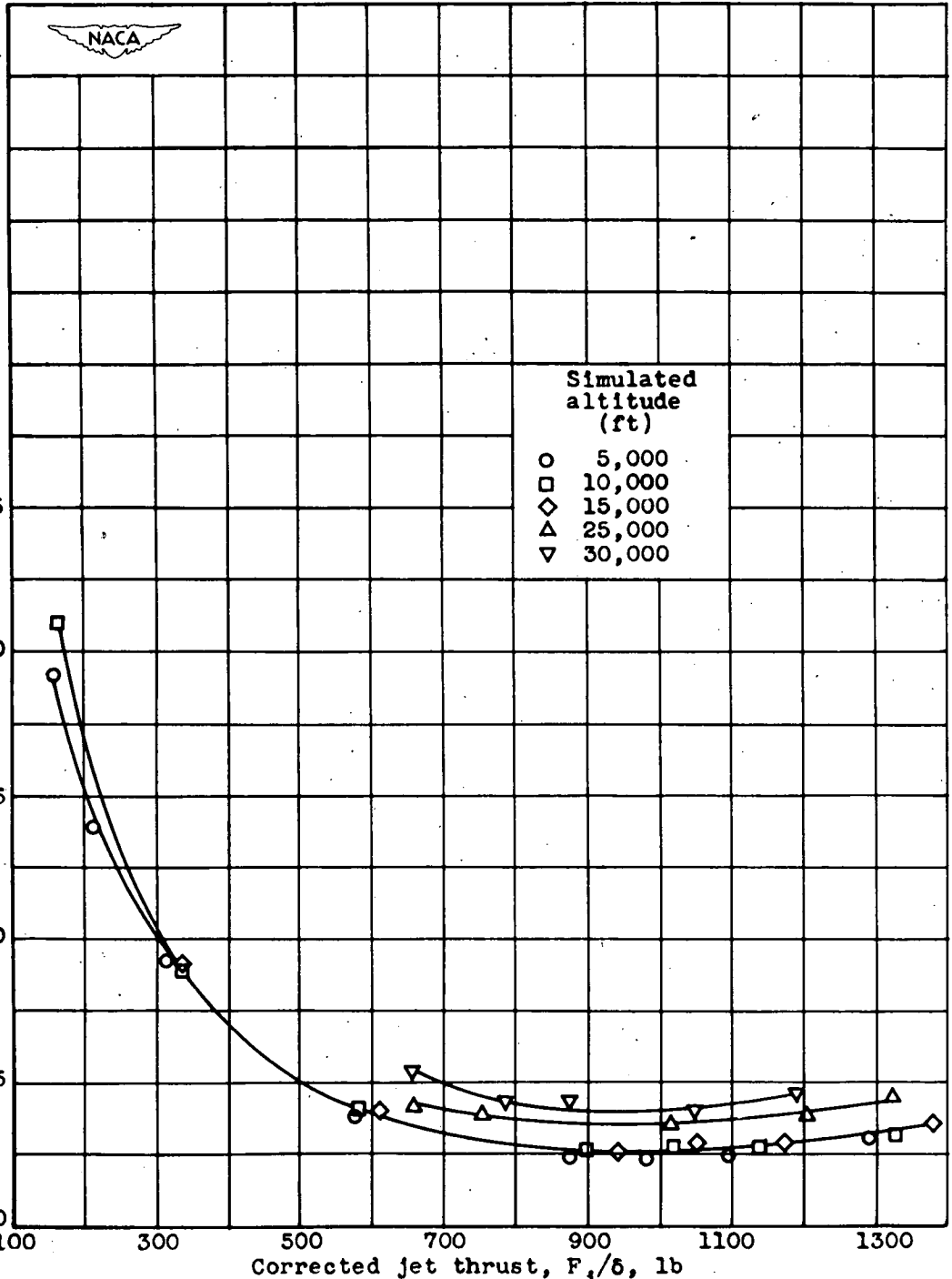
(e) Relation between corrected specific fuel consumption based on jet thrust and corrected jet thrust.
