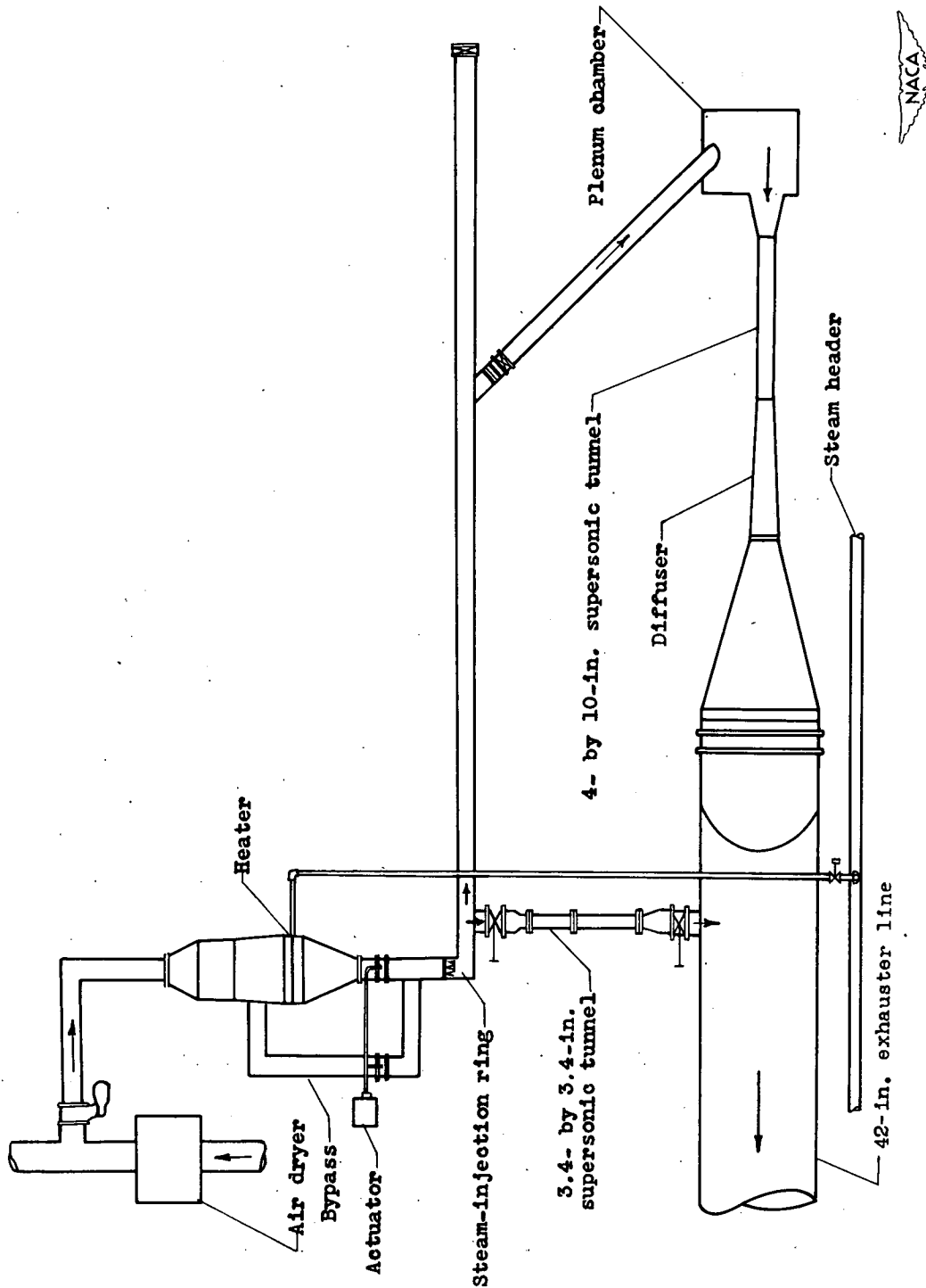
Figure 3. - Diagrammatic sketch of tunnel system.
