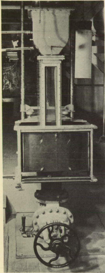
(a) 3.4- by 3.4-inch tunnel nozzle installation with included angle of 3.50^\circ ; nozzle in place; Mach number, 2.00.
