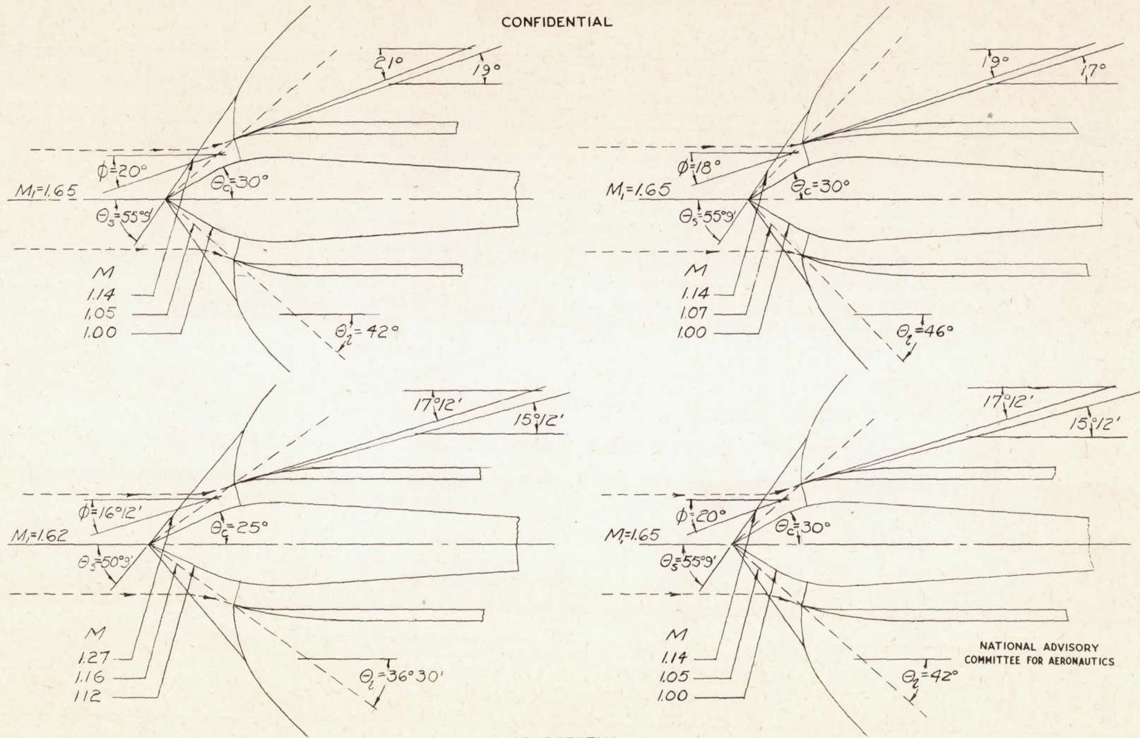
Figure 13.- Schematic diagram of the aerodynamic phenomena.
