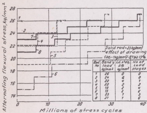
Figure 14.- Variation of the flexural fatigue strength through understress effect, unalloyed steel with 0.2 percent C (F. Körber).
