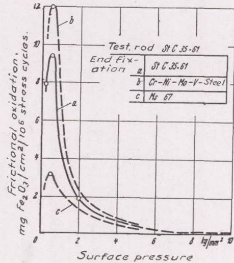
Figure 21.- Frictional oxidation as a function of surface pressure and material saving in the juncture for St C 35-61.
