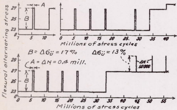
Figure 9.- Variation in the flexural fatigue strength of an unalloyed annealed steel with 0.2 percent C in overloading (F. Körber).
