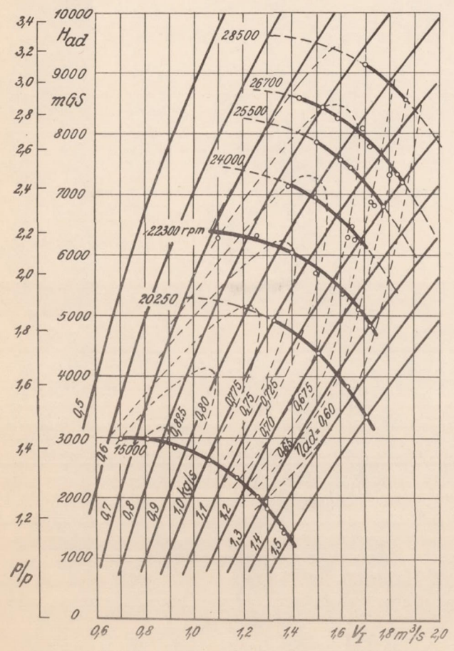
Figure 12.- Characteristic curves of DVL experimental supercharger.
