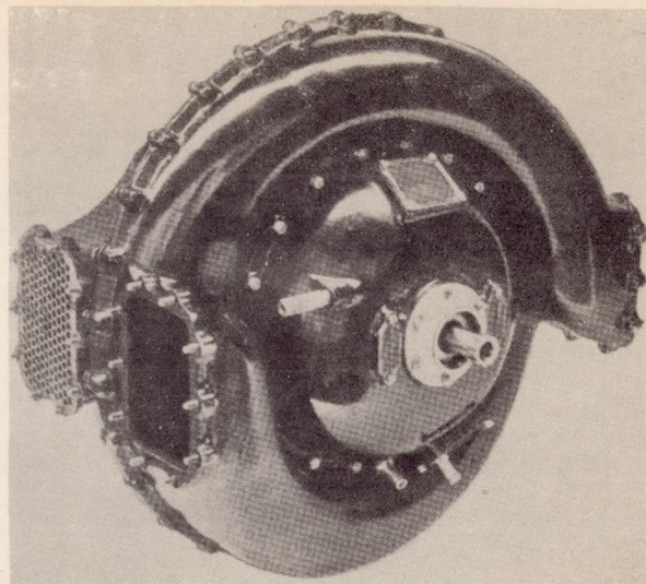
Figure 8.- Booster for Bristol Pegasus XVIII.
