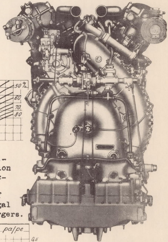
Figure 3.- Rolls-Royce Merlin engine - supercharger side.
