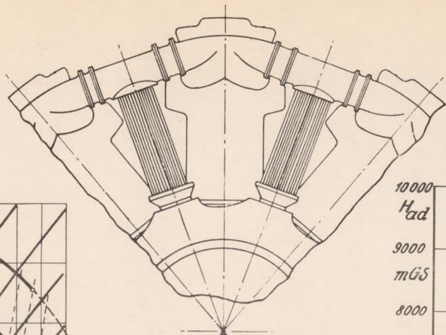
Figure 9.- Intercooler, Bristol patent.
