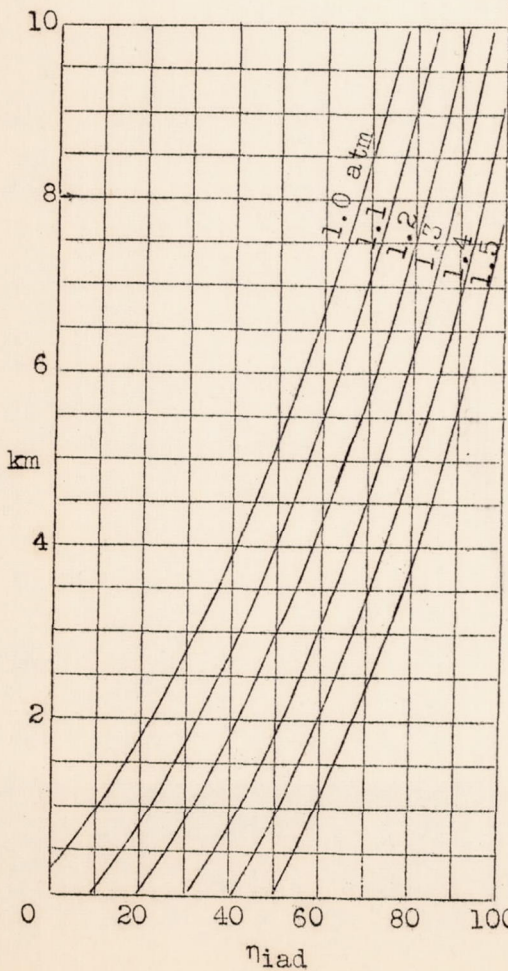
Figure 6.- Attainable rated hp height against supercharger end pressure (for 80°C induction pressure).
