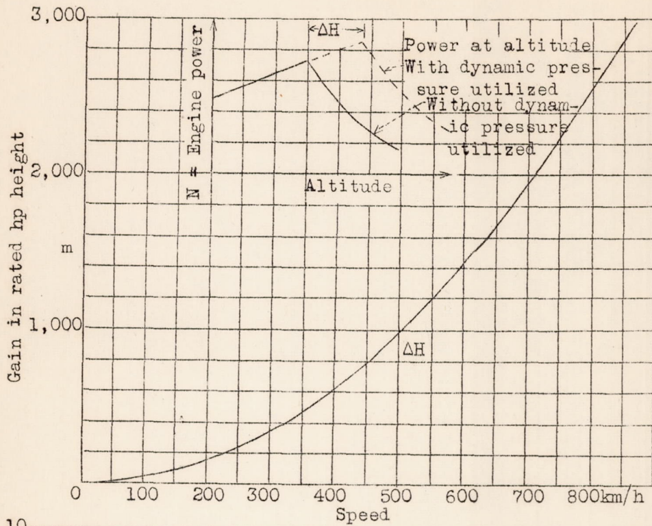
Figure 4.- Height gain at different flying speeds
