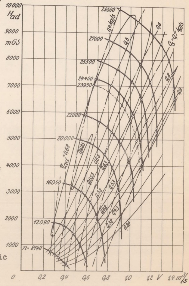
Figure 12.- Characteristic curves of DVL experimental supercharger.
