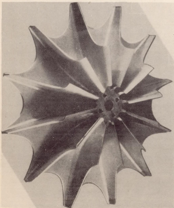
Figure 10.- Rotor of DB600-880g
