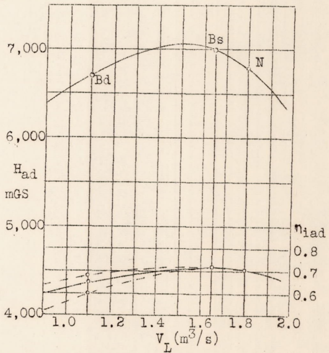
Figure 14.- Characteristic curves of a centrifugal supercharger.
