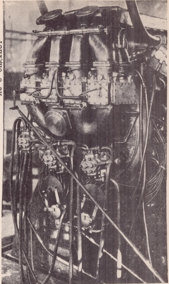
Figure 12.- Carburetors and fuel pumps. AS 6 engine.
