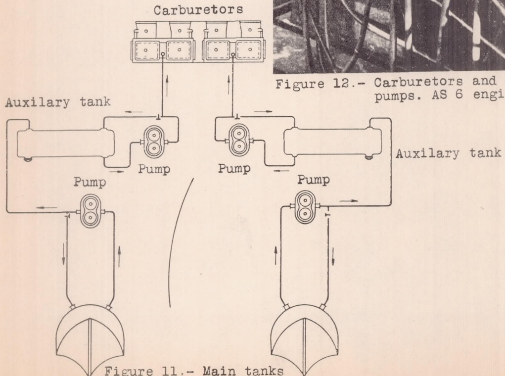
Figure 11.- Main tanks in the floats.
