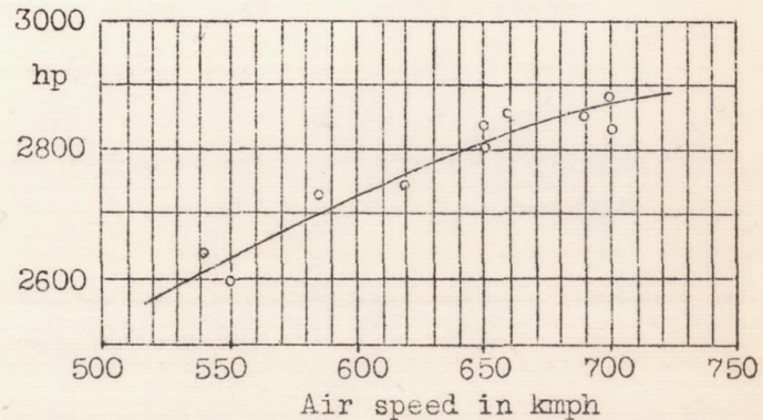
Figure 15.-Variation of power with air speed at 3200 rpm. Fiat engine AS6.
