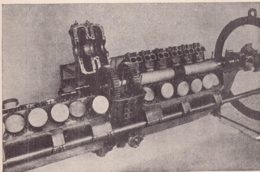
Figure 9.- AS 6 engine disassembled
