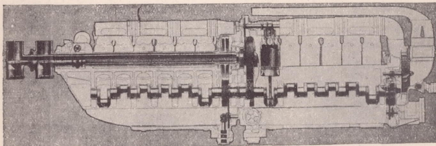
Figure 8.- Section of AS 6 engine.
