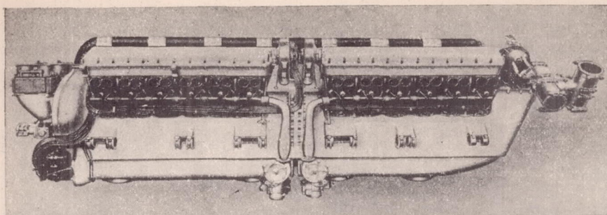
Figure 7.- Fiat AS 6 engine.
