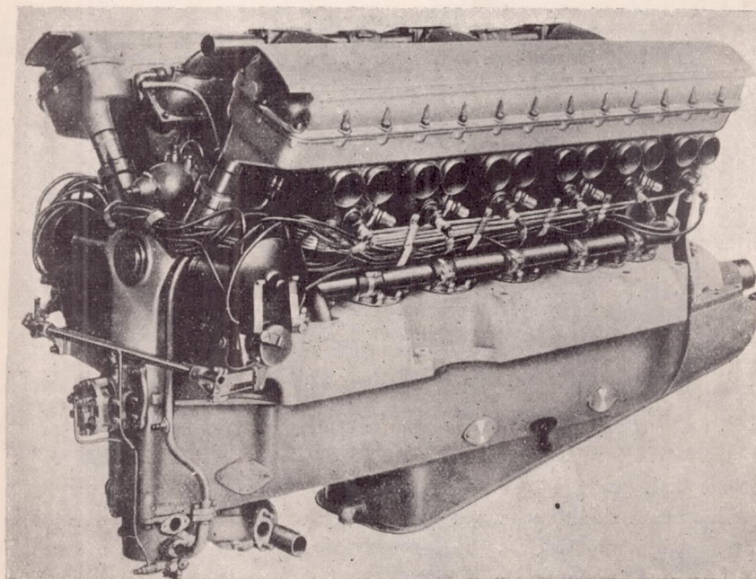
Figure 6.- Fiat AS 5 engine.
